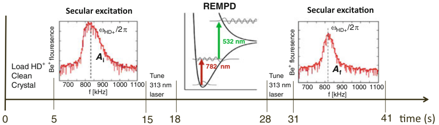
Fig. 3 The secular scan—REMPD—secular scan detection scheme. At the start of each cycle, a new sample of \text{HD}^+ ions is loaded into the ion trap. During loading the \text{Be}^+ ions are exposed to neutral \text{HD} gas, leading to the formation of a small number of \text{BeH}^+ and \text{BeD}^+ ions (see also Table 1). These are expunged from the trap by applying a dc quadrupole potential of \sim 0.9 \text{ V} , which reduces the trap depth such that only ions with mass \leq 9 \text{ amu} remain trapped. Five seconds after loading, the \text{HD}^+ is motionally excited by scanning an rf electric field over the secular motional resonance frequency at 830 kHz. A 313 nm laser detuning of -300 \text{ MHz} is used, in which case the secular excitation results in a rise in the \text{Be}^+ fluorescence. Ten seconds later, the 313 nm laser is tuned to -80 \text{ MHz} from the \text{Be}^+ cooling transition, and its intensity reduced to I \sim 2I_{\text{sat}} . After 10 s of REMPD, the 313 nm laser settings are restored to their values as used for the first secular scan, and a second secular scan is executed. A smaller 313 nm fluorescence peak indicates loss of \text{HD}^+
