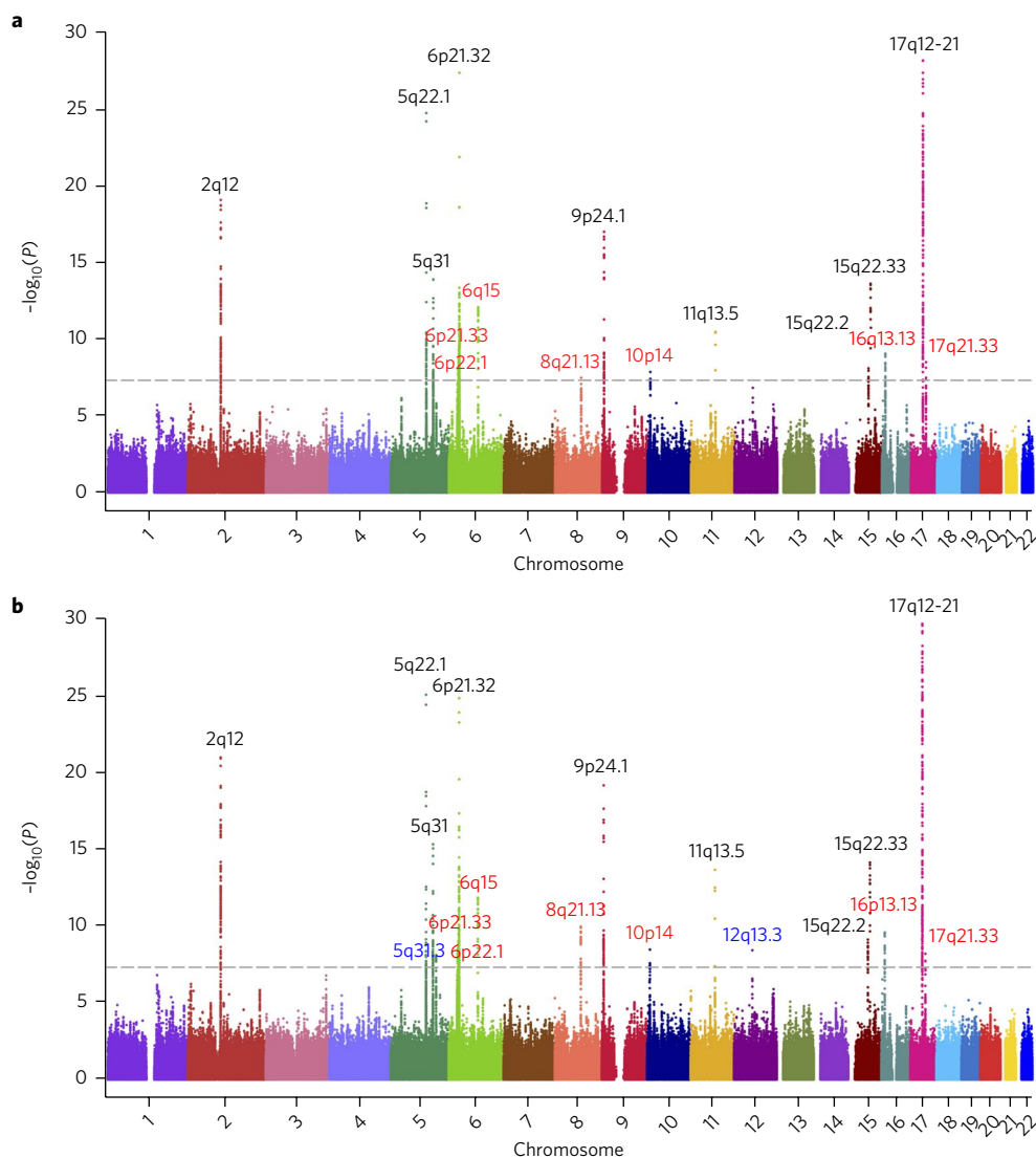
Fig. 1 | Manhattan plots of the results of European-ancestry and multiancestry random-effects meta-analyses of asthma risk. a , The European-ancestry meta-analysis pertains to 19,954 asthma cases and 107,715 controls. b , The multiancestry meta-analysis pertains to 23,948 asthma cases and 118,538 controls. Each locus is annotated according to its cytogenetic-band location. The x axis represents chromosomal location, and the y axis represents -\log_{10}(P) value for tests of association between SNPs and asthma. Black, previously known loci; red, new loci identified in the European-ancestry meta-analysis; blue, additional new loci identified in the multiancestry meta-analysis. The dashed horizontal line denotes P=5 \times 10^{-8} .
