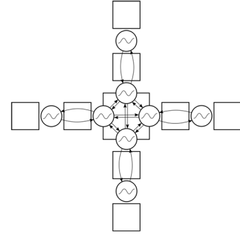
Figure 2: Schematic view of the CPG network generated for the body shown in the top-left panel of Fig. 3. The rectangular shapes indicate passive body parts, the circles show active hinges, each with their own differential oscillator, and the arrows indicate the connections between the oscillators.
