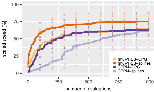
Figure 4: Learner and controller performances for the three size variations of the “spider” morphology. To adjust for the higher speeds obtained by the larger robots, the performances are normalised and combined into a single plot. The lines show the averaged best result and the dots indicate the performance of the separate runs.
