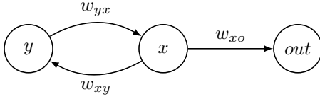
Figure 1: A differential oscillator with output node as used in the CPG controller.
