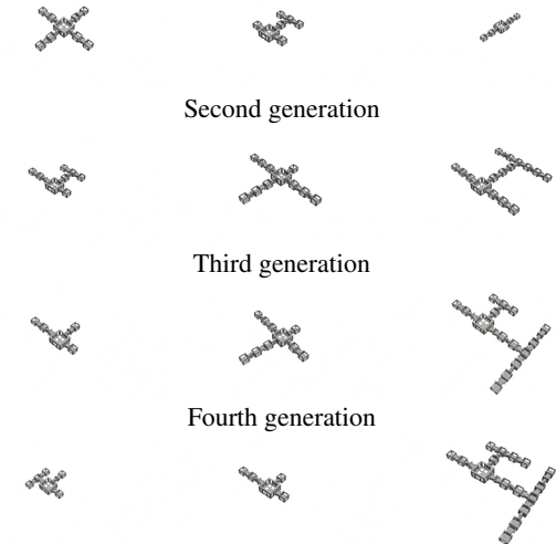
Figure 3: The morphologies used in this study. The top row shows the smallest versions of the three hand-designed initial morphologies. The following rows of robots result from recombination and mutation of the previous generations.
