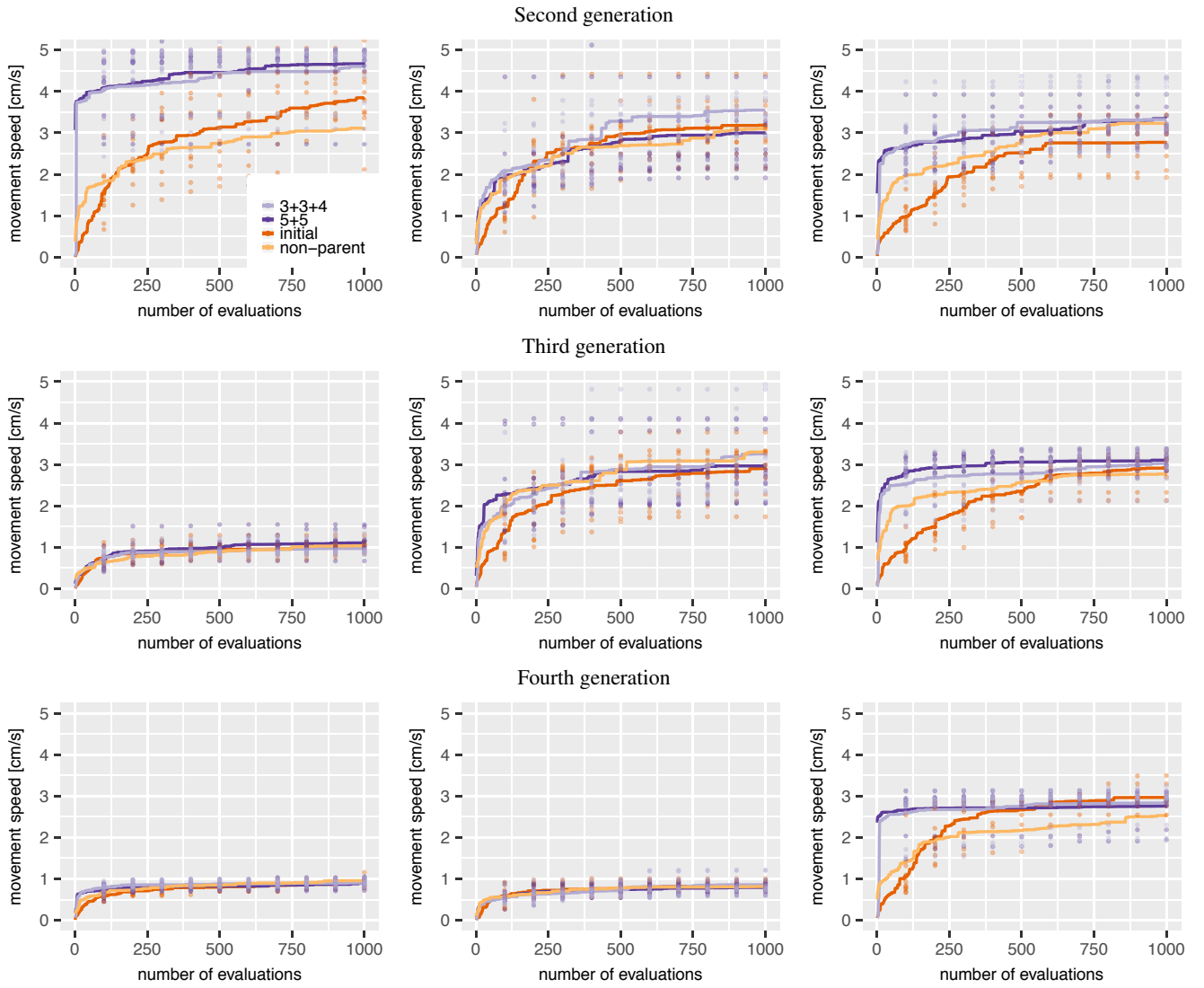
Figure 5: Results from running lifetime learning on offspring with new morphologies, using either re-initialized CPPNs ( initial ), CPPNs from the non-parent robot, 5 CPPNs from each parent ( 5+5 ), or a mix between re-initialized and 3 CPPNs from each parent ( 3+3+4 ). All learning methods are run 10 times, lines show the mean and dots show the individual run results. The plots are arranged coincidentally with the images in Fig. 3.
