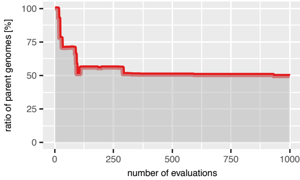
Figure 6: Percentage of parental genetic material in the best-performing CPPNs as lifetime learning progresses for the first depicted robot in the second generation.
