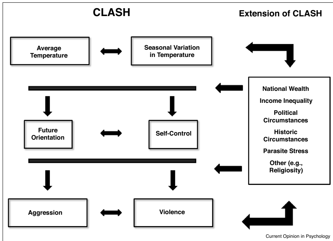
A schematic model of CLASH (adapted from Ref. [15**]) and its extensions.
