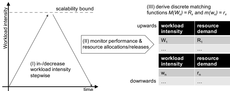
Figure 2.1: Illustration of a measurement-based derivation of matching functions
