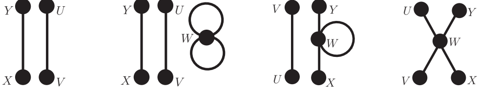
FIG. 2: Four-point function at leading order in 1/\kappa_4 .
