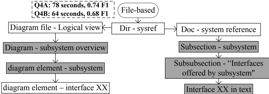
Figure 4: AK organisation for answering experiment questions at Océ
