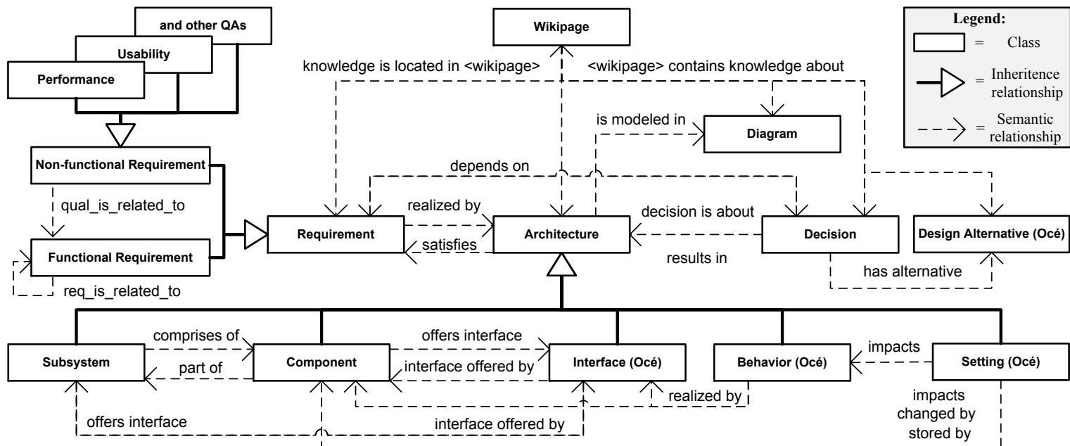
Figure 2: Software ontology extended for the Océ experiment domain
