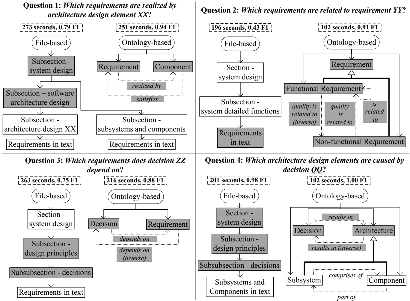
Figure 5: AK organisation for answering experiment questions at LaiAn
