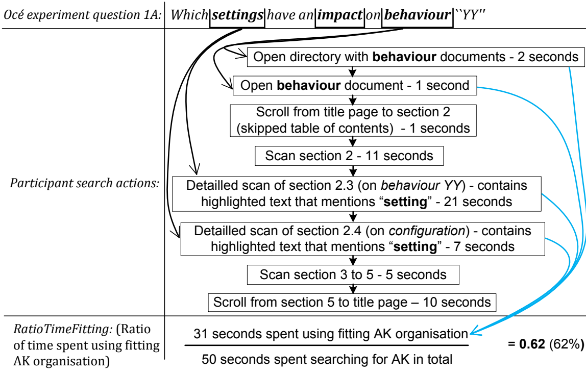
Figure 6: Example calculation of RatioTimeFitting from search actions of a participant using the file-based approach
