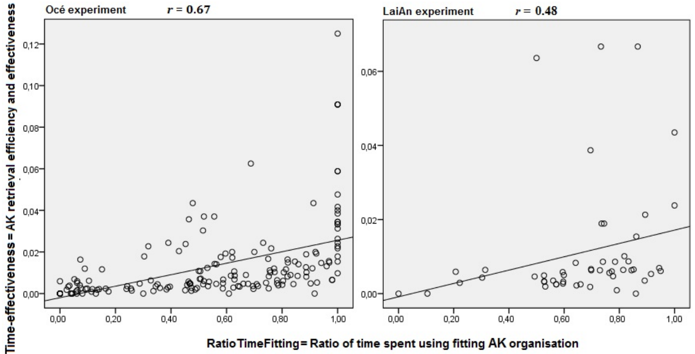
Figure 7: Correlation between RatioTimeFitting and Time-effectiveness when answering Océ and LaiAn experiment questions using both documentation approaches
