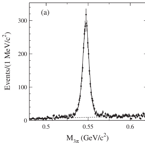
FIG. 4. The (a) \pi^+\pi^-\pi^0 and (b) \pi^+\pi^-\eta mass spectra for data events with 4 < Q^2 < 40 \text{ GeV}^2 . The solid curves are the results of the fits described in Sec. IV. The dashed curves represent non-peaking background.
