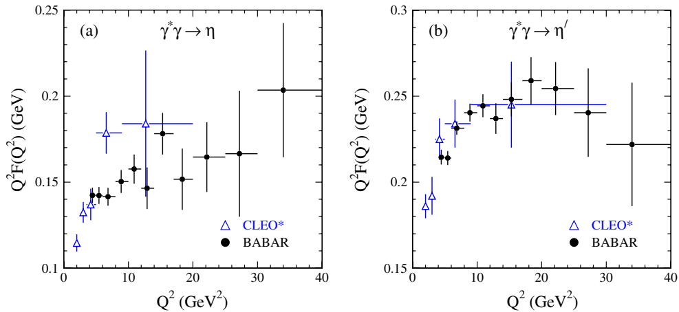
FIG. 15 (color online). The transition form factors multiplied by Q^2 for (a) \gamma\gamma^* \rightarrow \eta and (b) \gamma\gamma^* \rightarrow \eta' .
