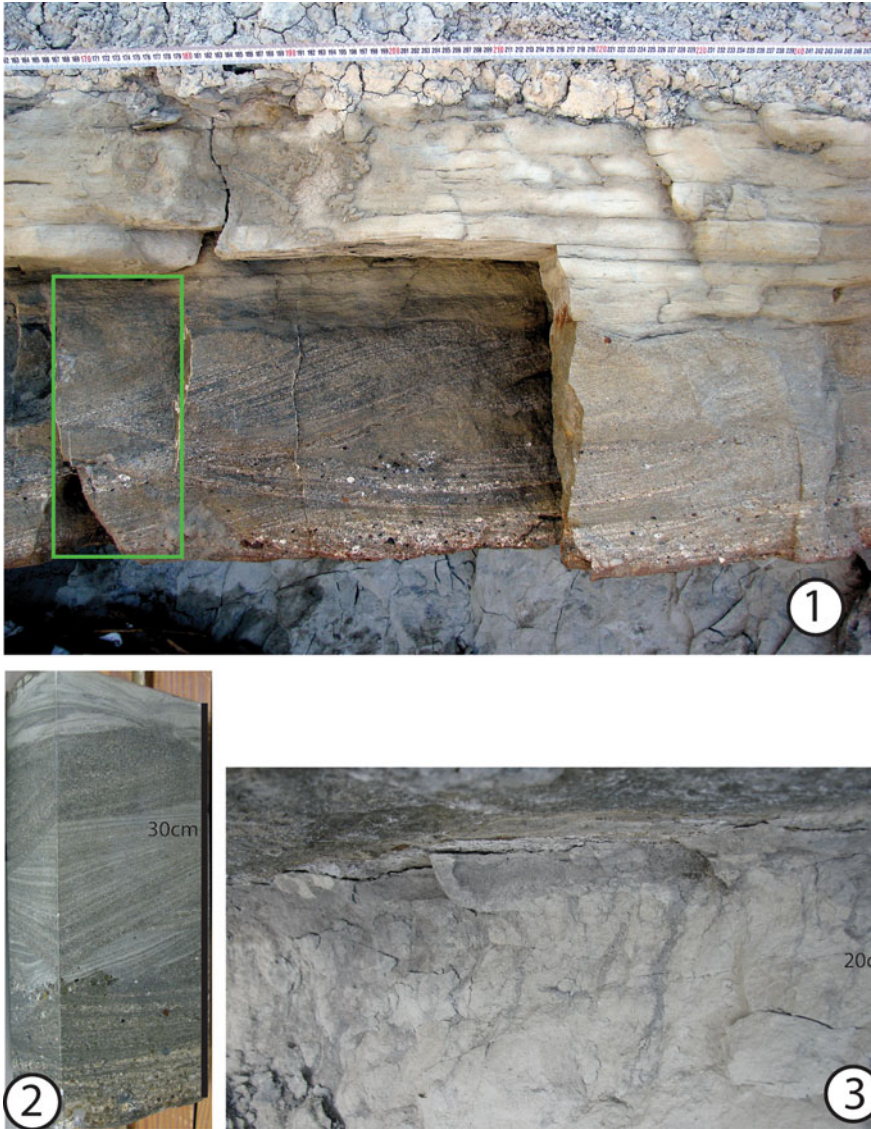
Fig. 10 Tsunamiite Ts2 with two coarse layers displaying trough cross-bedding (1) Graded trough cross-beds and inset of (2). 2 On perpendicular planes polished block of the lower bed of Ts2, taken at the green inset in (1). The two orientations made it possible to infer a paleocurrent direction toward the SW. Black chert , limestone and limnocardium bivalves are the main components. 3 Top of the mudstones directly underlying Ts2, containing many 5- to 15-cm-long fissures filled with coarse sand. The planar shape of the fissures makes it unlikely that these are plant roots in a soil, as suggested by Roveri et al. (2005)
