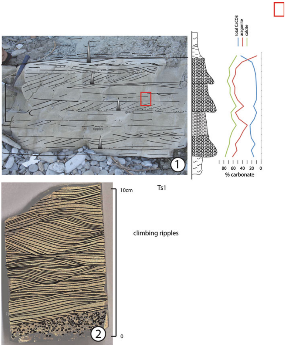
Fig. 9 Lowest tsunamite (Ts1). 1 Stack of three graded and cross-bedded sublayers, each eroding in the underlying mudstones or the underlying bed. The fourth graded unit is the settling unit into silts and clay from the suspension cloud. Right, TGA calcite and aragonite analyses. 2 polished slab of the inset of (1). These fine-to-medium sand intervals show several climbing-ripple intervals. At a different oriented section, these ripples can be easily interpreted as HCS and lead to a tempestite interpretation
