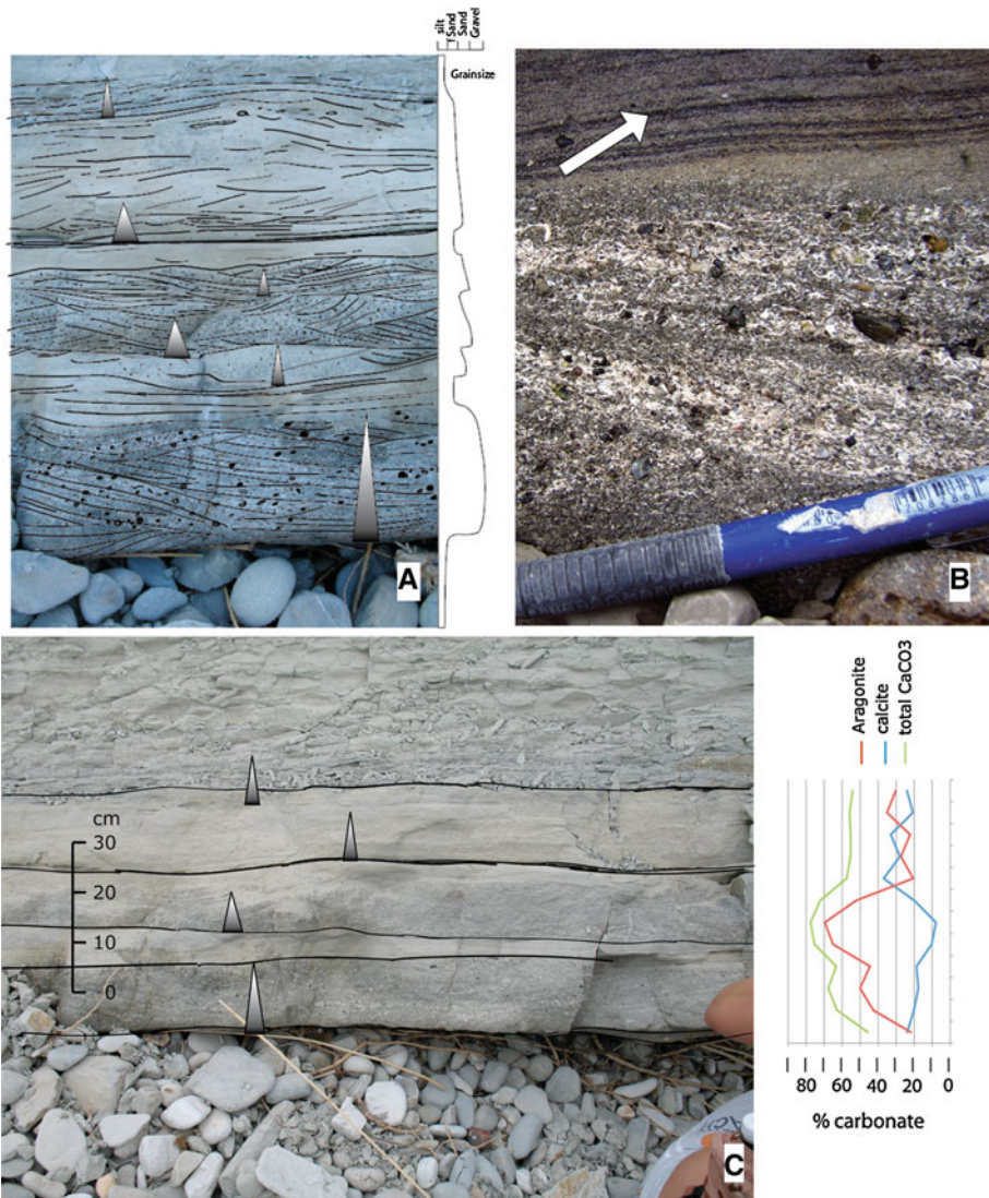
Fig. 11 Tsunamiite Ts2 with two coarse layers displaying trough cross-bedding (a) Outlined foreset lamina and graded beds. At least 6 graded beds visible in Ts2. b Details of the coarsely laminated cross-bedding of the lowest bed. Black chert , limestone and current-stable bivalves are the main components. Arrow points to lamina with abundant plant debris in the finer grain size interval between the coarse beds. c Ts2 layer with two tabular trough cross-bedded beds. The many broken bivalve shells cause the high aragonite content compared to the mudstones below
