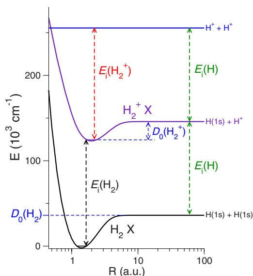
FIG. 5. (Color online) Potential energy diagram showing the potential energy functions of the X^1\Sigma_g^+ ground state of H 2 and the X^+ 2\Sigma_g^+ ground state of H 2 + and illustrating the relationship between the various ionization and dissociation energies.
