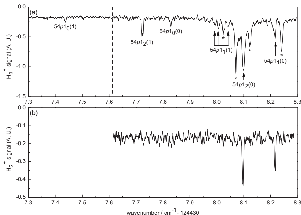
FIG. 2. Field ionization spectra of H_2 in the region of transitions to the 54p Rydberg states recorded using 397 nm laser pulse energies of (a) 700\ \mu\text{J} and (b) 40\ \mu\text{J} . The vertical dashed line indicates the junction point of two different scans. The scan on the low wave number side was taken with a smaller frequency step size and more averaging for each data point to increase the signal-to-noise ratio. The wave numbers are given relative to the position of the X\ 1\Sigma_g^+(v=0, N=0) ground state of para- H_2 .
