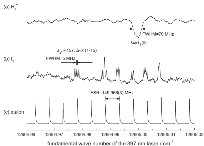
FIG. 3. Spectrum showing the transition from the EF\ ^1\Sigma_g^+(v=0, N=1) level to the 54p1_1(0) level (a) with the I_2 calibration (b) and etalon (c) traces. The position of the a_2 hyperfine component of the P157, B-X (1–15) rovibronic transition of I_2 was determined to be at 377 886 781.37(10) MHz using a frequency comb.
