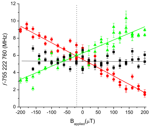
FIG. 8. (Color online) Transition frequency for the 4s^2S_{1/2}-4p^2P_{1/2} transition in \text{Ca}^+ with respect to an applied magnetic field B_{\text{applied}} . Three different polarizations were used (see text): Right-circular ( \sigma^+ , green triangles), left-circular ( \sigma^- , red circles), and linearly polarized light ( \sigma^++\sigma^- , black squares). The dotted line indicates the value of the applied field where B_{\text{applied}}=-B_{\text{earth}} .
