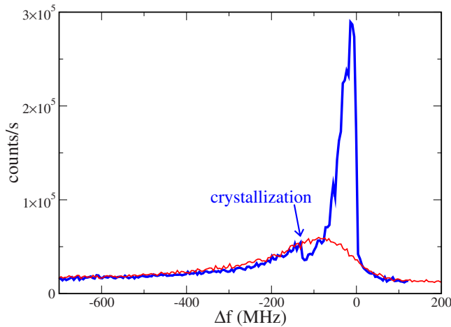
FIG. 4. (Color online) Observed fluorescence vs frequency detuning \Delta f , on scanning the cooling laser over the 4s^2S_{1/2}-4p^2P_{1/2} transition in \text{Ca}^+ . Red thin trace, T_{\text{ions}} \approx 40 K; blue thick trace, T_{\text{ions}} \approx 4 K. The sudden decrease in fluorescence in the blue thick curve is the typical signature for crystallization of the ion cloud (see text).
