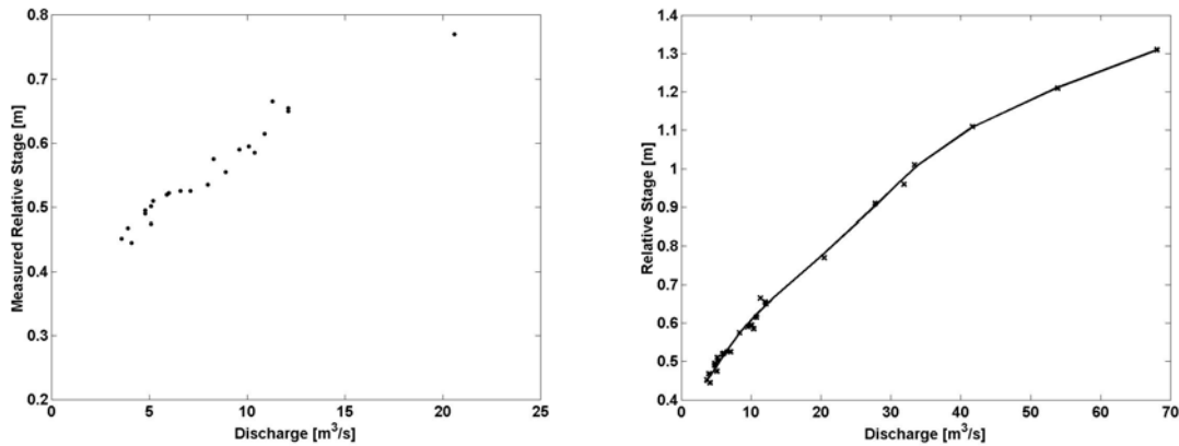
Figure V.9. (a) Measured stage-discharge relation for the Rio Chiquito (northern Costa Rica) and (b) Extrapolated discharge data and fitted rating curve.
