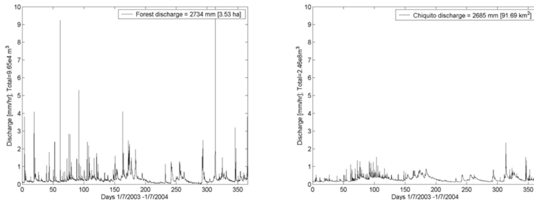
Figure V.1. Streamflow patterns for a micro-catchment (3.5 ha) under cloud forest (left-hand panel) and a meso-scale catchment (92 km 2 ) with mixed (cloud) forest and pasture (right-hand panel), northern Costa Rica
