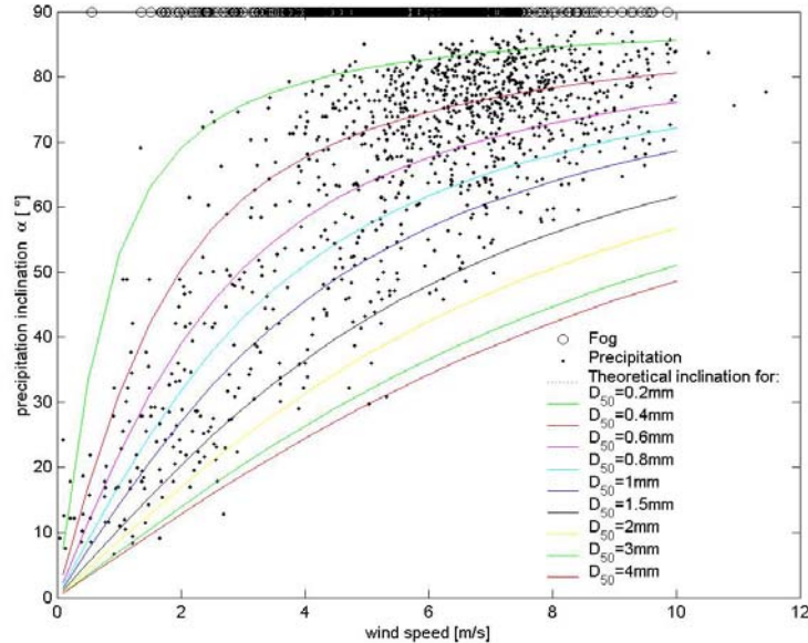
Figure II.26. Precipitation inclination as a function of wind speed. Lines represent theoretical relationships based on terminal velocities for different median droplet diameters. Dots represent measured inclinations (see next section).
