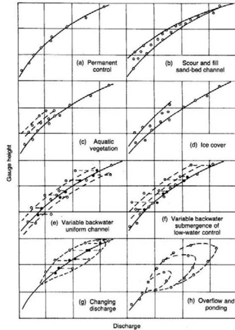
Fig. 4.4 Rating curves for different hydraulic conditions.
