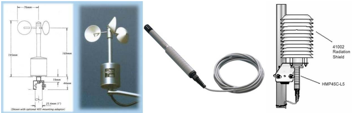
Figure III.12. Cup anemometer (Vector Instruments, left), Vaisala temperature and humidity sensor (HMP45, middle) and radiation shield housing Vaisala temperature and humidity sensor (right).
