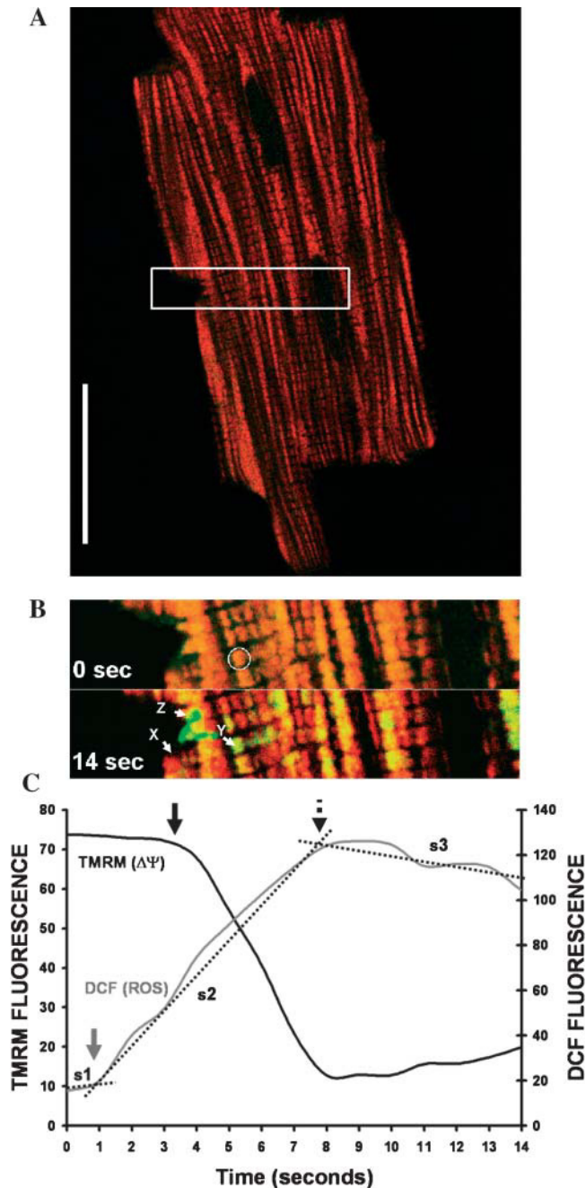
FIGURE 2 Localized photoexcitation of TMRM: dynamics of \Delta\Psi - and ROS production at the level of a single mitochondrion. The 0.2- \mu\text{M} TMRM and 10.0- \mu\text{M} DCF fluorescence were measured in mitochondria of a typical rat cardiomyocyte (as shown labeled with TMRM in A). (B) From t = 0 onwards, confocal imaging of DCF and TMRM fluorescence was confined to the region bounded by the white box and repeated each second, simultaneously recording the decrease in TMRM fluorescence (which reports changes in \Delta\Psi ) and increase in DCF fluorescence (which reports on the presence of ROS). (C) The kinetics of depolarization and ROS production in a single mitochondrion ( \circ in B). The arrows ( shaded for DCF and solid for TMRM) indicate the time points where a significant change occurred. Three lines ( s1 , s2 , and s3 ) refer to the slopes (rates) of changes in DCF fluorescence. Arrow 1 ( shaded ) indicates the shift to a faster increase in DCF fluorescence ( intersection of s1 and s2 ), arrow 2 ( solid ) indicates the point at which \Delta\Psi began to decrease, arrow 3 refers the point at which DCF
