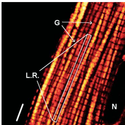
FIGURE 1 Organization of the mitochondria of an isolated cardiomyocyte. A rat cardiomyocyte was loaded with 0.2 \mu\text{M} TMRM, and a 0.7\text{-}\mu\text{m} optical section of the cell was imaged at a high spatial resolution ( 3\times Kalman averaging). This figure is representative of images used to calculate characteristics of mitochondria arranged longitudinally along the myofibrils (Table 1). L.R. is an example of a measured longitudinal row, N is a nucleus, and G refers to the longitudinal gaps between mitochondria. Scale bar = 5 \mu\text{m} .
