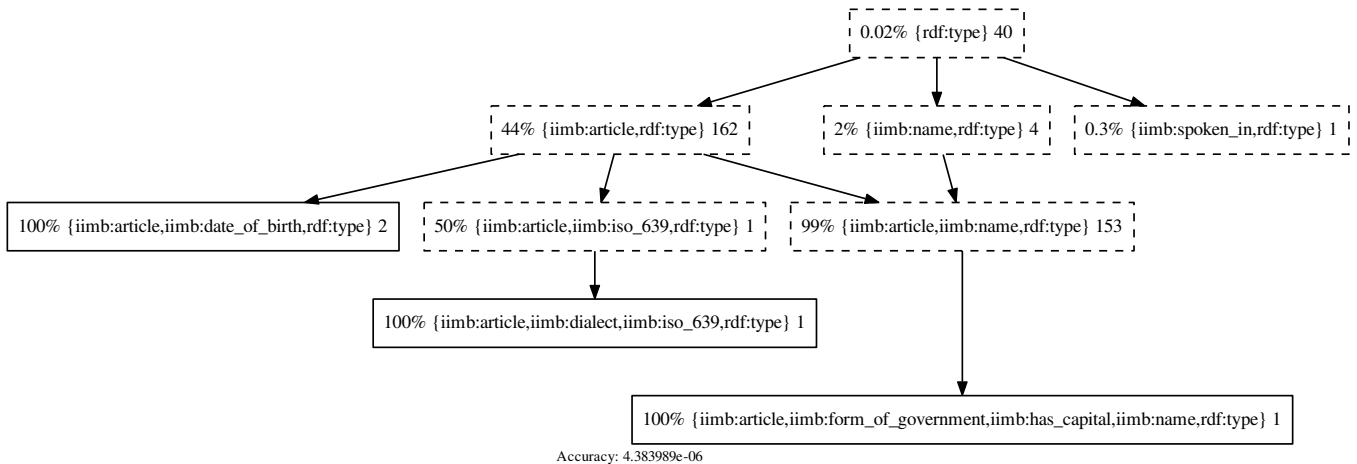
Figure 1: An example of a discernibility partition for an identity relation consisting of 365 pairs applied to the fourth IIMB linkset. Each node is annotated with the set of predicates P for which its pairs are P -indiscernible. The number of identity pairs within each partition set is displayed to the right of the predicate set label. Partition sets that contain no identity pair are not shown. The number that occurs to the left of the predicate label in each node indicates how many pairs in that node are identity pairs. The lower approximation consists of the nodes with a solid border, indicating that they contain only identity pairs. The higher approximation consists of all displayed nodes.
