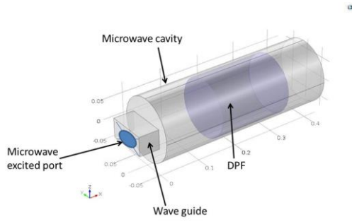
Figure 5: COMSOL geometry of the proposed microwave cavity
