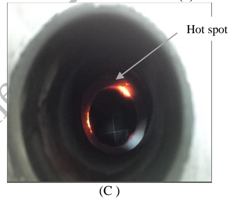
Figure 2: DPF at various stages (a) Clean DPF (b) Soot filled DPF and (C) DPF in microwave filed with glow.
