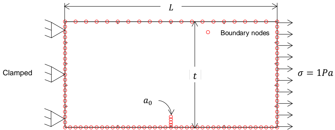
Figure 8. SENT schematic
