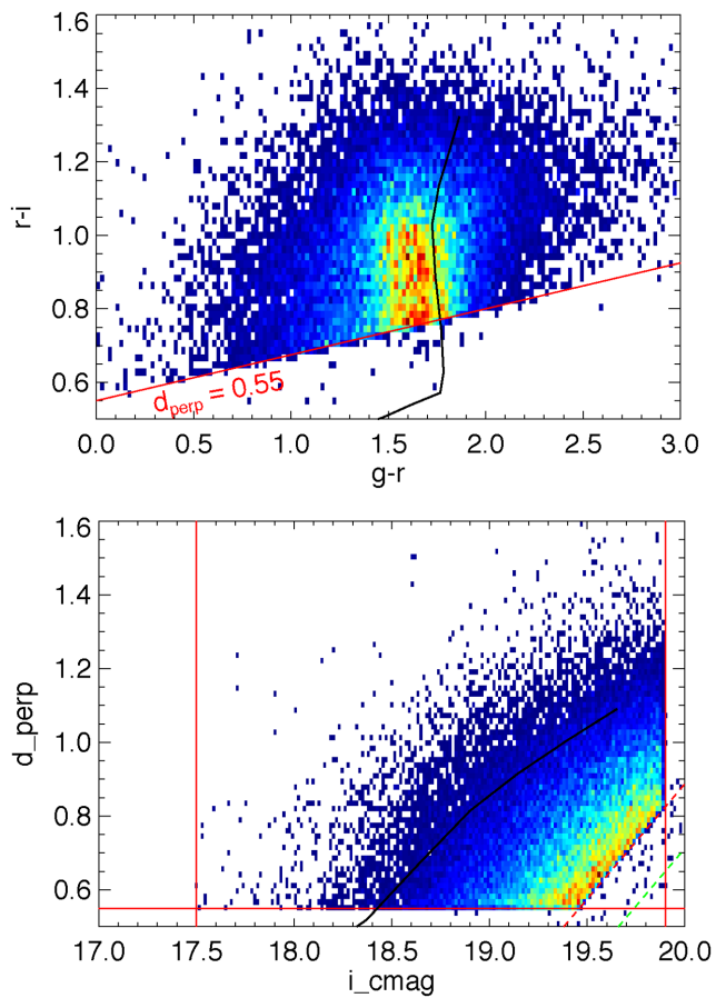
Figure 4. Both panels show density plots of CMASS galaxies; red corresponds to higher density and dark blue to lower density in an arbitrary normalization and linear scale. The black thick line shows the passively evolving LRG model of Maraston et al. (2009). Top: redshift increases upwards, starting at z \simeq 0.4 at d_{\perp} = 0.55 . Bottom: the sliding cut in d_{\perp} with i -band magnitude, designed to select an approximately stellar-mass complete sample. Stellar mass increases with the perpendicular distance to the sliding cut, represented here by the red dashed line – see Maraston et al. (2013) for details. The green dashed line shows the sliding cut adopted for the CMASS SPARSE sample (see Section 3.4). Vertical solid lines show the magnitude limits. On both panels, the small fraction of targets that lie outside of the selection cut are due to differences in the targeting and final photometry, see Section 2. Only chunks greater than 6 are shown.
