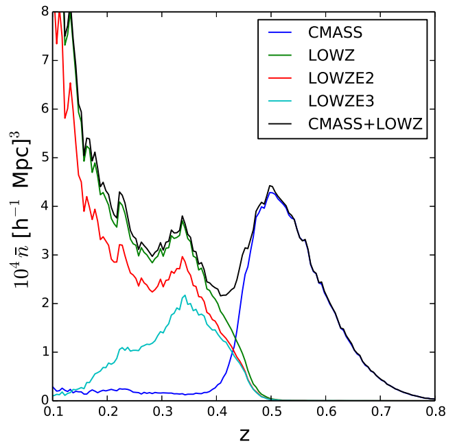
Figure 11. Number density of all four target classes assuming our fiducial cosmology with \Omega_m = 0.31 , along with the sum of the CMASS and LOWZ number densities (black).
