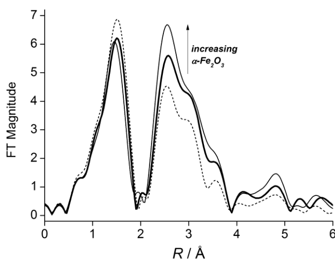
Figure 8 Fourier transform magnitudes of EXAFS spectra of MIL-100( \text{Sc}_{80}\text{Fe}_{20} )XS, MIL-100( \text{Sc}_{60}\text{Fe}_{40} )XS and MIL-100( \text{Sc}_{50}\text{Fe}_{50} )XS materials, showing increasing intensity in higher shells characteristic of \alpha - \text{Fe}_2\text{O}_3
