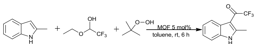
Scheme 3 Tandem Friedel-Crafts addition and oxidation reaction of 2-methylindole with trifluoroacetaldehyde ethyl-hemiacetal and tert-butyl hydroperoxide
