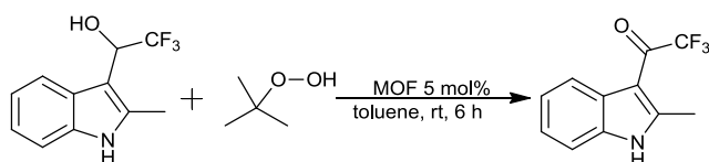
Scheme 5 Oxidation of 2,2,2-trifluoro-1-(2-methyl-1H-indol-3-yl)ethanol using tert-butyl hydroperoxide
