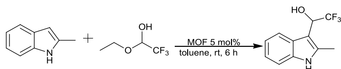
Scheme 4 Friedel-Crafts addition of trifluoroacetaldehyde ethyl-hemiacetal to 2-methylindole
