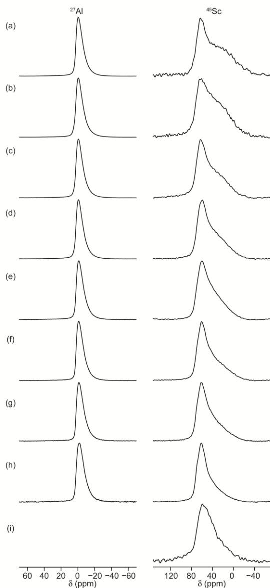
Figure 3. ^{27}\text{Al} (left) and ^{45}\text{Sc} (right) MAS NMR spectra (14.1 T) of MIL-100(Sc,Al) samples (a) \text{Sc}_{10}\text{Al}_{90} , (b) \text{Sc}_{20}\text{Al}_{80} , (c) \text{Sc}_{30}\text{Al}_{70} , (d) \text{Sc}_{40}\text{Al}_{60} , (e) \text{Sc}_{50}\text{Al}_{50} , (f) \text{Sc}_{60}\text{Al}_{40} , (g) \text{Sc}_{70}\text{Al}_{30} , (h) \text{Sc}_{80}\text{Al}_{20} and (i) \text{Sc}_{100} . Spectra were recorded at MAS rates of 14 ( ^{27}\text{Al} ) and 20-30 kHz ( ^{45}\text{Sc} ).
