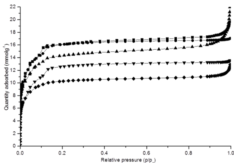
Figure 9. N 2 adsorption at 77 K (not offset) of MIL-100(Sc) (■), MIL-100(Sc 90 Fe 10 )XS (●), MIL-100(Sc 80 Fe 20 )XS (▲), MIL-100(Sc 60 Fe 40 )XS (▼) and MIL-100(Sc 50 Fe 50 )XS (◆)
