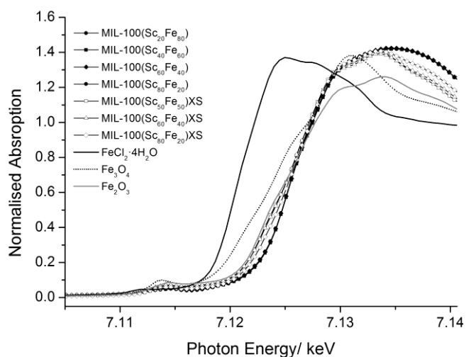
Figure 6 Fe K-edge XANES spectra of MIL-100(Sc,Fe) and MIL-100(Sc,Fe)XS materials, compared with XANES of standards \text{FeCl}_2 \cdot 4\text{H}_2\text{O} , \text{Fe}_3\text{O}_4 and \alpha\text{-Fe}_2\text{O}_3 .
