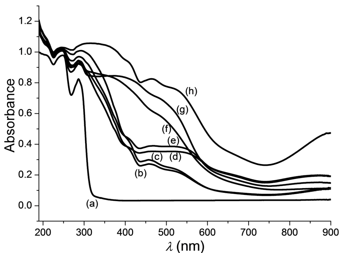
Figure 5 UV-visible spectroscopy of (a) MIL-100(Sc), (b) MIL-100(Sc 80 Fe 20 ), (c) MIL-100(Sc 60 Fe 40 ), (d) MIL-100(Sc 40 Fe 60 ), (e) MIL-100(Sc 20 Fe 80 ), (f) MIL-100(Sc 80 Fe 20 )XS, (g) MIL-100(Sc 60 Fe 40 )XS and (h) MIL-100(Fe).
