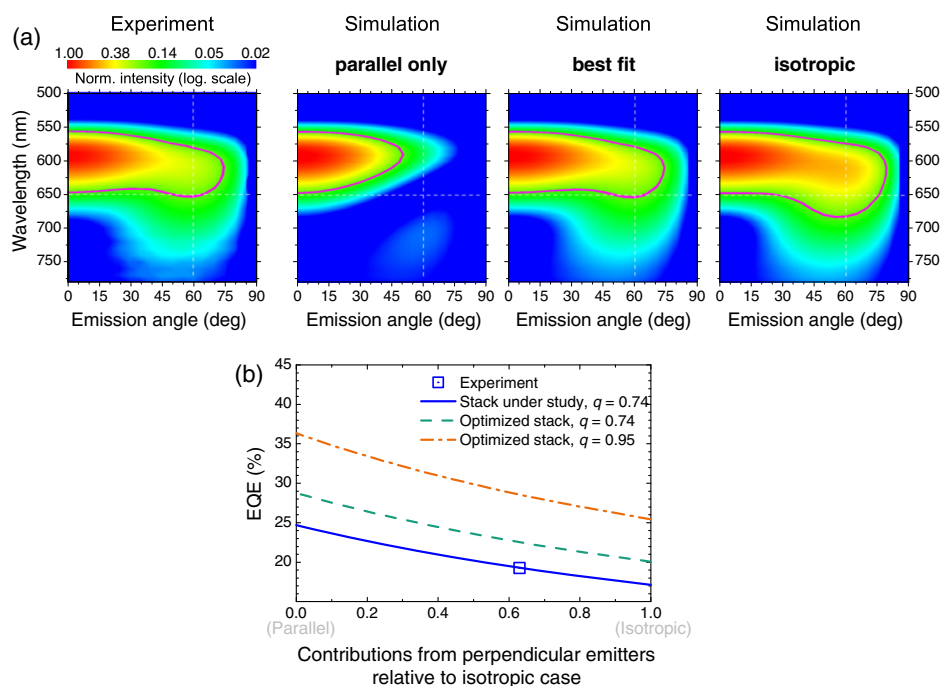
Fig. 9 (a) False color plots of the experimental and theoretical angle-resolved emission spectra of an Ir(MDQ) 2 (acac)-based OLED designed to show strong changes in emission characteristics with emitter orientation (electron transport layer thickness, 160 nm). The magenta line indicates a normalized intensity of 0.2 to enable better comparison between experiment and the three different simulations, each of which is performed for a different average emitter orientation. Neither the situation of parallel only dipoles nor the isotropic case describes the data whereas the best fit (76% orientation) is in good agreement with the experiment. (b) Optical simulation of expected external quantum efficiency as a function of the degree of emitter orientation for a red phosphorescent OLED. Different stack designs and different photoluminescence quantum yields q are considered. (Reproduced with permission, courtesy of Elsevier.) 79
