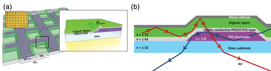
Fig. 4 Schematic illustration of an ITO grid-based approach to extract light from modes waveguided in the organic layers of OLEDs: (a) overview and (b) cross-sectional view indicating selected light paths. An ITO grid with tapered edges is coated with the low-index conductive polymer PEDOT:PSS to facilitate scattering of light guided in the organic film. Mesh size, line width, and taper angle can be tuned to optimize the efficiency of this approach. (Reproduced with permission, courtesy of John Wiley and Sons.) 54
