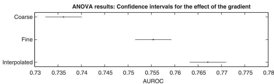
Figure 7 Influence of rate estimation. The figure shows confidence intervals for the group means associated with the main effect for the dependence of the performance (AUROC score) on the rate estimation method, based on the ANOVA analysis of equation (56). The horizontal axis shows the AUROC score. The vertical axis represents the three rate estimation methods, as described in Section 4.3: coarse gradient (top), fine gradient (middle), and gradient from smooth interpolant (bottom).
