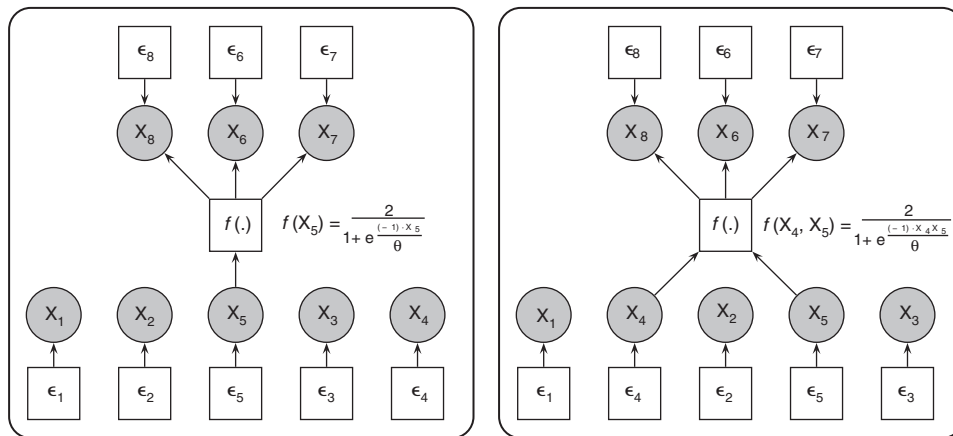
Figure 13 Regulatory network for synthetic data.
