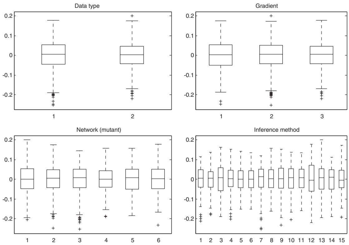
Figure 17 Residual diagnostic for different factors of the ANOVA model. The figure is arranged as a 2-by-2 matrix, whose four panels correspond to the four main effects of the ANOVA model of Section 4.8, equation (56). Each panel shows a boxplot representation of the distribution of the residuals for all possible values of the corresponding main effects.
