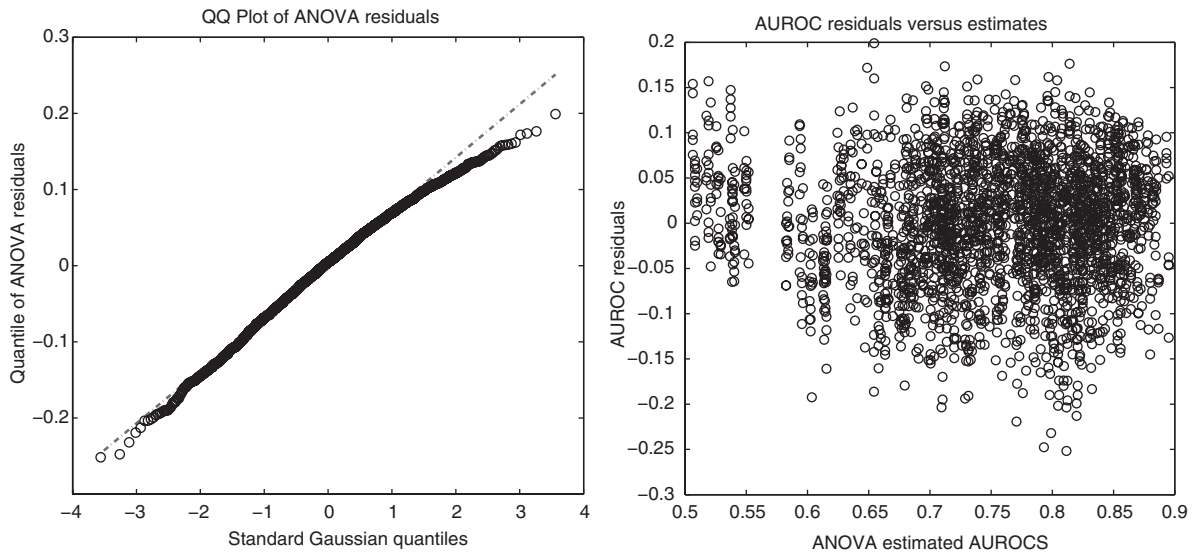
Figure 16 Residual diagnostic for the ANOVA model. Left panel: QQ-plot. The figure shows a Quantile-Quantile (QQ) plot of the residuals for the ANOVA model, described in Section 4.8, equation (56). The actual quantiles (vertical axis) are plotted against the quantiles of the Gaussian distribution (horizontal axis). The linear relation indicates good agreement with the Gaussian distribution; the deviations for very low and high values point to slightly longer tails. Right panel: Scatter plot diagnostic. The figure shows a scatter plot of the residuals (vertical axis) against the AUROC values fitted with the ANOVA model of Section 4.8, equation (56) (horizontal axis).
