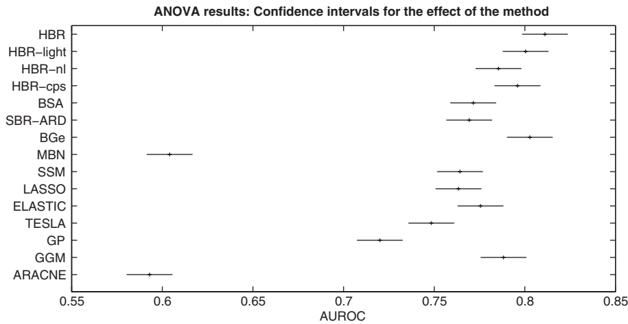
Figure 6 Comparison between different network reconstruction methods. The figure shows confidence intervals for the group means associated with the main effect for the network reconstruction method from the ANOVA analysis in equation (56). The horizontal axis shows the AUROC score. The vertical axis represents the different methods described in Section 2. The labels on the vertical axis refer to the methods described in Section 2, using the same abbreviations as in the subtitle headers.
