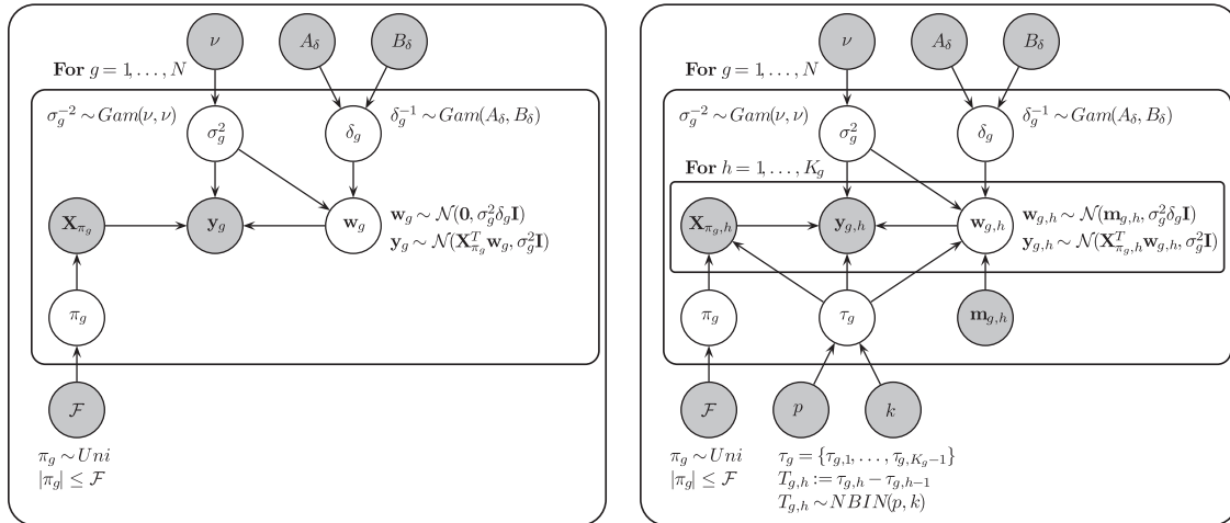
Figure 1 Representation of the hierarchical Bayesian regression models as graphical models. In both panels the gray circles refer to fixed hyperparameters, while the white circles refer to flexible (hyper-)parameters, which are inferred from the posterior distribution with MCMC. Left panel: The homogeneous Bayesian regression model. The outer plate includes the complete model, and the centre plate refers to the target variables, g=1, \dots, N ; see Section 2.5 for a detailed model description. Right panel: The uncoupled variant of the non-homogeneous Bayesian regression model. Variable-specific change-point sets, \boldsymbol{\tau}_g , divide the data into variable-specific segments. The additional inner plate refers to the variable-specific segments, h=1, \dots, K_g ; see Section 2.6 for more details. In the coupled variant of the non-homogeneous Bayesian regression model (not shown in this figure) the regression parameter vectors, \mathbf{w}_{g, h} ( h=1, \dots, K_g ), are sequentially coupled via equations (21–22).
