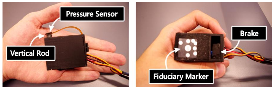
Figure 2. The HTP’s main components [14].
