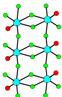
Fig.2 Ladder type [\text{VOF}_3]_n^+ chain
