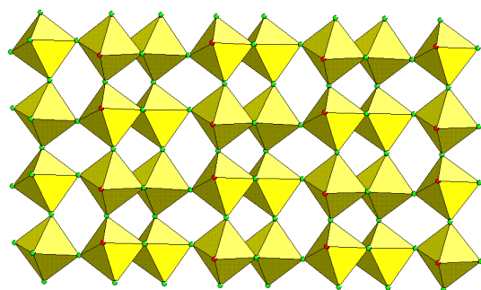
Fig.5 [V_2O_2F_5]_n^- layer found in VOF-3
