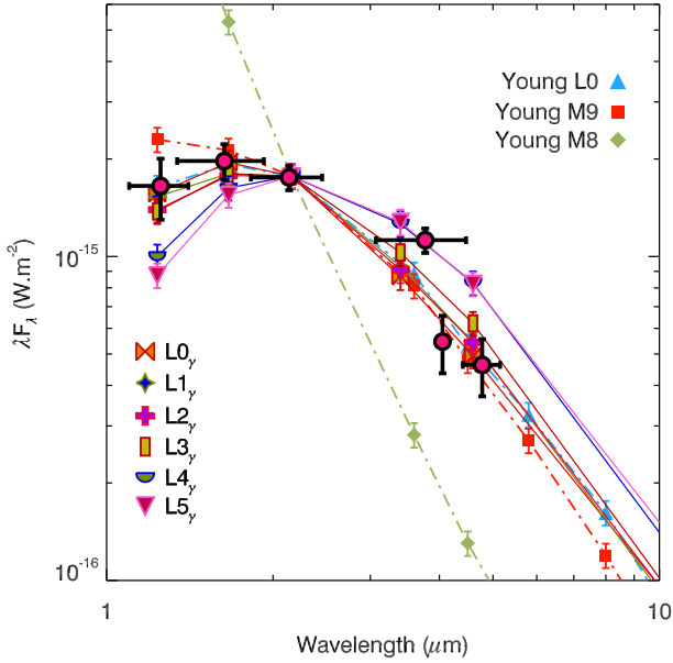
Fig. 7. \kappa And b spectral energy distribution (magenta dots) compared to the mean spectral energy distribution of young M8-L0 dwarfs (Luhman et al. 2010) and of L0-L5 \gamma dwarfs (Faherty et al. 2013).
