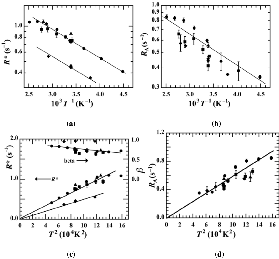
Figure 10. Various ways of presenting the ^{207}\text{Pb} NMR spin-lattice relaxation rate data in \text{PbI}_2 . (a) and (c) R^* , (b) and (d) R_A measured at 4.70 T (▲) and 7.05 T (●, ■) and R at 11.75 T (◆). In (a) and (b) the rates are plotted versus inverse temperature T^{-1} and in (c) and (d) they are plotted versus T^2 . Measurements were performed at the University of California at Los Angeles (●) and at the University of Delaware (■, ◆, ▲). The stretching parameter \beta is also shown in (c). The straight lines are guides for the eye.
