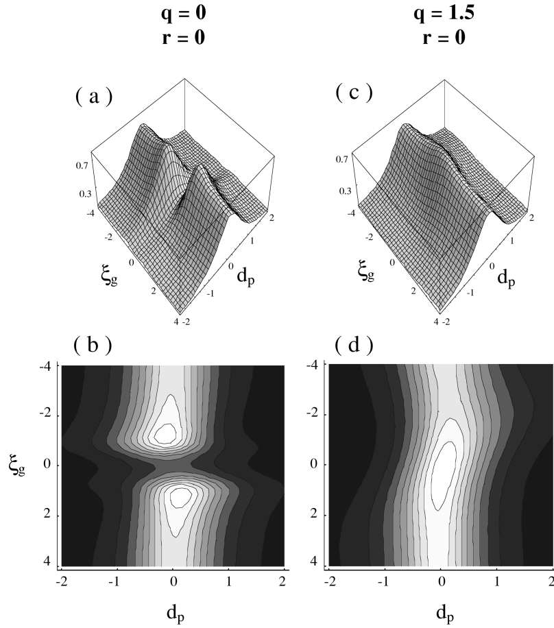
FIG. 9. TC-RFWM profiles for the parametric process depicted in Fig. 2 plotted as a function of the probe detuning d_p and the grating detuning \xi_g . (a) and (c) 3D plots of \mathcal{J}(\xi_g, d_p) for q=0 and 1.5. (b) and (d) contour plot of the surfaces in (a) and (c), respectively.
