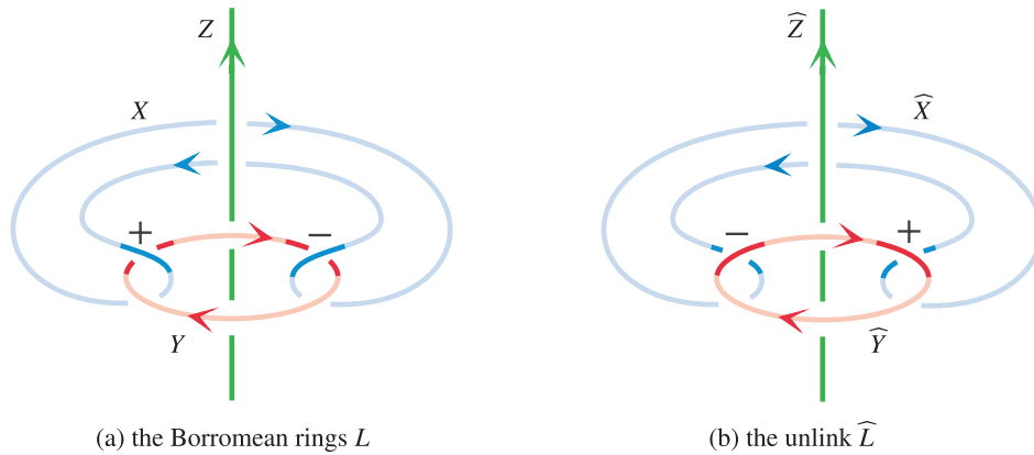
FIG. 19. A double crossing change.
