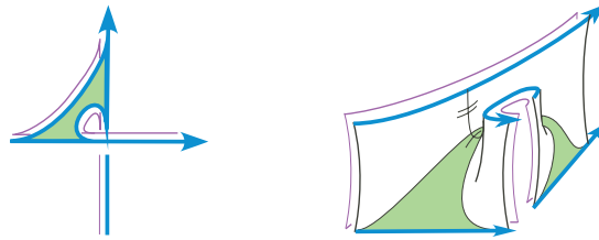
FIG. 9. The saddle bordism.
