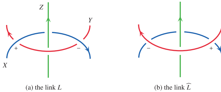
FIG. 21. A simple double crossing change.
