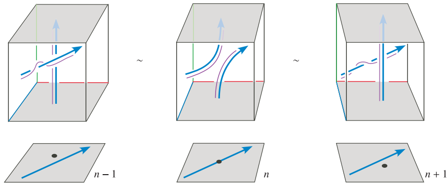
FIG. 27. Using saddles to gather the vertical circles.
