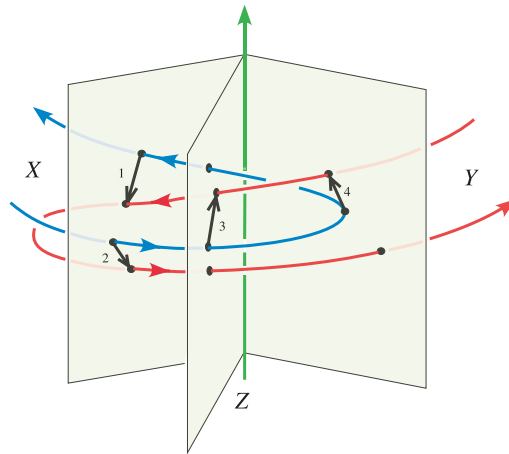
FIG. 15. Page vectors.
