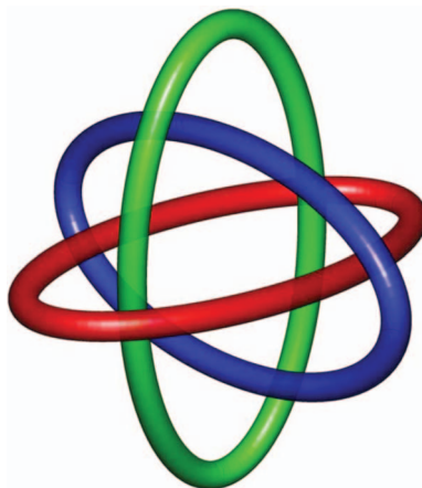
FIG. 31. Borromean rings.
