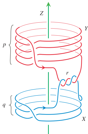
FIG. 22. A generic link L representing L_{pqr} .
