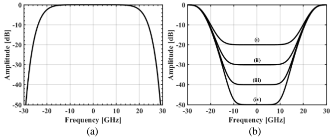
Fig. 5. Transfer function of the (a) optical Super-Gaussian 4 th order passband filter H_p(f) and (b) optical stopband filters H_b(f) with different blocking amplitudes (i) -20 dB (ii) -30 dB (iii) -40 dB and (iv) -50 dB.
