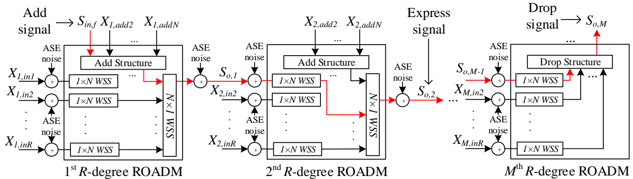
Fig. 9. Schematic model of a cascade of M multi-degree CDC ROADM based on the R&S architecture with in-band crosstalk signals and ASE noise addition.
