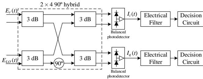
Fig. 1. Coherent receiver block diagram for a single polarisation QPSK signal.
