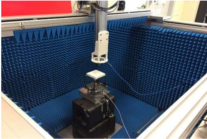
Figure 2. Setup used for the measurement of the antenna in the XYZ planar acquisition range of Universidad de Oviedo.
