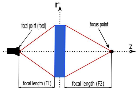
Figure 1. Description of the system employed to design the lens.
