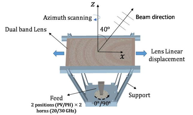
Fig. 1 - Working Principle
