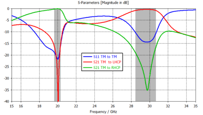
Fig. 4 The reflection and transmission coefficients of the polarizer UC simulated with periodic boundary condition.
