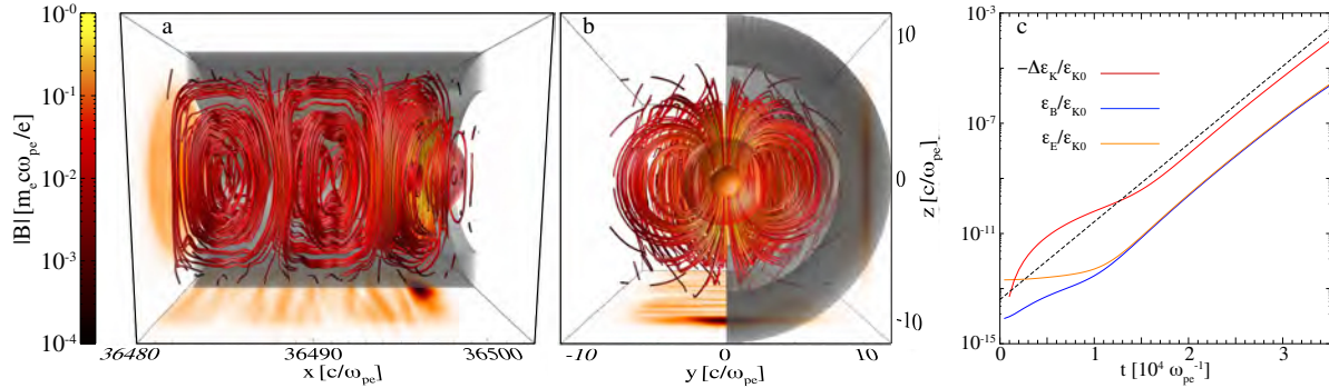
Figure 4. 3D PIC simulation of the development of the MI for \gamma_0 = 10^4 , \sigma_\perp = 2\sigma_\parallel = 2c/\omega_{pe} and R = 4\sigma_\perp . The e^-e^+ beam density is represented by the red isosurfaces, and the hollow plasma channel is represented by the grey isosurfaces (half of the cylindrical structure has been omitted to more clearly illustrate the dynamics of the e^-e^+ beam inside). The e^-e^+ beam propagates in the positive x direction. The red lines represent the structure of the MI-generated magnetic field. Figures (a) and (b) are side and front views of the simulation domain, respectively, taken at \omega_{pe}t = 36500 . Figure (c) shows the temporal evolution of the electric (orange curve) and magnetic (blue curve) field energy and the negative variation of the total kinetic energy of the beam (red curve), all normalized to the initial kinetic energy of the beam. The slope of the dashed line represents the growth rate of the MI.
