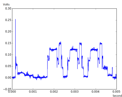
Figure 5.2: Wave form of Advertise Process
