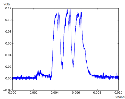
Figure 5.4: Wave form of Advertise Process
