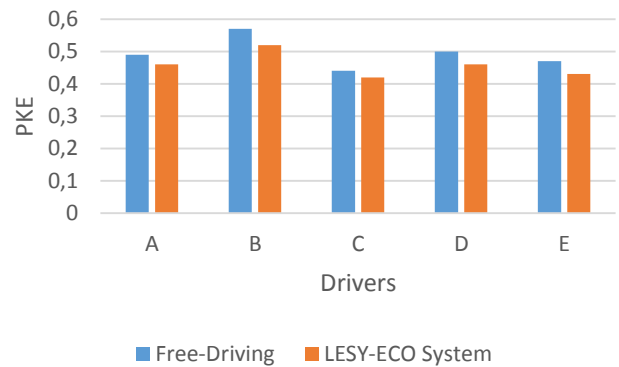
Fig. 7. Positive Kinetic Energy obtained by drivers from control group with and without LESY-ECO System.
