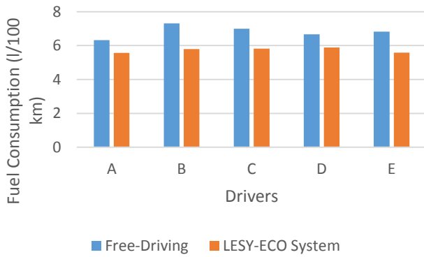
Fig. 4. Fuel Consumption obtained by drivers from experimental group with and without LESY-ECO System.
