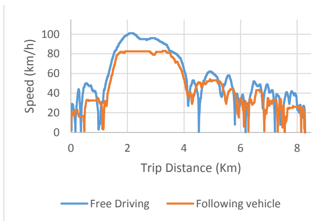
Fig. 5. Speed profiles with (following vehicle) and without (free driving) the LESY-ECO system.
