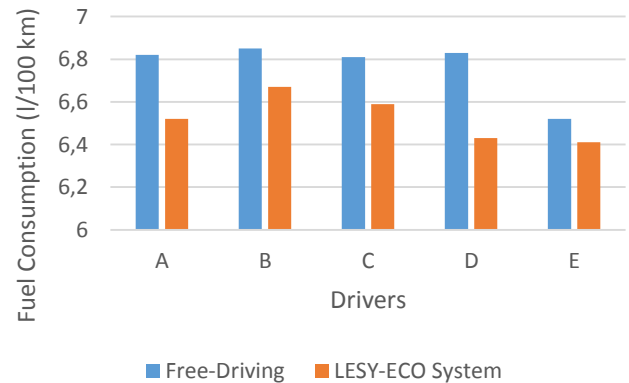
Fig. 8. Fuel Consumption obtained by drivers from control group with and without LESY-ECO System.
