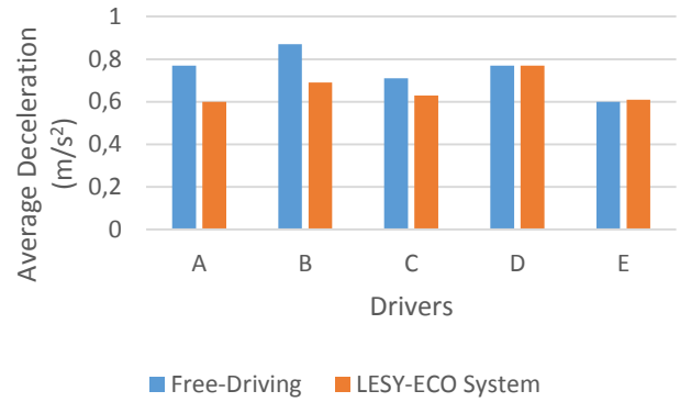
Fig. 6. Average Deceleration obtained by drivers from control group with and without LESY-ECO System .
