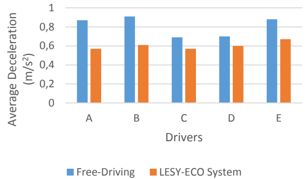
Fig. 2. Average Deceleration obtained by drivers from experimental group with and without LESY-ECO System .
