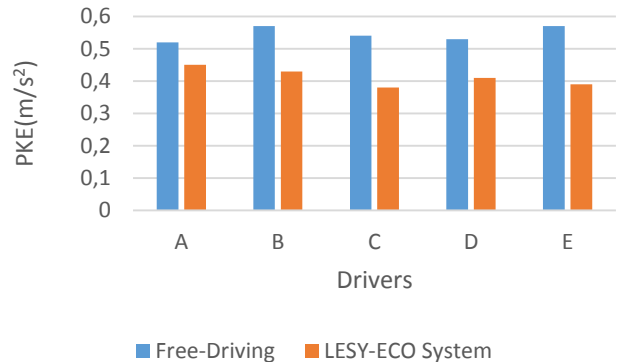
Fig. 3. Positive Kinetic Energy obtained by drivers from experimental group with and without LESY-ECO System.
