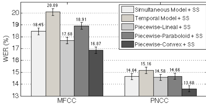
Fig. 6. Recognition results in terms of WER[%] and 95% confidence intervals using the AURORA 2 dataset (average over all the sets) for the different structuring elements in combination with spectral subtraction (SS).
