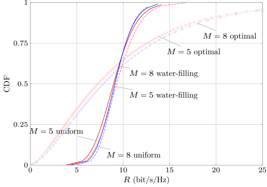
Figure 5.3: CDF of the achievable rate per user with r = 3 , t = 3 , and \text{SNR}=15 dB. Comparison between different power allocation schemes.
