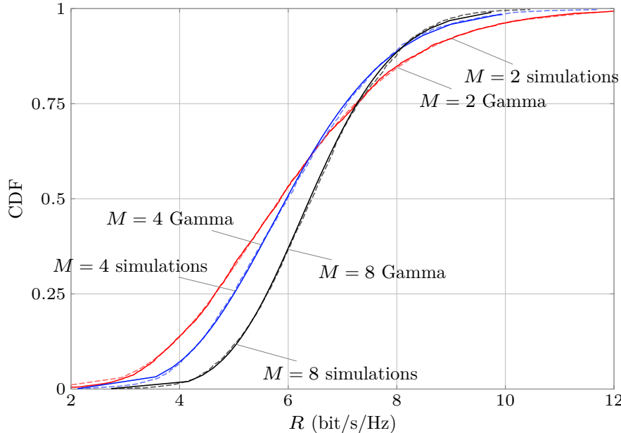
Figure 5.1: CDF of the achievable rate per user with r = 2 , t = 2 , and SNR=15 dB. Comparison with the Gamma distribution with the same mean and variance.
