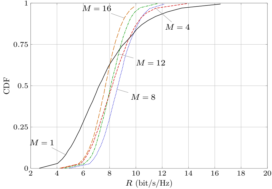
Figure 5.2: CDF of the achievable rate per user with r = 2 , t = 2 , and \text{SNR}=15 dB for different values of the cluster size.
