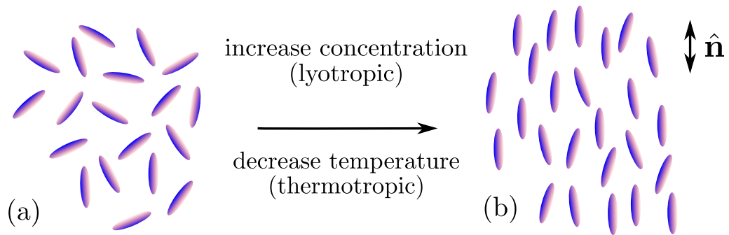
Figure 3.4: Schematic of (a) isotropic and (b) nematic phases of a LC. While neither state possesses translational ordering, the nematic exhibits orientational ordering.
