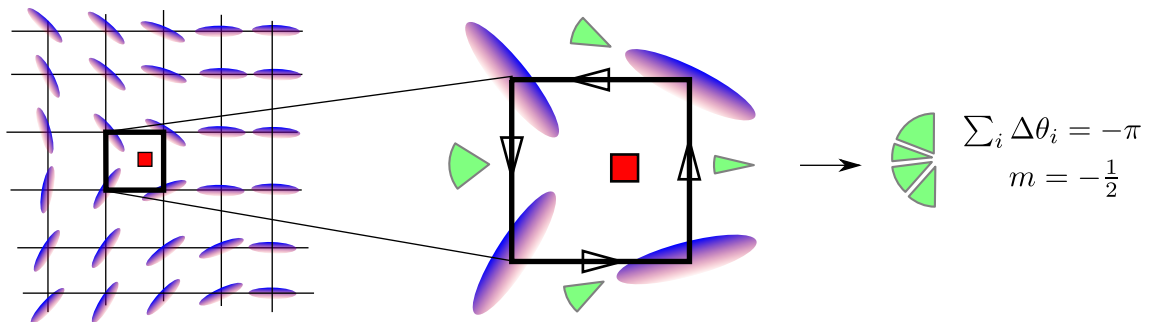
Figure 5.16: Schematic demonstrating how the topological charge and position of a defect is found numerically. The director angle is extracted on the regular grid, and the change in angle integrated round the four nearest grid points. After accounting for the head-tail symmetry of the director \hat{\mathbf{n}} , any square where the integrated angle is non-zero contains a defect. Here we demonstrate the process for a -1/2 defect (green wedges indicate the angular change from site to site). Red square marks the (approximate) location of the defect core.
