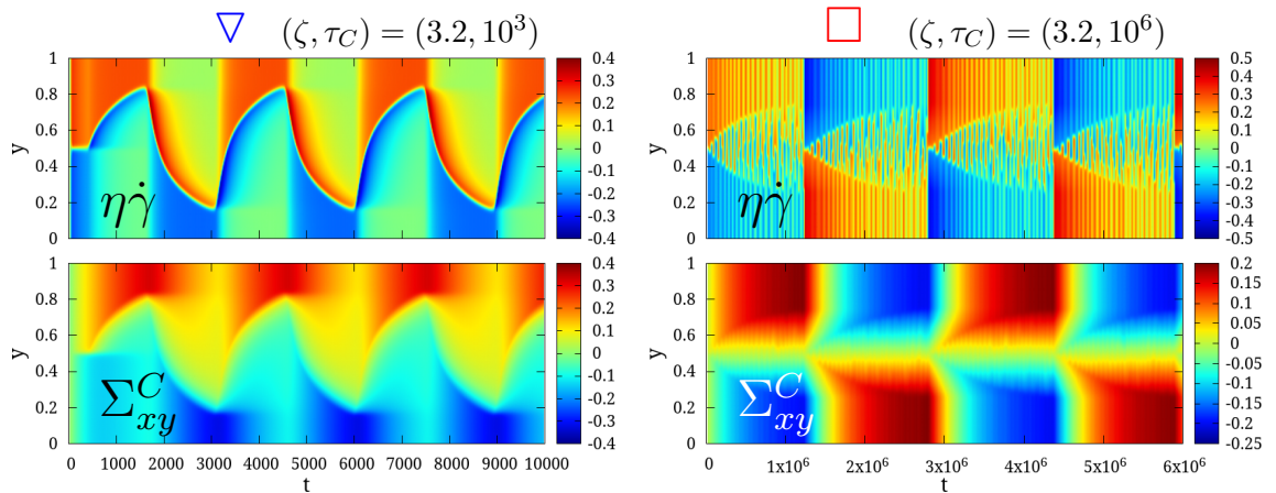
Figure 3.16: Space time plots for the marked coordinates in the phase diagram in Fig. 3.15. The x-axis time is t , y-axis position y , and colour scale: \eta\dot{\gamma} (top row), \Sigma_{xy}^C (bottom row). Left col: State with oscillating interface ( \zeta = 3.2 , \tau_C = 10^3 ), Right col: State with oscillating interface, flow direction also switches ( \zeta = 3.2 , \tau_C = 10^6 ).
