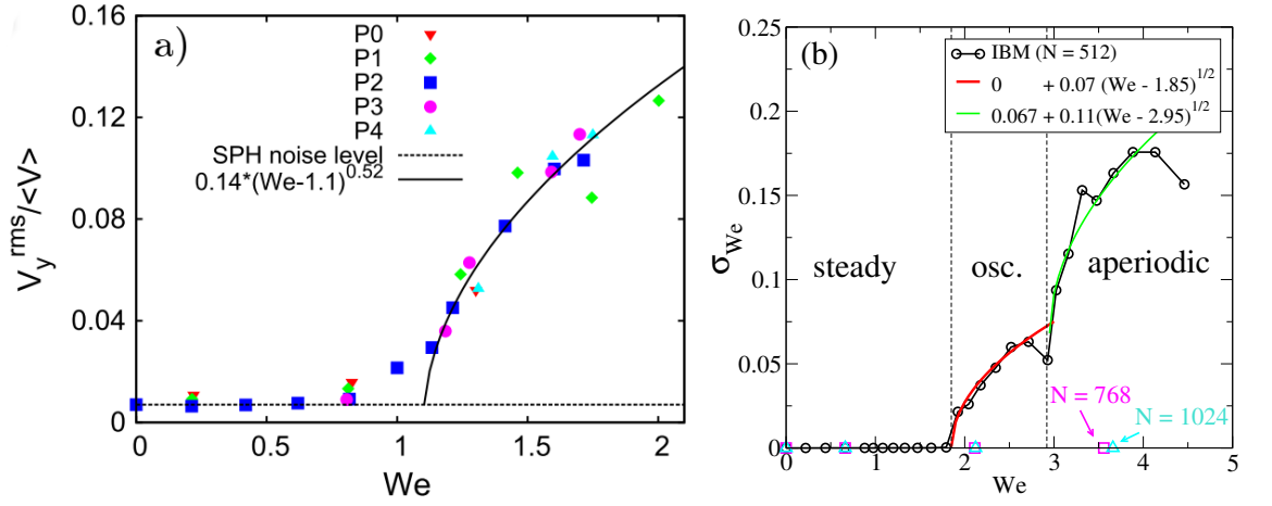
Figure 6.21: (a) Data from Ref. [25] showing an increase in fluctuations above We^{osc} \sim 1.1 . (b) Plot of the standard deviation \sigma_{We} against mean \mu_{We} , extracted from the time series We(t) . Data from higher resolution runs (magenta squares N_y = 768 , cyan triangles N_y = 1024 ) are also marked.
