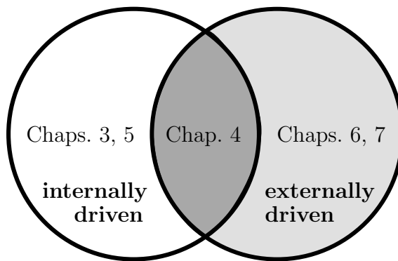
Figure 1.1: Overview of the chapters in this thesis according to the nature of the forcing, which may be internal (e.g., for biological active matter), external (e.g., pressure driven flow of multiphase fluids), or both (e.g., sheared active matter).
