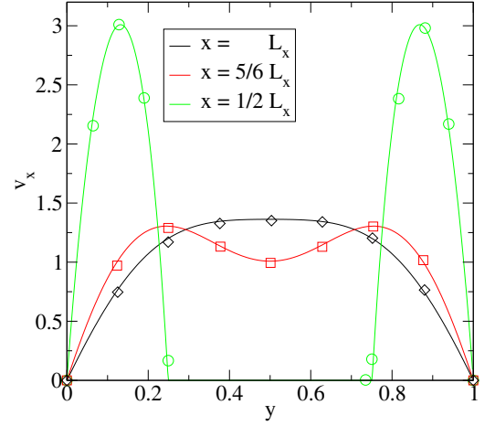
Figure 6.4: Vertical slices of v_x in the channel geometry at various x for L_x = 1.5 , showing good agreement between our IBM results (solid lines) with the SPH results of Ellero [227] (symbols). The SPH data was extracted using an online tool [228].
