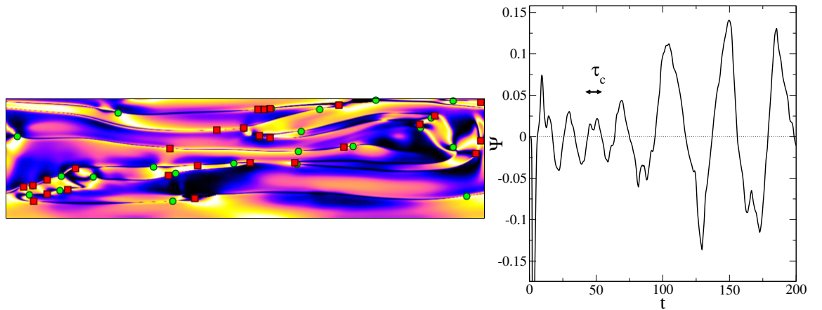
Figure 5.14: Example of an exotic oscillatory state which coherently shuffles left and right on a timescale of order \tau_C . Left: Snapshot of the state where (n_x n_y)^2 . Right: Throughput time-series showing the oscillatory nature of the state. Parameters: \zeta = 6 , \Delta = 10^{-4} , \tau_C = 10 , \chi = 0.002 .
