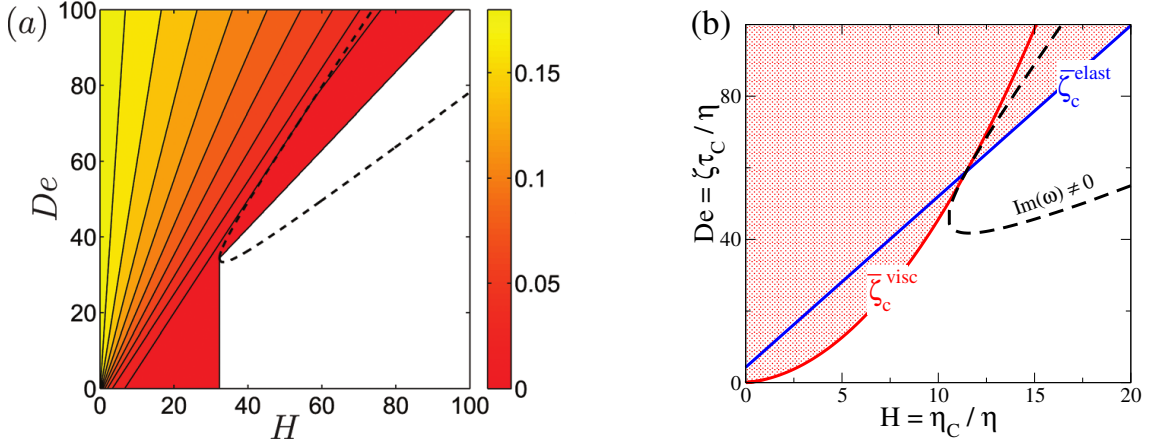
Figure 3.14: Stability diagrams in the limit k \rightarrow 0 for the dimensionless quantities De = \tau_C\zeta/\eta and H = \eta_C/\eta . Left: Data from Ref. [101], where colourscale marks growth-rate \omega (white regions are stable with \omega < 0 ) and dashed black line bounds the oscillatory region. Right: Our results cast in the same dimensionless groups, showing \bar{\zeta}_c^{visc} (Eq. 3.43) and \bar{\zeta}_c^{elast} (Eq. 3.44). Parameters: \gamma = 2.5 , G_C = 1 .
