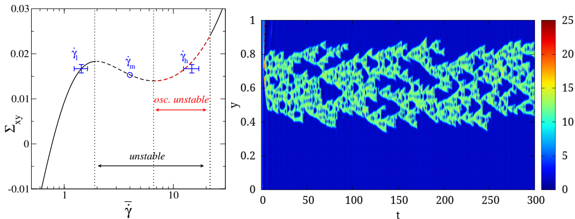
Figure 4.15: Example of rheochaotic behaviour under applied shear \bar{\gamma} = 4 . Left: Constitutive curve where both the negatively sloping and high shear-rate regions are unstable. As the system is unstable for our applied shear-rate \bar{\gamma} = 4 , shear-bands form at \dot{\gamma}_l, \dot{\gamma}_h . Our linear stability analysis predicts oscillatory growth of perturbations in the higher band, which results in chaotic fluctuations. Variations in shear-rate and shear-stress are marked by blue error bars. Right: Space-time plot showing coexistence of chaotic (high \dot{\gamma} , lighter colours) and homogeneous (low \dot{\gamma} , dark blue) regions. Parameters: \bar{\gamma} = 4 , \eta = 0.001 , \zeta = 0.75 , a = 0.3 , \tau_C = G_C = 1 , \Delta = 8 \times 10^{-5} .
