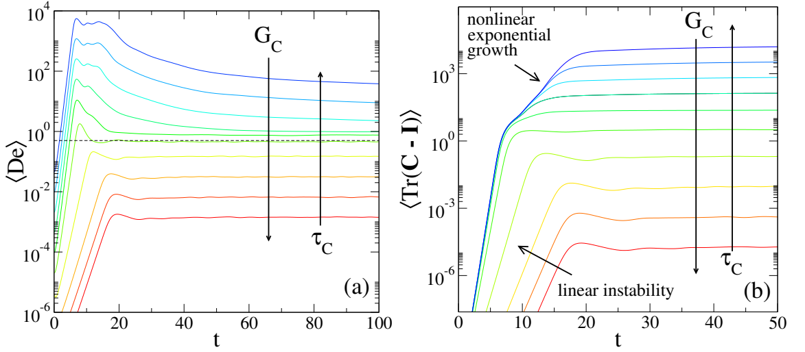
Figure 5.9: Results from 2D runs examining the short time dynamics of a point in the chaotic region of the phase diagram. We vary \tau_C from 10^{-2} (red) \rightarrow 10^4 (blue) with logarithmic spacing, keeping \eta_C constant by decreasing G_C . (a) Time series of the mean Deborah number \text{De} = \tau_C \sqrt{1/2 (\mathbf{D} : \mathbf{D})} for increasing \tau_C . Also marked is the threshold \text{De}_{\text{crit}} = 1/2 above which we might expect non-linear exponential growth (dashed line). (b) Spatial average of \text{Tr}[\mathbf{C} - \mathbf{I}] quantifying the mean polymer deformation. When \langle \text{De} \rangle > \text{De}_c (see left), we observe non-linear, exponential loading of the polymer in very short times. Parameters: \zeta = 2.2 , \Delta = 4 \times 10^{-5} , \eta_C = 1 .
