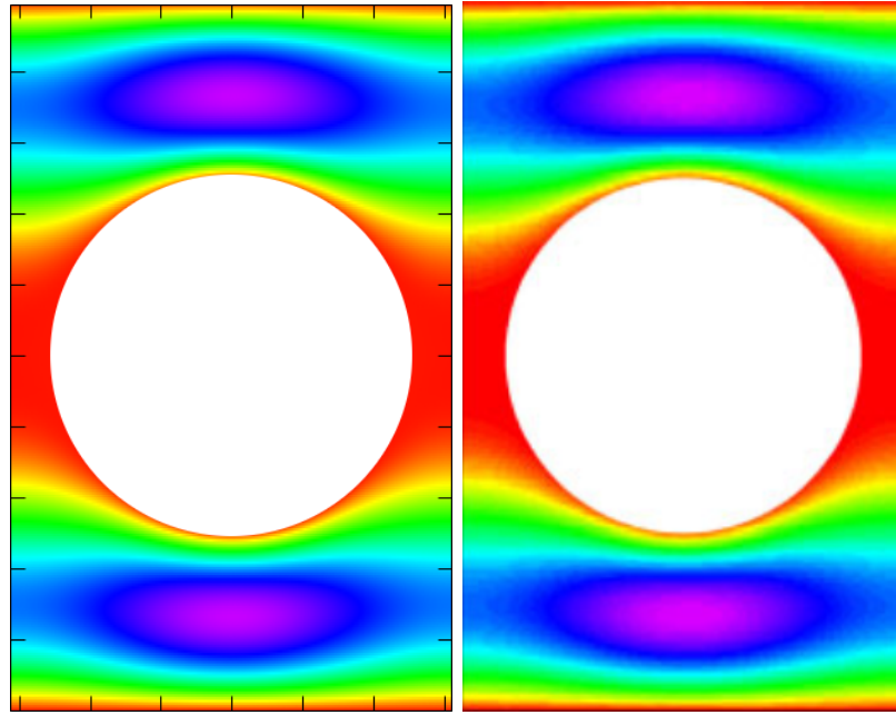
Figure 6.5: Colourmap of v_x in the channel geometry showing good agreement between our simulations (left) and those of Ellero et al. [227] (right), for L_x = 0.625 .
