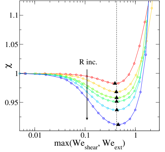
Figure 6.15: Replotting the data in Fig. 6.13 using \max(We_{\text{shear}}, We_{\text{ext}}) for any run, we find that the upturn is well described by a single value We^{\text{up}} \approx 0.42 (dashed line). Upturns in \chi are marked with solid black triangles.
