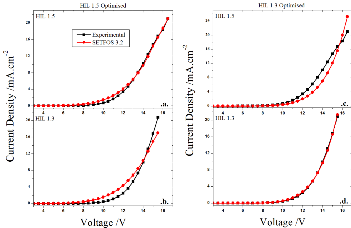
Figure 4.5: Plots of the simulated J-V curves for (a) PEDOT HIL 1.5 from a simulation optimised for HIL 1.5, (b) PEDOT HIL 1.3 from a simulation optimised for HIL 1.5, (c) PEDOT HIL 1.5 from a simulation optimised for HIL 1.3 and (d) PEDOT HIL 1.3 from a simulation optimised for HIL 1.3, produced using SETFOS 3.2, along with the experimentally determined J-V curves already seen in Figure 4.1.
