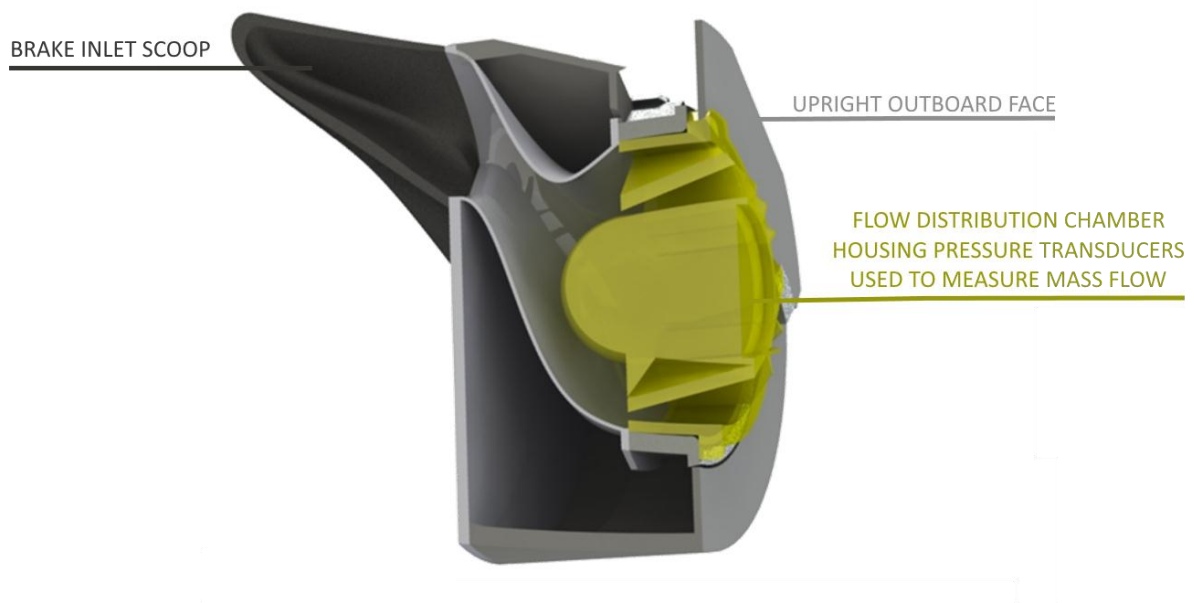
Figure 26: Upright CAD geometry cross sectional view of scoop inlet.
