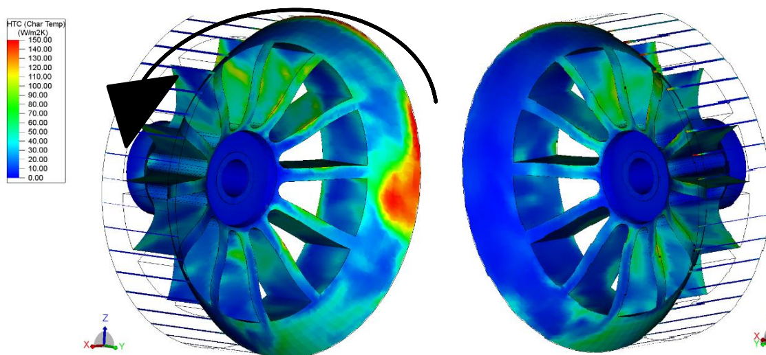
Figure 87: HTC surface Image for Spoke region at 25m/s MRF (disc, tyre and upright hidden).
