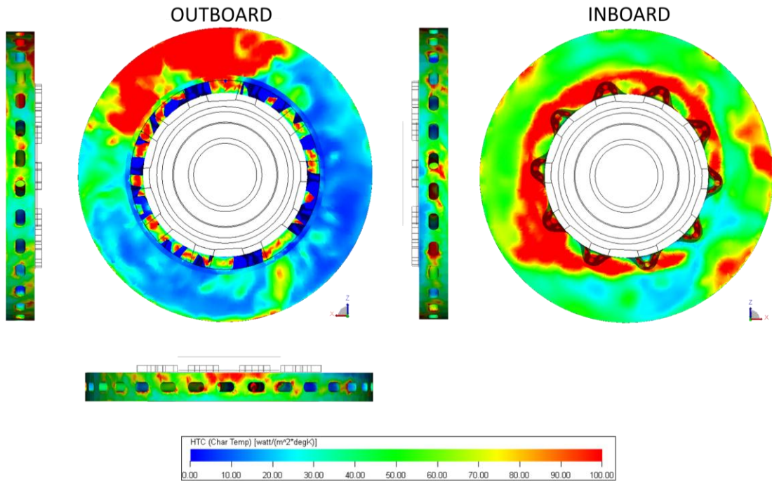
Figure 96: HTC surface contours for disc at all orientations - 100% scale at 25m/s using sliding mesh.
