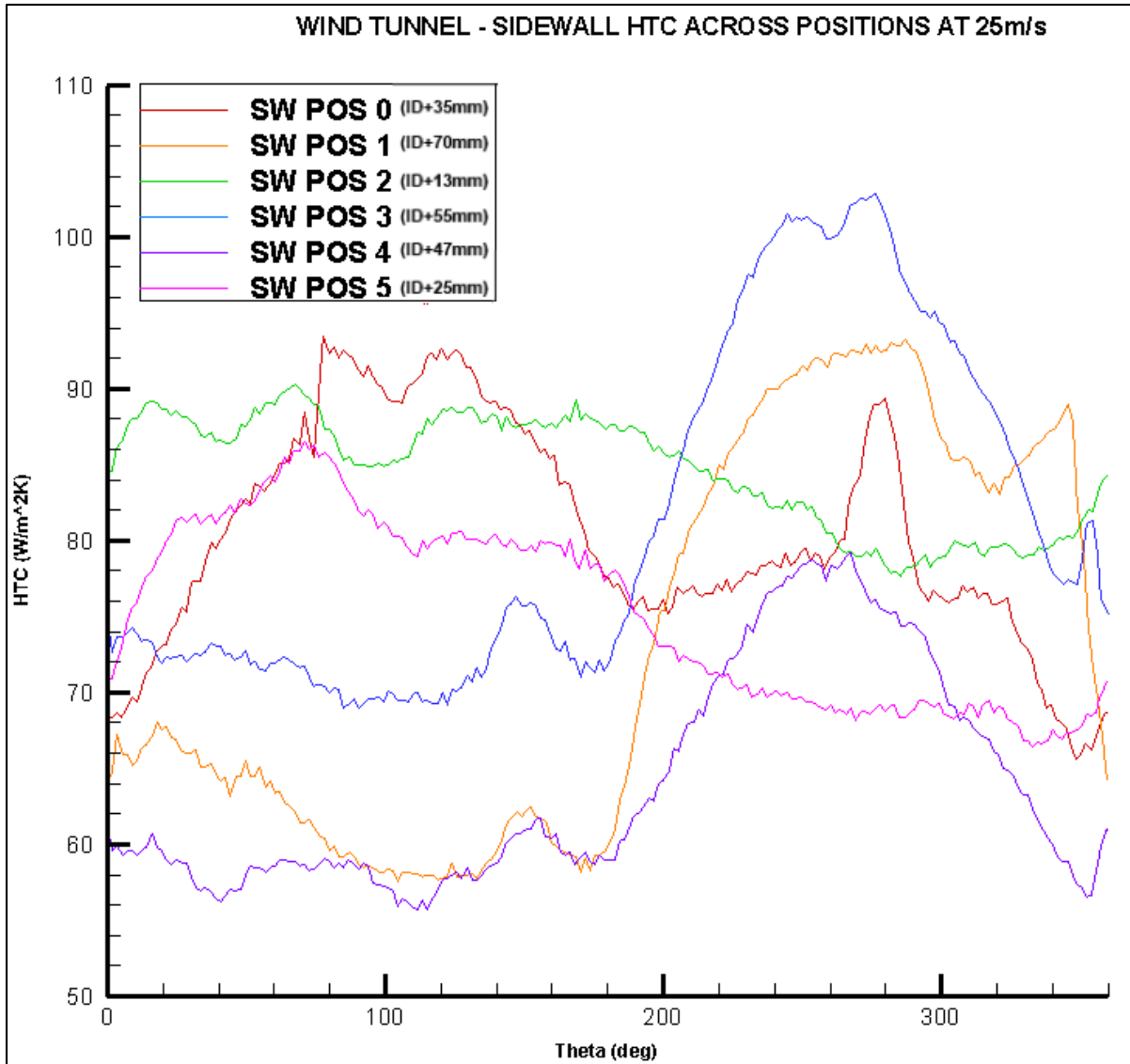
Figure 60: Sidewall HTC for 25m/s wind tunnel tests.
