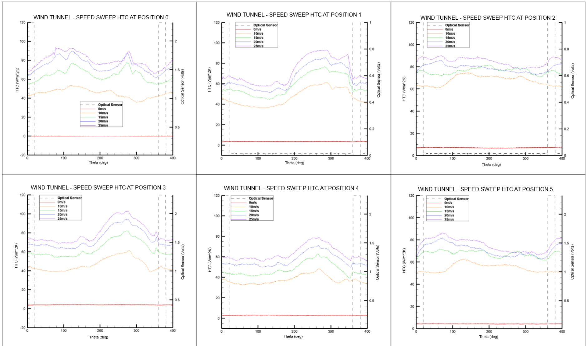
Figure 61: Sidewall positional graphs of heat transfer coefficient through 0-25m/s speed range.
