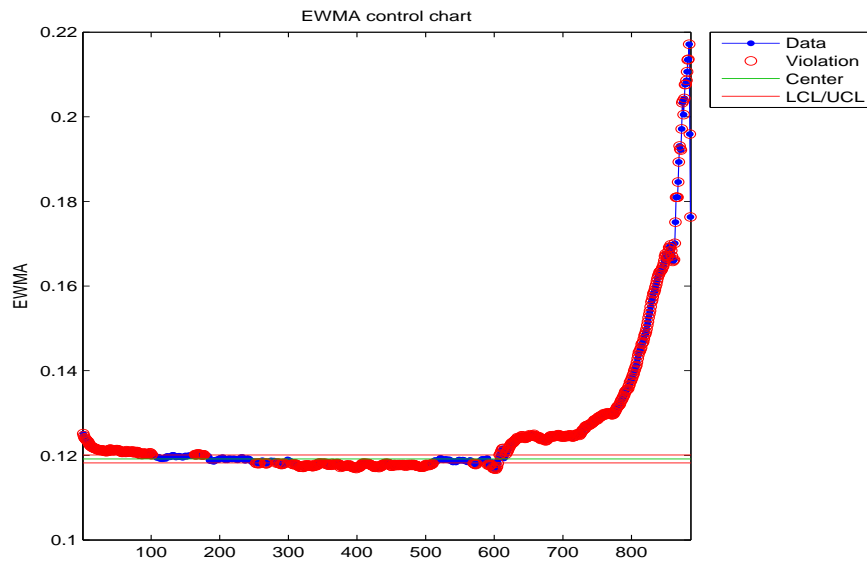
Figure B.68: EWMA chart for the 90 th percentile of the healthy bearing.
