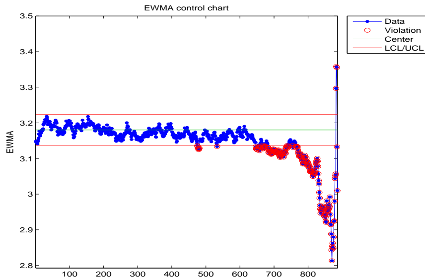
Figure B.44: EWMA chart for the kurtosis of the healthy bearing.
