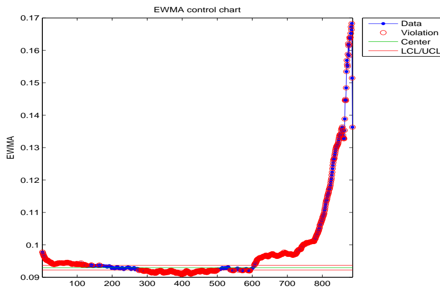
Figure B.38: EWMA chart for the median absolute deviation of the healthy bearing.
