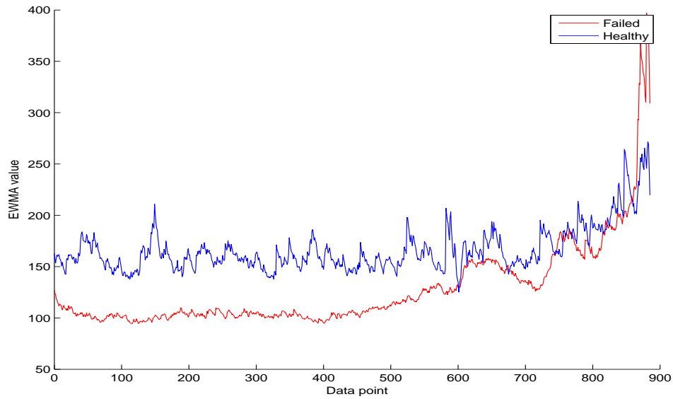
Figure B.72: Shannon entropy over time of the failed and healthy bearing.
