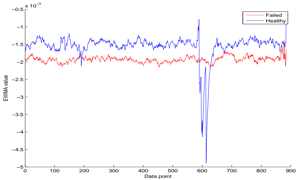
Figure B.3: Mean over time of the failed and healthy bearing.
