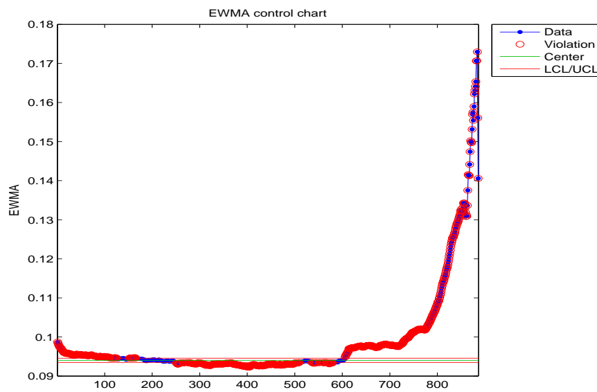
Figure B.14: EWMA chart for the RMS of the healthy bearing.
