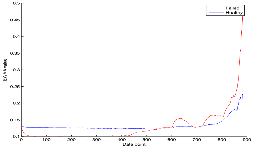
Figure B.27: IQR over time of the failed and healthy bearing.
