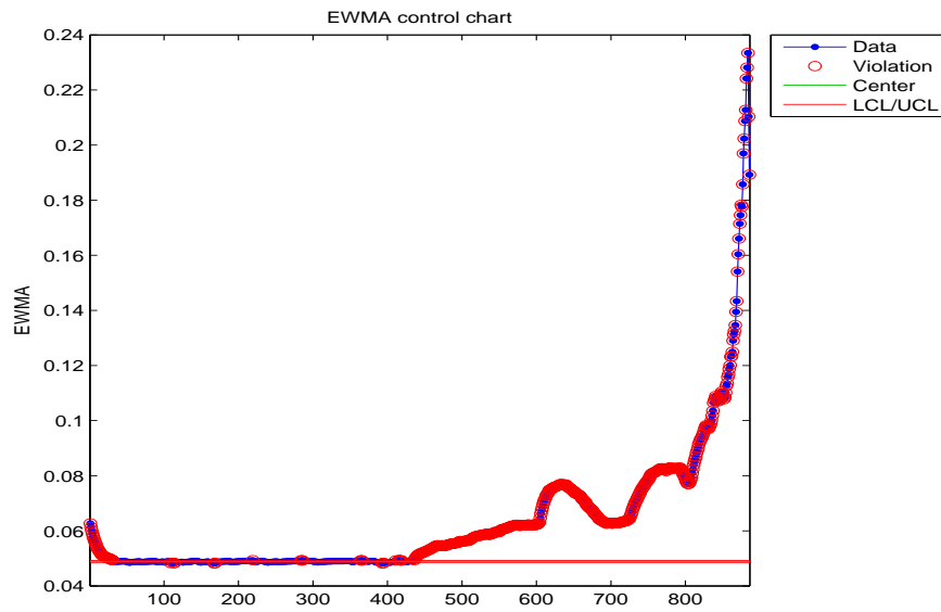
Figure B.64: EWMA chart for the 75 th percentile of the failed bearing.
