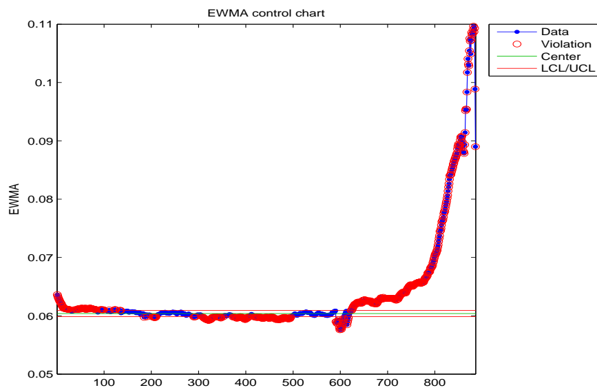
Figure B.65: EWMA chart for the 75 th percentile of the healthy bearing.
