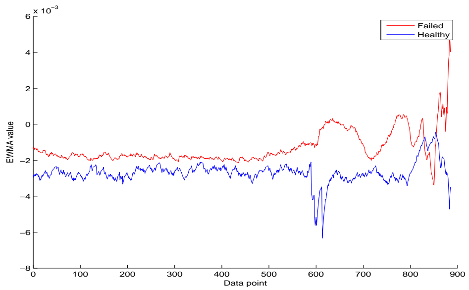
Figure B.12: Tri-mean over time of the failed and healthy bearing.
