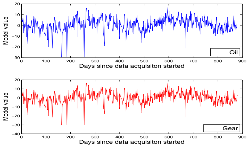
Figure 4.10: Wind turbine 3 health metric over 2 months.
