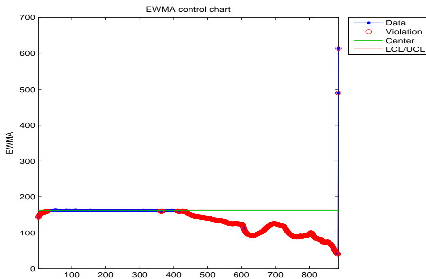
Figure B.73: EWMA chart for the Chao-Shen entropy of the failed bearing.
