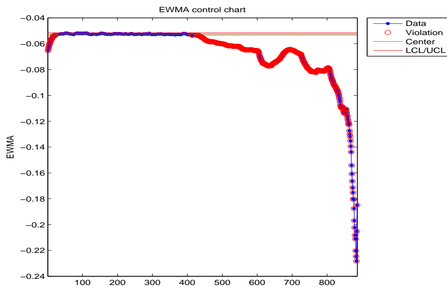
Figure B.61: EWMA chart for the 25 th percentile of the failed bearing.
