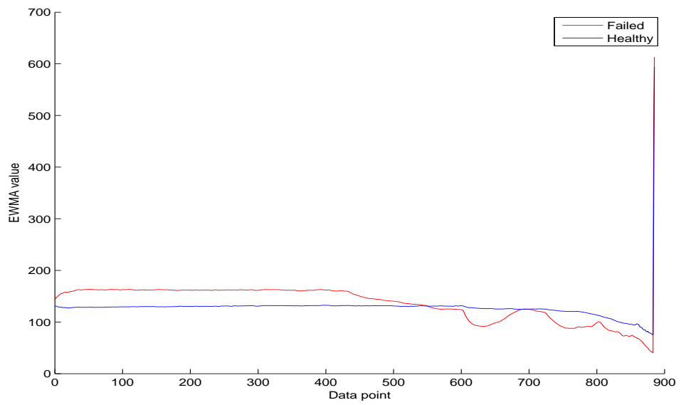
Figure B.75: Chao-Shen entropy over time of the failed and healthy bearing.
