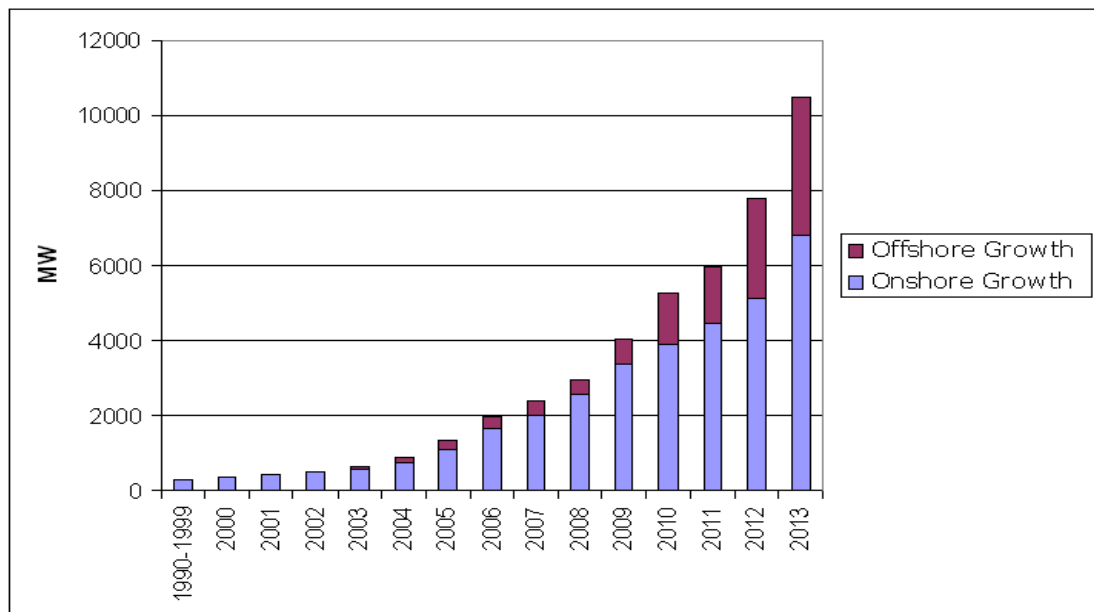
Figure 1.8: UK installed capacity (RenewableUK, 2014).
