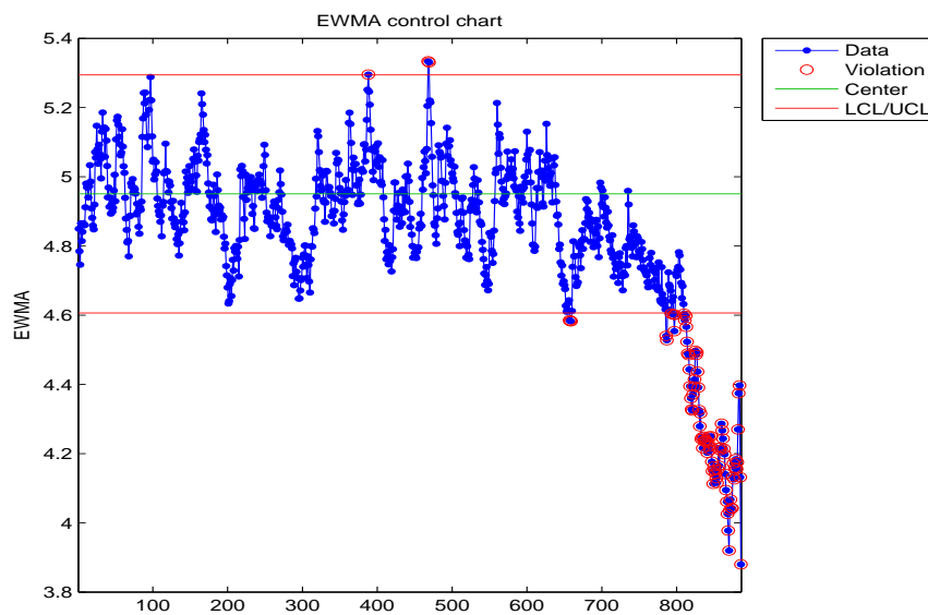
Figure B.53: EWMA chart for the crest factor of the healthy bearing.
