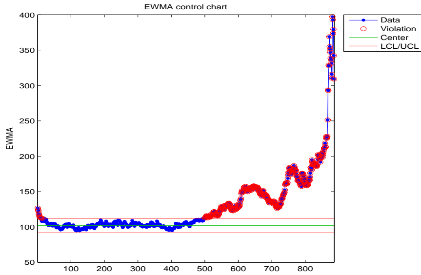
Figure B.70: EWMA chart for the Shannon entropy of the failed bearing.
