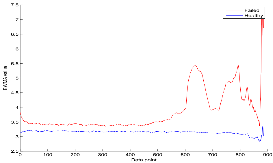
Figure B.45: Kurtosis over time of the failed and healthy bearing.
