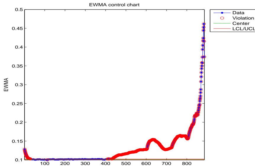
Figure B.25: EWMA chart for the IQR of the failed bearing.
