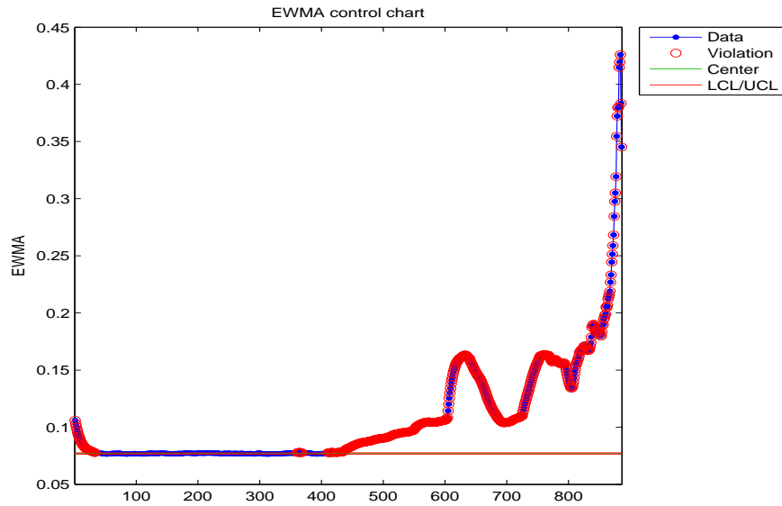
Figure B.19: EWMA chart for the standard deviation of the failed bearing.
