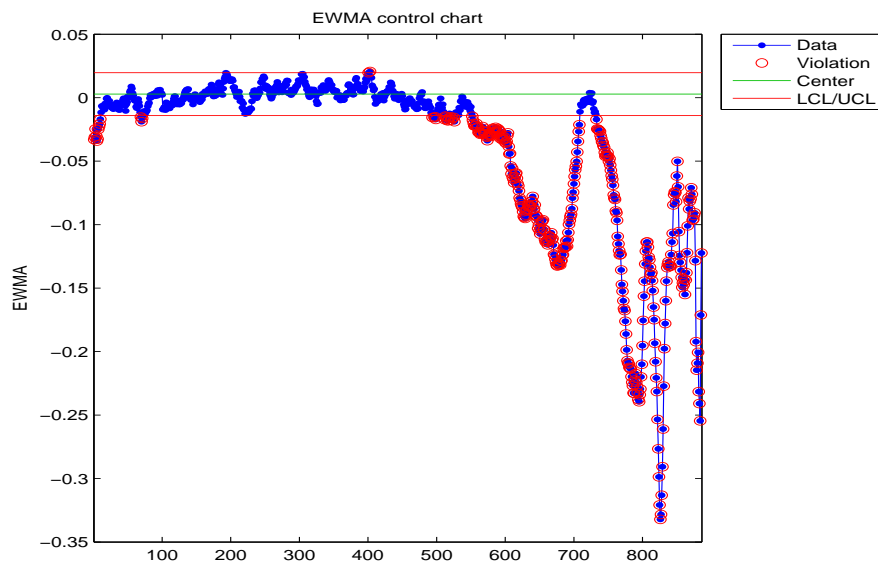
Figure B.40: EWMA chart for the skewness of the failed bearing.
