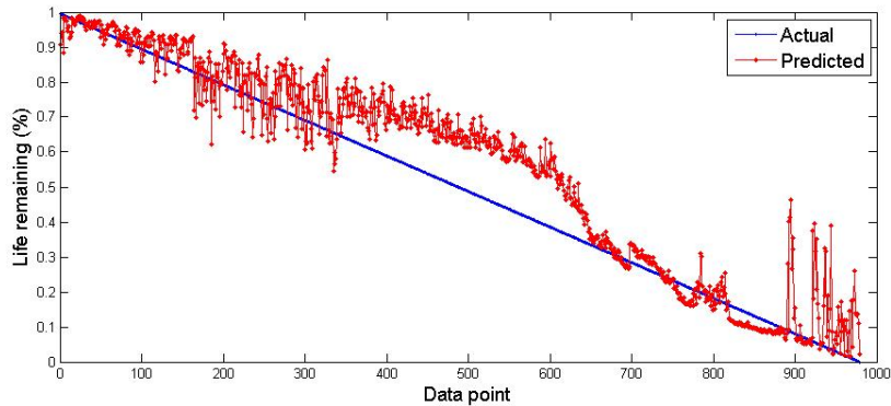
Figure 6.20: Refined RUL estimation of bearing 1 (training dataset).
