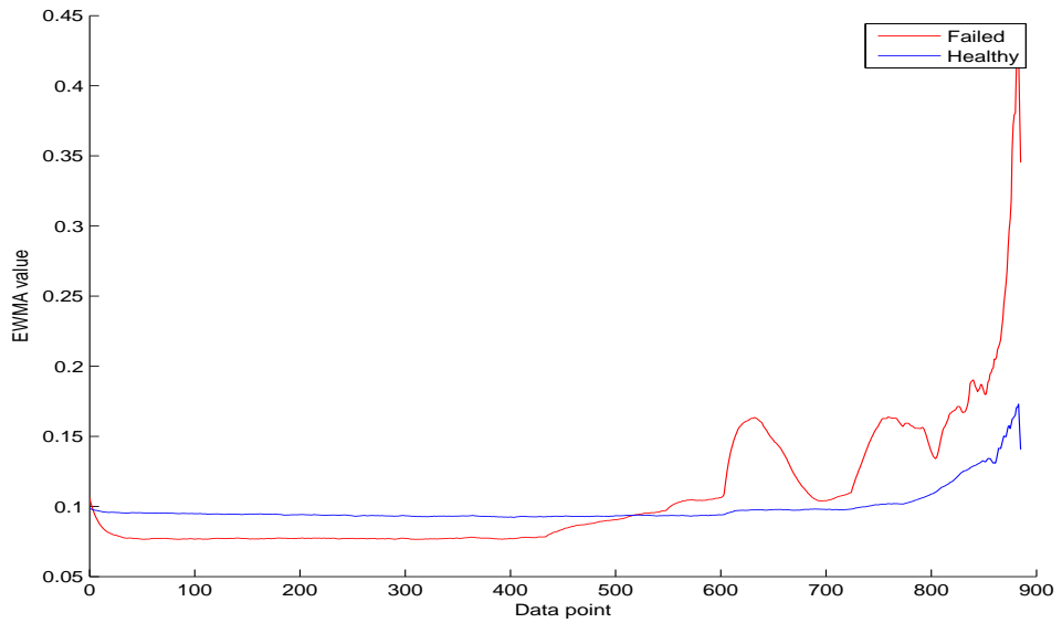
Figure B.15: RMS over time of the failed and healthy bearing.
