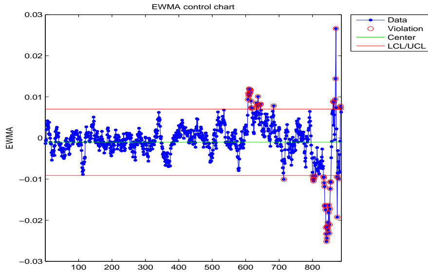
Figure B.7: EWMA chart for the mode of the failed bearing.
