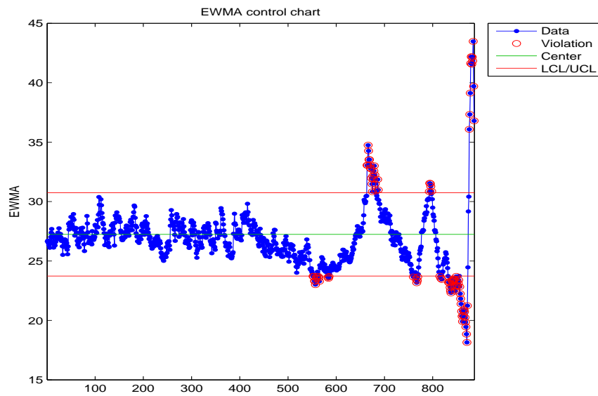
Figure B.55: EWMA chart for the peak to average power ratio of the failed bearing.
