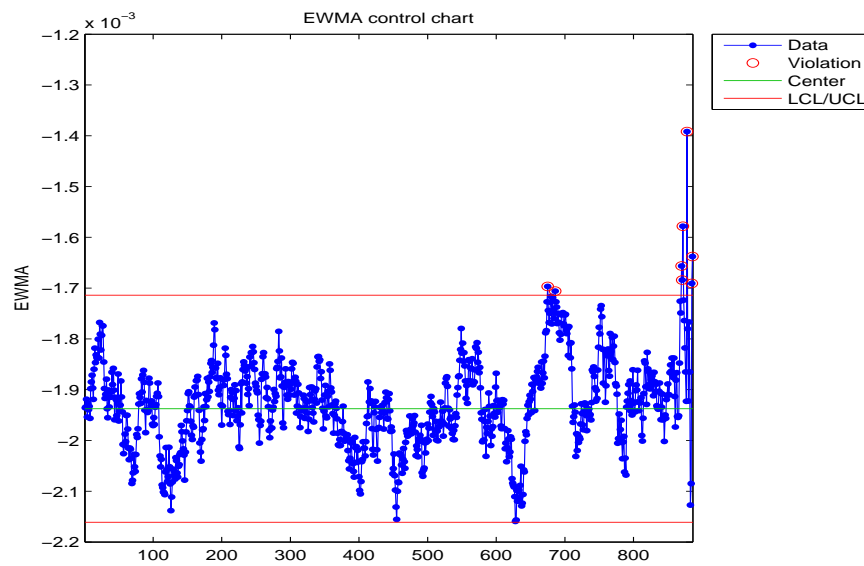
Figure B.1: EWMA chart for the mean of the failed bearing.
