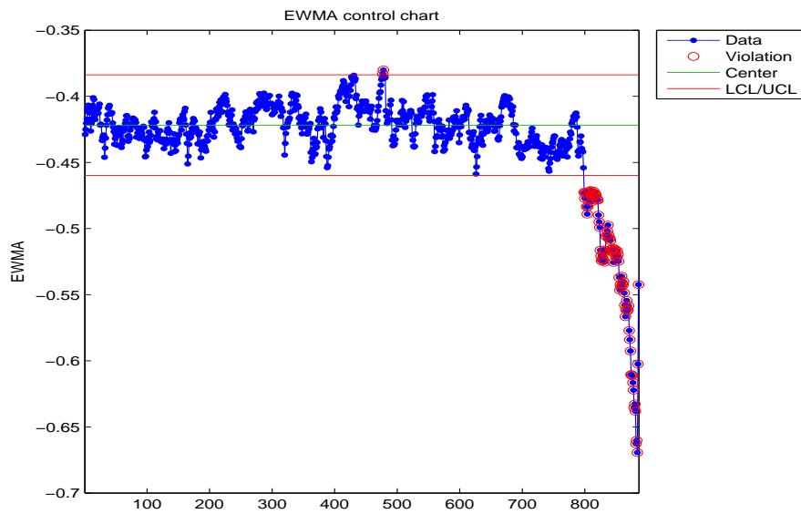
Figure B.32: EWMA chart for the minimum of the healthy bearing.
