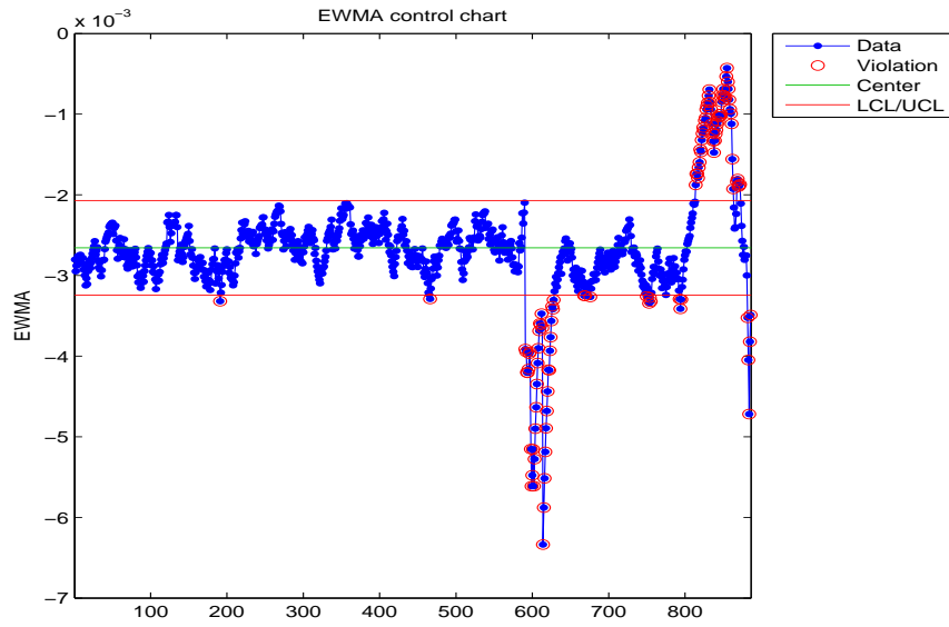
Figure B.11: EWMA chart for the tri-mean of the healthy bearing.
