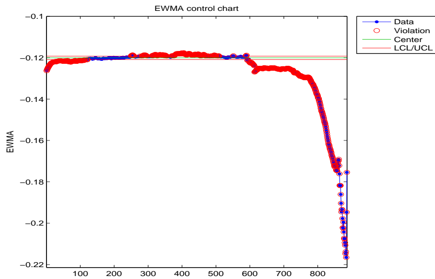
Figure B.59: EWMA chart for the 10 th percentile of the healthy bearing.
