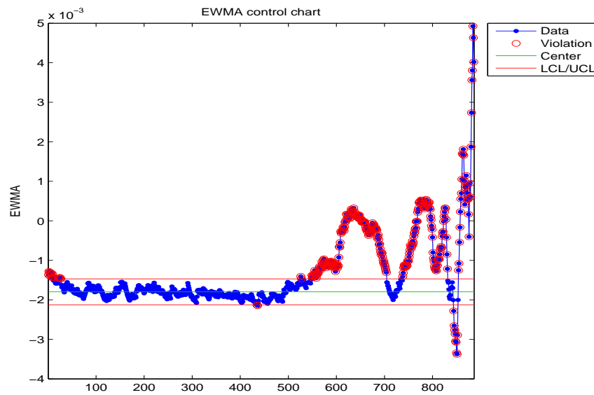
Figure B.10: EWMA chart for the tri-mean of the failed bearing.
