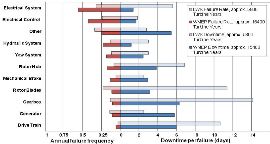
Figure 1.9: Wind turbine reliability by subsystem (onshore) (Crabtree, 2011).
