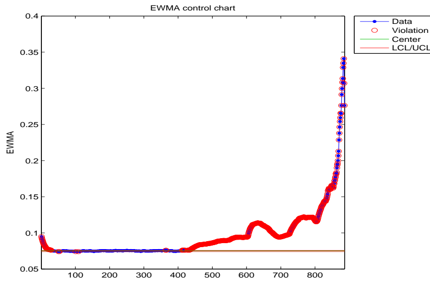
Figure B.37: EWMA chart for the median absolute deviation of the failed bearing.
