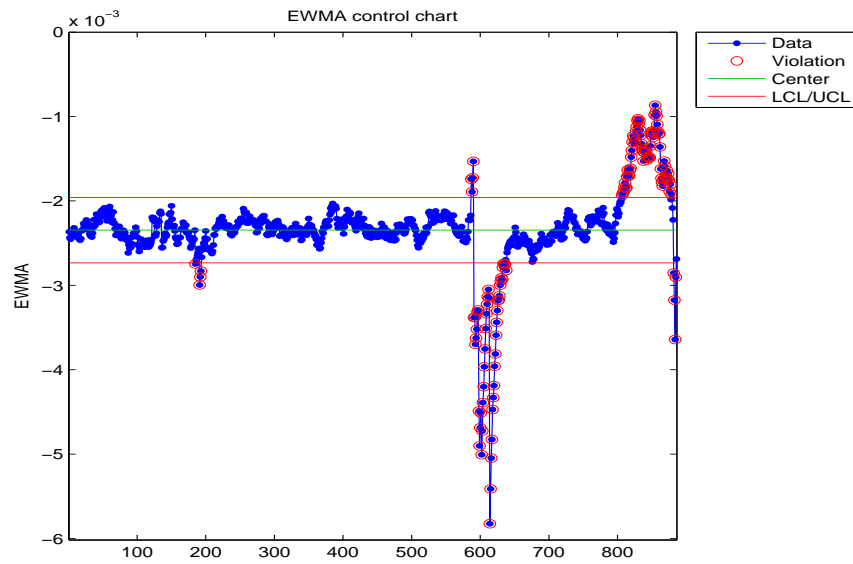
Figure B.17: EWMA chart for the winsorized mean of the healthy bearing.
