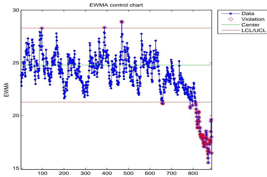
Figure B.56: EWMA chart for the peak to average power ratio of the healthy bearing.
