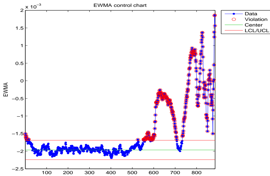
Figure B.16: EWMA chart for the winsorized mean of the failed bearing.
