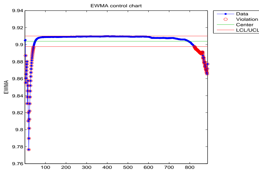
Figure B.77: EWMA chart for the KT entropy of the healthy bearing.
