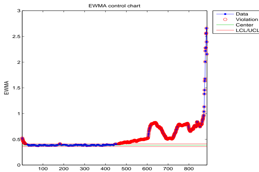
Figure B.34: EWMA chart for the maximum of the failed bearing.
