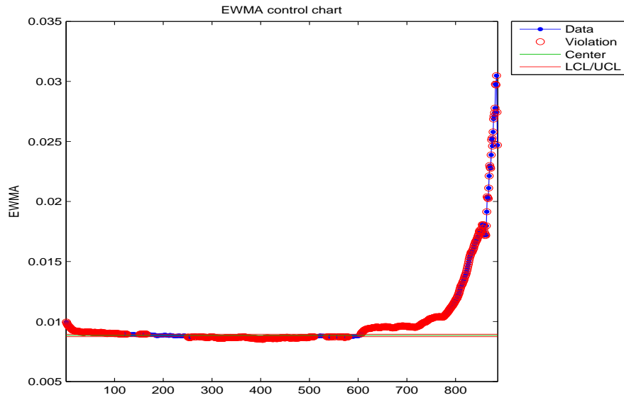
Figure B.23: EWMA chart for the variance of the healthy bearing.
