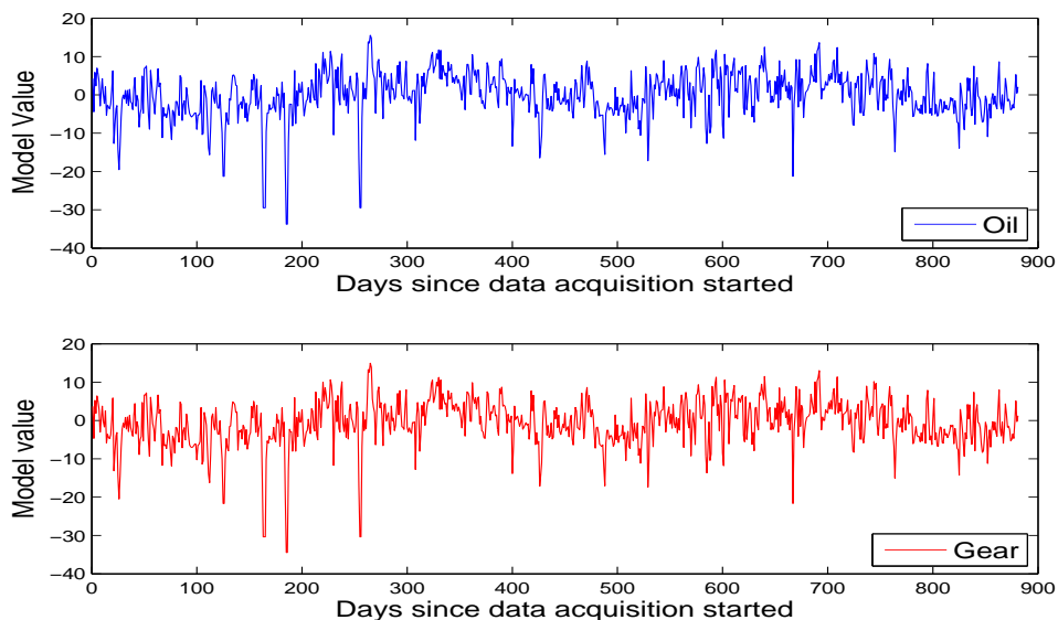
Figure 4.8: Wind turbine 1 health metric over 2 months.
