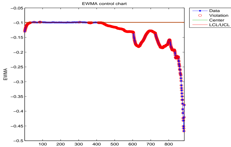
Figure B.58: EWMA chart for the 10 th percentile of the failed bearing.
