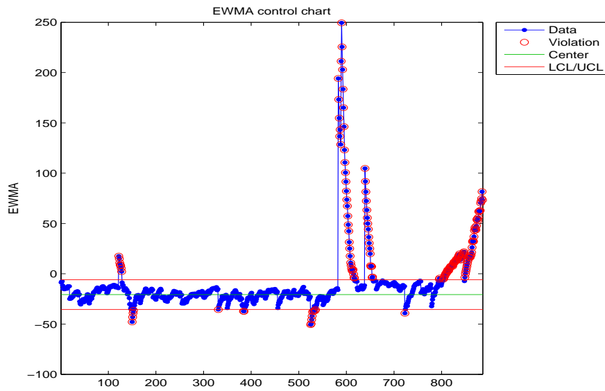
Figure B.80: EWMA chart for the Miller-Madow entropy of the healthy bearing.
