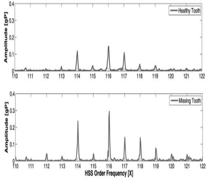
Figure 2.6: Sideband analysis as performed by Zappalá et al. (2012), showing healthy and missing gear tooth fault.
