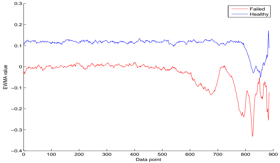
Figure B.42: Skewness over time of the failed and healthy bearing.
