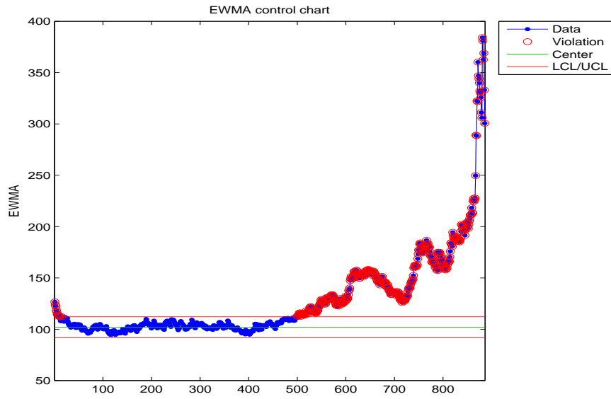
Figure B.82: EWMA chart for the James-Stein shrinkage entropy of the failed bearing.
