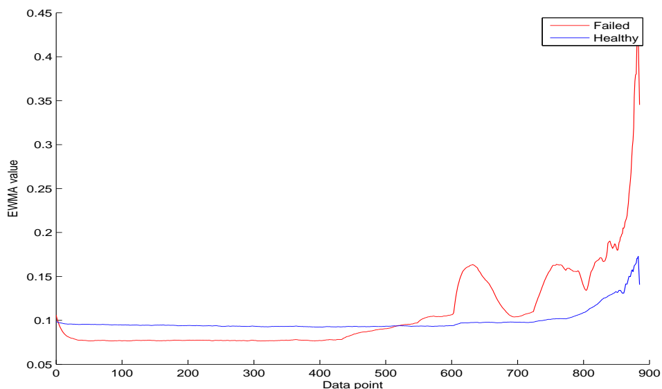
Figure 4.4: The RMS of the failed and healthy bearing.
