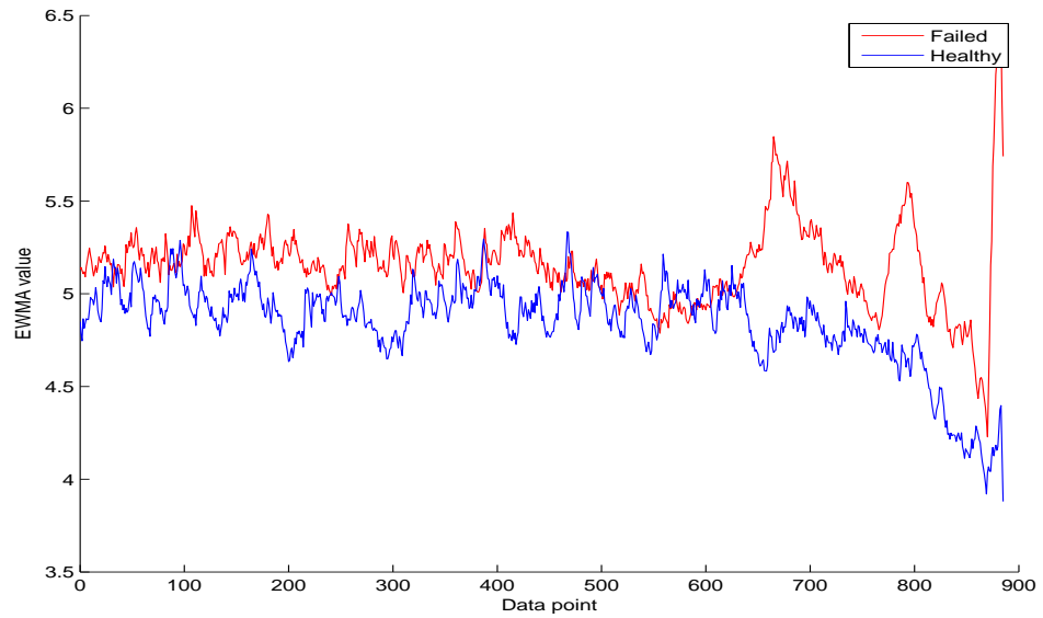
Figure B.54: Crest factor over time of the failed and healthy bearing.
