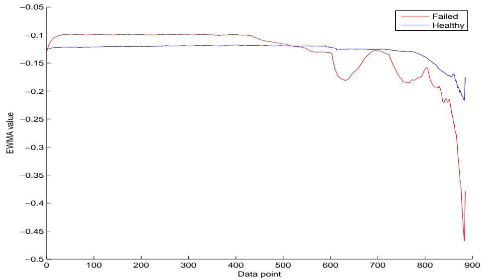
Figure B.60: 10 th percentile over time of the failed and healthy bearing.
