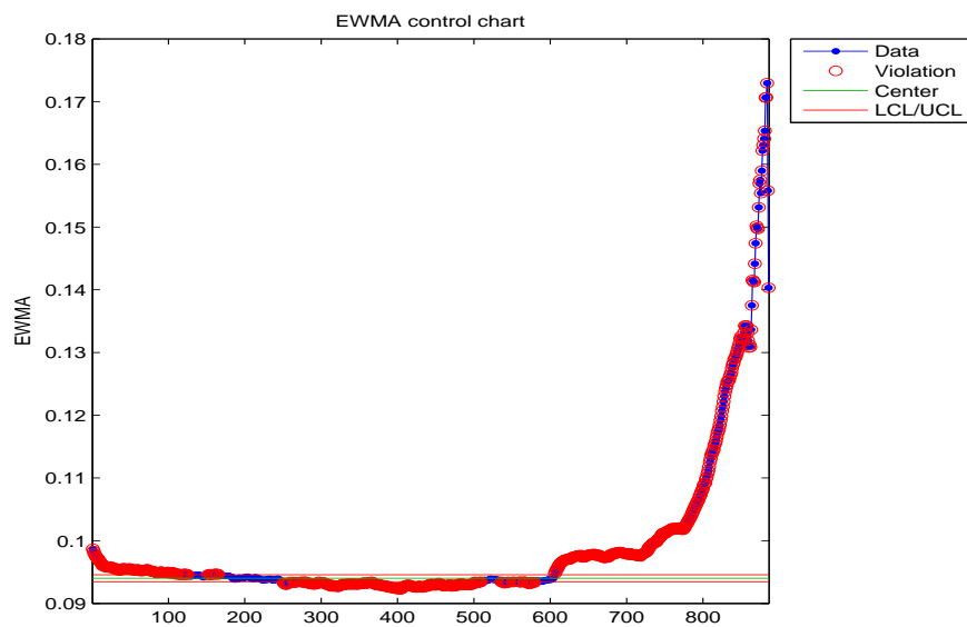
Figure B.20: EWMA chart for the standard deviation of the healthy bearing.
