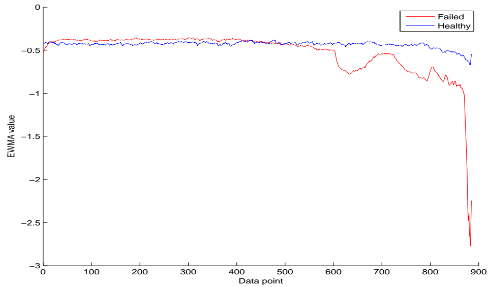
Figure B.33: Minimum over time of the failed and healthy bearing.
