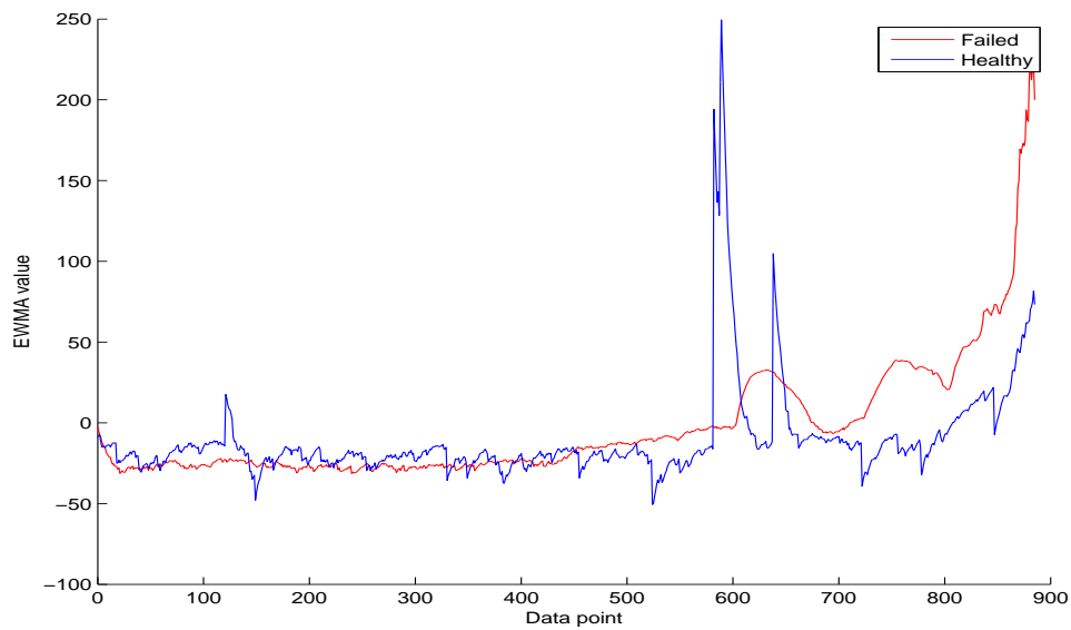
Figure B.81: Miller-Madow entropy over time of the failed and healthy bearing.
