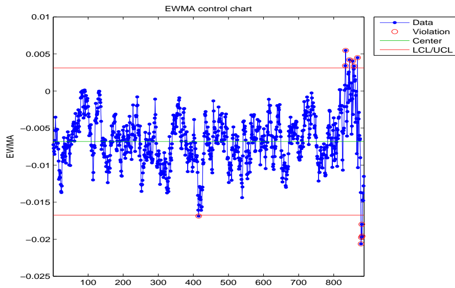
Figure B.8: EWMA chart for the mode of the healthy bearing.
