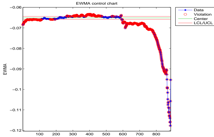
Figure B.62: EWMA chart for the 25 th percentile of the healthy bearing.
