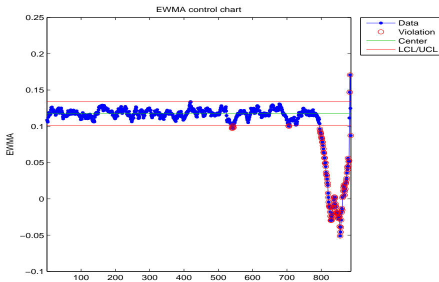
Figure B.41: EWMA chart for the skewness of the healthy bearing.
