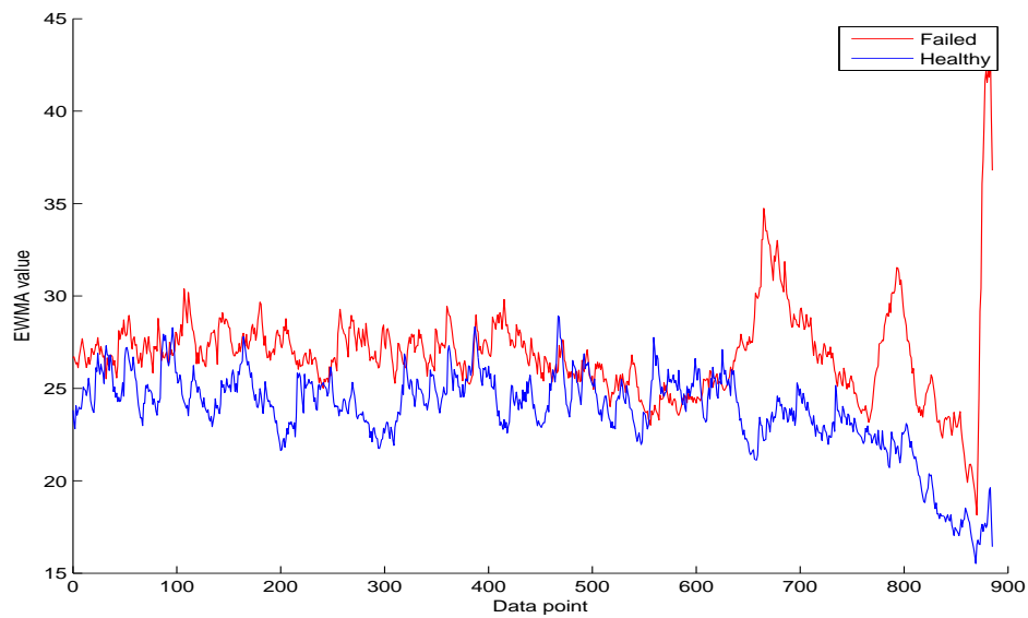
Figure B.57: Peak to average power ratio over time of the failed and healthy bearing.
