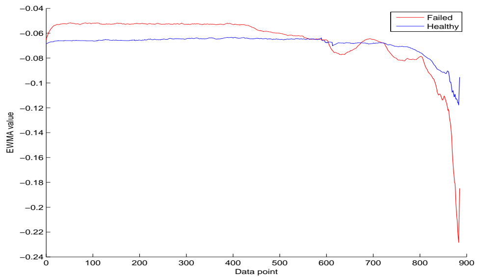
Figure B.63: 25 th percentile over time of the failed and healthy bearing.
