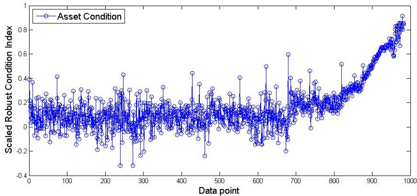
Figure 6.25: Time series of bearing condition of suspended bearing (bearing 2, validation dataset).
