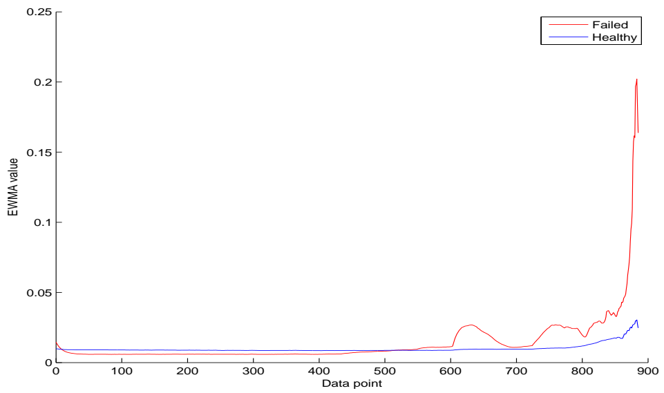
Figure B.24: Variance over time of the failed and healthy bearing.
