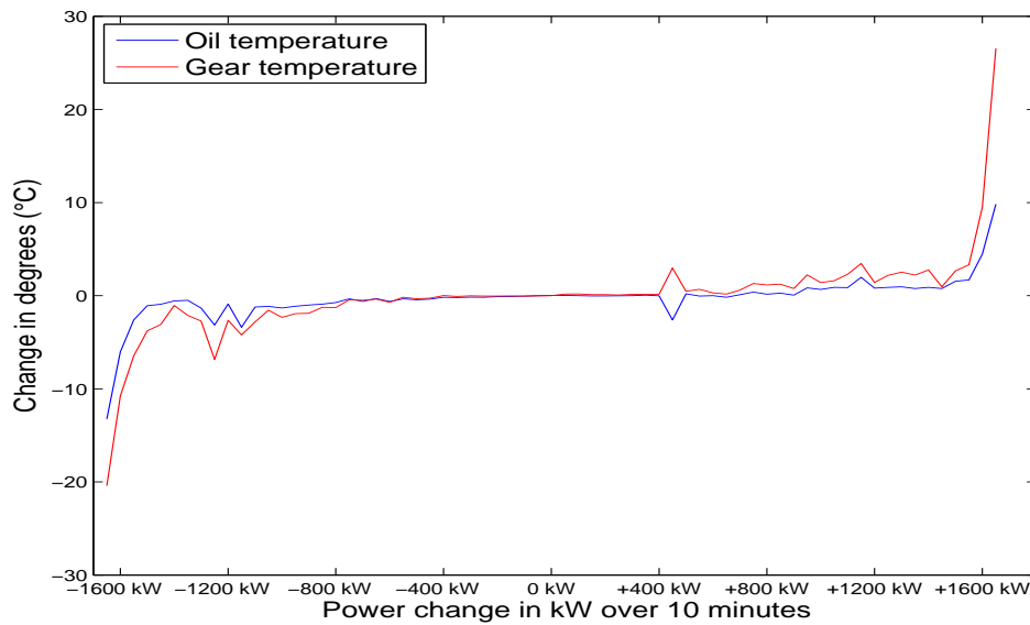
Figure 4.7: Normalisation of SCADA data against transient states based upon 10 minute SCADA data.
