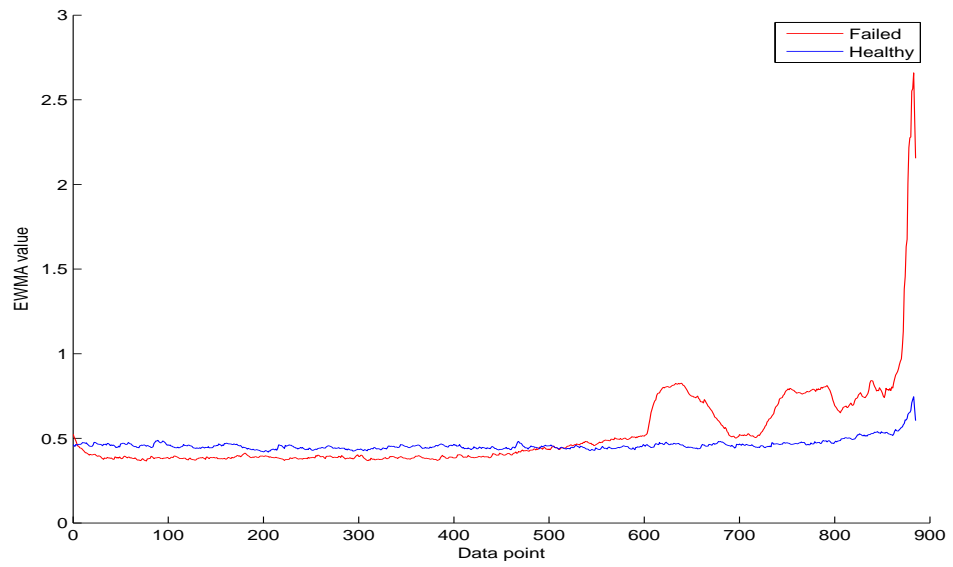
Figure B.36: Maximum over time of the failed and healthy bearing.
