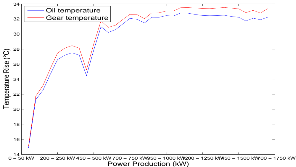
Figure 4.6: Normalisation of SCADA data against turbine loading based upon 10 minute SCADA data.
