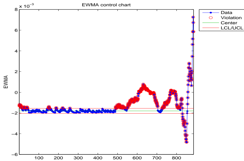
Figure B.4: EWMA chart for the median of the failed bearing.
