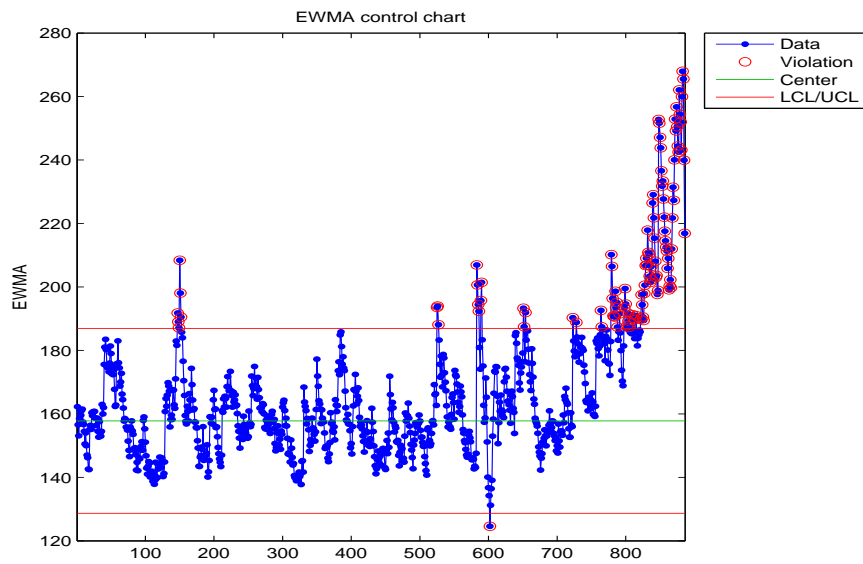
Figure B.83: EWMA chart for the James-Stein shrinkage entropy of the healthy bearing.
