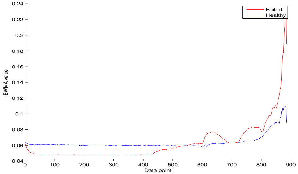
Figure B.66: 75 th percentile over time of the failed and healthy bearing.
