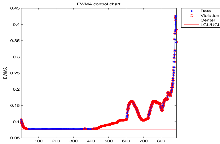
Figure B.13: EWMA chart for the RMS of the failed bearing.
