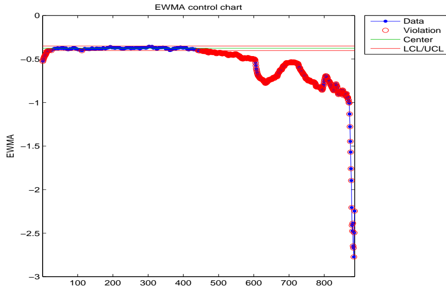
Figure B.31: EWMA chart for the minimum of the failed bearing.
