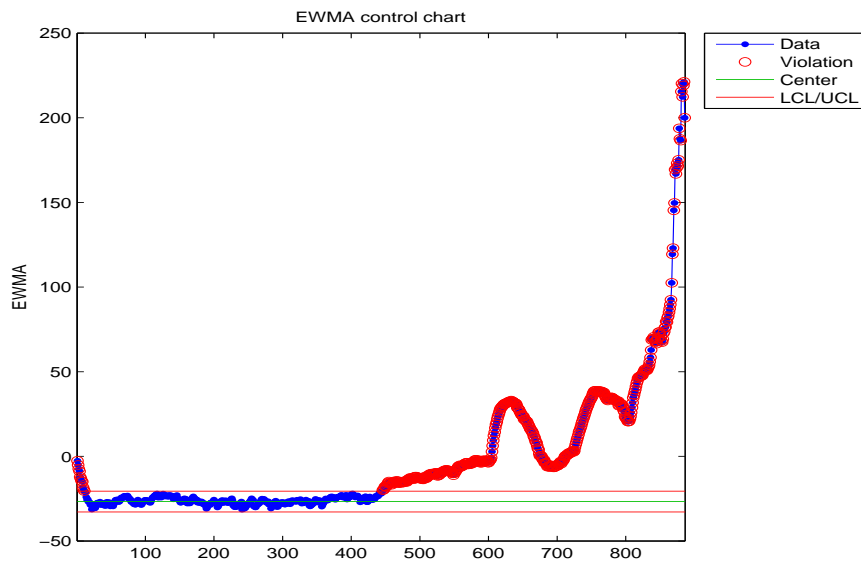
Figure B.79: EWMA chart for the Miller-Madow entropy of the failed bearing.
