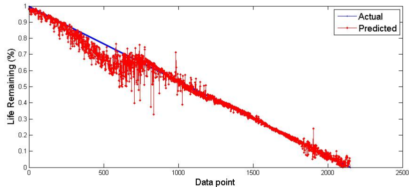
Figure 6.22: Refined RUL estimation of bearing 3 (training dataset).
