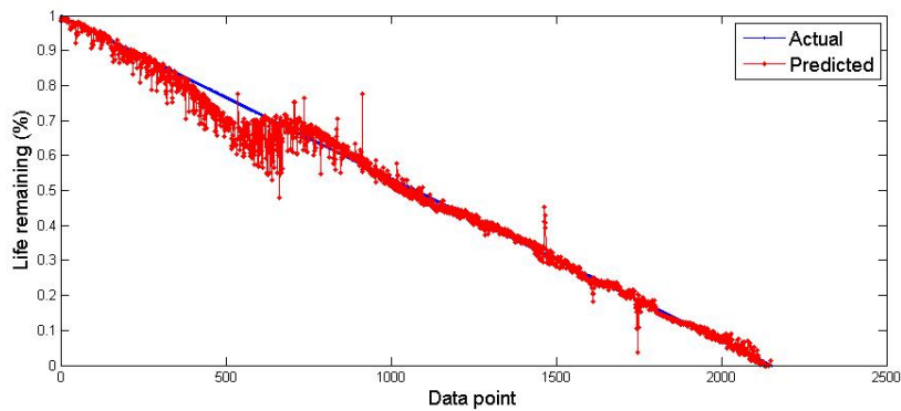
Figure 6.21: Refined RUL estimation of bearing 2 (training dataset).
