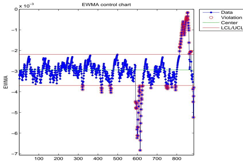
Figure B.5: EWMA chart for the median of the healthy bearing.
