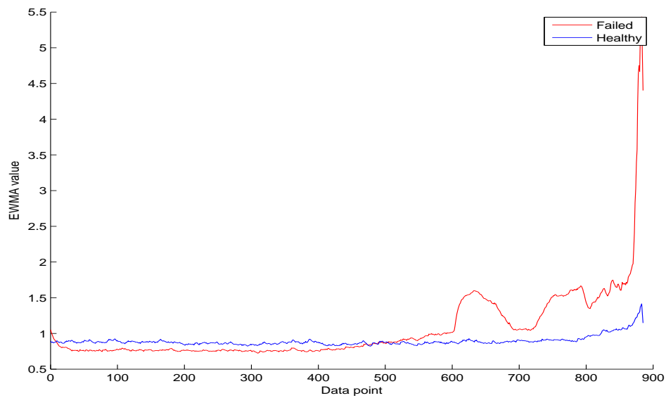
Figure B.30: Range over time of the failed and healthy bearing.
