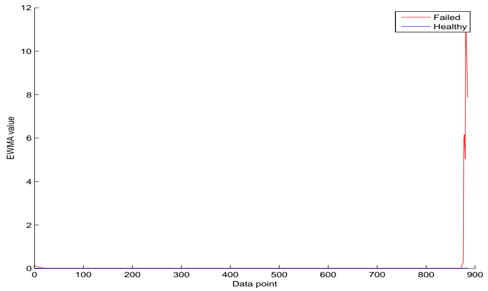
Figure B.51: Hyperflatness over time of the failed and healthy bearing.
