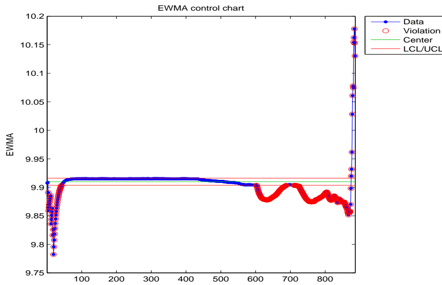
Figure B.76: EWMA chart for the KT entropy of the failed bearing.
