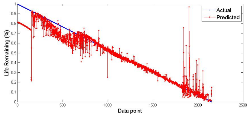
Figure 6.23: Validation of refined RUL estimation on independent failure history with r = .96 . (bearing 1, validation dataset).
