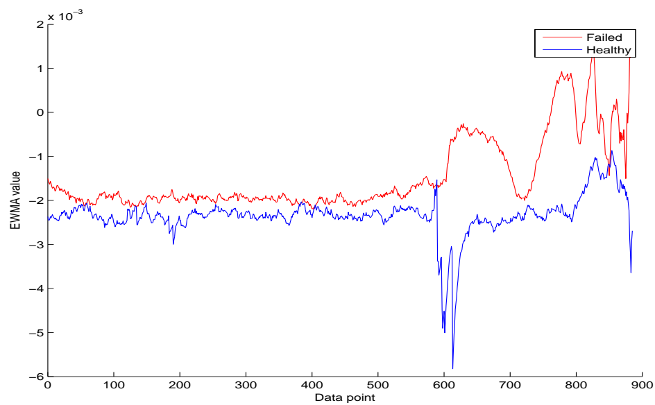
Figure B.18: Winsorized mean over time of the failed and healthy bearing.
