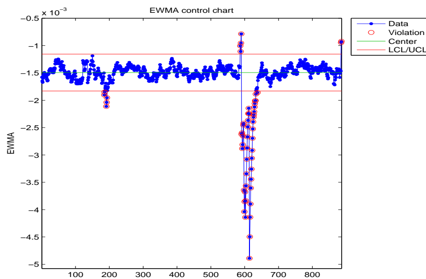
Figure B.2: EWMA chart for the mean of the healthy bearing.
