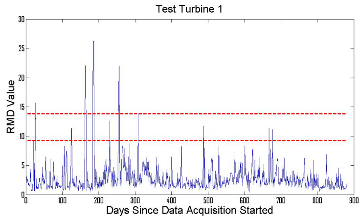
Figure 6.4: Thresholds for test turbine 1 plotted against health index over time.
