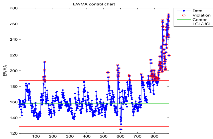
Figure B.71: EWMA chart for the Shannon entropy of the healthy bearing.
