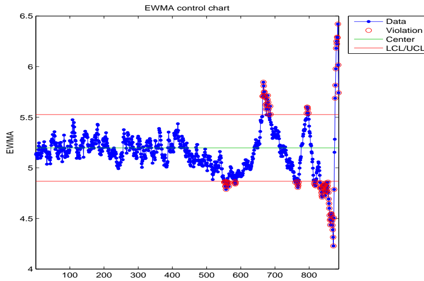
Figure B.52: EWMA chart for the crest factor of the failed bearing.
