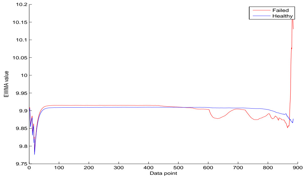
Figure B.78: KT entropy over time of the failed and healthy bearing.
