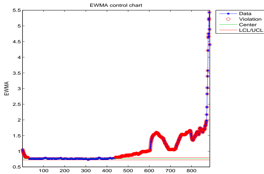
Figure B.28: EWMA chart for the range of the failed bearing.
