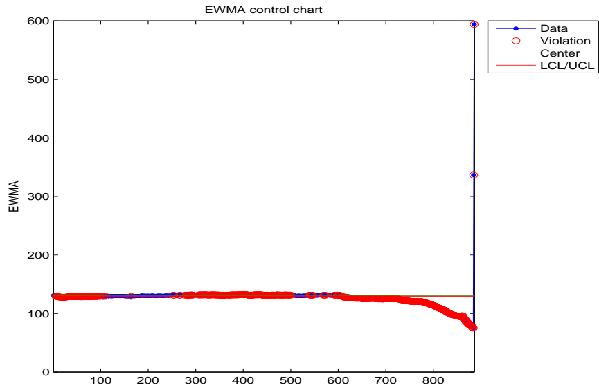
Figure B.74: EWMA chart for the Chao-Shen entropy of the healthy bearing.
