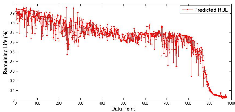
Figure 6.24: Validation of refined RUL estimation on independent suspension history (bearing 2, validation dataset).
