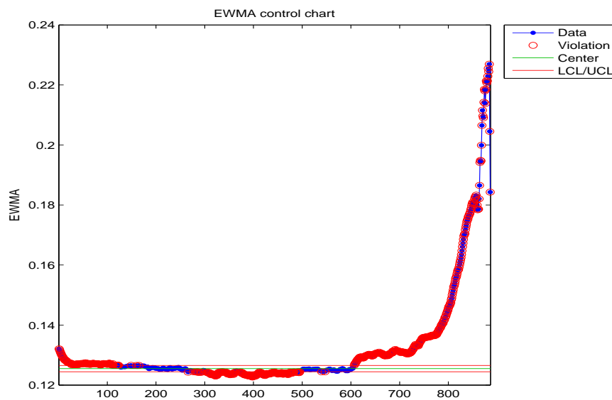
Figure B.26: EWMA chart for the IQR of the healthy bearing.
