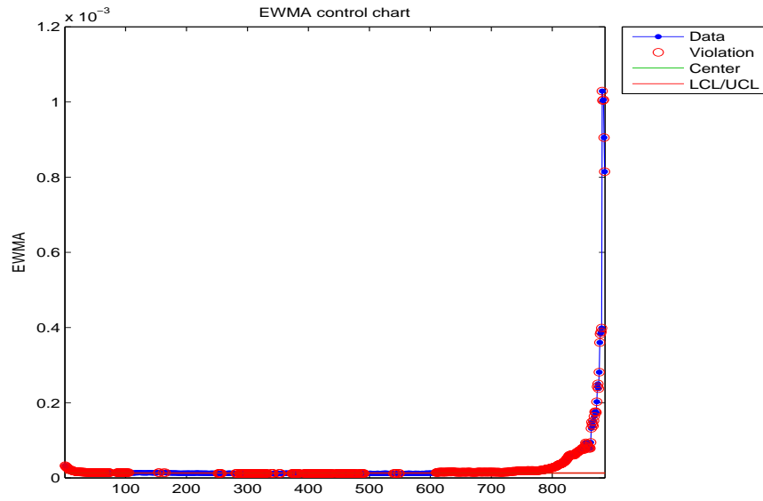
Figure B.50: EWMA chart for the hyperflatness of the healthy bearing.
