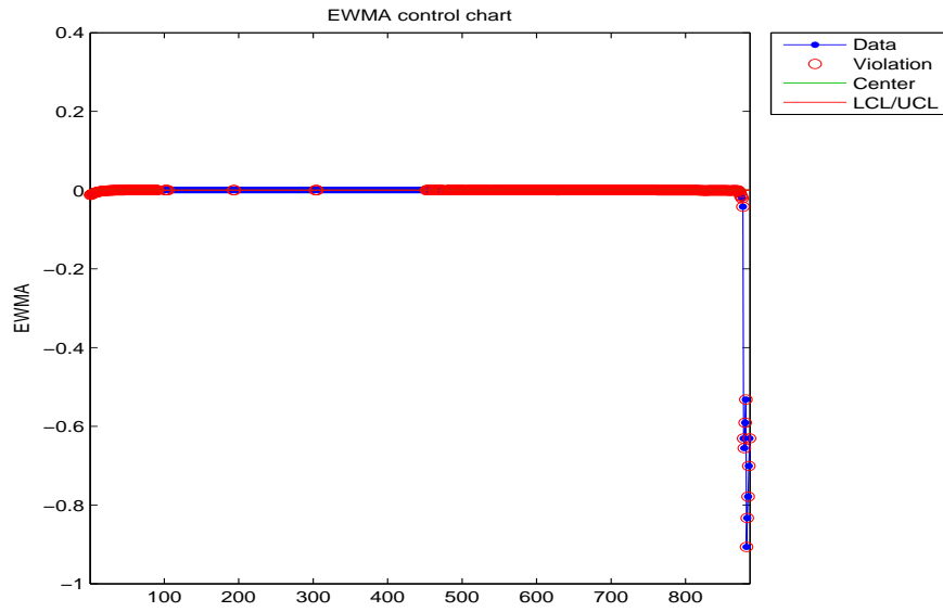
Figure B.46: EWMA chart for the hyperskewness of the failed bearing.
