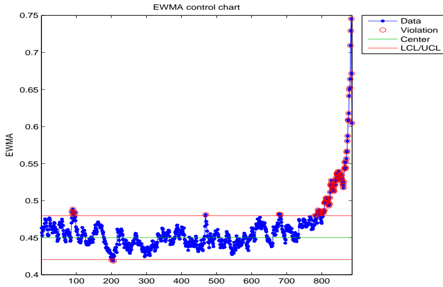
Figure B.35: EWMA chart for the maximum of the healthy bearing.
