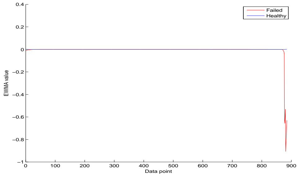
Figure B.48: Hyperskewness over time of the failed and healthy bearing.
