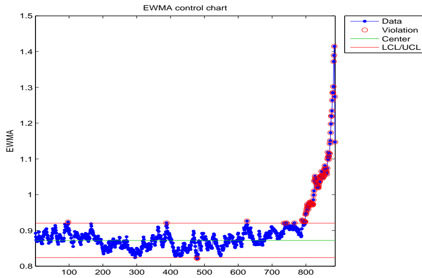
Figure B.29: EWMA chart for the range of the healthy bearing.
