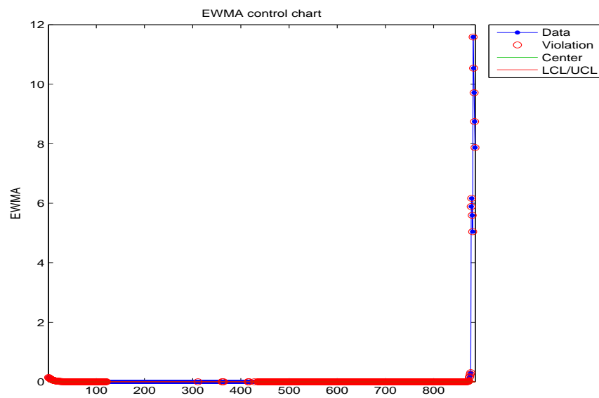
Figure B.49: EWMA chart for the hyperflatness of the failed bearing.
