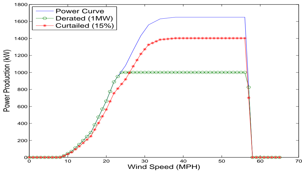
Figure 4.5: Example Vestas 1.65 MW wind turbine power curve with additional power curves showing curtailment (by 15%) and de-rating (to 1 MW).
