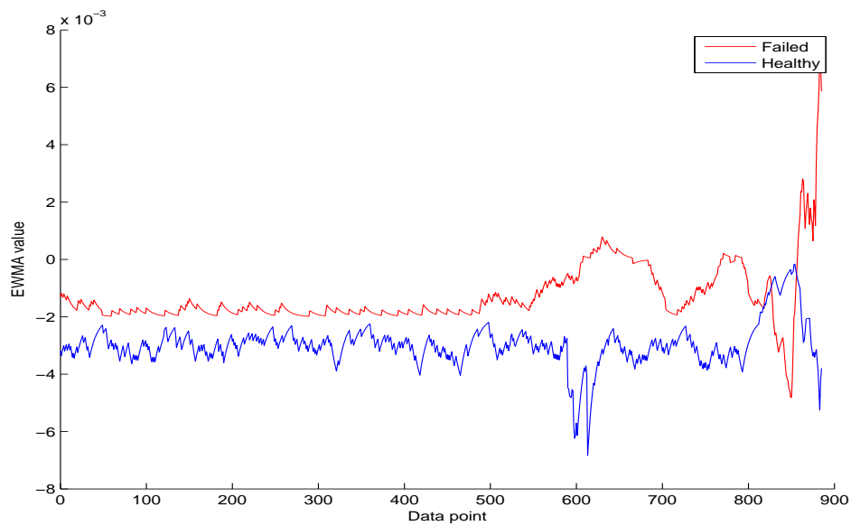
Figure B.6: Median over time of the failed and healthy bearing.
