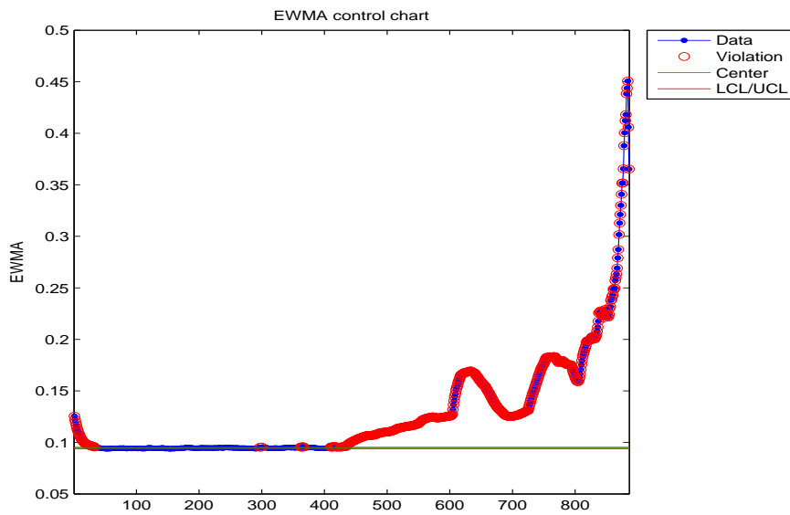
Figure B.67: EWMA chart for the 90 th percentile of the failed bearing.
