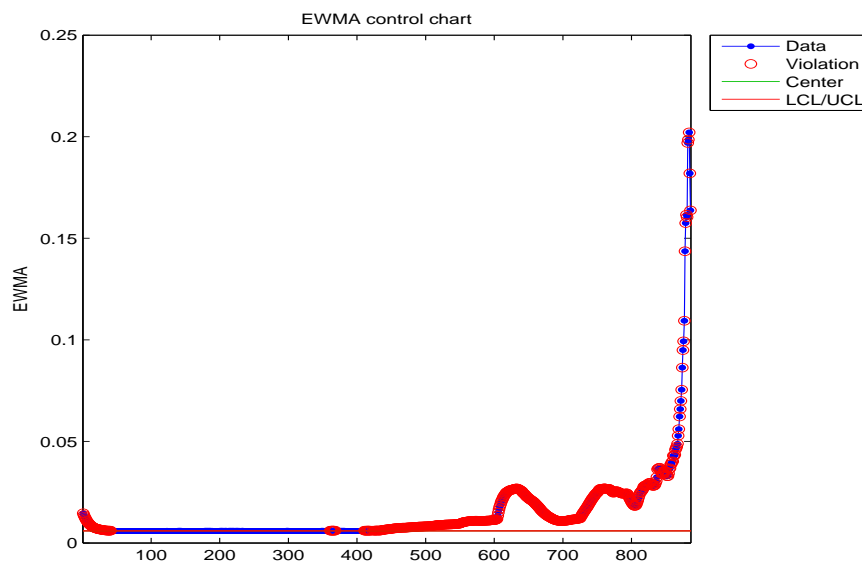
Figure B.22: EWMA chart for the variance of the failed bearing.
