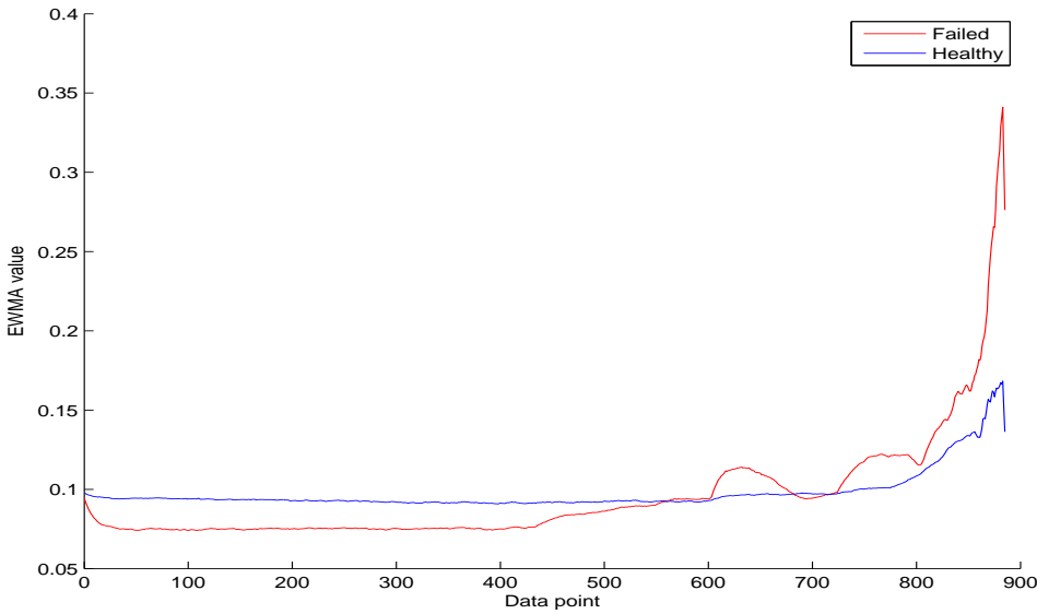
Figure B.39: Median absolute deviation over time of the failed and healthy bearing.
