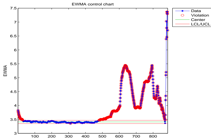
Figure B.43: EWMA chart for the kurtosis of the failed bearing.
