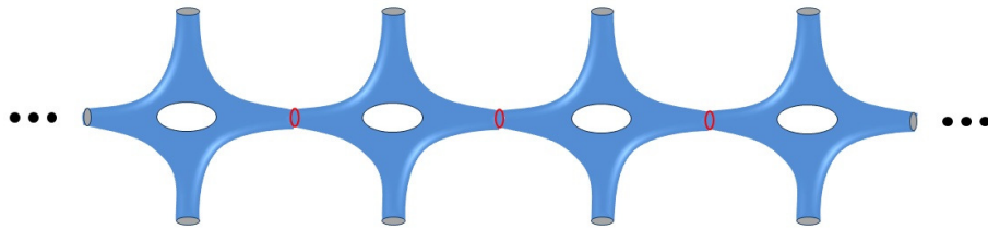
Figure 3.3: Combining an infinite number of elementary spectral curves to generate a (1+1)-dimensional theory. By performing a similar gluing along the vertical direction we expect to generate a (2+1)-dimensional theory.
