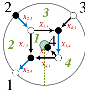
Figure C.1: An on-shell diagram on an annulus. This particular graph can be planarized by flipping the X_{1,1} edge.
