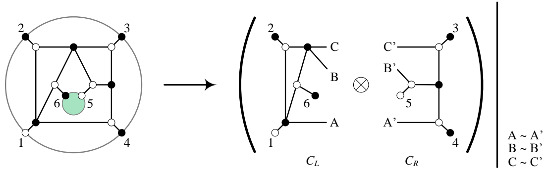
Figure 6.10: On the left, NMHV leading singularity corresponding to (345) = 0 . This diagram can be obtained by the two diagrams on the right upon direct product and projection of the edges A \sim A' , B \sim B' , C \sim C' .
