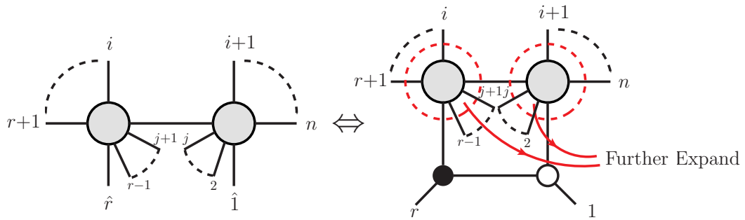
Figure 6.2: A one-to-one correspondence between a BCFW diagram with non-adjacent shifts and a non-planar two-mass-hard box. The tree-level amplitudes at two massive corners can be further expanded into either non-planar or planar two-mass-hard boxes until reaching an on-shell diagram representation of the BCFW diagram.
