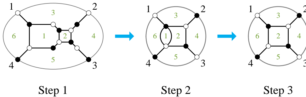
Figure 2.12: A reduction of the example in Figure 2.8.
