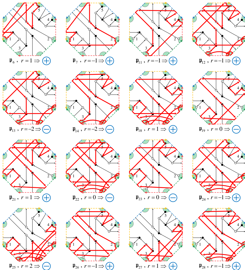
Figure A.2: Flows contributing to (A.2.2) completed to loops within the unit cell, the corresponding rotation numbers and the resulting signs.
