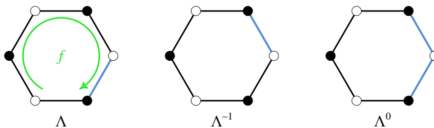
Figure 3.5: Examples of \Lambda scalings of a f_i cycle. We indicate the edge associated with a field with a non-zero vev in blue.
