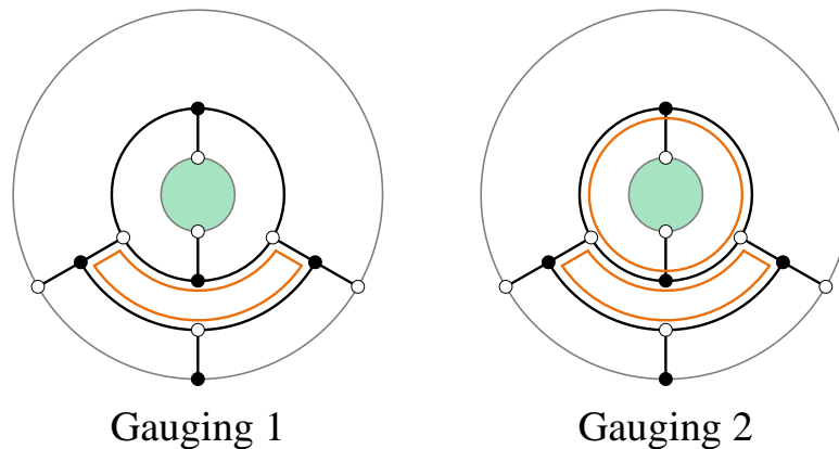
Figure 2.2: Difference between \text{BFT}_1 and \text{BFT}_2 in an example with two boundaries. The orange loops are those which are gauged in each gauging. The surface has genus g = 0 and hence there are no loops with non-trivial homology.
