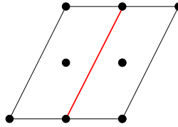
Figure 3.7: Toric diagram for the double F_0 . The red line indicates how we split it into two components.
