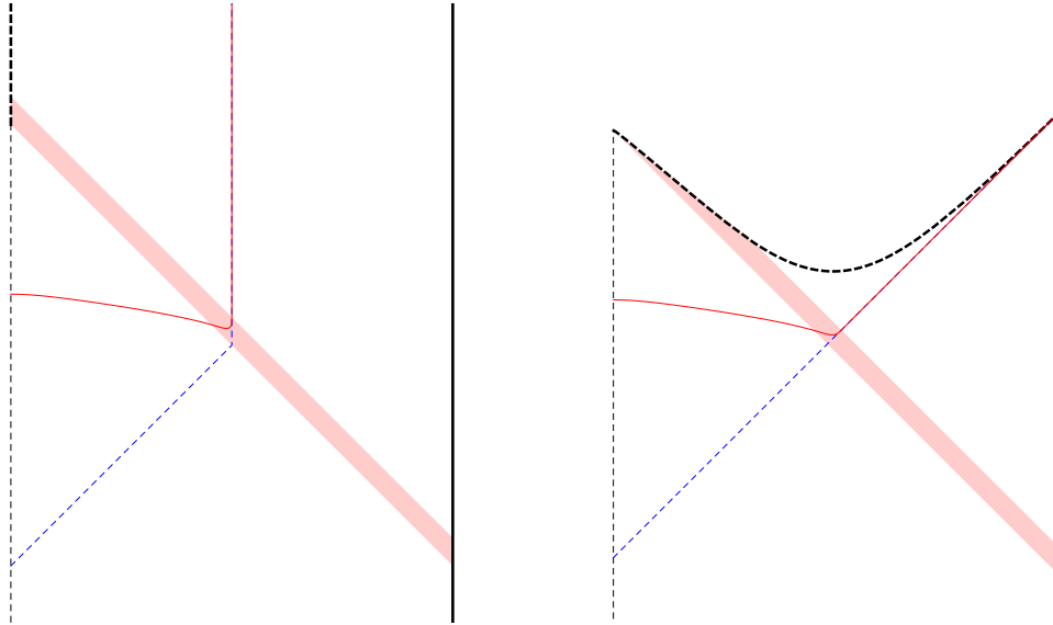
Figure 3.15: The region of relevant initial conditions. Surfaces whose earliest point (with respect to the ingoing time v ) lie outside or inside the curve reach the boundary or end in the singularity respectively.
