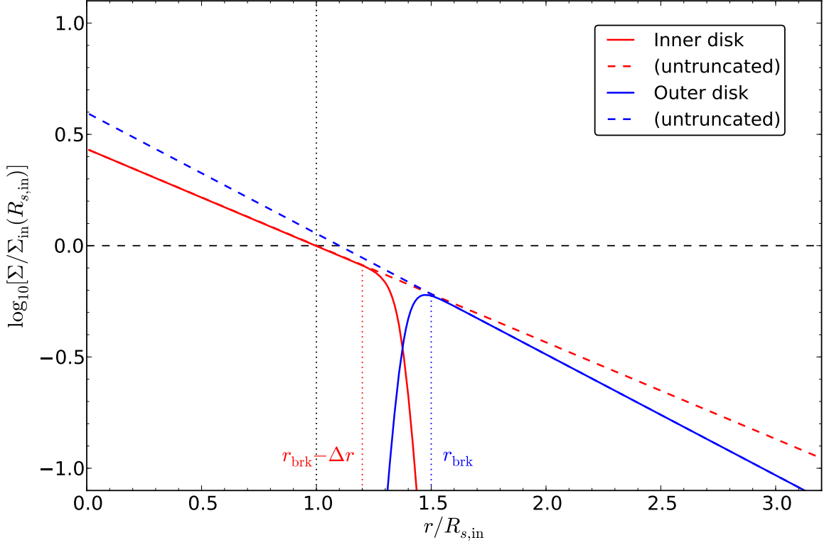
Figure 7.1: Cartoon example of the broken disk profile, indicating surface brightnesses of the inner (red) and outer (blue) disks (and their untruncated forms). r is normalised to the inner disk scale length, R_{s,\text{in}} (black dotted line), and \Sigma is normalised to the inner disk surface brightness at R_{s,\text{in}} (black dashed line). The inner ( r_{\text{brk}} - \Delta r ) and outer ( r_{\text{brk}} ) truncation radii are indicated by red and blue dotted lines. In this example, R_{s,\text{out}} = 0.8R_{s,\text{in}} , r_{\text{brk}} = 1.5R_{s,\text{in}} , and \Delta r = 0.3R_{s,\text{in}} .
