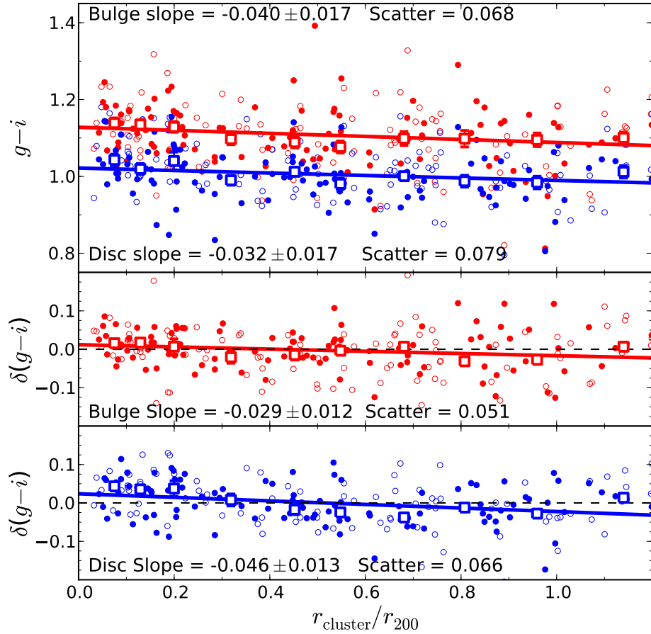
Figure 6.7: Colour-radius diagrams for Coma cluster galaxies (component gradients included). Upper panels: bulge (red) and disk (blue) g-i colours plotted against the projected separation between the galaxy and the Coma cluster centre (in fractional units of r_{200} ). Middle panels: Bulge g-i colours after subtracting the equivalent colour-magnitude trend, \delta(g-i) , plotted against r_{\text{cluster}} . Lower panels: disk g-i colours after subtracting the equivalent colour-magnitude trend, \delta(g-i) , plotted against r_{\text{cluster}} . Unfilled points indicate ‘flagged’ fits (containing weak extra components or asymmetries, see Section 3.5). Best-fit linear trends (solid lines) are fit to median colour values calculated in bins of projected radius (large square points), weighted by the robust standard error in each bin (error bars). Slope uncertainties are bootstrap errors calculated from the unbinned data.
