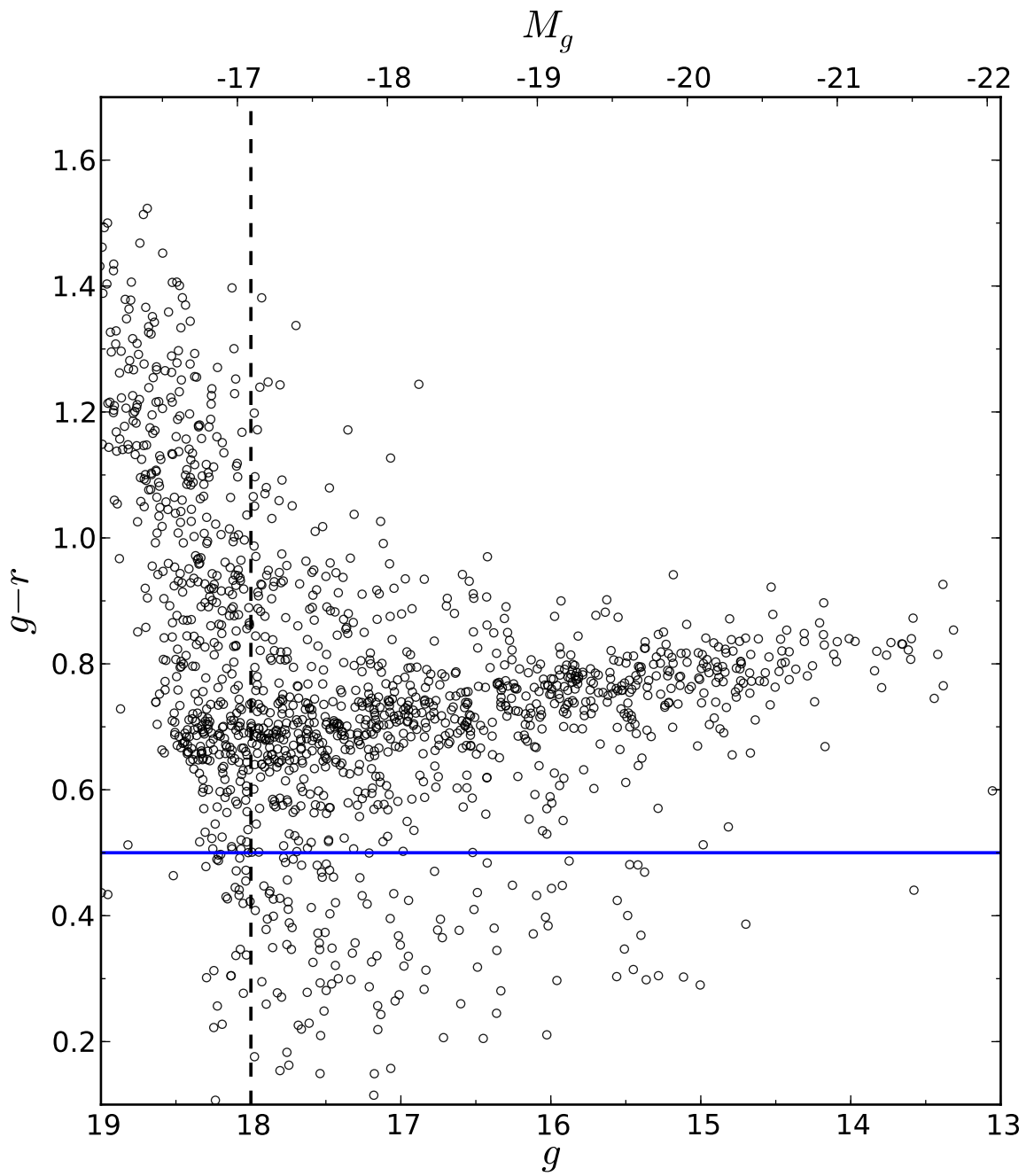
Figure 2.2: Colour-magnitude diagram for the Coma cluster, using total galaxy magnitudes from SDSS (DR9). The (g - r) colour, and g band brightness limits used to define the Coma sample are included as a solid blue line and dashed black line respectively.
