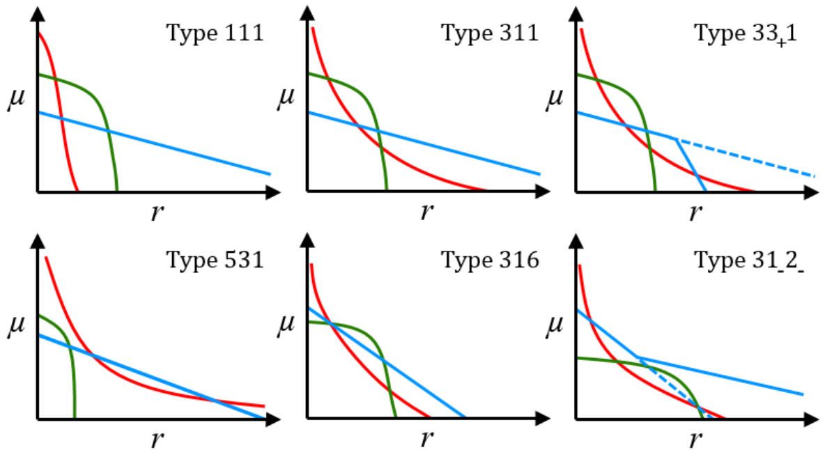
Figure 7.3: Cartoon surface brightness profiles for 3-component galaxies with profile Types 111 ( top left ), 311 ( top middle ), 33 +1 ( top right ), 531 ( bottom left ), 316 ( bottom middle ), and 31_2_ ( bottom right ), indicating the bulge (red), bar (green), and disk (blue) component surface brightnesses as a function of distance from the galaxy centre. The Type 33 +1 profile is identical to the Type 311 example, except for the disk truncation which causes the bulge to dominate at large radii. Likewise, the Type 31_2_ profile is equivalent to the Type 316 profile, except the outer Type III disk does not cross the bulge or bar profiles.
