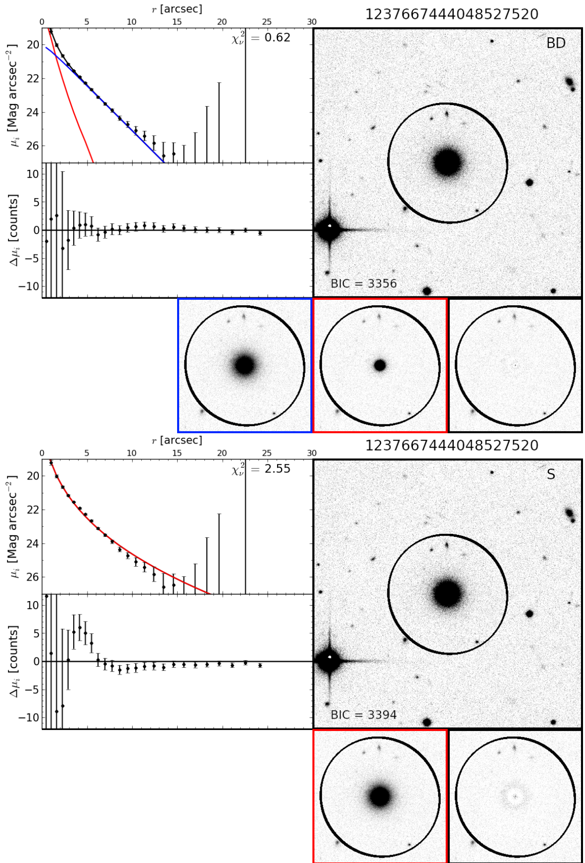
Figure 7.6: An example galaxy best fit by a BD model (DR8 ObjID 1237667444048527520). As Figure 7.5 for a BD model ( top : bulge = red, disk = blue), and the corresponding S model ( bottom : Sérsic = red).
