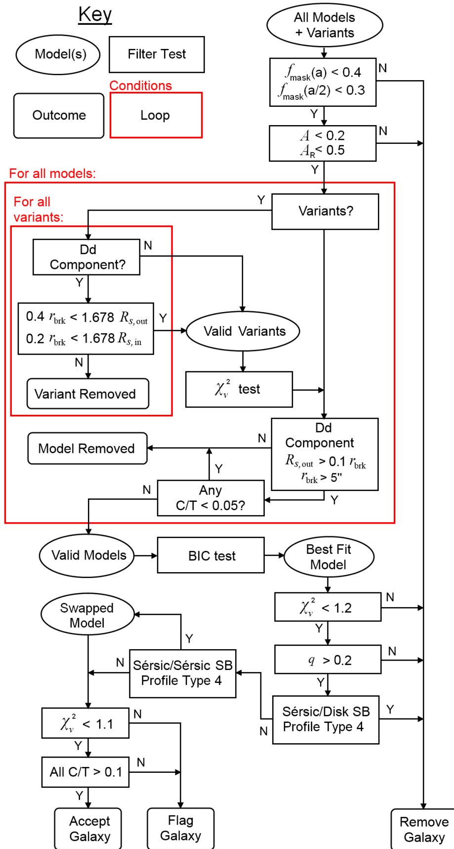
Figure 7.4: Flow chart illustrating multi-component fitting model selection for models S, BD, CD, BS, BDd, CDd, BDD, BSD, BSS, and BSDd. For profile type definitions, refer to Section 1.4 and Allen et al. (2006).
