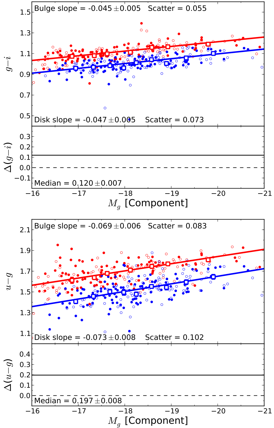
Figure 6.5: As Figure 6.1 for g - i ( top ) and u - g ( bottom ) colours and colour differences (bulges – disks) as a function of component magnitude when internal component gradients are permitted. Note that the slope of \Delta(C) is zero by definition for component magnitudes.
