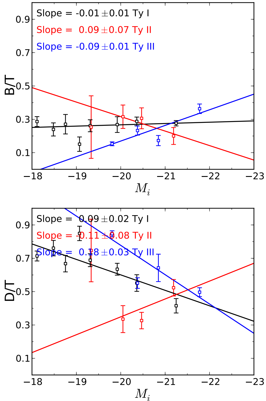
Figure 8.8: Component fraction ( C/T ) as a function of total absolute i band model magnitude for galaxies with Type I (black), Type II (red) and Type III (blue) disk models. Upper plot: bulge fraction ( B/T ). Lower plot: disk fraction ( D/T ). Note that due to the presence of bar components in some galaxies, B/T + D/T \neq 1 . Square points are median parameter values in bins of M_i , to which linear trends have been fit.
