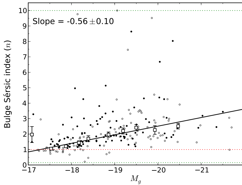
Figure 5.3: As Figure 5.2: the bulge Sérsic indices ( n ) for g band (analysis sample) galaxy models plotted against the corresponding absolute (bulge + disk) magnitudes ( M_g ).
