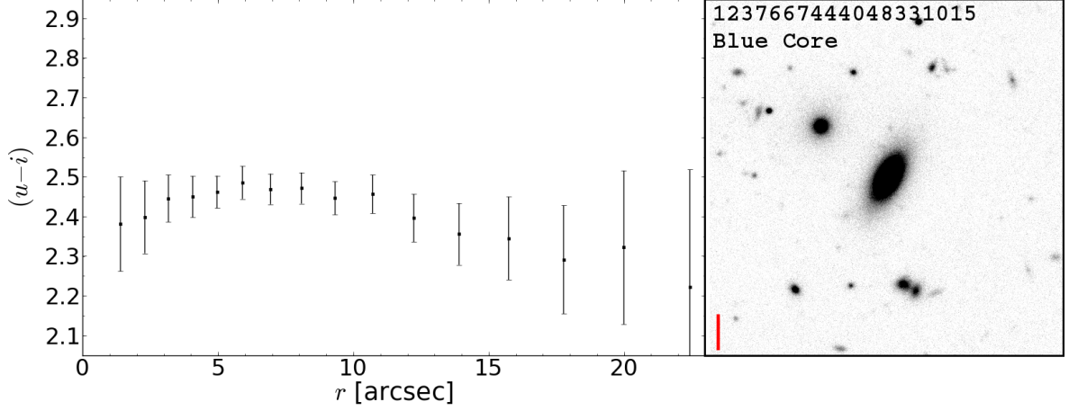
Figure 3.9: Example ( g band) thumbnail and radial (u - i) colour data (as measured in elliptical annuli) for a ‘blue core’ galaxy (SDSS DR8 ObjID 1237667444048331015). A red scale bar corresponding to 10'' ( \equiv 4.8 kpc) is included in the thumbnail.
