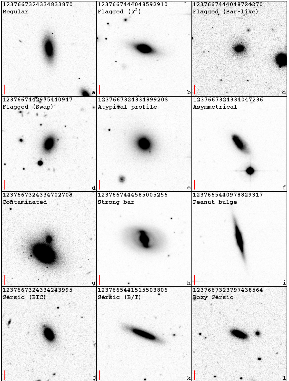
Figure 3.8: Example ( g band) thumbnail images of galaxies illustrating the filter subsamples described in Table 3.4. Each thumbnail includes the SDSS (DR8) ObjID of the example galaxy, and a red scale bar corresponding to 10'' ( \equiv 4.8 kpc).
