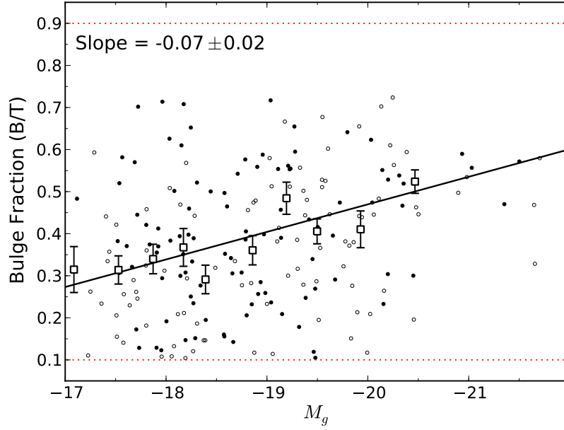
Figure 5.2: The galaxy bulge fractions (B/T) measured from g band (analysis sample) galaxy models plotted against the corresponding absolute (bulge + disk) magnitudes ( M_g ). Unfilled points indicate flagged fits (see Section 3.5). Best-fit linear trends (solid lines) are fit to median parameter values calculated in magnitude bins (large square points), weighted by the robust standard error in each bin (error bars). The slopes and their bootstrap errors (calculated from the unbinned data) are included in each plot. Dashed lines in each plot indicate any constraints on parameters values (green: hard limits imposed on GALFIT; red: sample filtering cuts).
