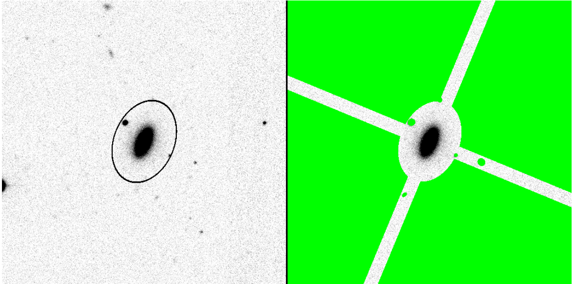
Figure 2.5: Example of image masking for SDSS DR8 ObjID 1237665427553321062. Left: Galaxy thumbnail with target ellipse overlotted in black. Right: Galaxy thumbnail with final cross mask (including neighbouring source masking) overlaid in green.
