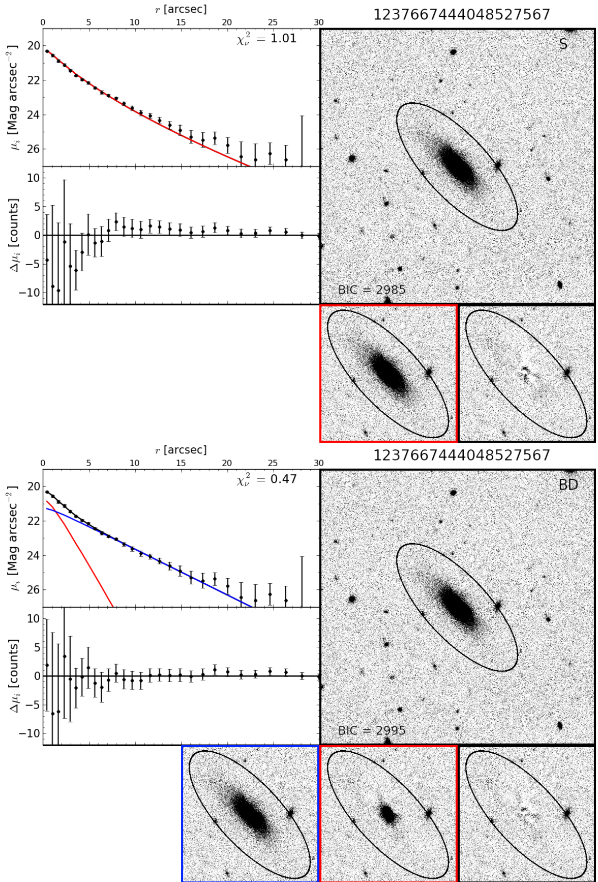
Figure 7.5: An example galaxy best fit by an S model (DR8 ObjID 1237667444048527567): Surface brightness profiles ( \mu_i ), residuals ( \Delta\mu_i ), and i band thumbnails for the S model ( top : Sérsic = red), and the corresponding BD model ( bottom : bulge = red, disk = blue). Small images depict isolated model components (border colours \equiv \mu_i plot), and the total residual (black borders). The target ellipse is noted in black in all thumbnails, and 1D \chi^2_\nu (major axis) and 2D BIC values are included for both models.
