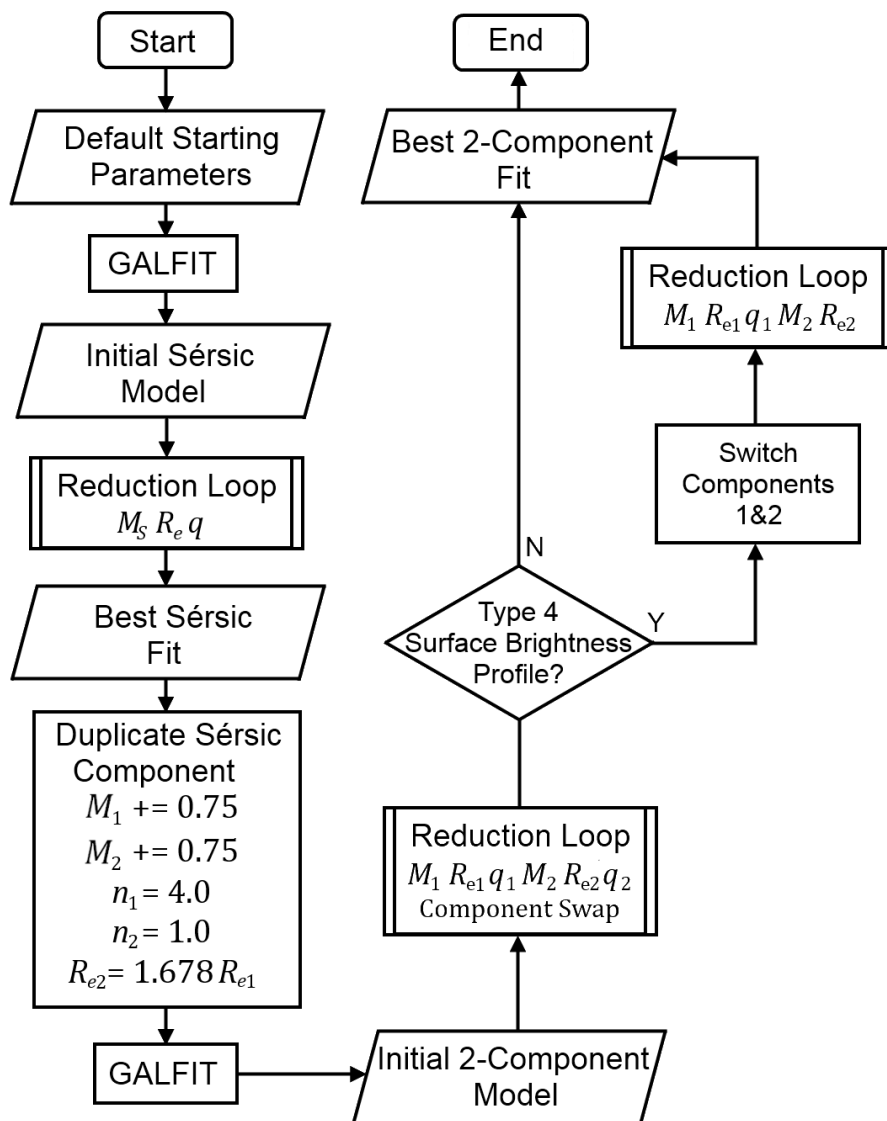
Figure 3.1: Flow chart: Overall fitting process for 1- and 2-component model fitting. The reduction loop process is described in Figure 3.2.
