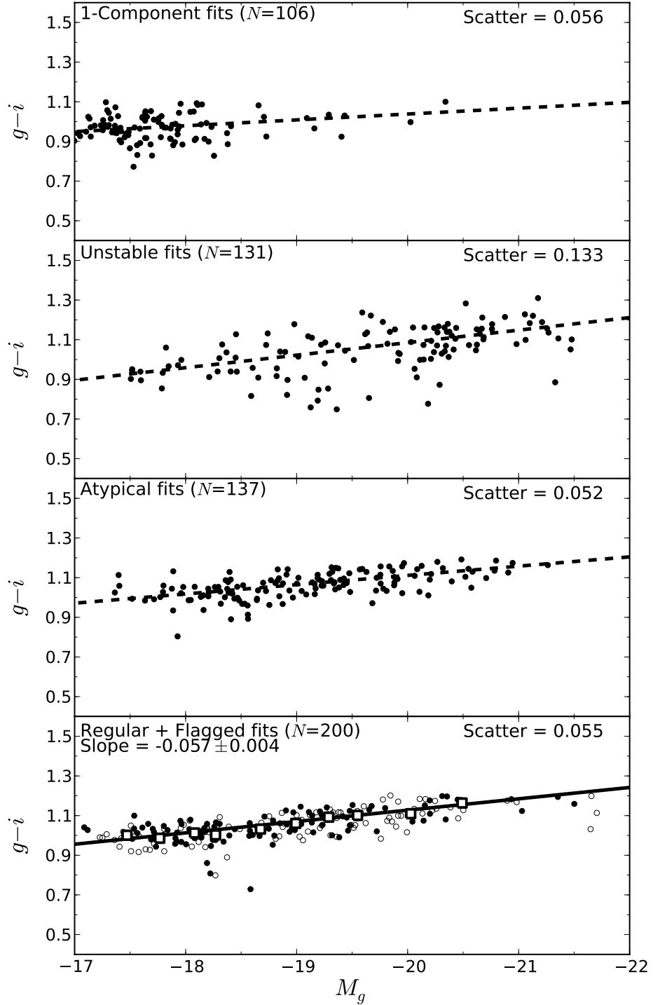
Figure 3.10: The measured ( GALFIT ) model g - i colours plotted against their absolute (bulge + disk) g band magnitudes. Top Panel: Galaxies best fit with a Sérsic-only model. Upper-middle Panel: Galaxies with no stable 1 or 2-component fit. Lower-middle Panel: 2-component galaxies which do not possess an archetypal central bulge + outer disk morphology. Bottom Panel: Regular (filled points) and flagged (unfilled points) fits. The large square points indicate median colour values calculated in magnitude bins, to which a linear trend (solid line) is fitted. The slope uncertainty is calculated from bootstrap fitting the unbinned data. This best fit line is plotted for comparison as a dashed line in the other three panels.
