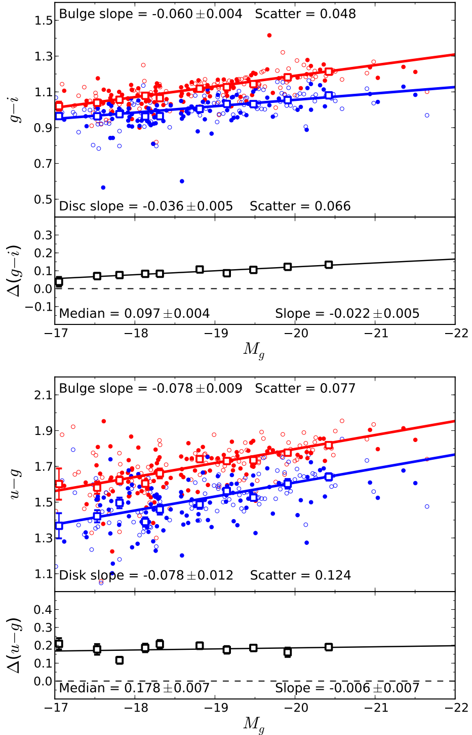
Figure 6.1: Colour-magnitude diagrams ( top: g - i , bottom: u - g ) for fixed multi-band structure. Upper panels: The bulge (red) and disk (blue) colours plotted against the absolute (bulge + disk) g band magnitudes of each galaxy. Lower panels: The colour difference (bulge – disk) plotted against absolute g band magnitude. Unfilled points indicate ‘flagged’ fits (containing weak extra components or asymmetries, see Section 3.5). Best-fit linear trends (solid lines) are fit to median colour values calculated in magnitude bins (large square points), weighted by the robust standard error in each bin (error bars). Slope uncertainties are bootstrap errors calculated from the unbinned data. A dashed black line at \Delta(g - i) = 0 is included in the lower plot for comparison.
