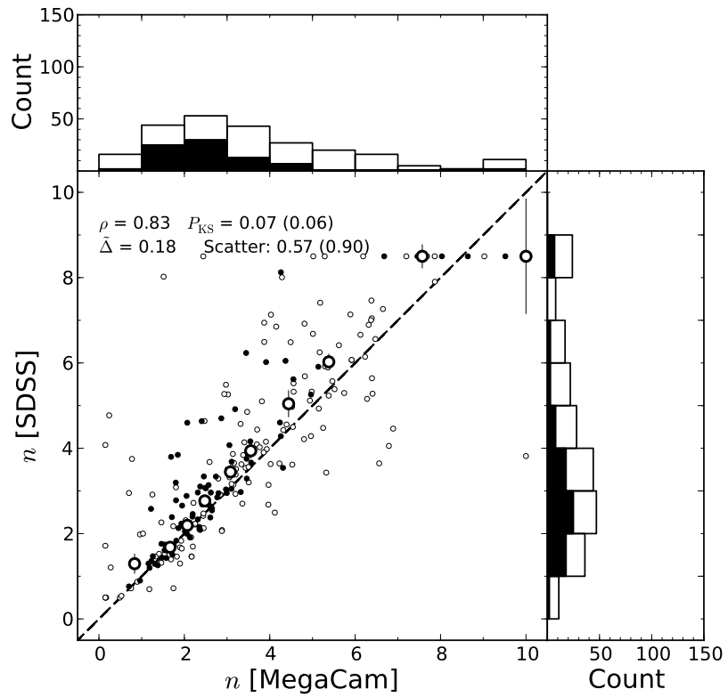
Figure 4.4: As Figure 4.1, displaying n for the Sérsic model (upper plot) and 2-component model bulge (lower plot) obtained from fitting MegaCam ( x ) and SDSS DR8 ( y ) imaging of Coma cluster galaxies.
