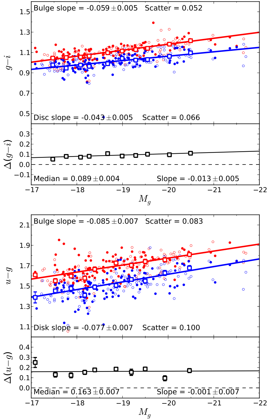
Figure 6.4: As Figure 6.1 for g - i ( top ) and u - g ( bottom ) colours and colour differences (bulges – disks) when internal component gradients are permitted. 60 galaxies (out of 200) are affected by the inclusion of component gradients.
