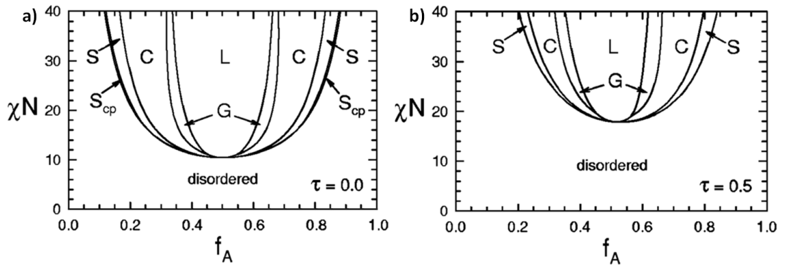
Figure 3.122: Phase diagrams for (a) a di-block copolymer ( \tau = 0.0 ) and (b) a symmetric ABA tri-block copolymer ( \tau = 0.5 ). Reprinted with permission from Matsen, M. W., The Journal of Chemical Physics , Vol. 113/13, Page 5539-5544, 2000. Copyright 2000, American Institute of Physics. 16
