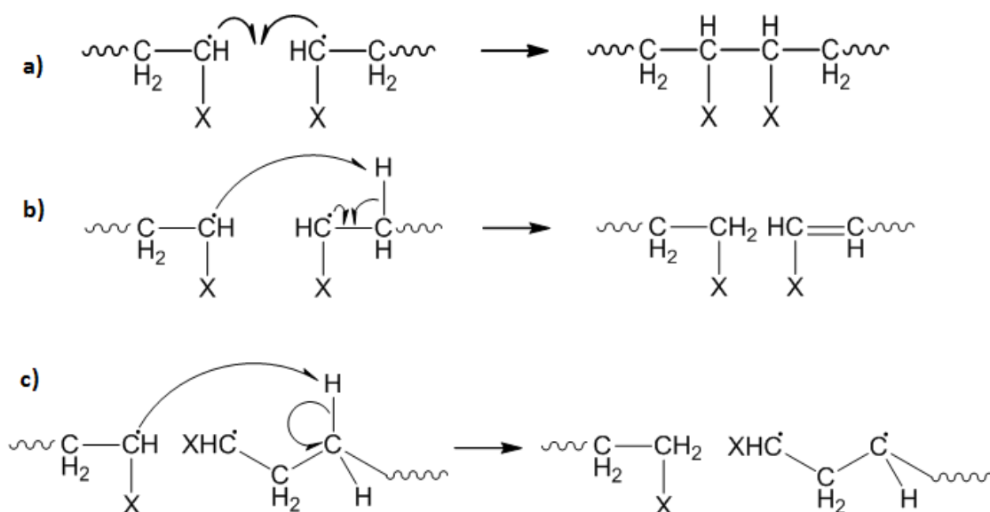
Figure 1.2: Mechanism for termination by (a) recombination (b) disproportionation and (c) chain transfer for a polymerization of a generic vinyl monomer, CH_2=CHX .
