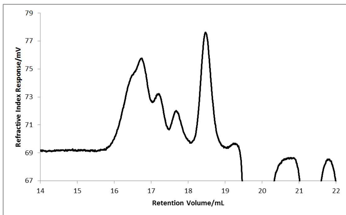
Figure 4.152: SEC trace for poly(butadiene- co -DPE-OSi) copolymer, P(Bd- co -D OSi )-2c, showing the refractive index response.
