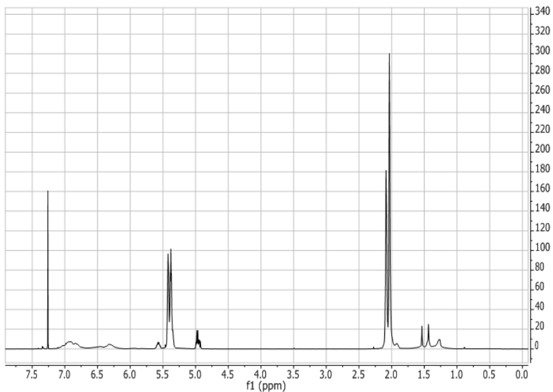
Figure 2.78: 1 H NMR spectrum (in CDCl 3 ) for the poly(styrene- co -DPE)- block -polybutadiene- block -poly(styrene- co -DPE) copolymer, P(SD)-PBd-P(SD)-3, synthesized in benzene with a molar feed ratio of 1.00 : 1.60 : 12.39 styrene : DPE : butadiene.
