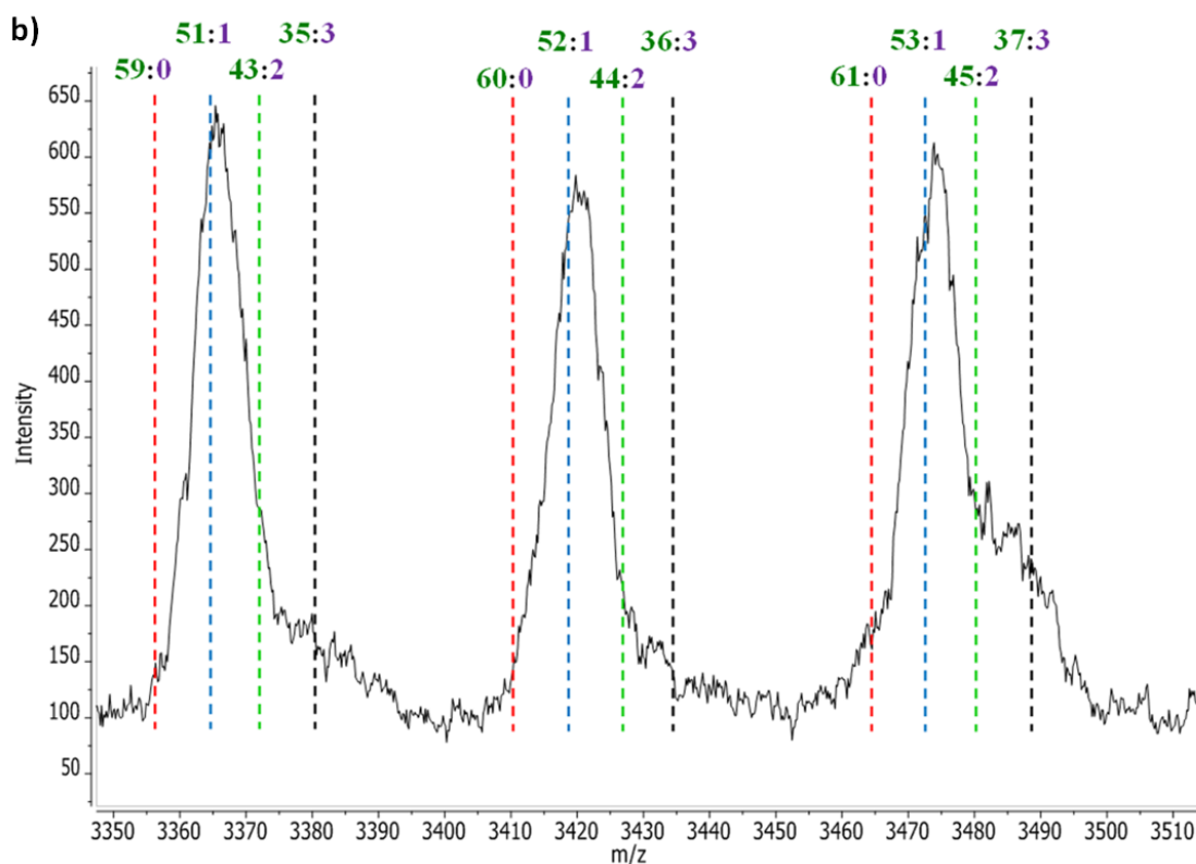
Figure 4.164: (a) MALDI-ToF mass spectrum for the anionic copolymerization (in benzene) of butadiene and DPE-OSi after 3 days, P(Bd-co-D OSi )-6a, with a molar feed ratio of Bd : DPE-OSi = 13.0 : 1.0 and (b) expansion showing the range m/z = 3350 – 3510 with red, blue and green dashed lines indicating where chains containing 0, 1 and 2 units of DPE-OSi respectively, would be expected to appear. The mole ratio of butadiene : DPE-OSi for any given chain is labelled with butadiene in green and DPE-OSi in purple.
