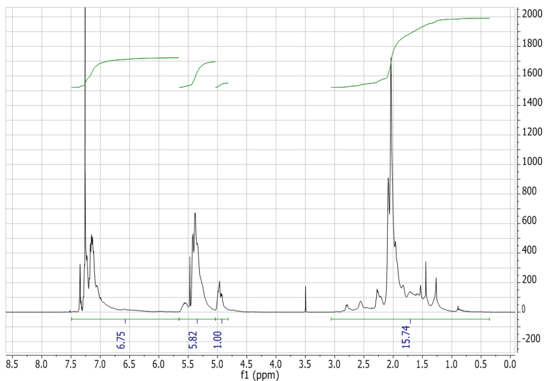
Figure 2.71: ^1\text{H} NMR spectrum (in \text{CDCl}_3 ) of Poly(butadiene- co -styrene- co -DPE), PBdSD-17, synthesized in toluene with a molar feed ratio of 1.00 : 1.00 : 1.87 styrene : DPE : butadiene with TMEDA injected after 22 hours when the reaction mixture was red.
