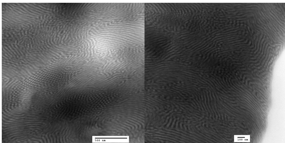
Figure 3.120: TEM images of the copolymer poly(butadiene- co -styrene- co -DPE), PBdSD-8, with the butadiene blocks stained black with OsO 4 .
