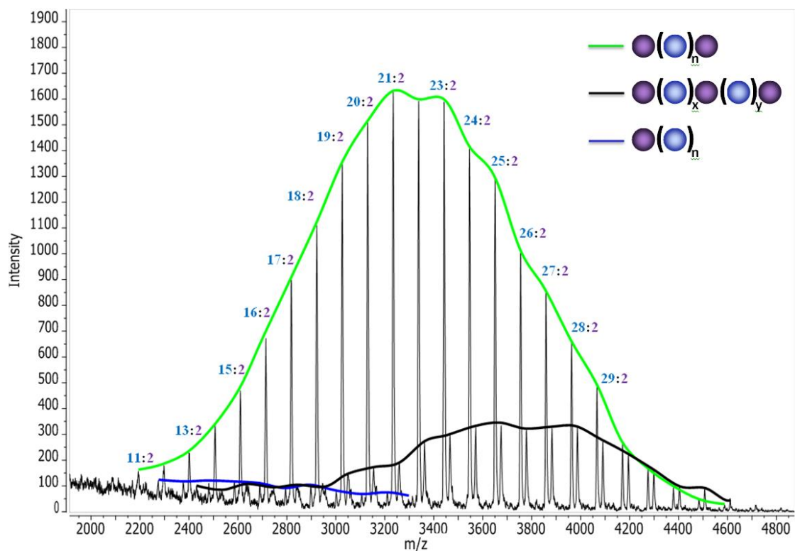
Figure 4.157: MALDI-ToF spectrum for anionic copolymerization (in benzene) of styrene (blue) and DPE-OSi, P(S-co-D OSi )-1b, (purple) (monomer molar feed ratio of Sty : DPE-OSi = 9.6 : 1.0) with TMEDA injected after 24 hours. The mole ratio of styrene : DPE-OSi for any given chain is labelled with styrene in blue and DPE-OSi in purple.
