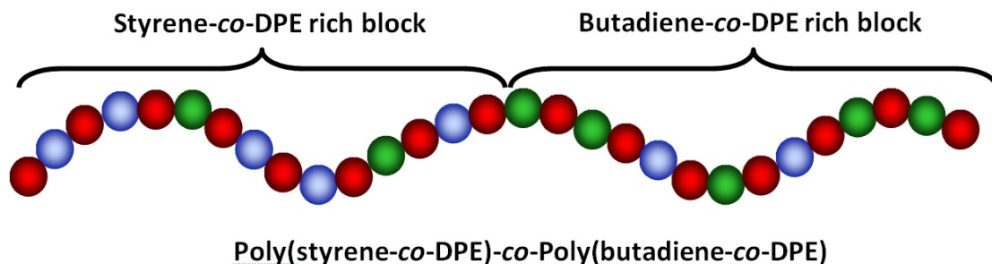
Figure 2.65: Schematic diagram to show the potential structure of a poly(styrene-co-DPE)-co-poly(butadiene-co-DPE) terpolymer when polymerized in THF with a molar feed ratio of styrene : DPE : butadiene = 1 : 2 : 1 where styrene is represented by blue balls, DPE by red balls and butadiene by green balls.
