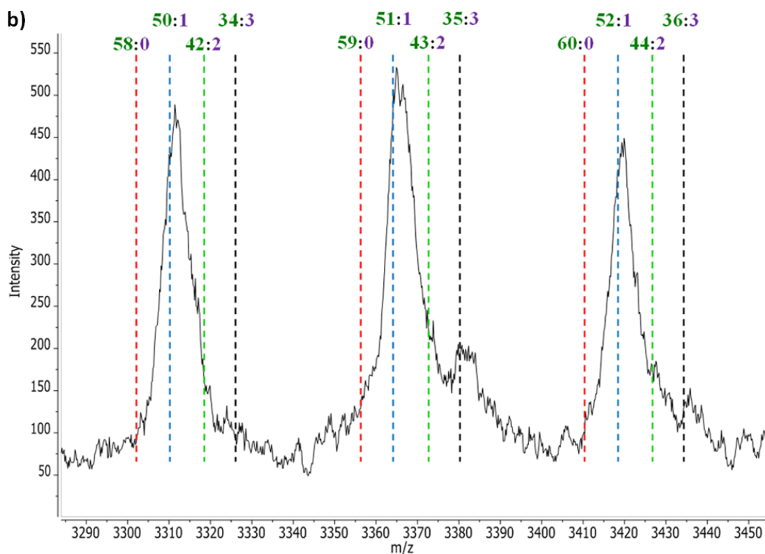
Figure 4.165: (a) MALDI-ToF mass spectrum for the anionic copolymerization (in benzene) of butadiene and DPE-OSi after 9 days, P(Bd-co-D OSi )-6b, with a molar feed ratio of Bd : DPE-OSi = 13.0 : 1.0 and (b) expansion showing the range m/z = 3290 - 3450 with red, blue and green dashed lines indicating where chains containing 0, 1 and 2 units of DPE-OSi respectively, would be expected to appear. The mole ratio of butadiene : DPE-OSi for any given chain is labelled with butadiene in green and DPE-OSi in purple.
