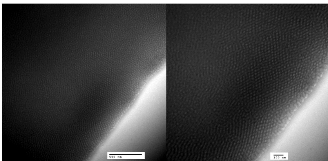
Figure 3.114: TEM images of the copolymer poly(styrene- co -DPE)- block -polybutadiene, PSD-PBd-6, with the butadiene blocks stained black with OsO 4 .
