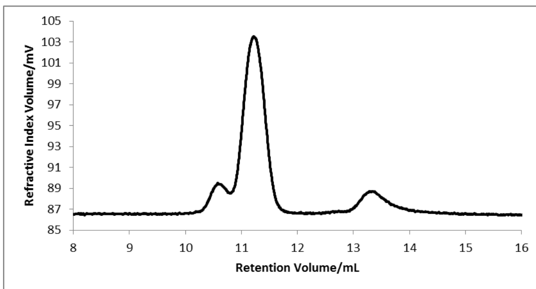
Figure 2.82: SEC chromatogram (refractive index) for the poly(styrene- co -DPE)- block -polybutadiene- block -poly(styrene- co -DPE) copolymer after the addition of the coupling agent, P(SD)-PBd-P(SD)-4c.
