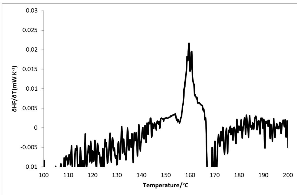
Figure 3.134: Derivative of Heat Flow (HF) vs Temperature (T) for the poly(butadiene- co -styrene- co -DPE) copolymer, PBdSD-10b.
