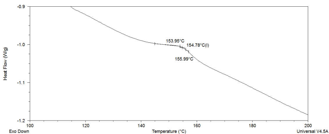
Figure 3.131: DSC thermogram obtained for the poly(butadiene- co -styrene- co -DPE) copolymer, PBdSD-10d, showing the T_g observed upon heating at 40 °C/min.
