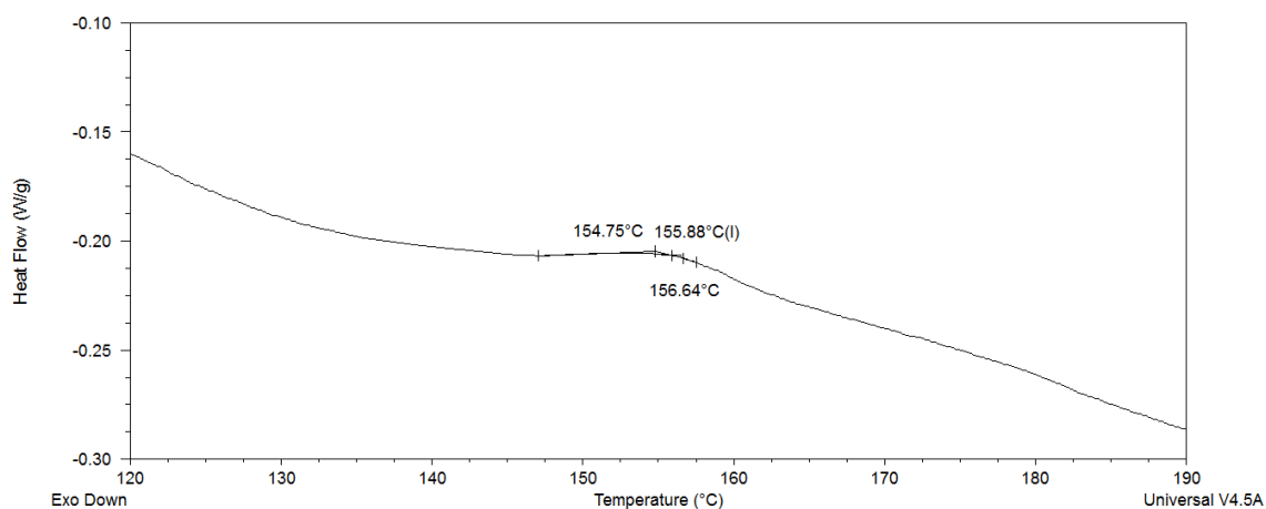
Figure 3.132: DSC thermogram obtained for the poly(butadiene- co -styrene- co -DPE) copolymer, PBdSD-10e, showing the T_g observed upon heating at 40 °C/min.
