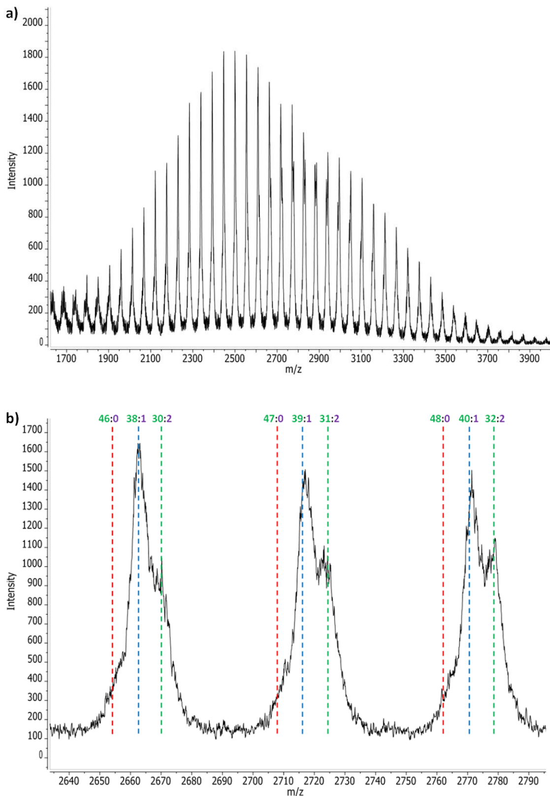
Figure 4.163: (a) MALDI-ToF spectrum of a sample (P(Bd-co-D OSi )-5c) collected after 151 hours (127 hours with TMEDA) of the anionic copolymerization of butadiene and DPE-OSi, in benzene with a molar feed ratio of Bd : DPE-OSi = 18.5 : 1.0 and (b) expansion showing the range m/z = 2640 – 2790 with red, blue and green dashed lines indicating where chains containing 0, 1 and 2 units of DPE-OSi respectively, would be expected to appear. The mole ratio of butadiene : DPE-OSi for any given chain is labelled with butadiene in green and DPE-OSi in purple.
