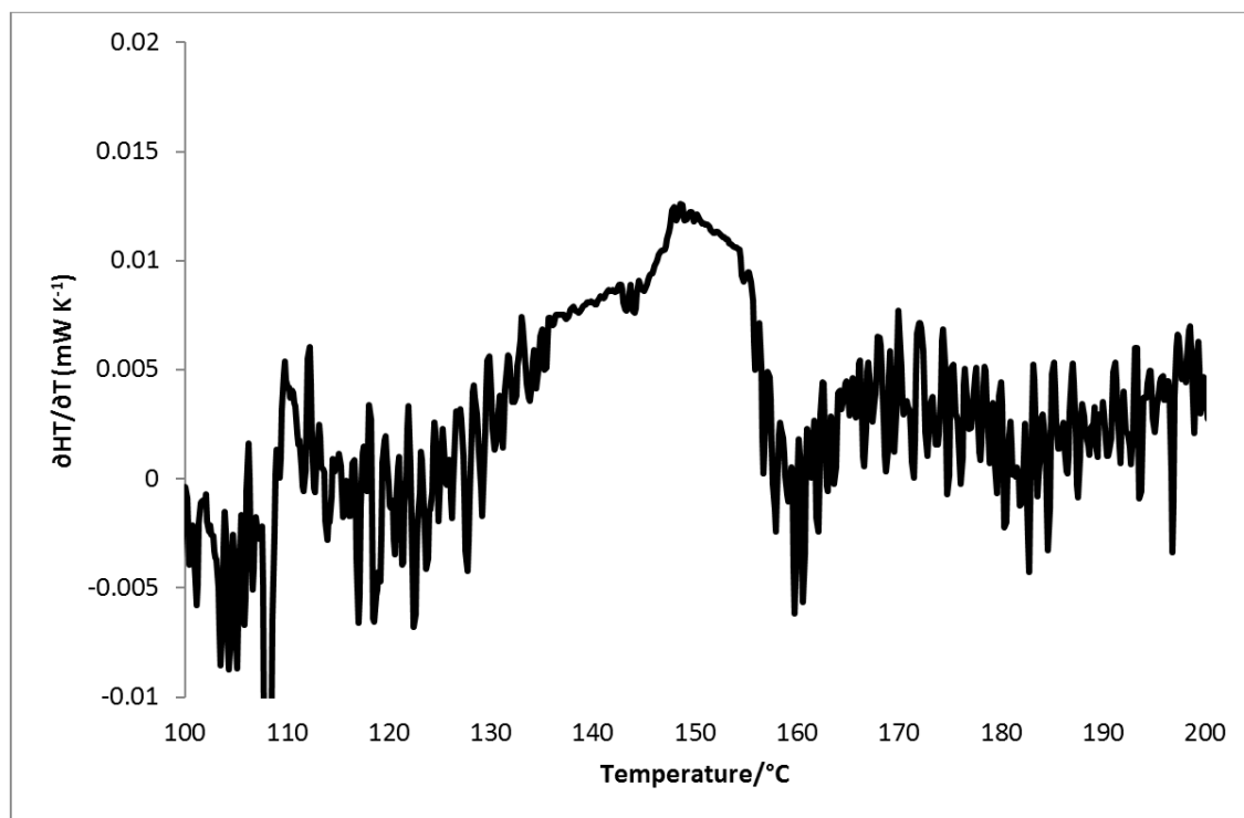
Figure 3.137: Derivative of Heat Flow (HF) vs Temperature (T) for the poly(butadiene-co-styrene-co-DPE) copolymer, PBdSD-10e.
