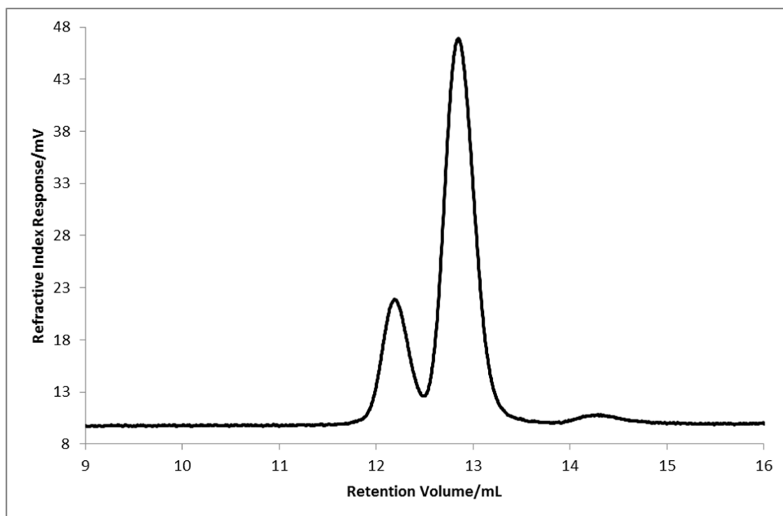
Figure 3.124: SEC chromatogram (refractive index) for the commercial copolymer polystyrene- block -polybutadiene- block -polystyrene, PS-PBd-PS.
