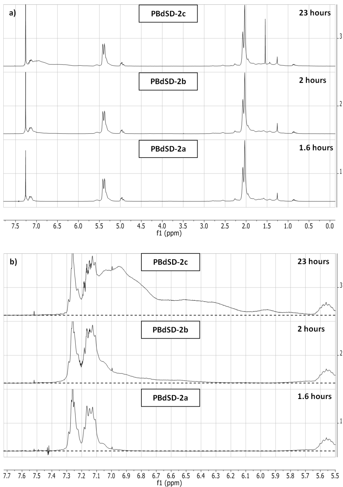
Figure 2.48: (a) ^1\text{H} NMR spectrum (in \text{CDCl}_3 ) of Poly(butadiene- co -styrene- co -DPE) copolymers, PBdSD-2a-c, synthesized in benzene with a molar feed ratio of 1.00 : 0.58 : 3.28 styrene : DPE : butadiene and (b) expansion of the aromatic region (5.6 – 7.8 ppm) with the baseline indicated by a dotted line.
