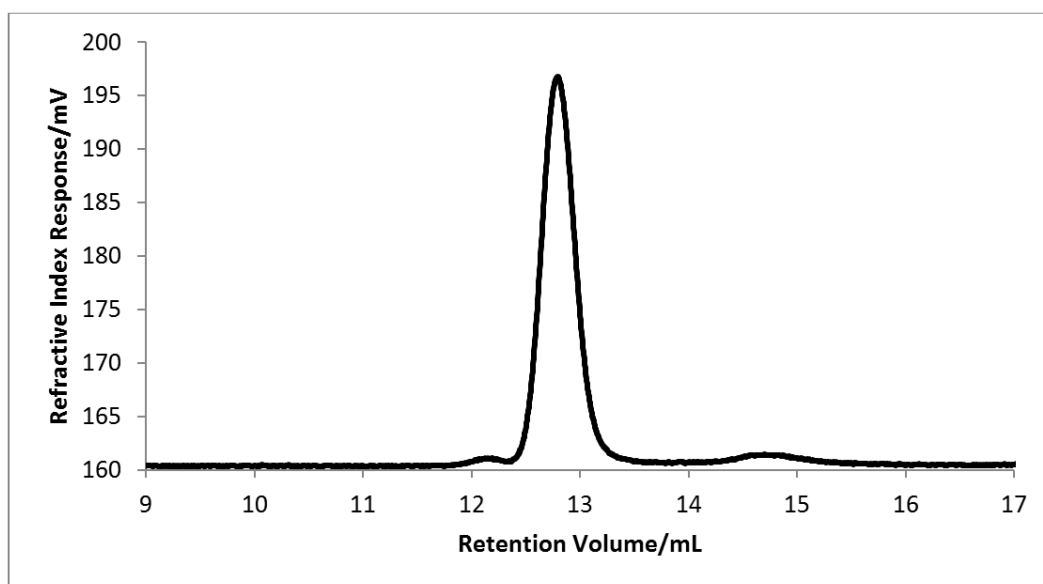
Figure 2.41: SEC chromatogram (refractive index) for poly(styrene- co -DPE)- block -polybutadiene copolymer, P(SD)-PBd-7.
