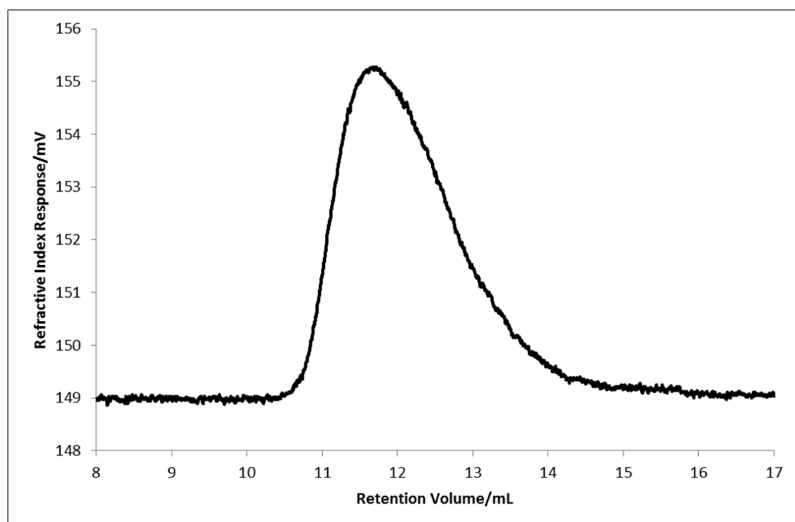
Figure 2.86: SEC chromatogram (refractive index) for the poly(butadiene- co -DPE) copolymer, PBdD-4b.
