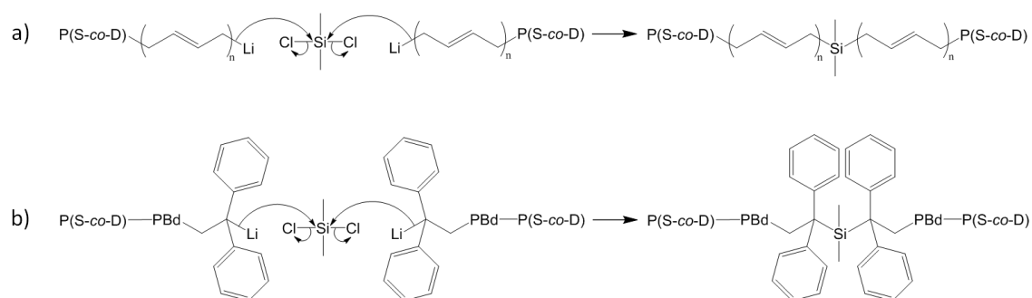
Figure 2.80: Reaction scheme showing the coupling of (a) poly(styrene- co -DPE)- block -polybutadienyllithium and (b) 1,1-diphenylethyllithium end-capped poly(styrene- co -DPE)- block -polybutadiene with DCDMS. Note: it is unlikely that the reaction of the two polymeric chains with DCDMS will happen simultaneously as depicted.
