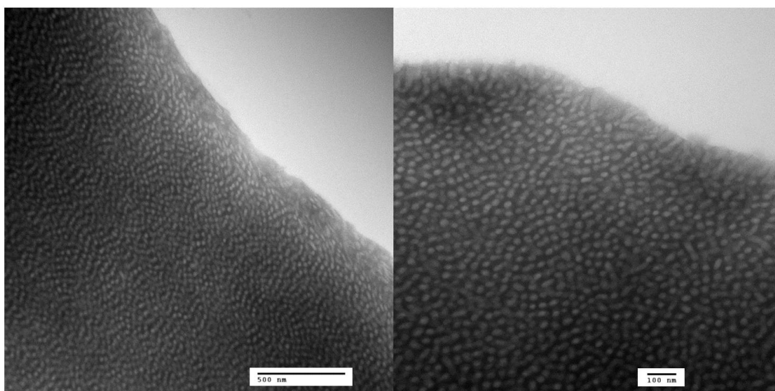
Figure 3.123: TEM images of a tapered poly(styrene- co -DPE)- block -polybutadiene- block -poly(styrene- co -DPE), P(BdSD) 2 -I, synthesized by the simultaneous copolymerization of butadiene, styrene and DPE with a difunctional initiator, with the butadiene blocks stained black with OsO 4 .
