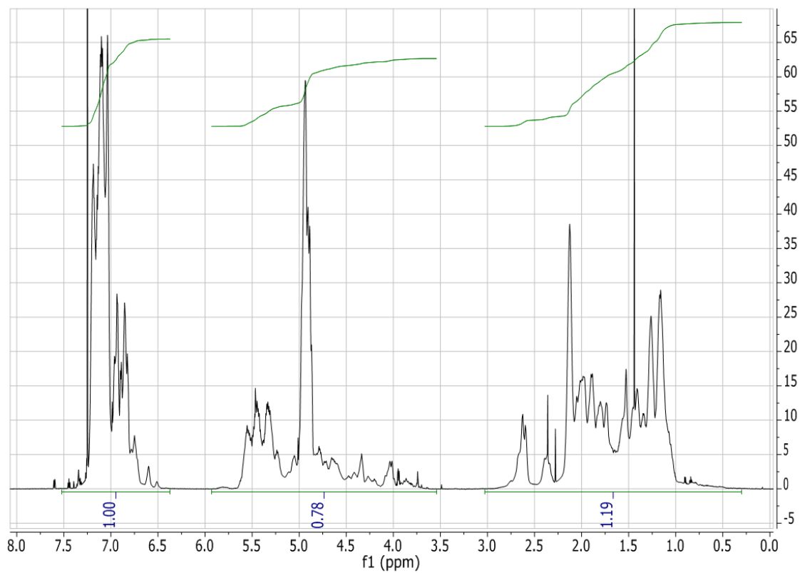
Figure 2.97: 1 H NMR spectrum (in CDCl 3 ) for the poly(butadiene- co -DPE), PBdD-8, synthesized in THF with a molar feed ratio of 1.00 : 2.85 DPE : butadiene and terminated after 15.2 hours at 0 °C.
