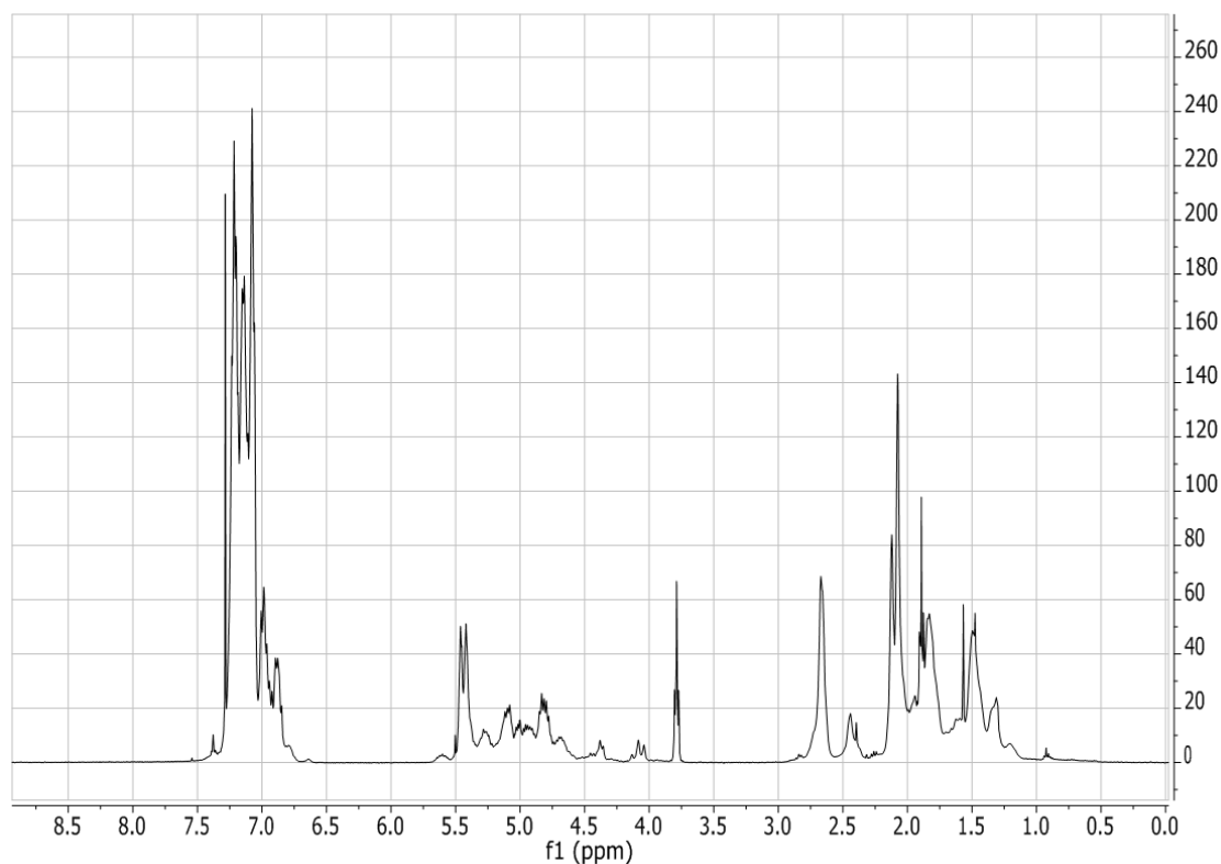
Figure 2.91: ^1\text{H} NMR spectrum (in \text{CDCl}_3 ) for the poly(butadiene- co -DPE), PBdD-6b, synthesized in toluene with THF added after 57 minutes at 40^\circ\text{C} and with a molar feed ratio of 1.00 : 0.96 DPE : butadiene.
