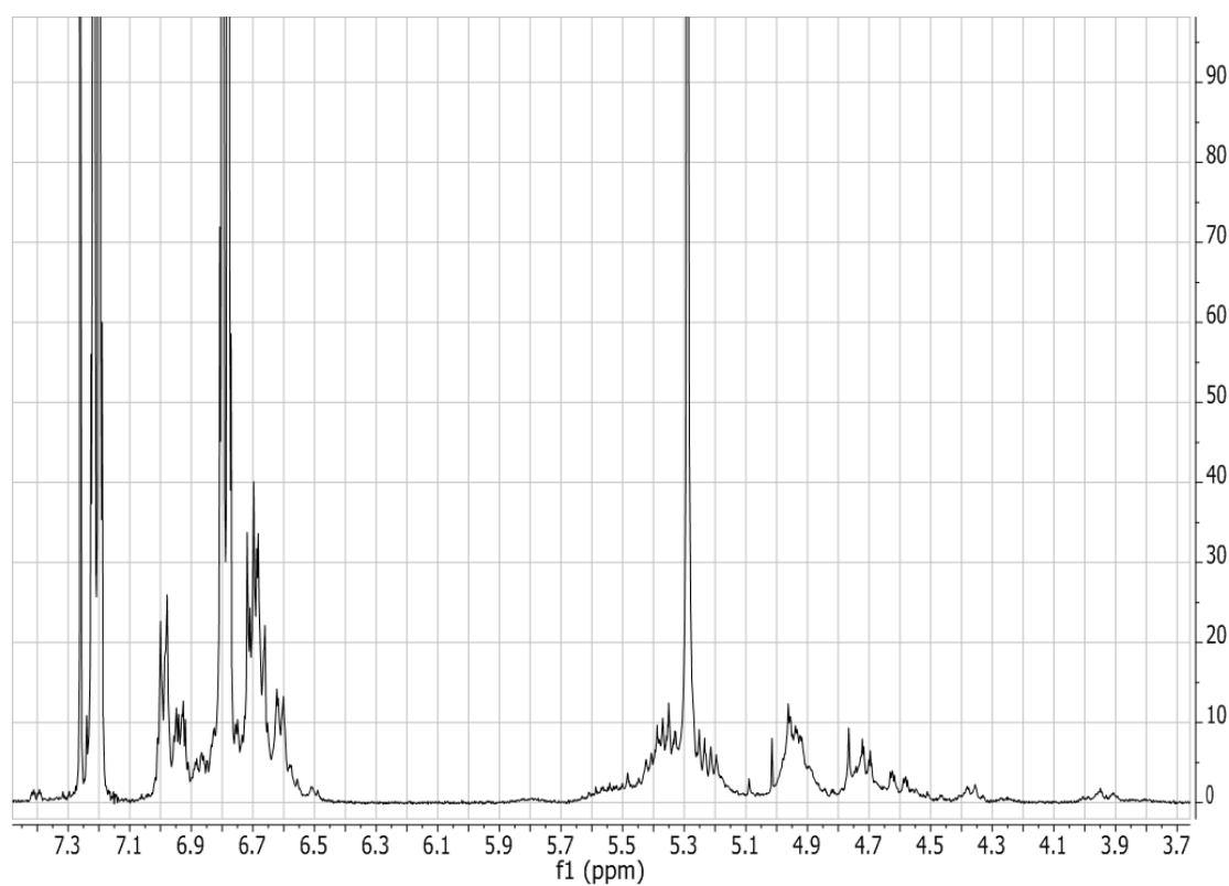
Figure 4.150: ^1\text{H} NMR spectrum (in \text{CDCl}_3 ) of poly(butadiene- co -DPE-OSi), P(Bd- co -D OSi )-1, synthesized in THF with a molar feed ratio 1.0 : 1.0 butadiene : DPE-OSi and expanded over the region 3.7 – 7.3 ppm.
