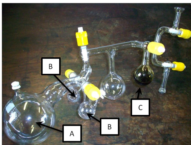
Figure 5.167: Reaction vessel used for polymerizations, showing (A) main reaction vessel (B) side flasks and (C) living polystyrene cleaning solution.
