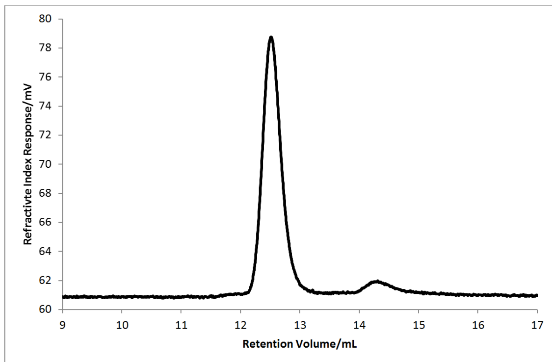
Figure 3.119: SEC chromatogram (refractive index) for the copolymer poly(styrene- co -DPE)- block -polybutadiene, PSD-PBd-8.
