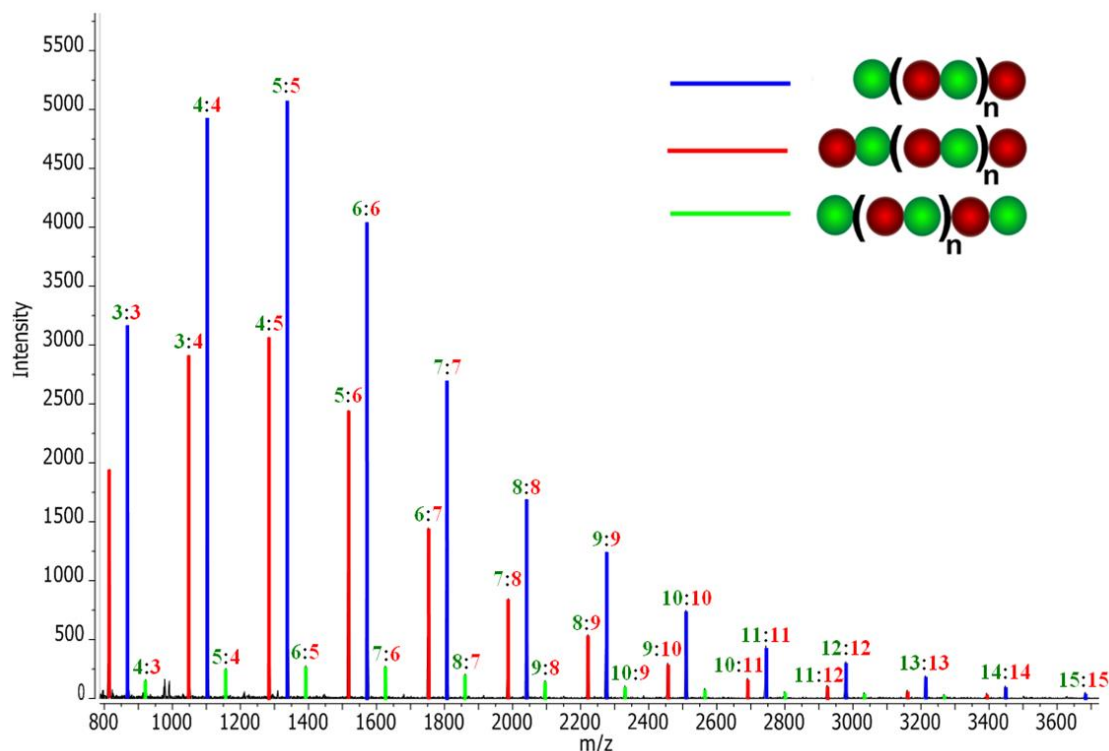
Figure 2.29: MALDI-ToF mass spectrum for the copolymer PBdD-2 prepared by the anionic copolymerization (in THF) of butadiene and DPE (monomer molar feed ratio of butadiene : DPE = 0.97 : 1.00). The mole ratio of butadiene : DPE for any given chain is labelled with butadiene in green and DPE in red.
