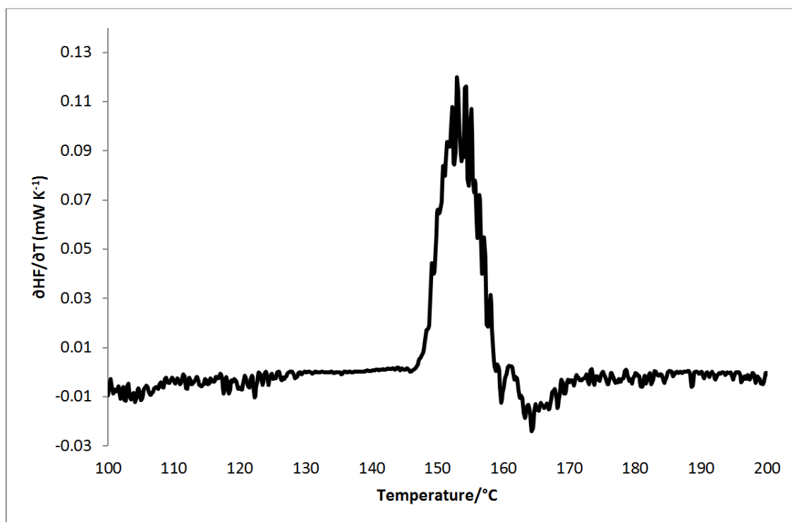
Figure 3.133: Derivative of Heat Flow (HF) vs Temperature (T) for the poly(butadiene- co -styrene- co -DPE) copolymer, PBdSD-10a.
