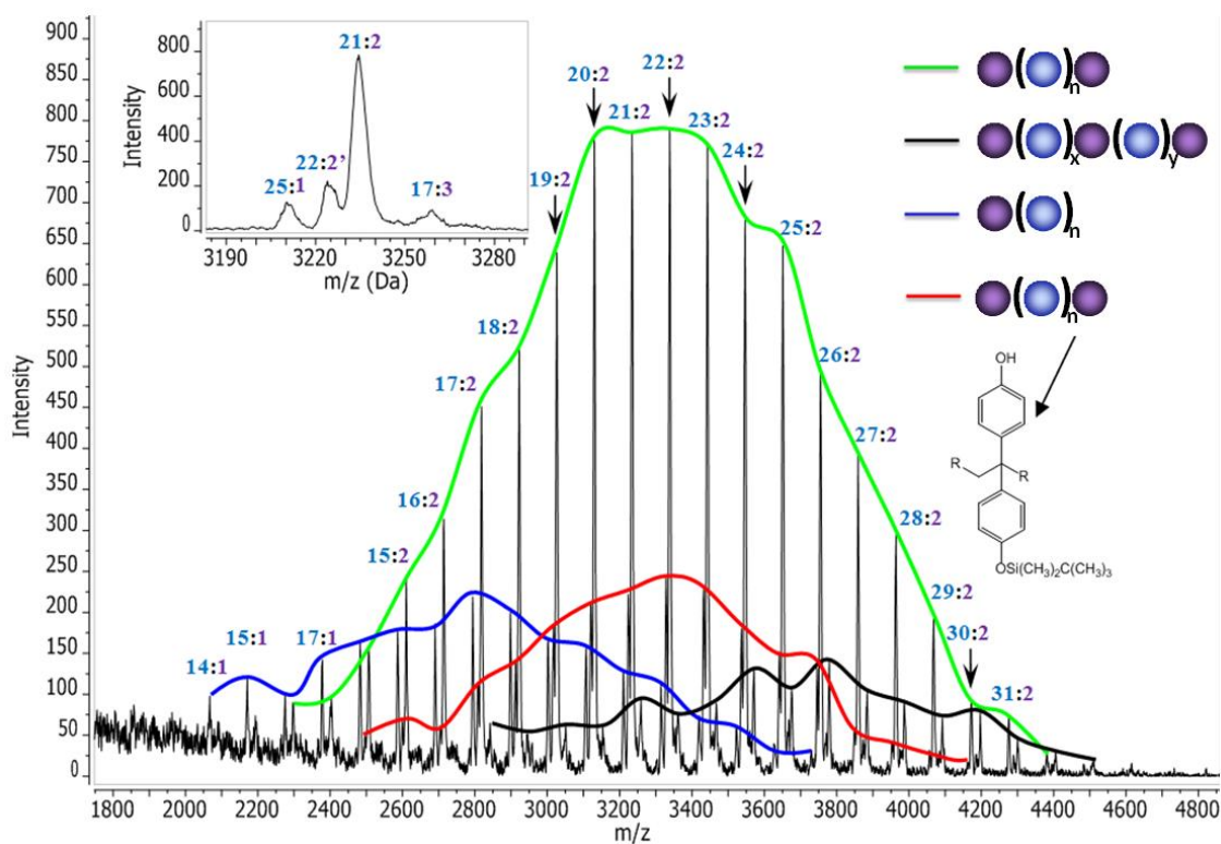
Figure 4.156: MALDI-ToF mass spectrum for the anionic copolymerization (in benzene) of styrene (blue) and DPE-OSi (purple), P(S-co-D OSi )-1a, (monomer molar feed ratio of Sty : DPE-OSi = 9.6 : 1.0). The mole ratio of styrene : DPE-OSi for any given chain is labelled with styrene in blue and DPE-OSi in purple.
