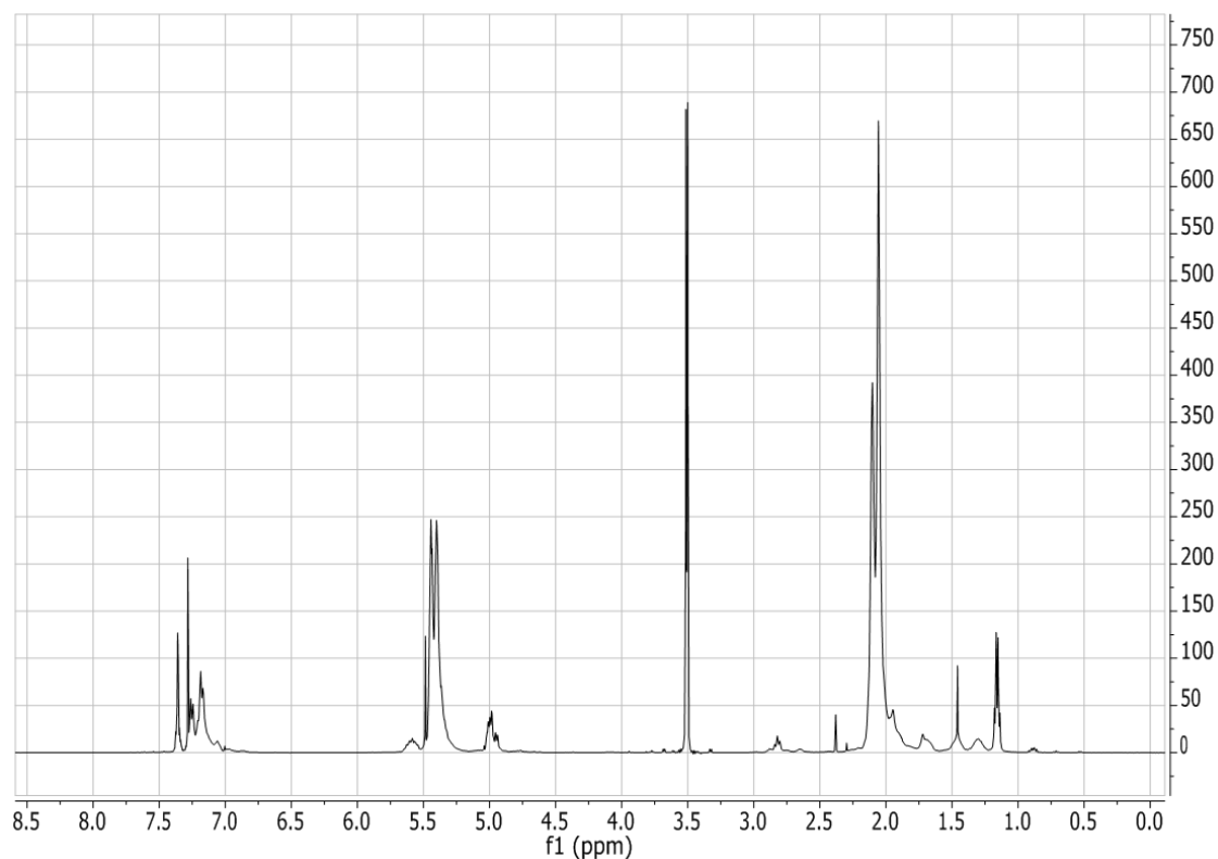
Figure 2.88: ^1\text{H} NMR spectrum (in \text{CDCl}_3 ) for the poly(butadiene-co-DPE), PBdD-5b, synthesized in toluene with THF added after 3.3 hours at 40^\circ\text{C} and with a molar feed ratio of 1.00 : 0.96 DPE : butadiene.
