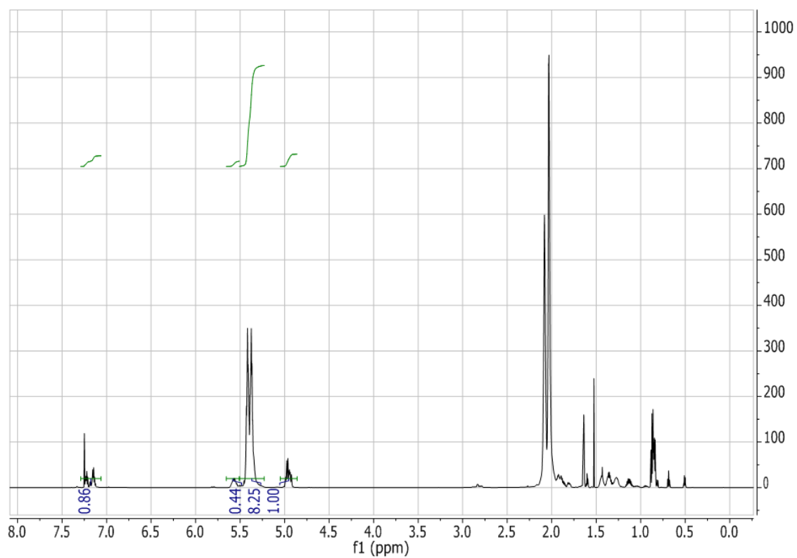
Figure 2.32: ^1\text{H} NMR spectrum (in \text{CDCl}_3 ) of Poly(butadiene-co-DPE), PBdD-3a, synthesized in benzene with a molar feed ratio of 3.26 : 1.00 butadiene : DPE and terminated after 1.9 hours.
