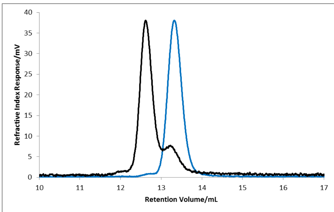
Figure 2.93: Overlay of the SEC chromatograms (refractive index) for the poly(butadiene-co-DPE) copolymers, PBdD-7a (blue) and PBdD-7b (black).
