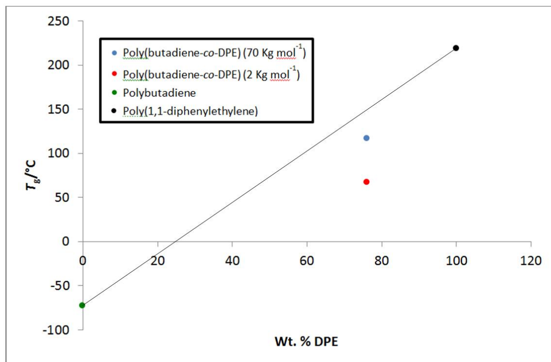
Figure 3.106: Graph showing the correlation between T_g and wt. % DPE for poly(butadiene-co-DPE) copolymers.
