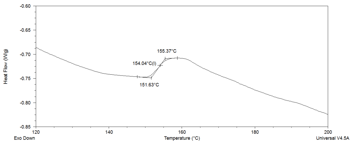
Figure 3.130: DSC thermogram obtained for the poly(butadiene- co -styrene- co -DPE) copolymer, PBdSD-10c, showing the T_g observed upon heating at 40 °C/min.
