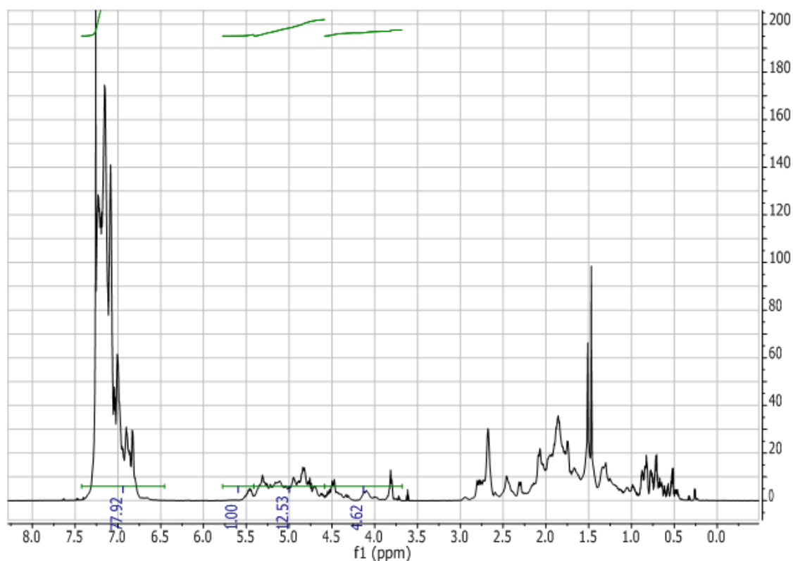
Figure 2.24: ^1\text{H} NMR spectrum (in \text{CDCl}_3 ) of poly(butadiene- co -DPE), PBdD-2, synthesized in THF with a molar feed ratio of 0.97 : 1.00 butadiene : DPE.
