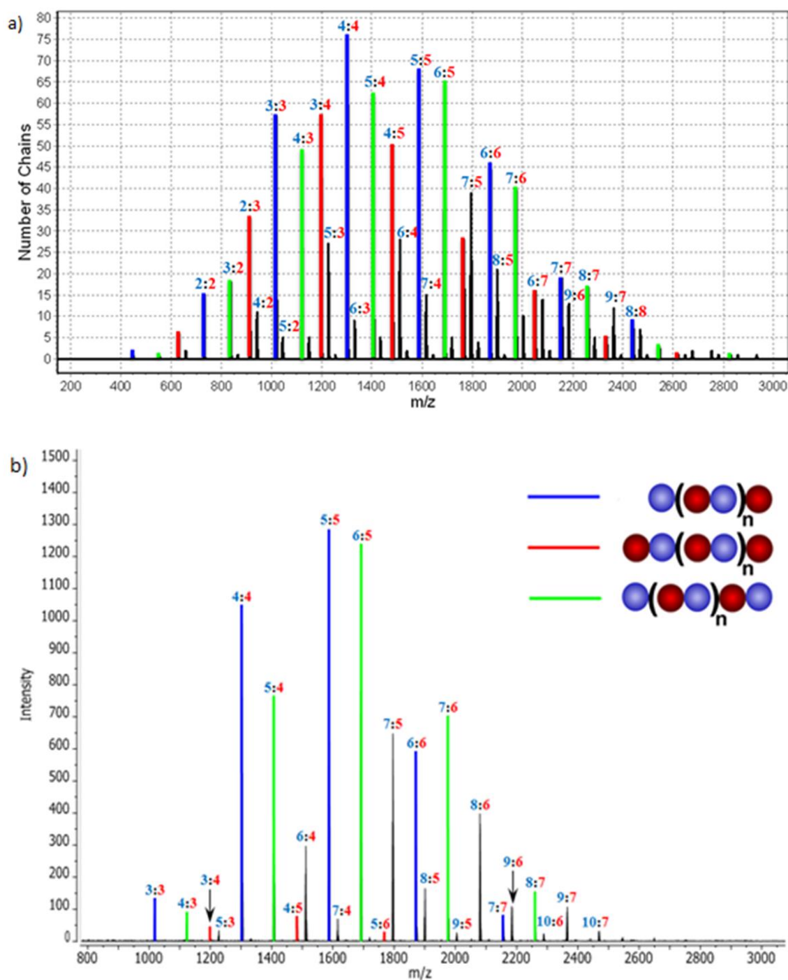
Figure 2.36: (a) Simulated versus (b) experimental MADLI-ToF data for the copolymer PSD-5 prepared by the anionic copolymerization (in benzene) of styrene and DPE (monomer molar feed ratio of styrene : DPE = 0.97 : 1.00). The mole ratio of styrene : DPE for any given chain is labelled with styrene in blue and DPE in red.
