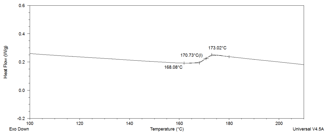
Figure 3.101: DSC thermogram obtained for the poly(styrene- co -DPE) copolymer, PSD-3b, heated at a rate of 20 °C/min.
