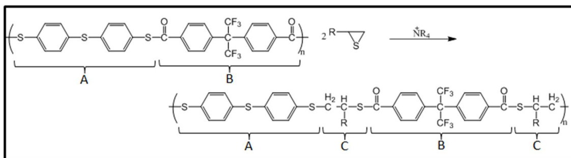
Figure 1.10: Synthetic scheme showing the synthesis of a sequence controlled copolymer by the monomer insertion of an ethylene sulfide derivative. 21
