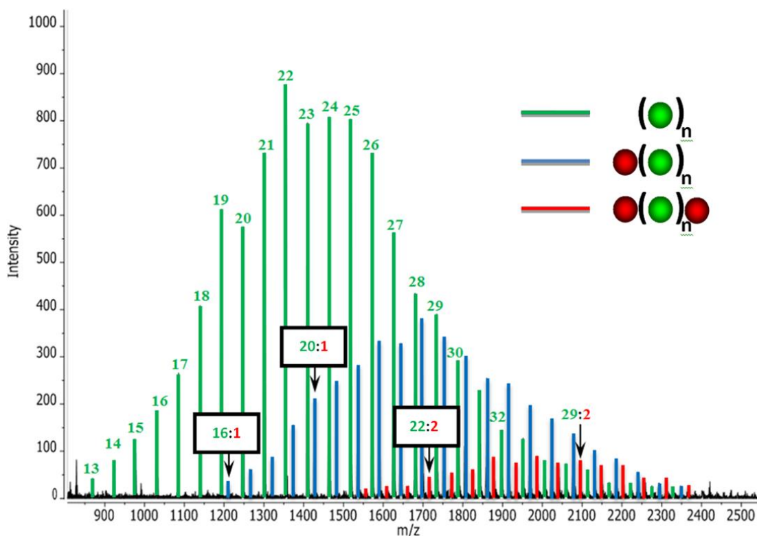
Figure 2.35: MALDI-ToF mass spectrum for the copolymer PBdD-3b prepared by the anionic copolymerization (in benzene) of butadiene and DPE (monomer molar feed ratio of butadiene : DPE = 3.26 : 1.00) after 19.7 hours. The mole ratio of butadiene : DPE for any given chain is labelled with butadiene in green and DPE in red.
