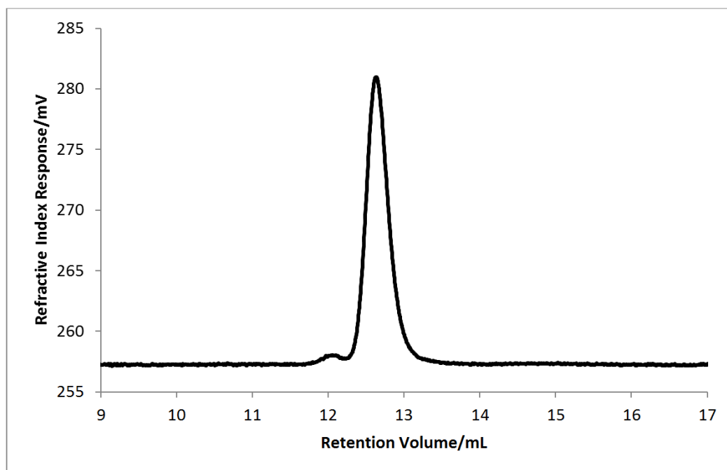
Figure 2.56: SEC chromatogram (refractive index) for poly(butadiene- co -styrene- co -DPE) copolymer, PBdSD-6.
