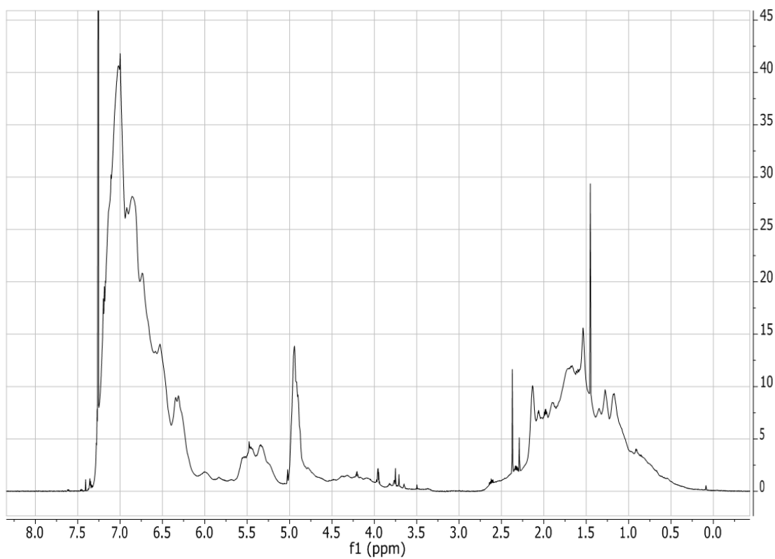
Figure 2.62: ^1\text{H} NMR spectrum (in \text{CDCl}_3 ) of Poly(butadiene-co-styrene-co-DPE), PBdSD-12a, synthesized in THF with a molar feed ratio of 1.00 : 1.07 : 1.02 styrene : DPE : butadiene.
