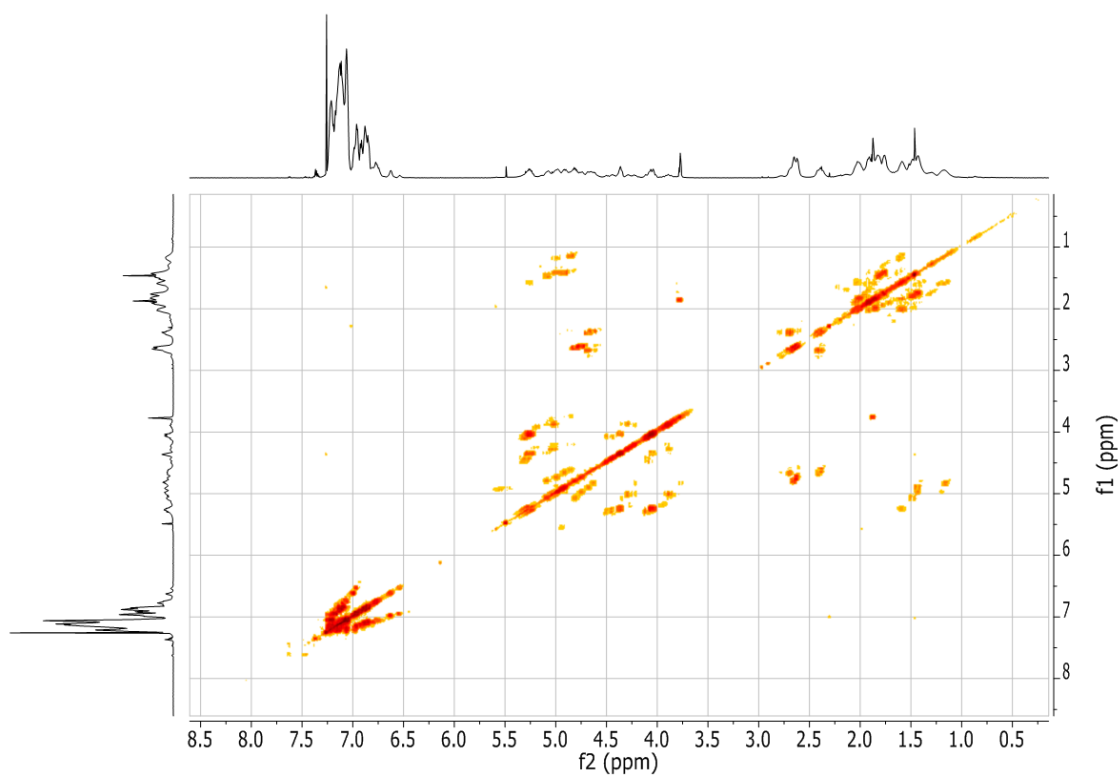
Figure 2.22: COSY NMR spectrum (in \text{CDCl}_3 ) of poly(butadiene-co-DPE), PBdD-1.
