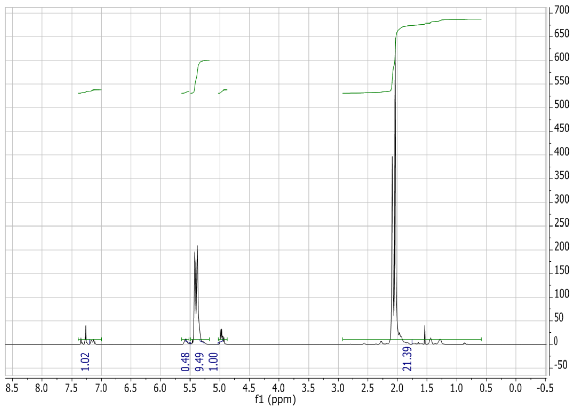
Figure 2.46: ^1\text{H} NMR spectrum (in \text{CDCl}_3 ) of Poly(butadiene- co -styrene- co -DPE), PBdSD-1a, synthesized in benzene with a molar feed ratio of 1.00 : 0.67 : 5.37 styrene : DPE : butadiene.
