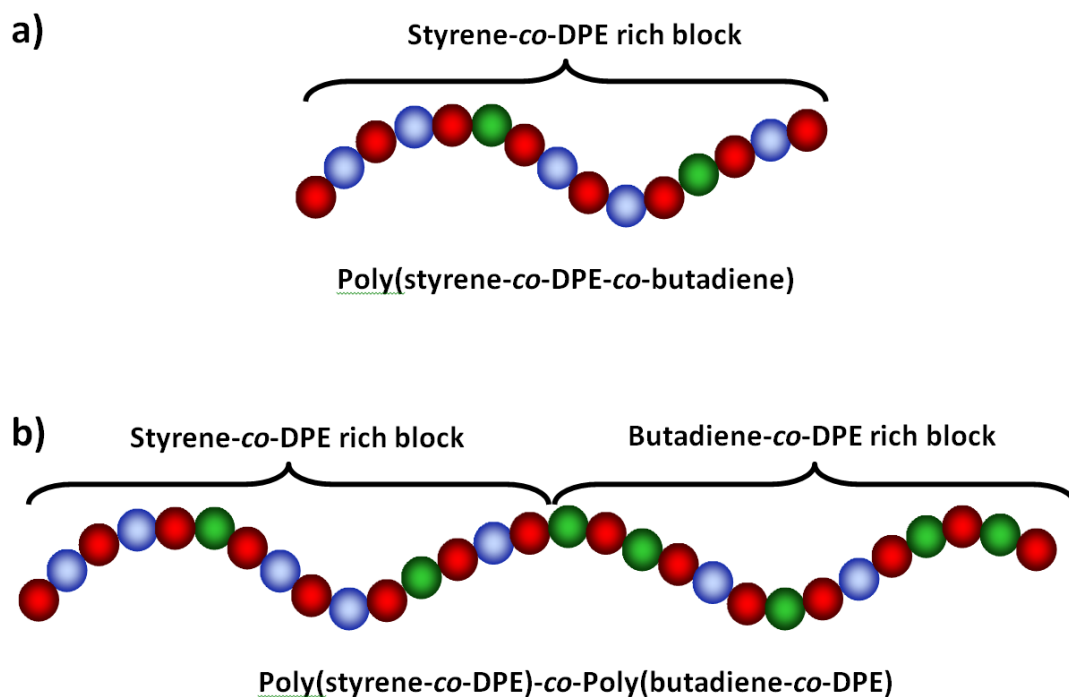
Figure 3.126: Schematic diagram to show the potential structure of (a) poly(styrene- co -DPE- co -butadiene) collected during the early stages of the reaction and (b) the final poly(styrene- co -DPE)- co -poly(butadiene- co -DPE) terpolymer when butadiene (green balls), styrene (blue balls) and DPE (red balls) are copolymerized in THF with a molar feed ratio of styrene : DPE : butadiene = 1 : 2 : 1.
