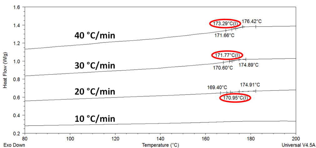
Figure 3.112: DSC thermogram obtained for the poly(butadiene-co-styrene-co-DPE) copolymer, PBdSD-4d, showing the T_g observed upon heating at 10 °C/min; 20 °C/min; 30 °C/min and 40 °C/min.
