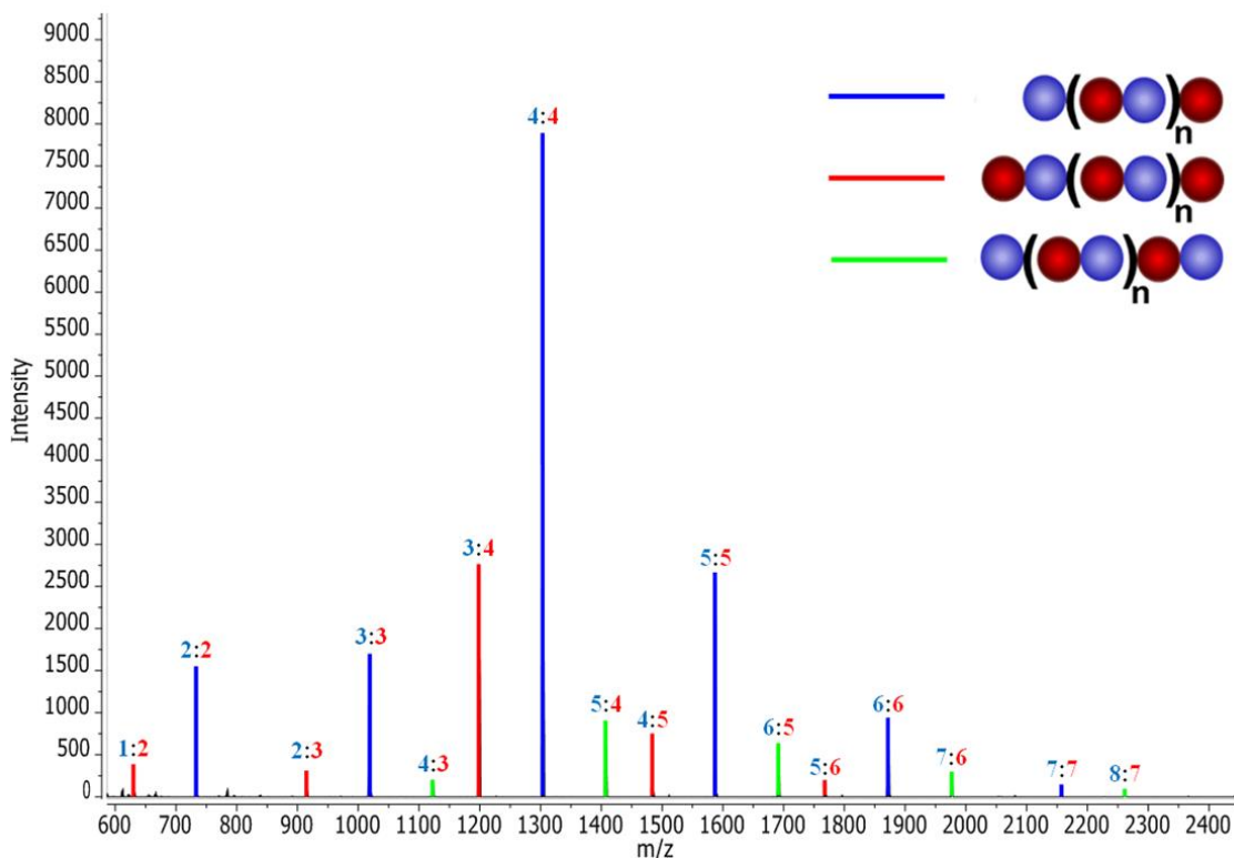
Figure 2.18: MALDI-ToF mass spectrum for the copolymer PSD-10 prepared by the anionic copolymerization (in THF) of styrene and DPE (monomer molar feed ratio of styrene : DPE = 0.95 : 1.00). The mole ratio of styrene : DPE for any given chain is labelled with styrene in blue and DPE in red.
