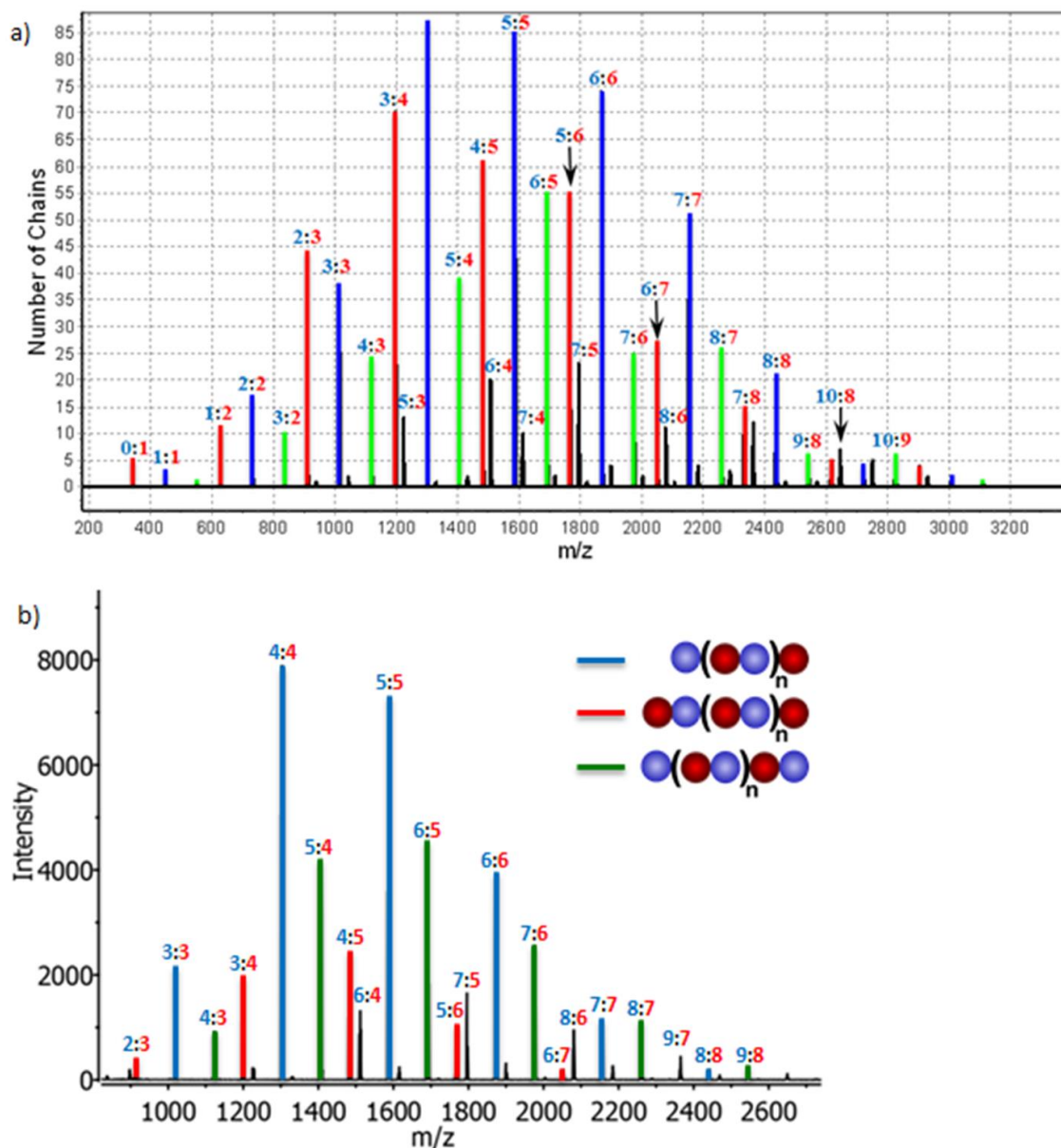
Figure 2.37: (a) Simulated versus (b) experimental MADLI-ToF data for the copolymer PSD-6 prepared by the anionic copolymerization (in benzene) of styrene and DPE (monomer molar feed ratio of styrene : DPE = 0.65 : 1.00). The mole ratio of styrene : DPE for any given chain is labelled with styrene in blue and DPE in red.
