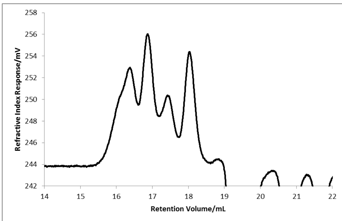
Figure 4.153: SEC trace for poly(butadiene-co-DPE-OSi) copolymer, P(Bd-co-DOSi)-4, showing the refractive index response.
