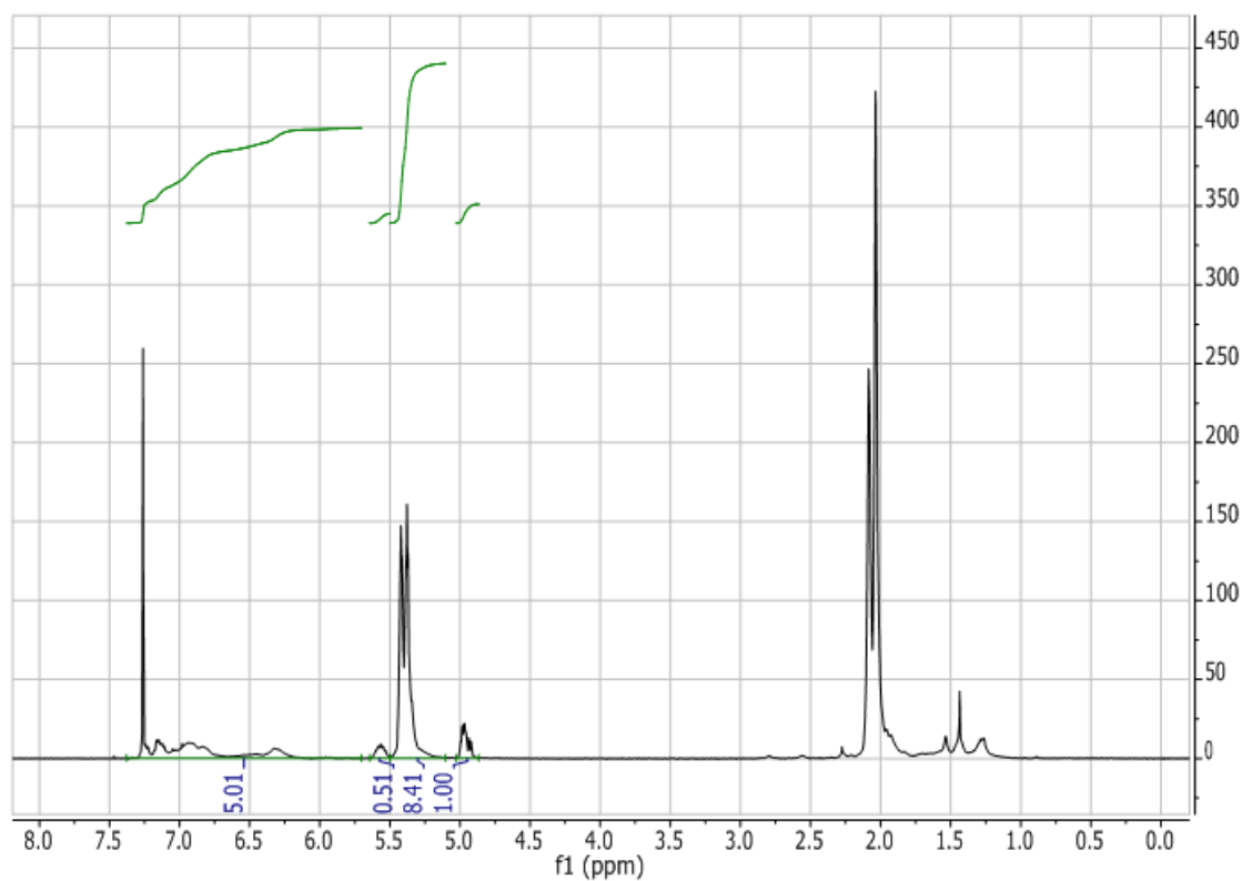
Figure 2.76: 1 H NMR spectrum (in CDCl 3 ) for the poly(styrene- co -DPE)- co -polybutadiene- co -poly(styrene- co -DPE) copolymer, P(BdSD) 2 -I, synthesized in benzene with a molar feed ratio of 1.00 : 1.60 : 12.39 styrene : DPE : butadiene.
