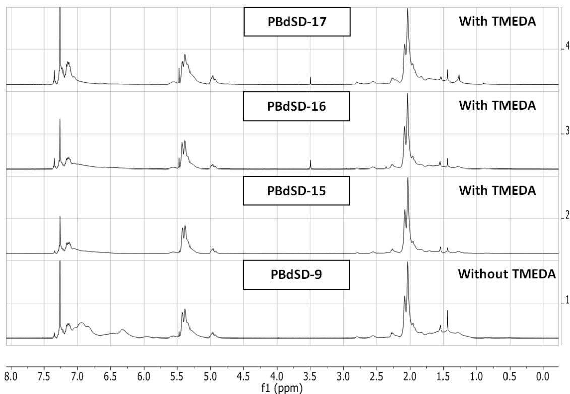
Figure 2.72: ^1\text{H} NMR spectra (in \text{CDCl}_3 ) of poly(butadiene- co -styrene- co -DPE) copolymers, PBdSD-9 (without TMEDA); PBdSD-15 (TMEDA injected when the reaction was pale yellow); PBdSD-16 (TMEDA injected when the reaction was dark yellow) and PBdSD-17 (TMEDA injected when the reaction was red).
