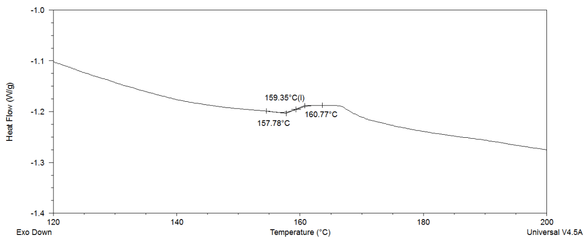
Figure 3.129: DSC thermogram obtained for the poly(butadiene-co-styrene-co-DPE) copolymer, PBdSD-10b, showing the T_g observed upon heating at 40 °C/min.
