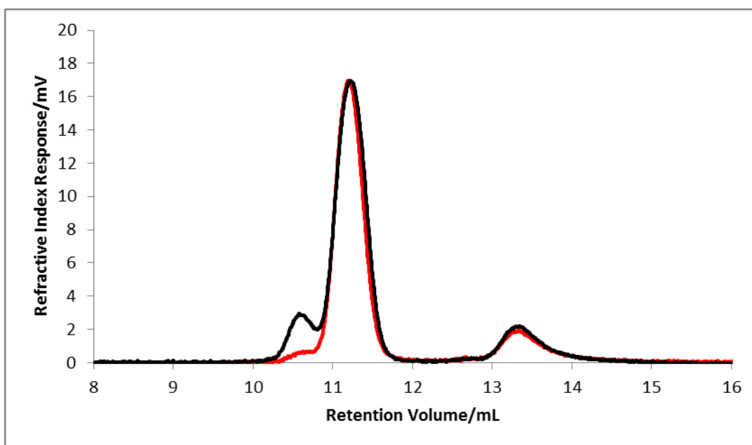
Figure 2.83: SEC chromatogram (refractive index) showing the poly(styrene- co -DPE)- block -polybutadiene- block -poly(styrene- co -DPE) copolymer after the addition of the coupling agent, P(SD)-PBd-P(SD)-4c (black) and poly(styrene- co -DPE)- block -polybutadiene copolymer prior to the addition of the coupling agent, P(SD)-b-PBd-b-P(SD)-4b (red).
