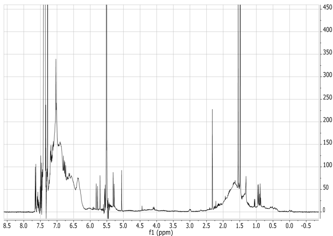
Figure 2.67: ^1\text{H} NMR spectrum (in \text{CDCl}_3 ) of Poly(butadiene-co-styrene-co-DPE), product of reaction PBdSD-14, synthesized in THF with a molar feed ratio of 1.00 : 1.94 : 0.94 styrene : DPE : butadiene.
