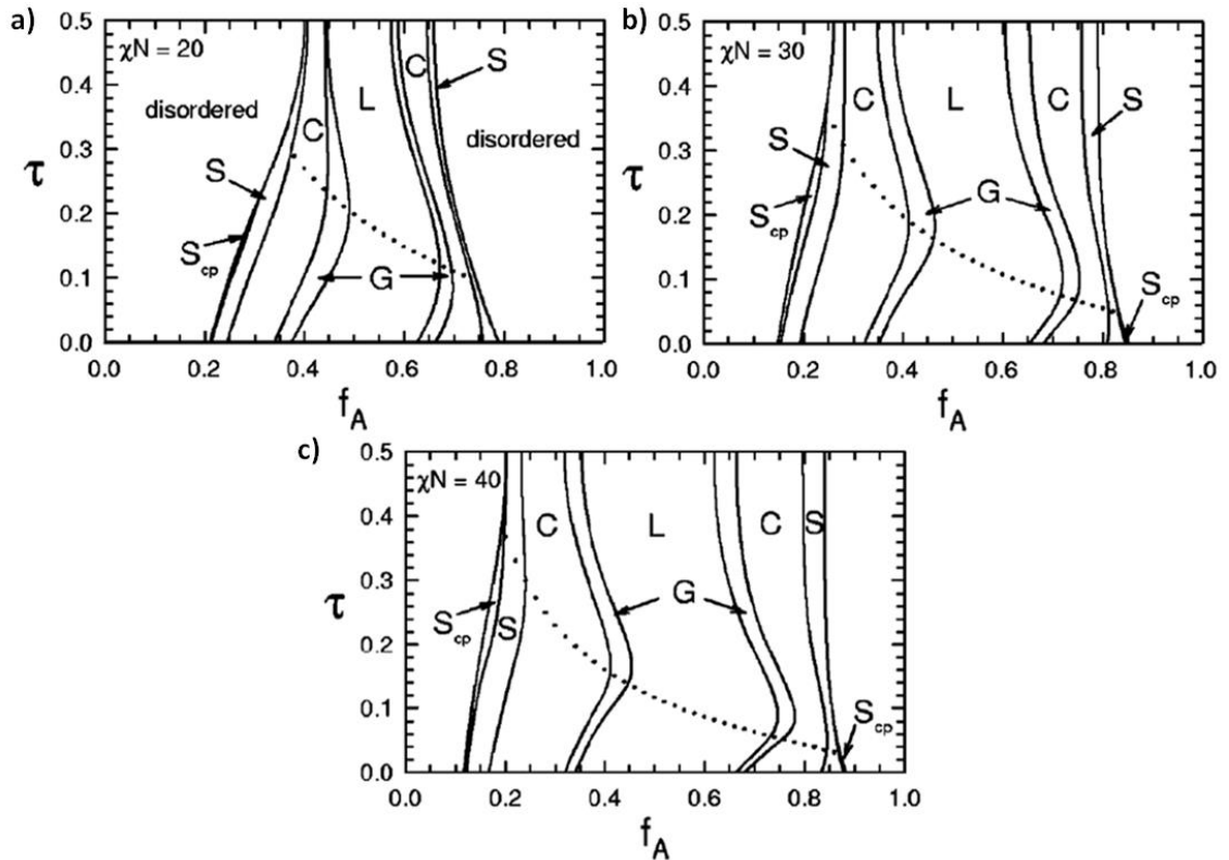
Figure 3.121: Phase diagrams for asymmetric ABA tri-block copolymers spanning the di-block ( \tau = 0.0 ) and symmetric tri-block ( \tau = 0.5 ) limits for (a) \chi N = 20 , (b) \chi N = 30 and (c) \chi N = 40 . Reprinted with permission from Matsen, M. W., The Journal of Chemical Physics , Vol. 113/13, Page 5539-5544, 2000. Copyright 2000, American Institute of Physics. 16
