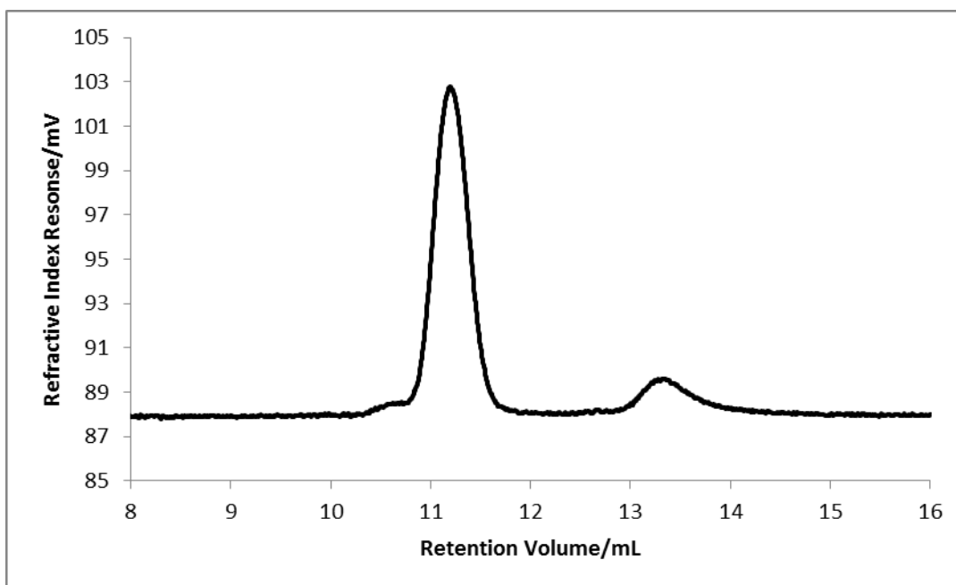
Figure 2.81: SEC chromatogram (refractive index) for the poly(styrene- co -DPE)- block -polybutadiene copolymer prior to the addition of the coupling agent, P(SD)-PBd-P(SD)-4b.
