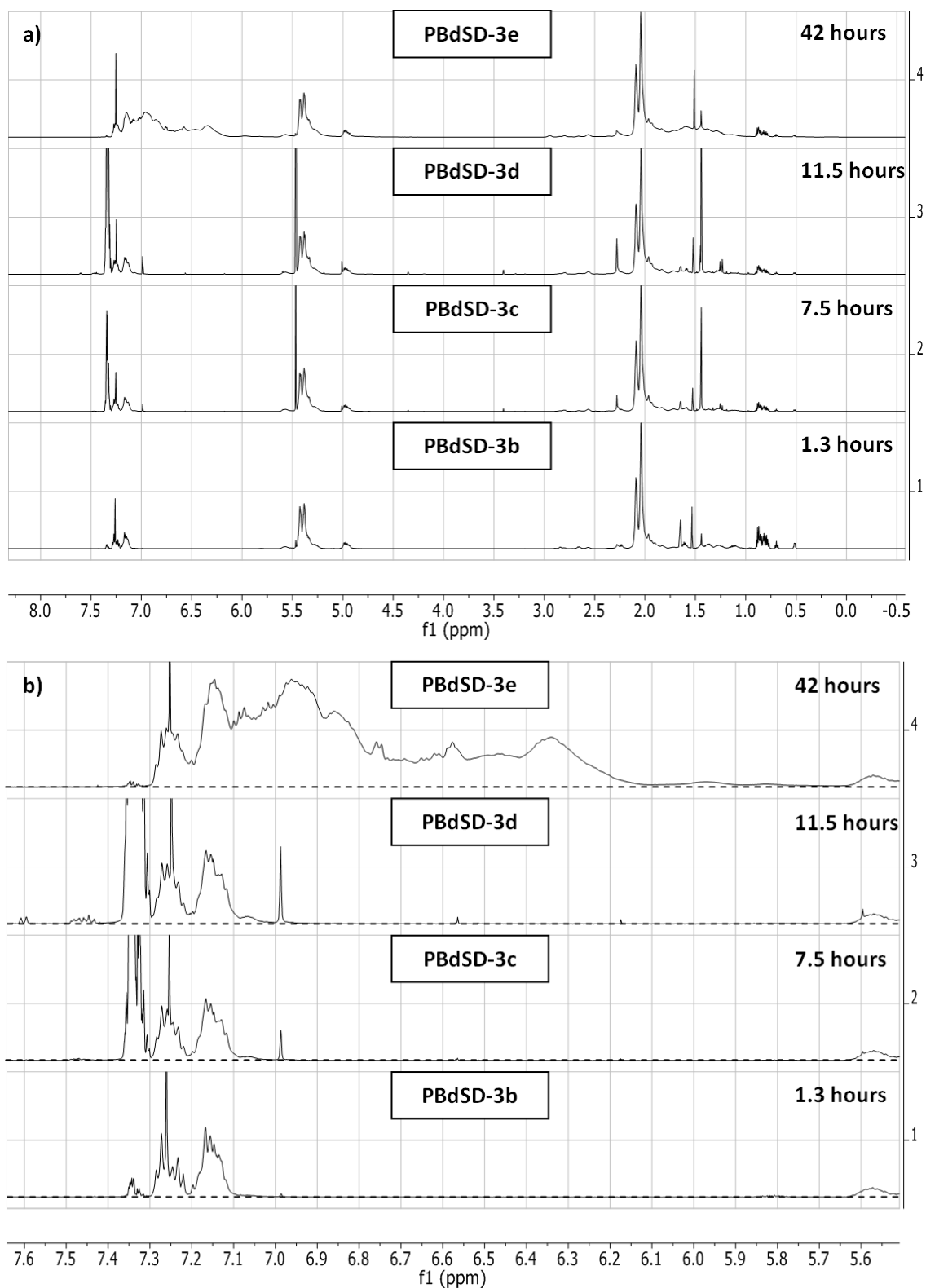
Figure 2.50: (a) 1 H NMR spectrum (in CDCl 3 ) of Poly(butadiene-co-styrene-co-DPE) copolymers, PBdSD-3b-e, synthesized in benzene with a molar feed ratio of 1.00 : 1.55 : 1.99 styrene : DPE : butadiene and (b) expansion of the aromatic region (5.6 – 7.6 ppm) with the baseline indicated by a dotted line.
