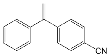
Figure 4.140: Structure of 4-cyanodiphenylethylene (DPE-CN).
