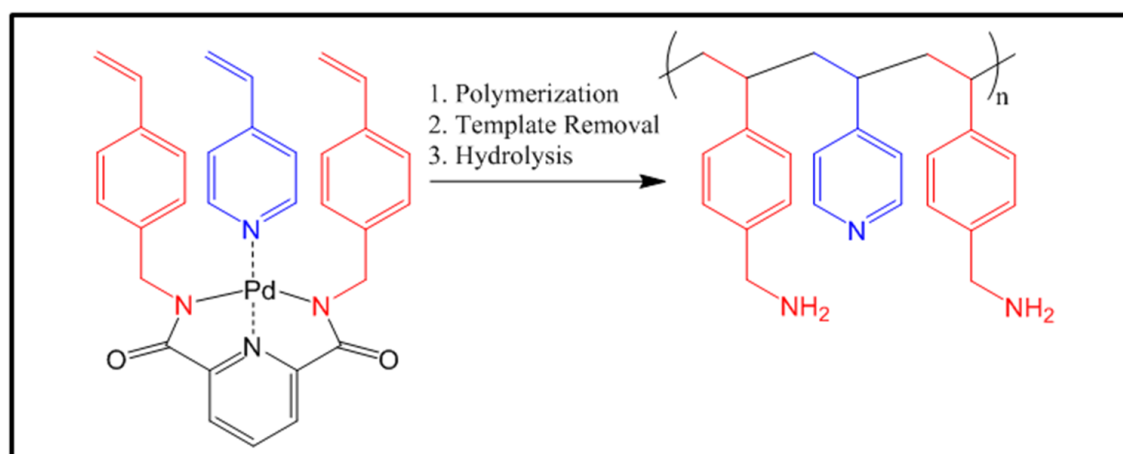
Figure 1.12: Synthetic scheme showing a sequence controlled living radical polymerization using a three-monomer template. 24
