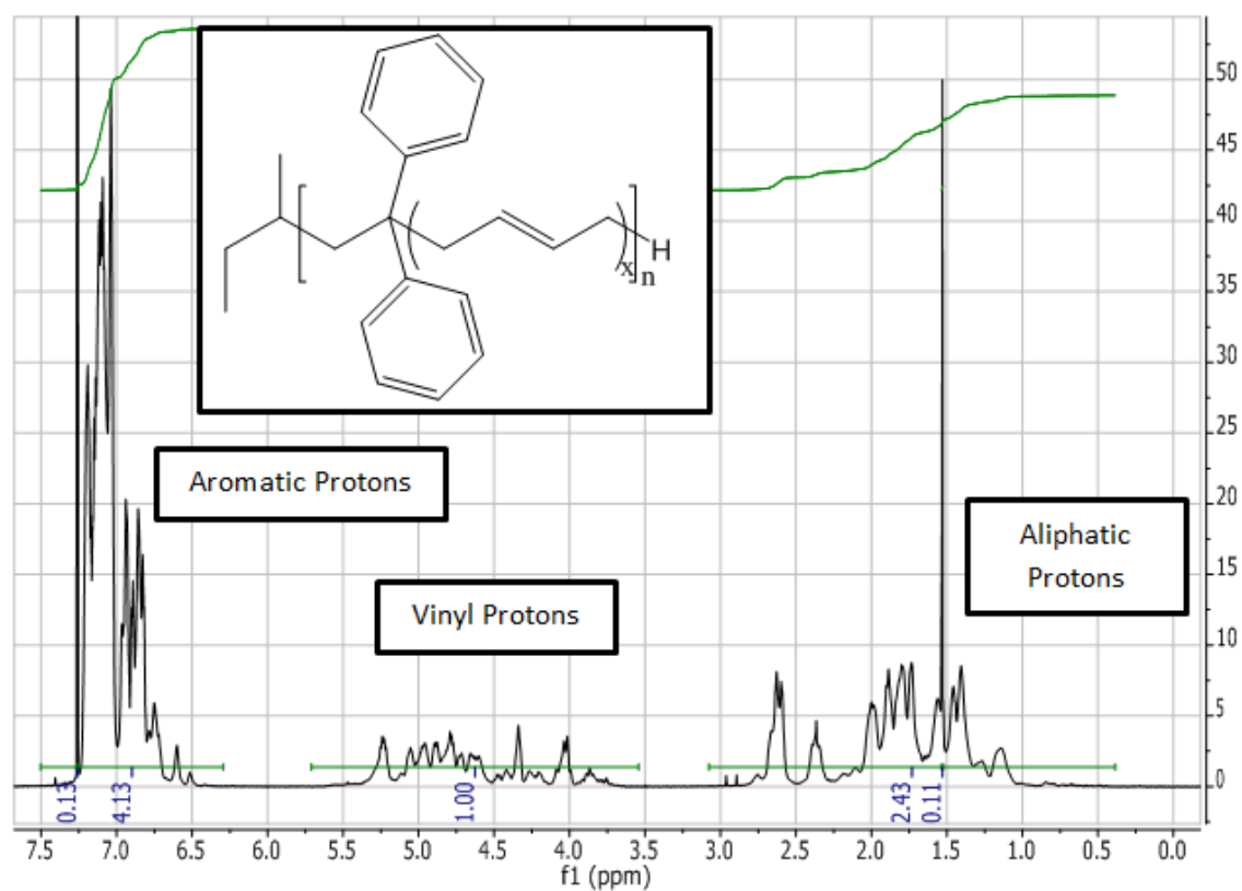
Figure 2.19: ^1\text{H} NMR spectrum (in \text{CDCl}_3 ) of Poly(butadiene-co-DPE), PBdD-1, synthesized in THF with a molar feed ratio of 1.04 : 1.00 butadiene : DPE.
