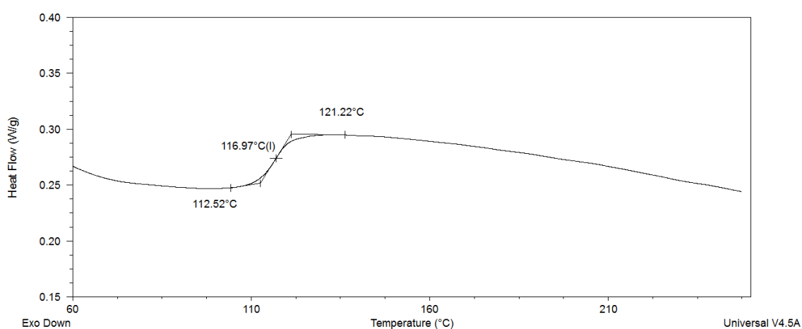
Figure 3.104: DSC thermogram obtained for the poly(butadiene-co-DPE) copolymer, PBdD-1, heated at a rate of 10 °C/min.
