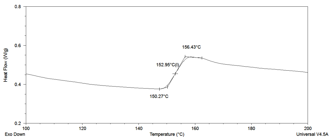
Figure 3.128: DSC thermogram obtained for the poly(butadiene-co-styrene-co-DPE) copolymer, PBdSD-10a, showing the T_g observed upon heating at 40 °C/min.
