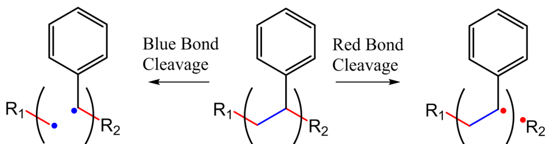
Figure 4.158: Schematic diagram showing the fragmentation of a styrene unit.
