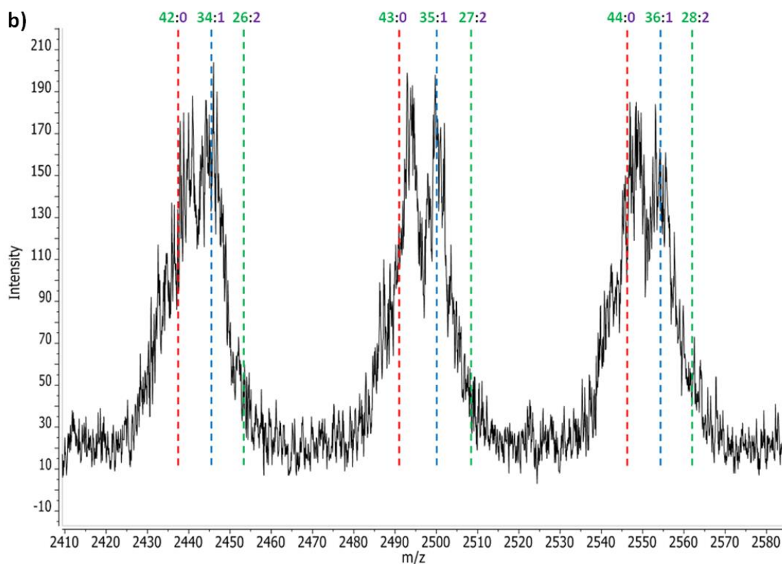
Figure 4.162: (a) MALDI-ToF spectrum of a sample (P(Bd-co-D OSi )-5b) collected after 32 hours (15 hours with TMEDA) of the anionic copolymerization of butadiene and DPE-OSi, in benzene with a molar feed ratio of Bd : DPE-OSi = 18.5 : 1.0 and (b) expansion showing the range m/z = 2410 - 2580 with red, blue and green dashed lines indicating where chains containing 0, 1 and 2 units of DPE-OSi respectively, would be expected to appear. The mole ratio of butadiene : DPE-OSi for any given chain is labelled with butadiene in green and DPE-OSi in purple.
