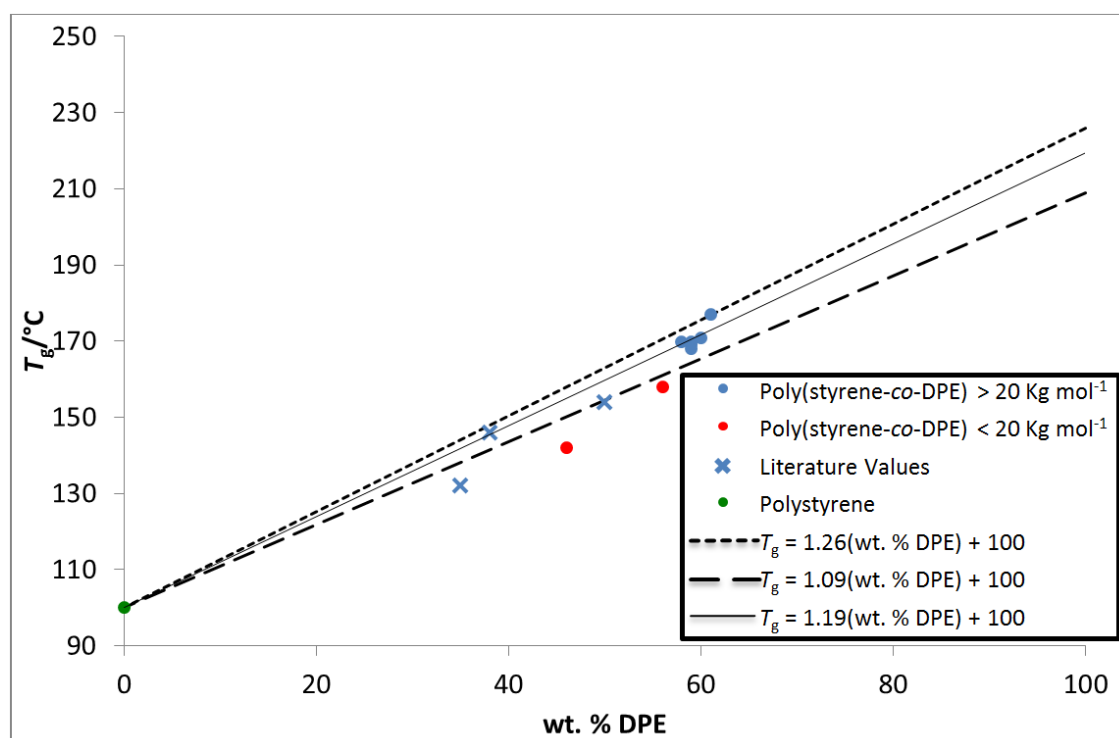
Figure 3.103: Graph showing the correlation between T_g and wt. % DPE for poly(styrene-co-DPE) copolymers.
