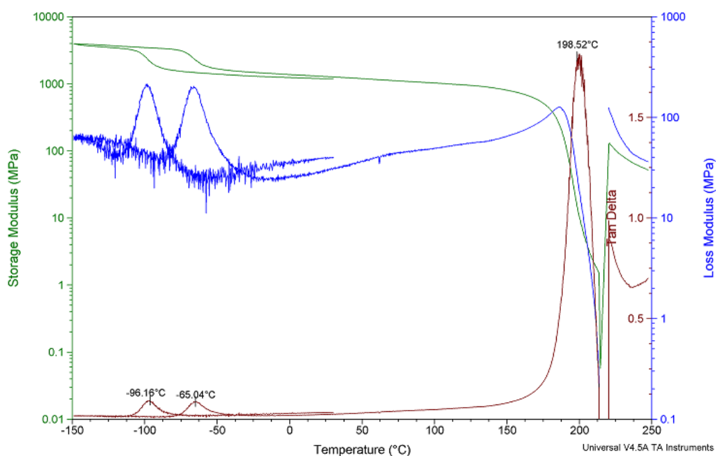
Figure 3.107: DMA analysis on the poly(styrene- co -DPE)- block -polybutadiene copolymer, PSD-PBd-3, showing the T_g observed upon heating and cooling at 5 °C/min.
