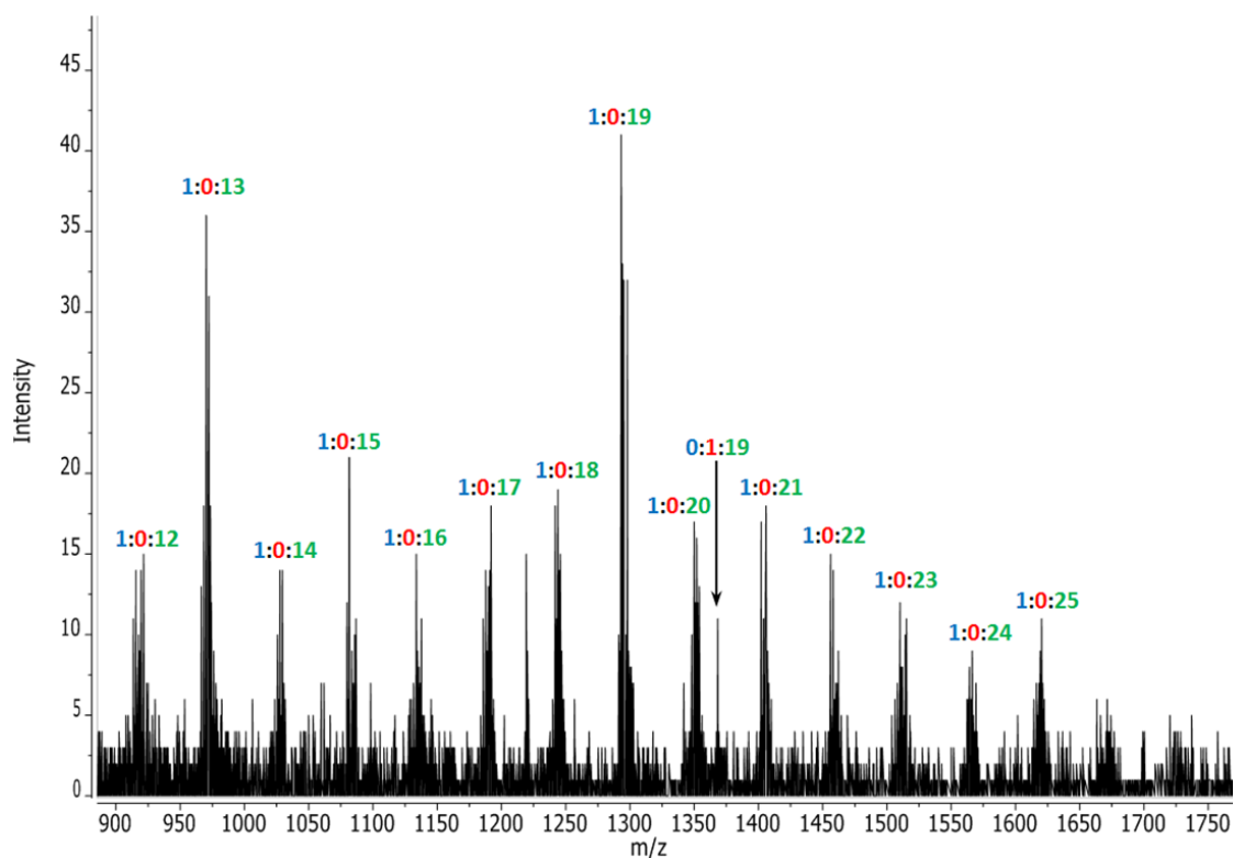
Figure 2.53: MALDI-ToF mass spectrum for the copolymer PBdSD-3c prepared by the anionic copolymerization (in benzene) of styrene, DPE and butadiene (monomer molar feed ratio of styrene : DPE : butadiene = 1.00 : 1.55 : 1.99) after 7.5 hours. The mole ratio of styrene : DPE : butadiene for any given chain is labelled with styrene in blue, DPE in red and butadiene in green.
