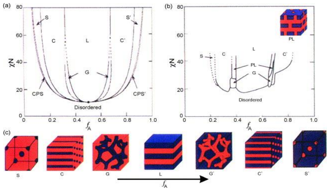
Figure 1.7: (a) Theoretical and (b) Experimental Phase diagram for a Polyisoprene- block -Polystyrene copolymer, and (c) microstructure schematics of (S) spherical (C) cylindrical (G) gyroid (L) lamellar and (PL) perforated layers. f_A is the volume fraction of polyisoprene, \chi is the interaction parameter, N is the degree of polymerization and CPS are close packed spheres. Reprinted with permission from Bates, F. S., Fredrickson, G. H., Physics Today , Vol. 52/2, Page 32-38, 1999. Copyright 1999, American Institute of Physics. 10
