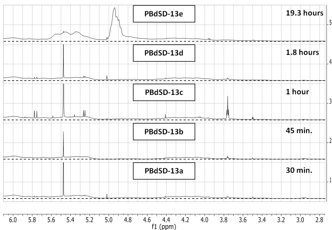
Figure 2.64: (a) ^1\text{H} NMR spectrum (in \text{CDCl}_3 ) of Poly(butadiene- co -styrene- co -DPE) copolymers, PBdSD-13a-e, synthesized in benzene with a molar feed ratio of 1.00 : 1.05 : 1.14 styrene : DPE : butadiene and (b) expansion of the alkene region (2.8 – 6.0 ppm) with the baseline indicated by a dotted line.
