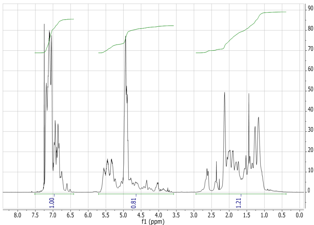
Figure 2.95: ^1\text{H} NMR spectrum (in \text{CDCl}_3 ) for the poly(butadiene-co-DPE), PBdD-7b, synthesized in THF with a molar feed ratio of 1.00 : 2.85 DPE : butadiene and terminated after 22.8 hours at 0^\circ\text{C} .
