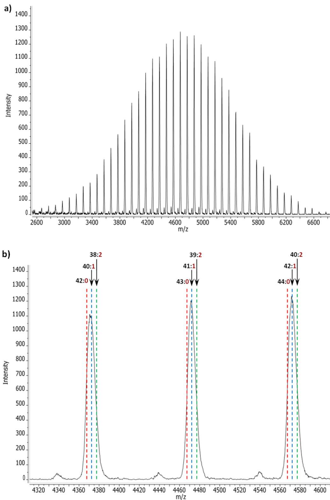
Figure 4.144: (a) MALDI-ToF mass spectrum of poly(MMA-co-DPE-CN), P(MMA-co-D CN )-1, synthesized in THF with a molar feed ratio 10.0 : 1.0 MMA : DPE-CN and (b) expansion showing the range m/z = 4320 – 4600 with red, blue and green dashed lines indicating where chains containing 0, 1 and 2 units of DPE-CN respectively, would be expected to appear. The mole ratio of MMA : DPE-CN for any given chain is labelled with MMA in black and DPE-CN in red.
