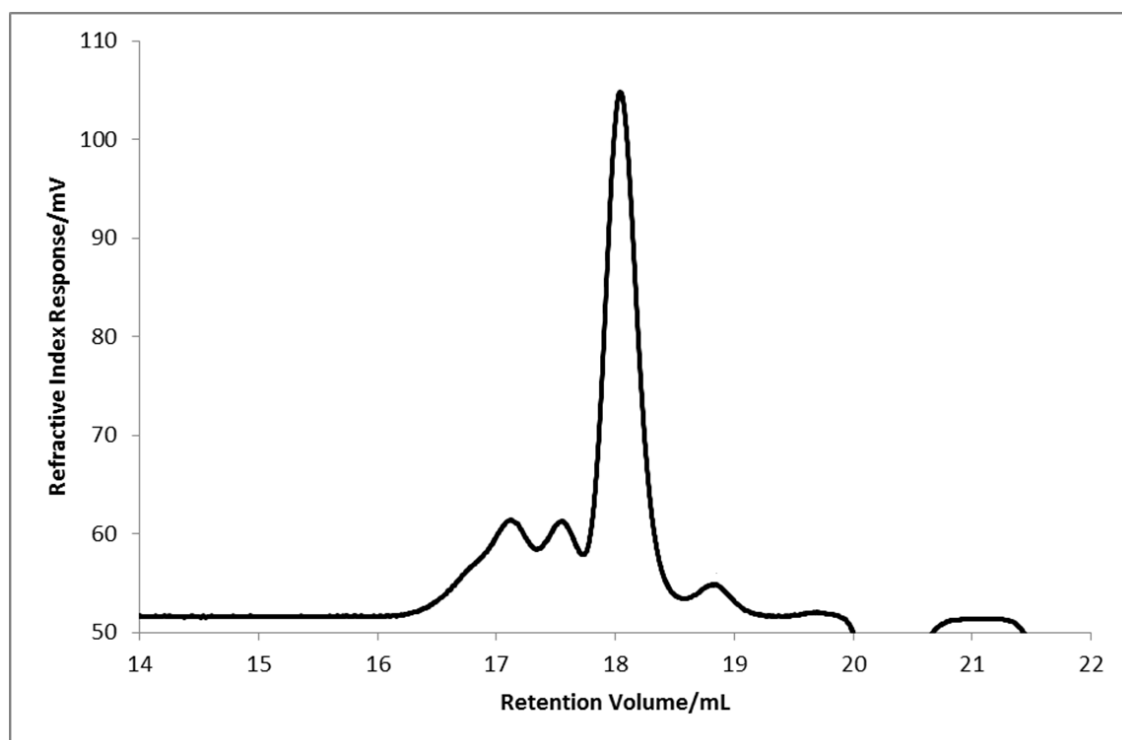
Figure 4.148: SEC trace for poly(butadiene-co-DPE-OSi) copolymer, P(Bd-co-DOSi)-1, showing the refractive index response.
