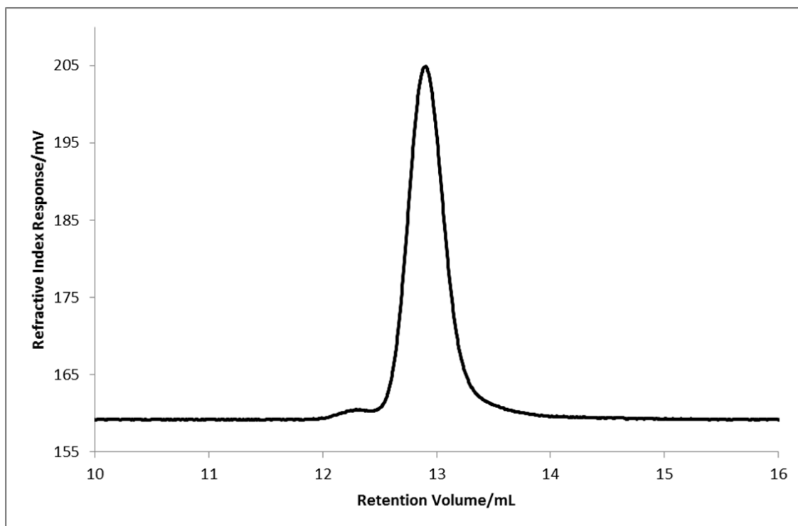
Figure 2.98: SEC chromatogram (refractive index) for the poly(butadiene- co -DPE) copolymer, PBdD-8.
