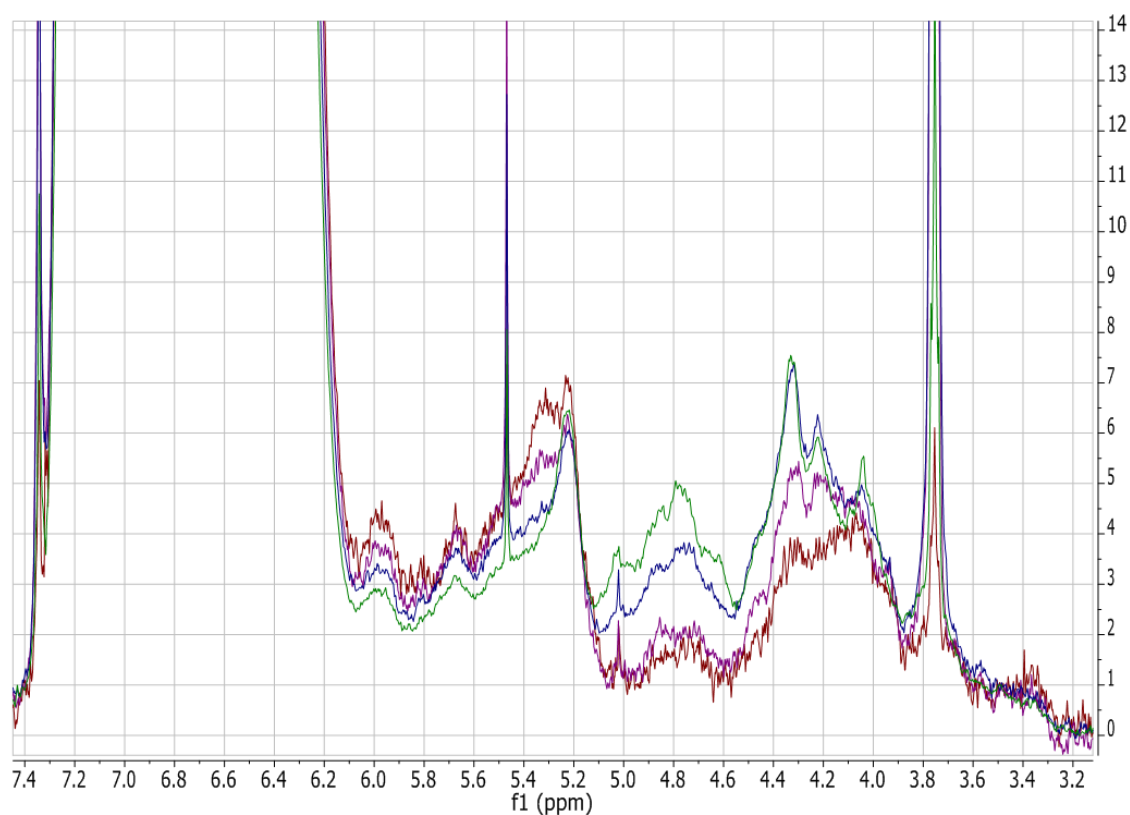
Figure 2.60: Overlay and expansion of the alkene region of the ^1\text{H} NMR spectrum (in \text{CDCl}_3 ) of Poly(butadiene- co -styrene- co -DPE) copolymers, PBdSD-10a-e, synthesized in THF with a molar feed ratio of 1.00 : 2.06 : 1.00 styrene : DPE : butadiene. Red corresponds to PBdSD-10a; purple corresponds to PBdSD-10b; blue corresponds to PBdSD-10c and green corresponds to PBdSD-10e.
