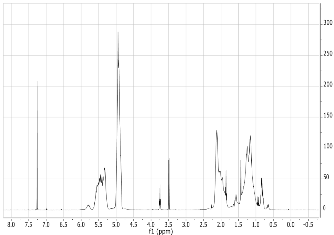
Figure 2.63: ^1\text{H} NMR spectrum (in \text{CDCl}_3 ) of high 1,2-polybutadiene, synthesized in THF (1,2-polybutadiene content = 84 %).
