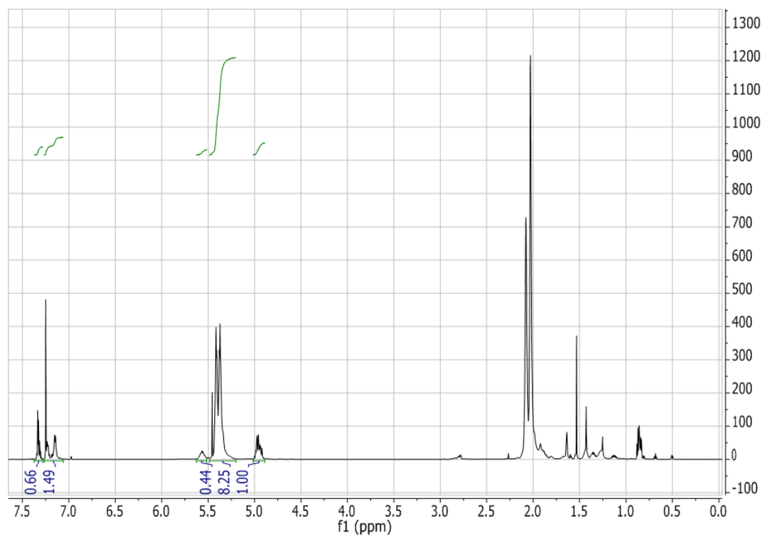
Figure 2.33: ^1\text{H} NMR spectrum (in \text{CDCl}_3 ) of Poly(butadiene-co-DPE), PBdD-3b, synthesized in benzene with a molar feed ratio of 3.26 : 1.00 butadiene : DPE and terminated after 19.7 hours.
