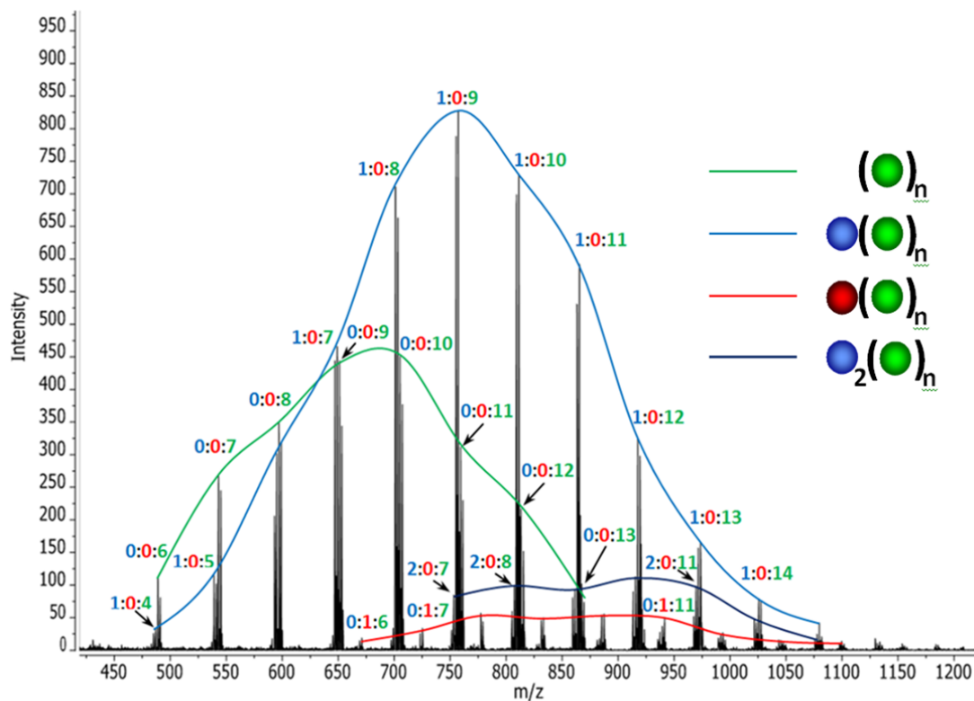
Figure 2.51: MALDI-ToF mass spectrum for the copolymer PBdSD-3b prepared by the anionic copolymerization (in benzene) of styrene, DPE and butadiene (monomer molar feed ratio of styrene : DPE : butadiene = 1.00 : 1.55 : 1.99) after 1.3 hours. The mole ratio of styrene : DPE : butadiene for any given chain is labelled with styrene in blue, DPE in red and butadiene in green.
