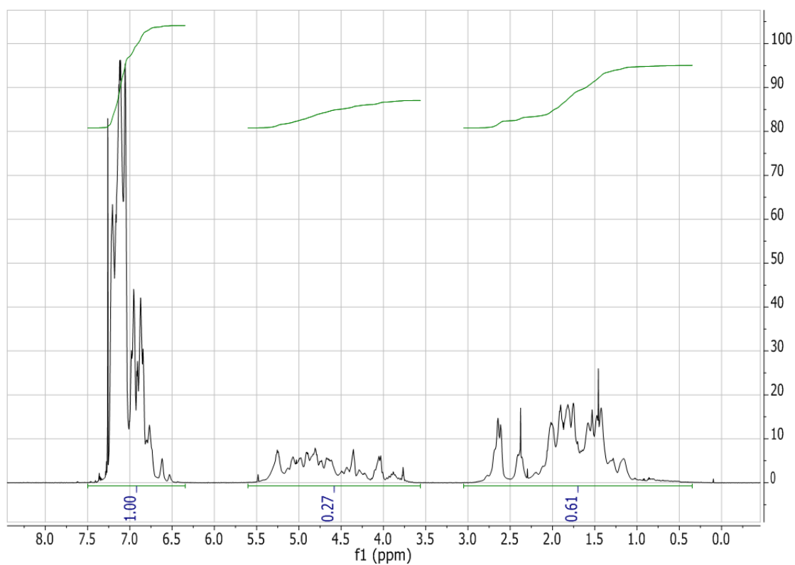
Figure 2.94: 1 H NMR spectrum (in CDCl 3 ) for the poly(butadiene-co-DPE), PBdD-7a, synthesized in THF with a molar feed ratio of 1.00 : 2.85 DPE : butadiene and terminated after 1.5 hours at 0 °C.
