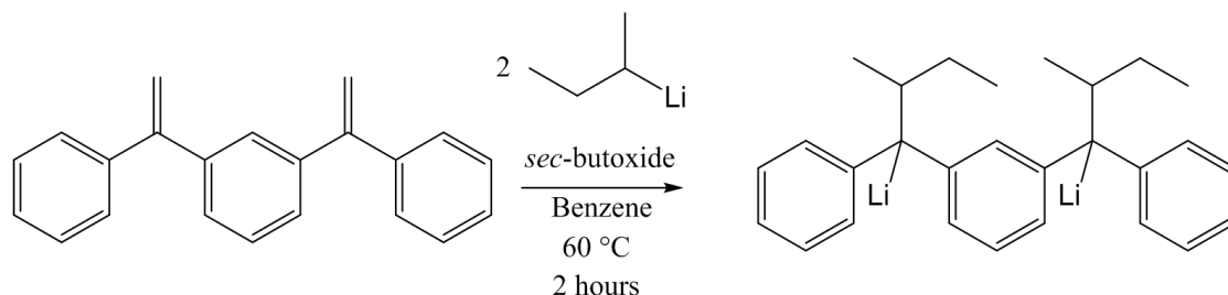
Figure 2.74: Reaction scheme for the formation of the difunctional initiator from 1,3-bis(1-phenylvinyl)benzene).
