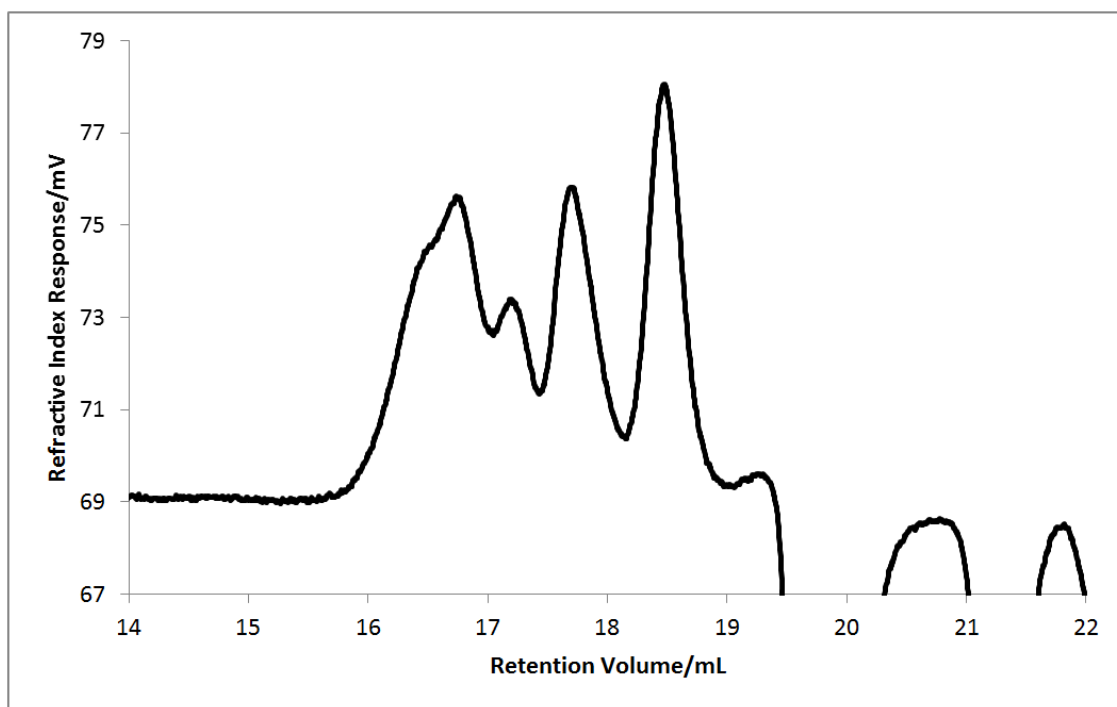
Figure 4.151: SEC trace for poly(butadiene- co -DPE-OSi) copolymer, P(Bd- co -D OSi )-2a, showing the refractive index response.
