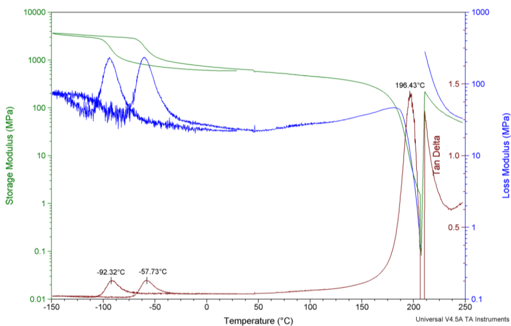
Figure 3.110: DMA analysis on the poly(butadiene-co-styrene-co-DPE) copolymer, PBdSD-4d, showing the T_g observed upon heating and cooling at 5 °C/min.
