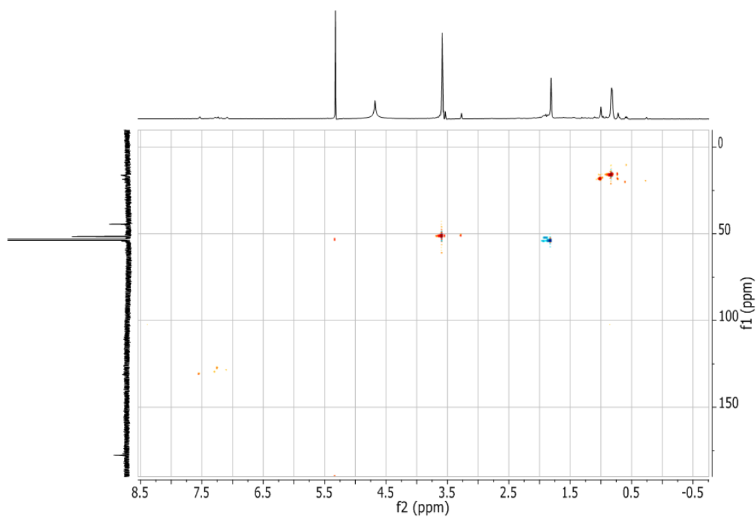
Figure 4.146: HSQCAD NMR spectrum (in \text{CD}_2\text{Cl}_2 ) of poly(MMA-co-DPE-CN), P(MMA-co- \text{D}_{\text{CN}} )-2, synthesized in THF with a molar feed ratio 1.0 : 1.0 MMA : DPE-CN.
