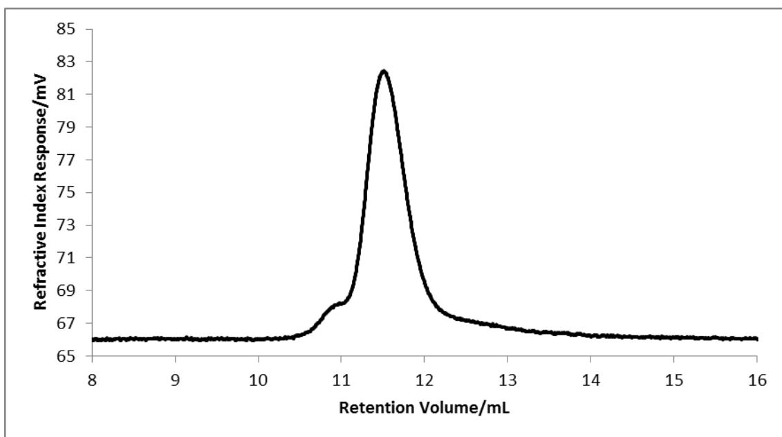
Figure 2.75: SEC chromatogram (refractive index) for the poly(styrene- co -DPE)- co -polybutadiene- co -poly(styrene- co -DPE) copolymer.
