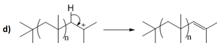
Figure 1.3: Schematic showing (a) the formation of the initiator species (b) initiation of the monomer (c) propagation and (d) termination via a unimolecular rearrangement for the cationic polymerization of isobutene using the initiator [\text{BF}_3\text{OH}]^-\text{H}^+ .
