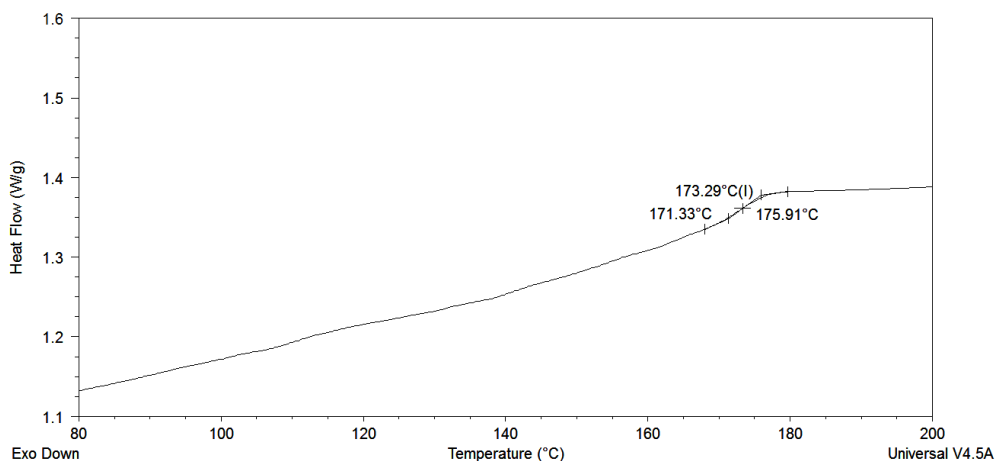
Figure 3.111: DSC thermogram obtained for the poly(butadiene-co-styrene-co-DPE) copolymer, PBdSD-4d, showing the T_g observed upon heating at 40 °C/min.
