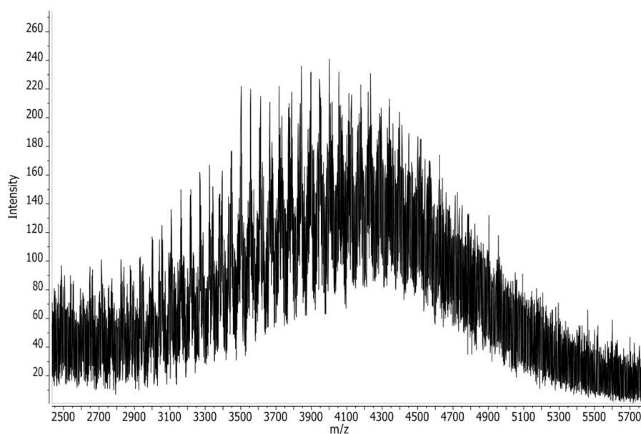
Figure 2.43: MALDI-ToF mass spectrum for the copolymer P(SD)-PBd-5 prepared by sequential addition of butadiene to a copolymerization (in benzene) of styrene and DPE using living anionic polymerization (monomer molar feed ratio of styrene : DPE : butadiene = 1.00 : 1.54 : 4.42).
