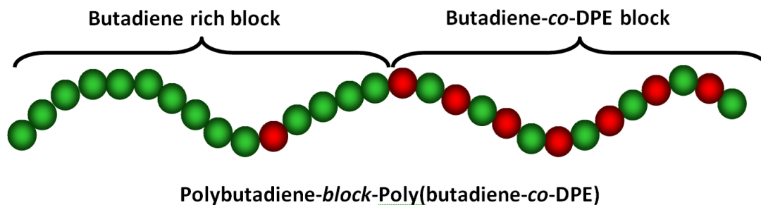
Figure 2.84: Schematic diagram to show the potential structure of a polybutadiene- block -poly(butadiene-co-DPE) terpolymer when butadiene (green balls) and DPE (red balls) (molar feed ratio of butadiene : DPE = 1 : 1) are initially copolymerized in toluene with THF added before the complete consumption of butadiene.
