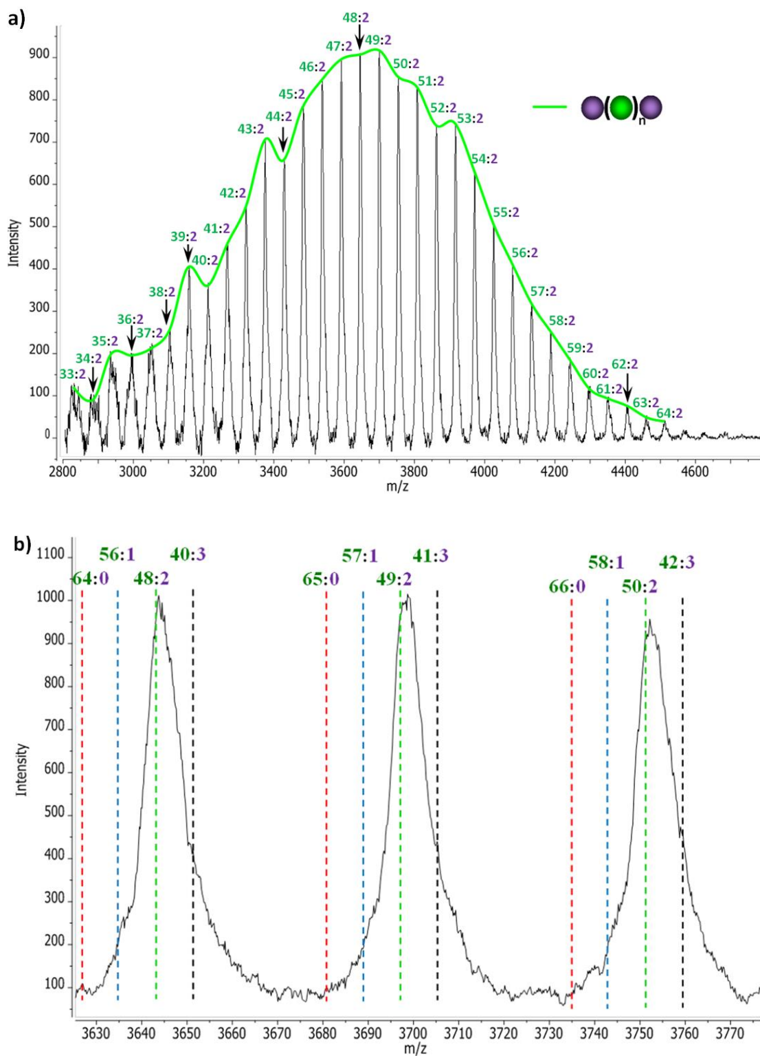
Figure 4.166: (a) MALDI-ToF mass spectrum for the anionic copolymerization (in benzene) of butadiene and DPE-OSi after 3 days without TMEDA and 6 days with TMEDA, \text{P}(\text{Bd-co-DOSi})\text{-6c} , with a molar feed ratio of \text{Bd} : \text{DPE-OSi} = 13.0 : 1.0 and (b) expansion showing the range m/z = 3630 - 3770 with red, blue and green dashed lines indicating where chains containing 0, 1 and 2 units of DPE-OSi respectively, would be expected to appear. The mole ratio of butadiene : DPE-OSi for any given chain is labelled with butadiene in green and DPE-OSi in purple.
