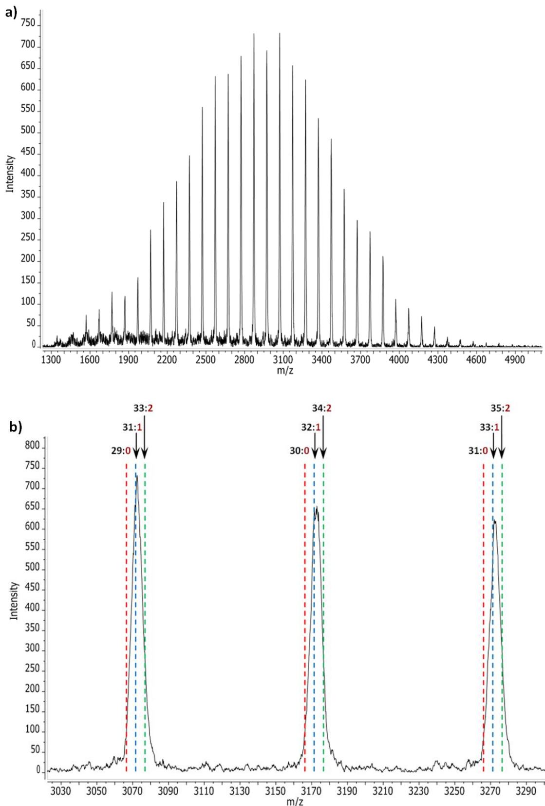
Figure 4.147: (a) MALDI-ToF mass spectrum of poly(MMA-co-DPE-CN), P(MMA-co-D CN )-2, synthesized in THF with a molar feed ratio 1.0 : 1.0 MMA : DPE-CN and (b) expansion showing the range m/z = 3030 – 3290 with red, blue and green dashed lines indicating where chains containing 0, 1 and 2 units of DPE-CN respectively, would be expected to appear. The mole ratio of MMA : DPE-CN for any given chain is labelled with MMA in black and DPE-CN in red.
