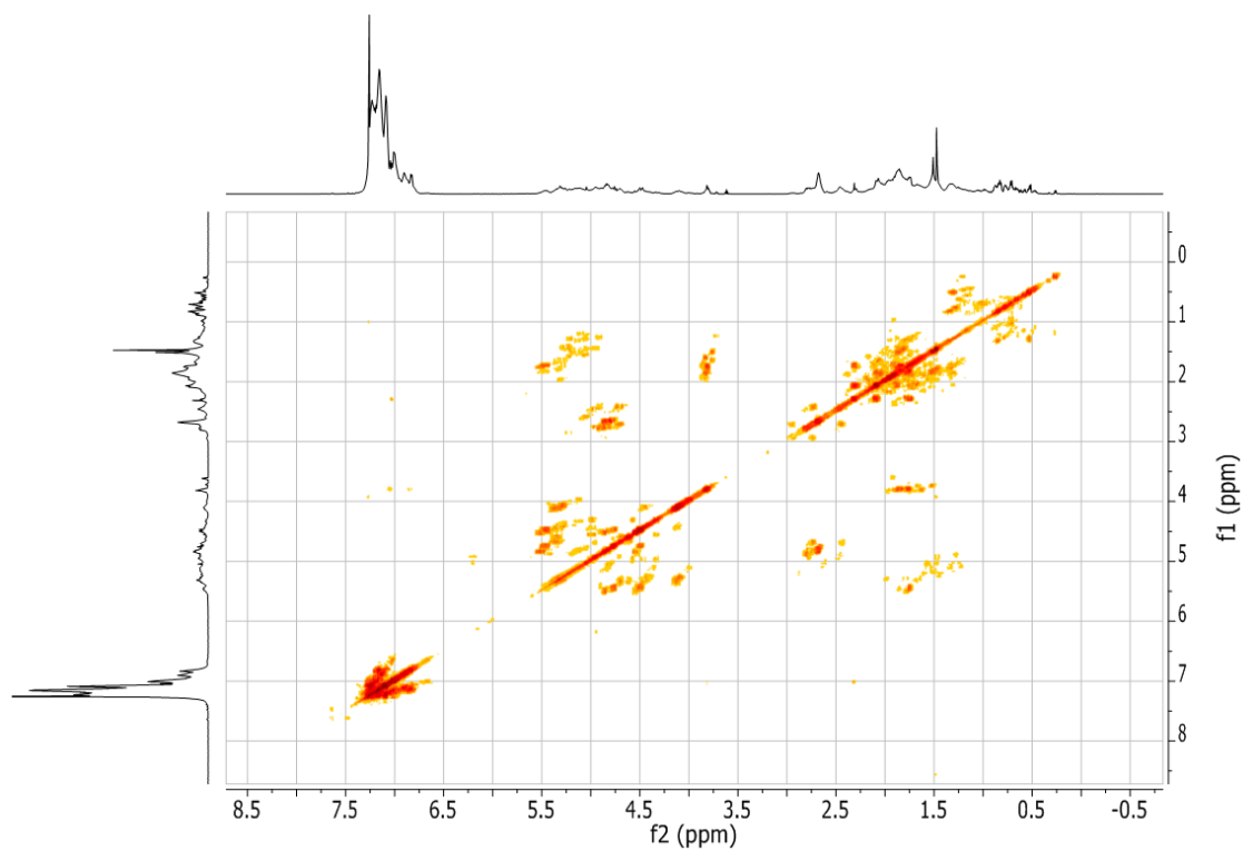
Figure 2.27: COSY NMR spectrum (in \text{CDCl}_3 ) of poly(butadiene- co -DPE), PBdD-2.
