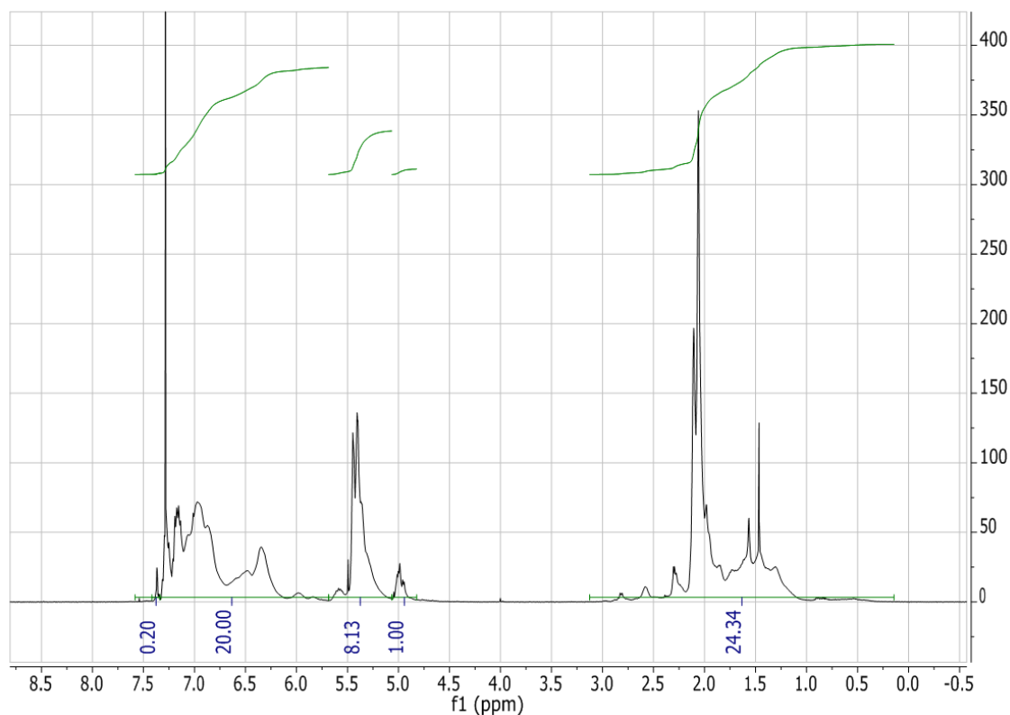
Figure 2.57: ^1\text{H} NMR spectrum (in \text{CDCl}_3 ) of Poly(butadiene- co -styrene- co -DPE), PBdSD-9, synthesized in toluene with a molar feed ratio of 1.00 : 1.06 : 1.70 styrene : DPE : butadiene.
