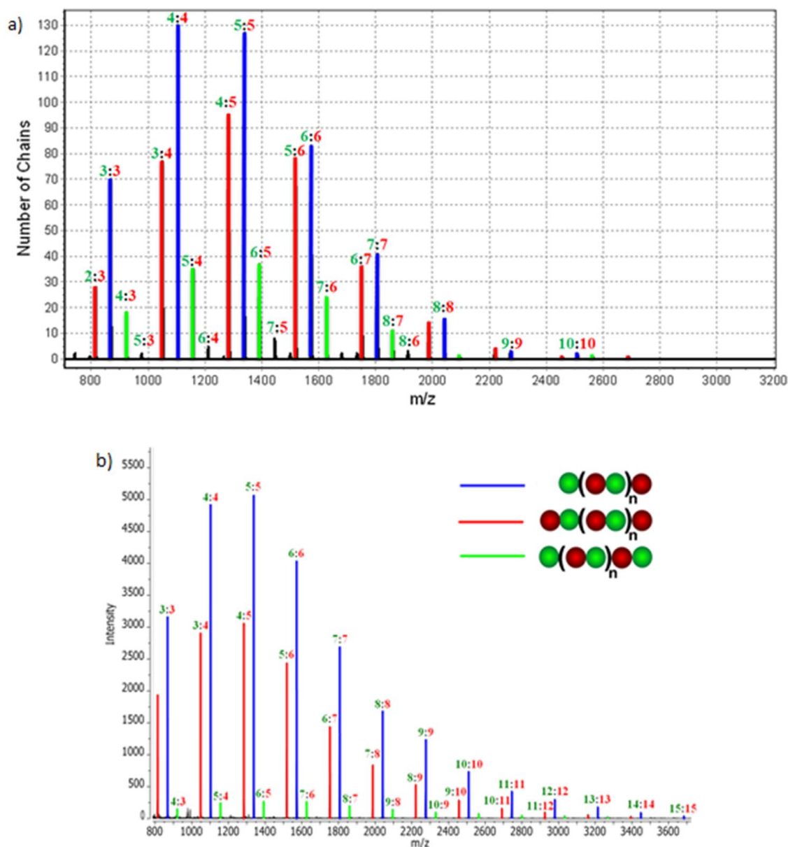
Figure 2.38: (a) Simulated versus (b) experimental MADLI-ToF data for the copolymer PBdD-2 prepared by the anionic copolymerization (in THF) of butadiene and DPE (monomer molar feed ratio of butadiene : DPE = 0.97 : 1.00). The mole ratio of butadiene : DPE for any given chain is labelled with butadiene in green and DPE in red.
