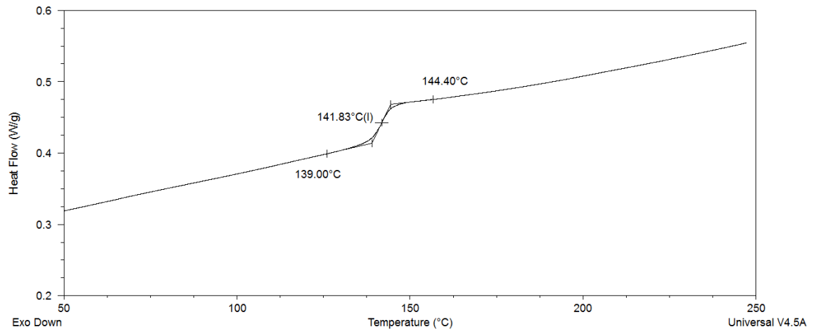
Figure 3.99: DSC thermogram obtained for the poly(styrene- co -DPE) copolymer, PSD-1, heated at a rate of 10 °C/min.
