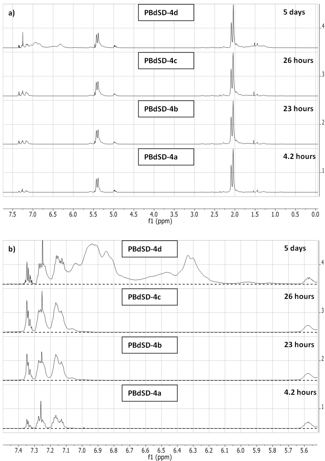
Figure 2.55: (a) 1 H NMR spectrum (in CDCl 3 ) of Poly(butadiene-co-styrene-co-DPE) copolymers, PBdSD-4a-d, synthesized in benzene with a molar feed ratio of 1.00 : 1.55 : 2.71 styrene : DPE : butadiene and (b) expansion of the aromatic region (5.6 – 7.4 ppm) with the baseline indicated by a dotted line.
