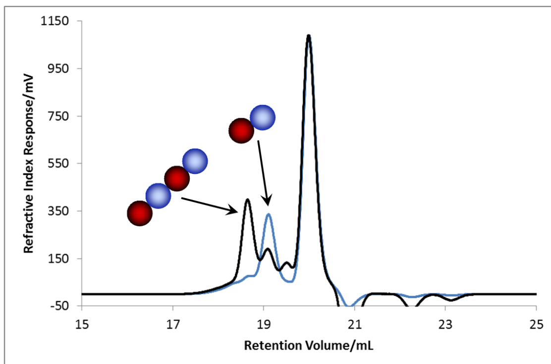
Figure 4.141: Size exclusion chromatography (RI) data for the copolymerization of styrene (blue balls) and DPE-CN (red balls) after 15 hours (blue line) and 24 hours (black line).
