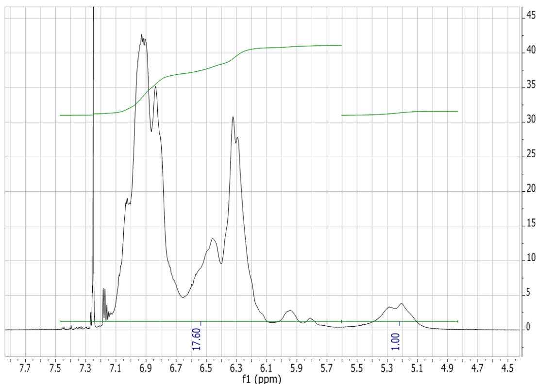
Figure 2.40: ^1\text{H} NMR spectrum (in \text{CDCl}_3 ) of Poly(styrene- co -DPE), PSD-4, synthesized in benzene with a molar feed ratio of 1.00 : 1.55 styrene : DPE (the aromatic region).
