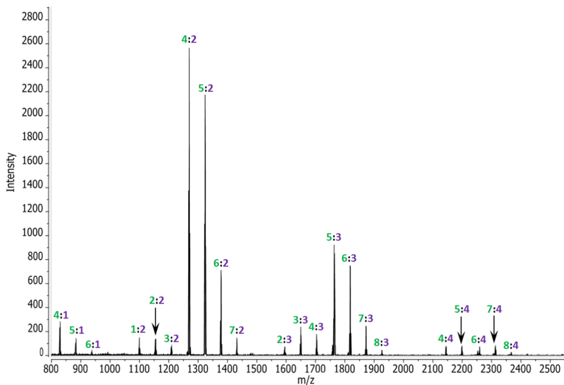
Figure 4.154: MALDI-ToF mass spectrum for the copolymer P(Bd-co-DOSi)-4 prepared by the copolymerization of butadiene and DPE-OSi (monomer molar feed ratio of butadiene : DPE-OSi = 1.09 : 1.00) in THF. The mole ratio of butadiene : DPE-OSi for any given chain is labelled with butadiene in green and DPE-OSi in purple.
