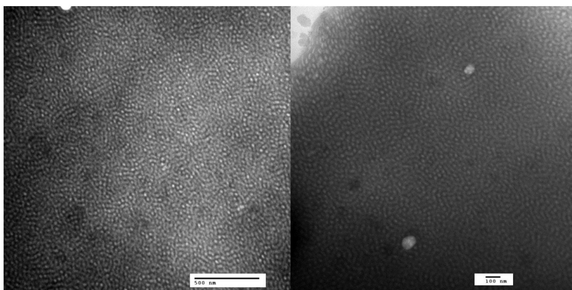
Figure 3.117: TEM images of the copolymer poly(butadiene- co -styrene- co -DPE), PBdSD-5, with the butadiene blocks stained black with OsO _4 .
