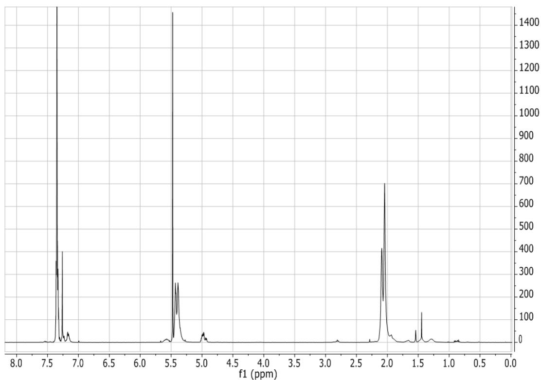
Figure 2.90: ^1\text{H} NMR spectrum (in \text{CDCl}_3 ) for the poly(butadiene-co-DPE), PBdD-6a, synthesized in toluene with a molar feed ratio of 1.00 : 0.96 DPE : butadiene.
