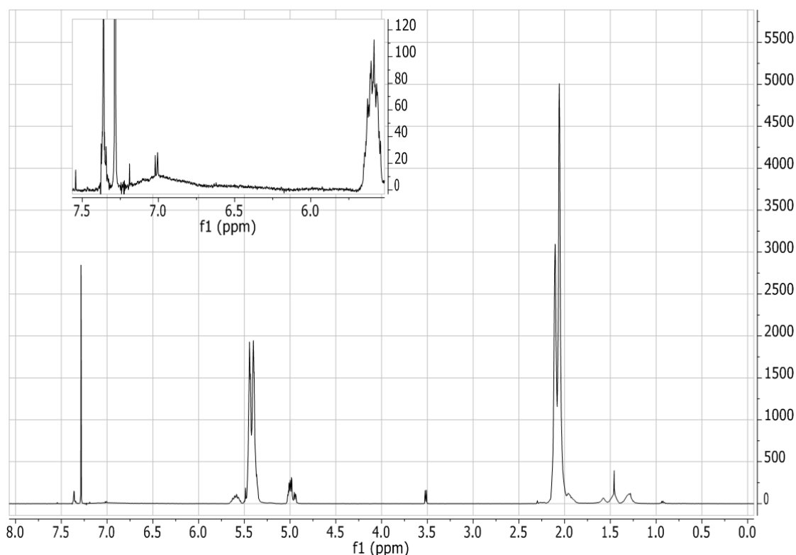
Figure 2.77: ^1\text{H} NMR spectrum (in \text{CDCl}_3 ) for the poly(styrene- co -DPE)- block -polybutadiene- block -poly(styrene- co -DPE) copolymer, P(SD)-PBd-P(SD)-1, synthesized in benzene with a molar feed ratio of 1.00 : 1.76 : 12.74 styrene : DPE : butadiene.
