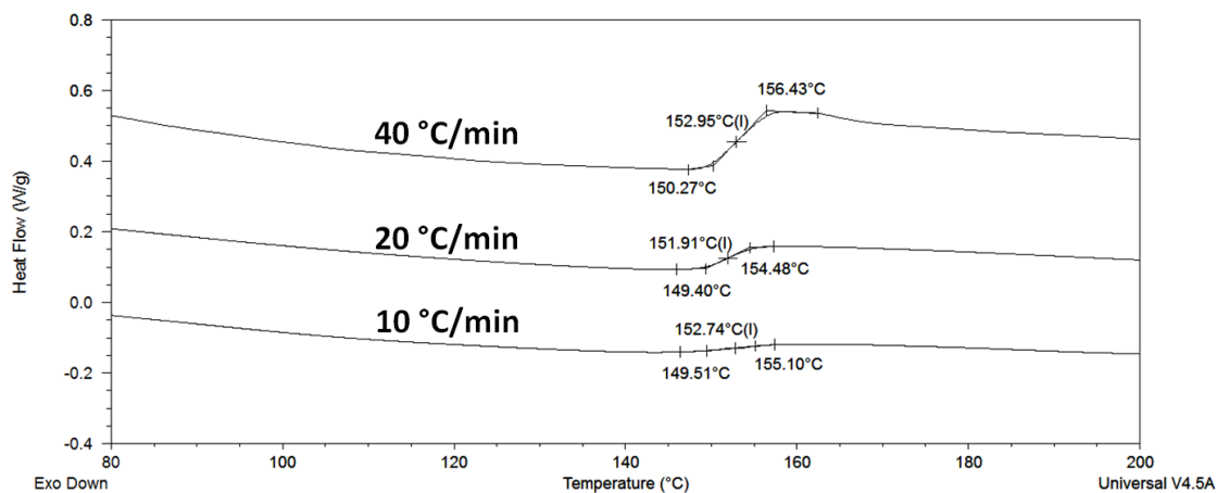
Figure 3.127: DSC thermogram obtained for the poly(butadiene-co-styrene-co-DPE) copolymer, PBdSD-10a, showing the T_g observed upon heating at 10 °C/min; 20 °C/min and 40 °C/min.
