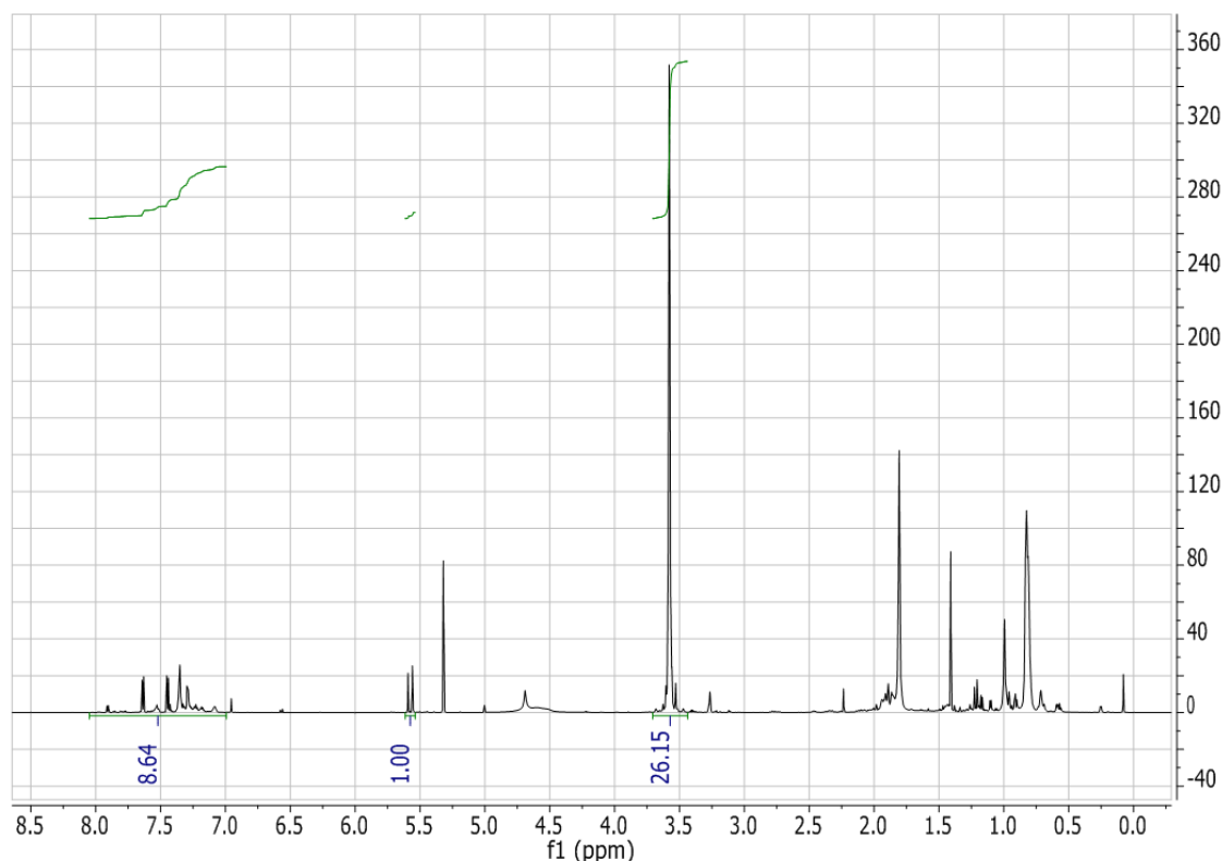
Figure 4.143: ^1\text{H} NMR spectrum (in \text{CD}_2\text{Cl}_2 ) of poly(MMA-co-DPE-CN), P(MMA-co-D CN )-1, synthesized in THF with a molar feed ratio 10.0 : 1.0 MMA : DPE-CN.
