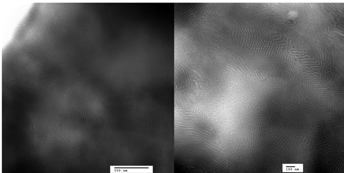
Figure 3.125: TEM images of a commercial polystyrene- block -polybutadiene- block -polystyrene copolymer, with the butadiene blocks stained black with OsO 4 .
