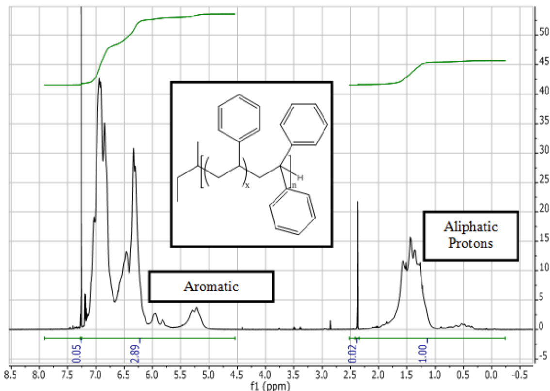
Figure 2.15: 1 H NMR spectrum (in CDCl 3 ) of Poly(styrene-co-DPE), PSD-4, synthesized in benzene with a molar feed ratio of 0.65 : 1.00 styrene : DPE.
