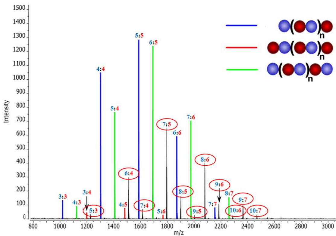
Figure 2.16: MALDI-ToF mass spectrum for the copolymer PSD-5 prepared by the anionic copolymerization (in benzene) of styrene and DPE (monomer molar feed ratio of styrene : DPE = 0.97 : 1.00). The mole ratio of styrene : DPE for any given chain is labelled with styrene in blue and DPE in red.
