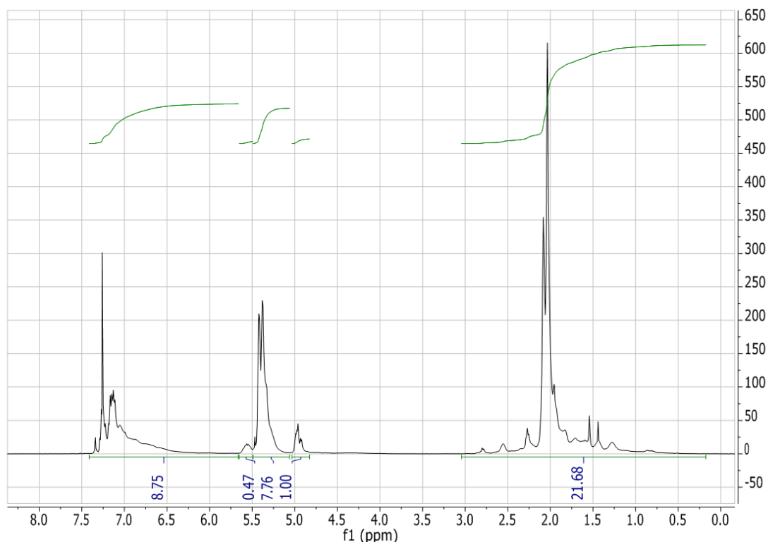
Figure 2.69: ^1\text{H} NMR spectrum (in \text{CDCl}_3 ) of Poly(butadiene- co -styrene- co -DPE), PBdSD-15, synthesized in toluene with a molar feed ratio of 1.00 : 1.02 : 1.82 styrene : DPE : butadiene with TMEDA injected after 25.6 hours when the reaction had just begun to darken.
