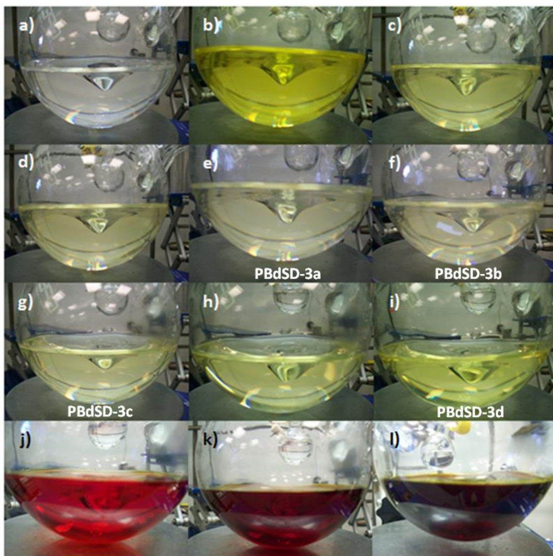
Figure 2.49: Photographs of the copolymerization of styrene, DPE and butadiene (a) before initiation (b) immediately after initiation and after (c) 12 seconds (d) 28 seconds (e) PBdSD-3a; 35 minutes (f) PBdSD-3b; 1.3 hours (g) PBdSD-3c; 7.5 hours (h) 9.6 hours (i) PBdSD-3d; 11.5 hours (j) 16.3 hours (k) 17.5 hours and (l) 21.8 hours at room temperature.
