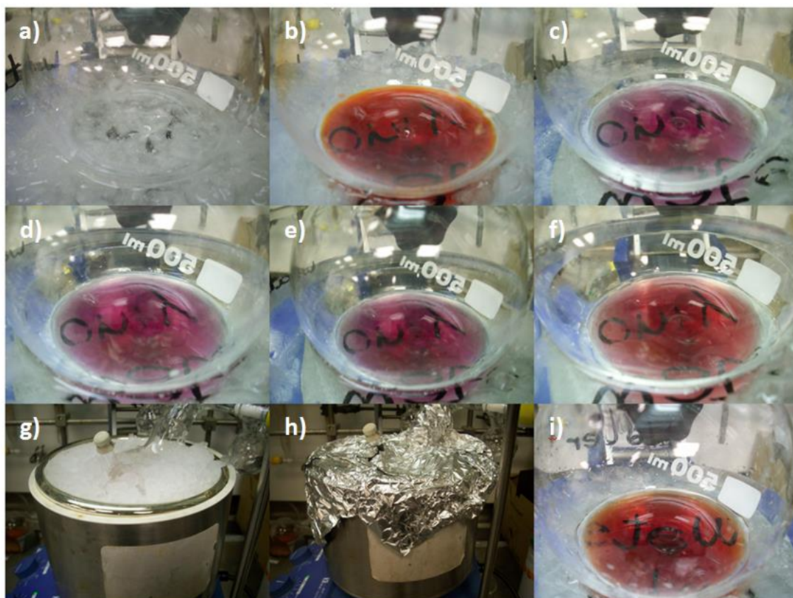
Figure 2.96: Photographs of the copolymerization of DPE and butadiene (PBdD-8) (a) before initiation (b) immediately after initiation and after (c) 1.1 hours (d) 1.7 hours (e) 2 hours (f) 2.7 hours (g) 2.8 hours (h) 2.9 – 14.7 hours (overnight) (i) 14.7 hours at 0 °C.
