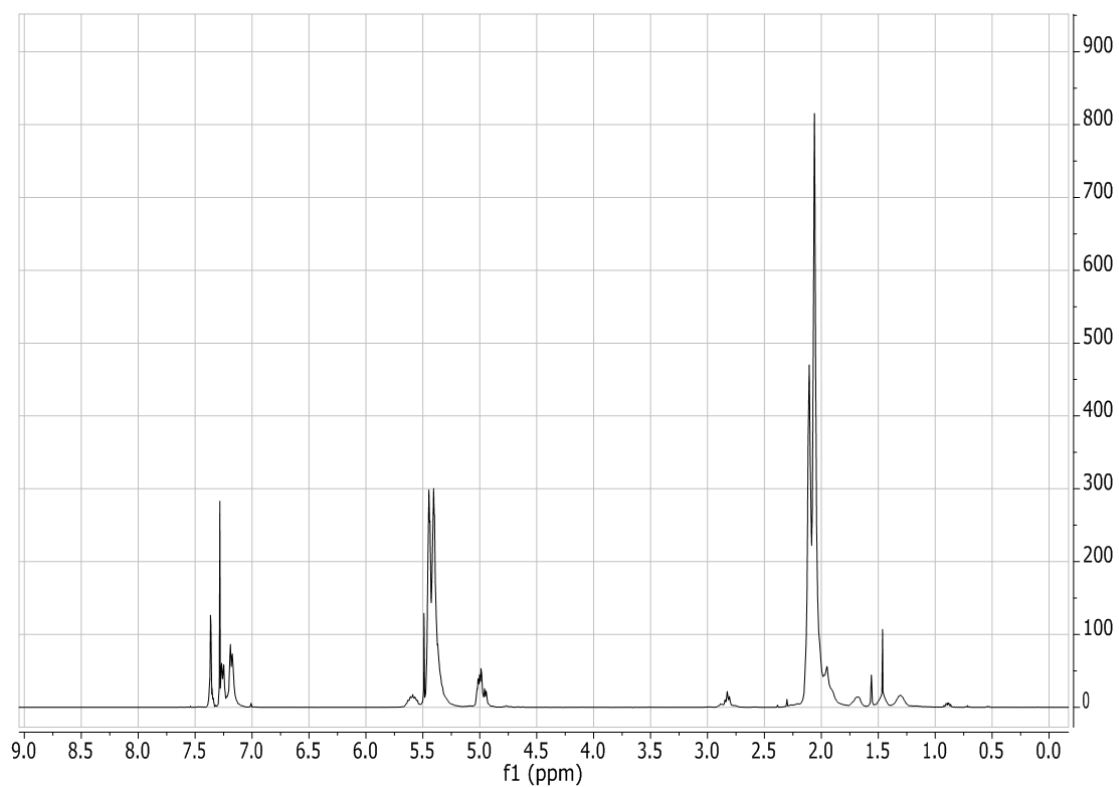
Figure 2.87: ^1\text{H} NMR spectrum (in \text{CDCl}_3 ) for the poly(butadiene-co-DPE), PBdD-5a, synthesized in toluene with a molar feed ratio of 1.00 : 0.96 DPE : butadiene.
