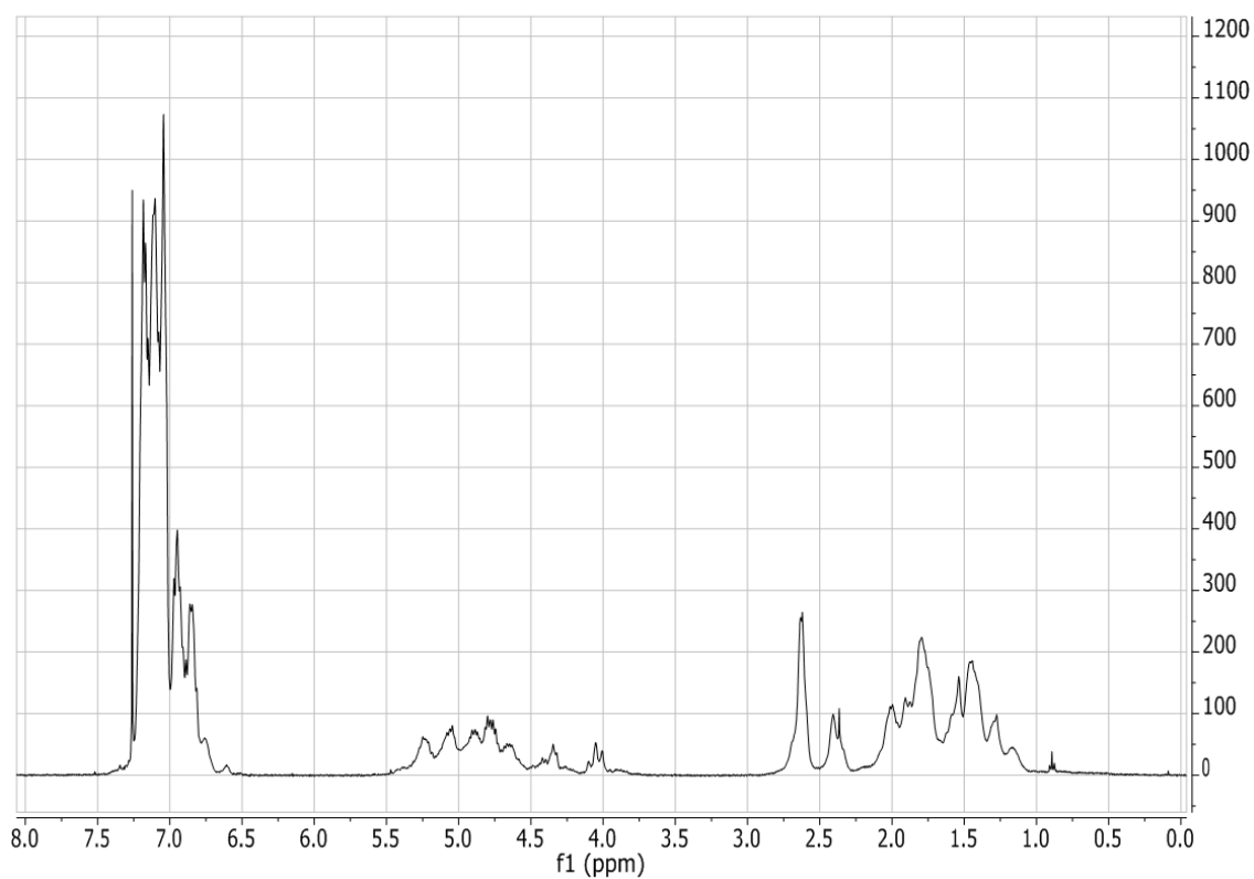
Figure 2.85: ^1\text{H} NMR spectrum (in \text{CDCl}_3 ) for the poly(butadiene- co -DPE), PBdD-4b, synthesized in toluene with THF added after 2.5 hours at room temperature and with a molar feed ratio of 1.00 : 1.05 DPE : butadiene.
