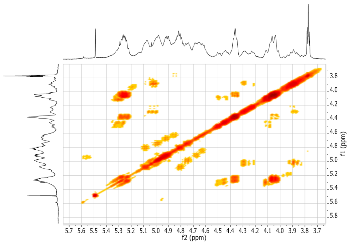
Figure 2.23: COSY NMR spectrum (in \text{CDCl}_3 ) of the alkene region of poly(butadiene-co-DPE), PBdD-1.
