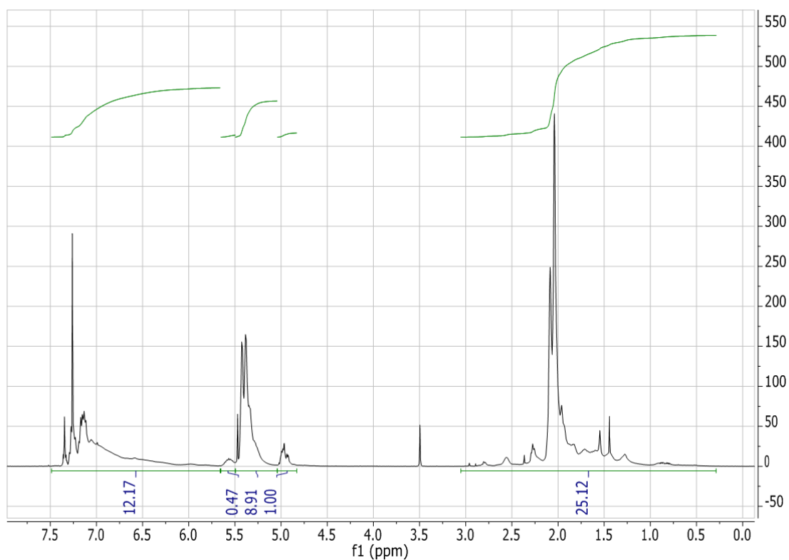
Figure 2.70: ^1\text{H} NMR spectrum (in \text{CDCl}_3 ) of Poly(butadiene- co -styrene- co -DPE), PBdSD-16, synthesized in toluene with a molar feed ratio of 1.00 : 1.06 : 1.60 styrene : DPE : butadiene with TMEDA injected after 23.8 hours when the reaction was dark yellow.
