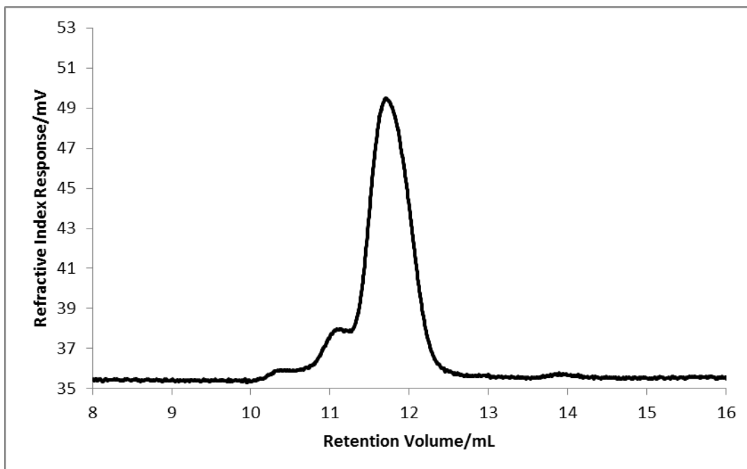
Figure 2.79: SEC chromatogram (refractive index) for the poly(styrene- co -DPE)- block -polybutadiene- block -poly(styrene- co -DPE) copolymer, P(SD)-PBd-P(SD)-3.
