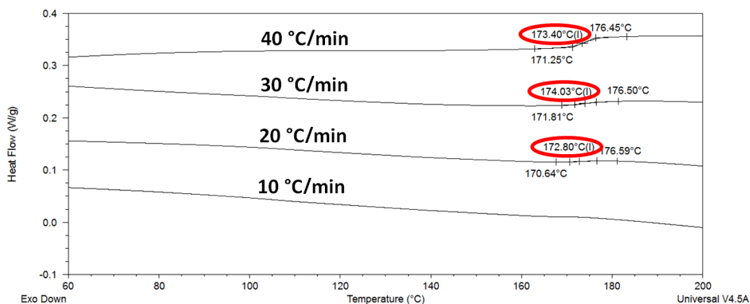
Figure 3.109: DSC thermogram obtained for the poly(styrene- co -DPE)- block -polybutadiene copolymer, PSD-PBd-3, showing the T_g observed upon heating at 10 °C/min; 20 °C/min; 30 °C/min and 40 °C/min with the T_g highlighted by red circles.
