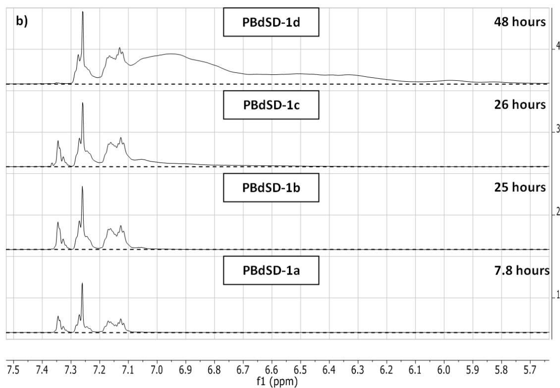
Figure 2.45: (a) ^1\text{H} NMR spectrum (in \text{CDCl}_3 ) of Poly(butadiene- co -styrene- co -DPE) copolymers, PBdSD-1a-d, synthesized in benzene with a molar feed ratio of 1.00 : 0.67 : 5.37 styrene : DPE : butadiene and (b) expansion of the aromatic region (5.7 – 7.5 ppm) with the baseline indicated by a dotted line.
