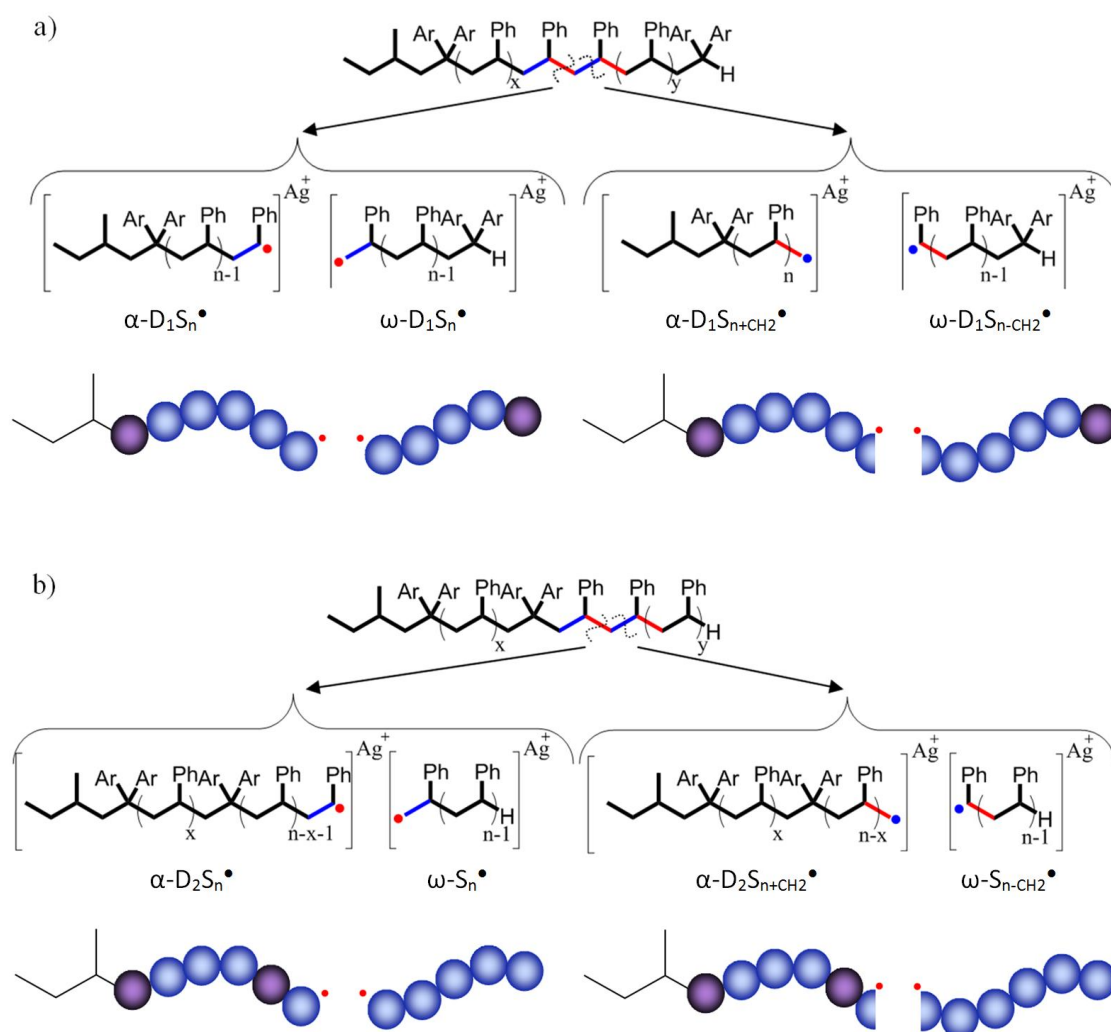
Figure 4.159: Possible sequences arising from fragmentation of (a) a perfect telechelic copolymer (b) a non-telechelic copolymer.
