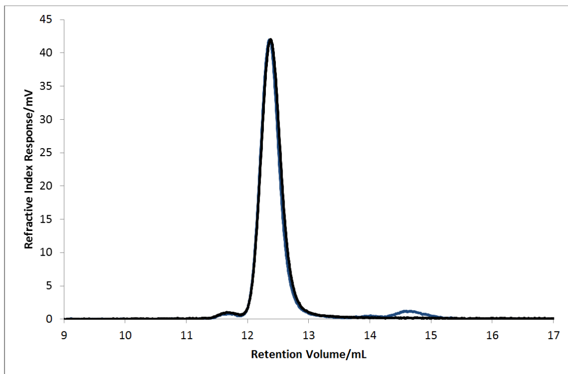
Figure 3.115: SEC chromatogram (refractive index) for the copolymer poly(styrene- co -DPE)- block -polybutadiene, PSD-PBd-6, before fractionation (blue) and after fractionation (black).
