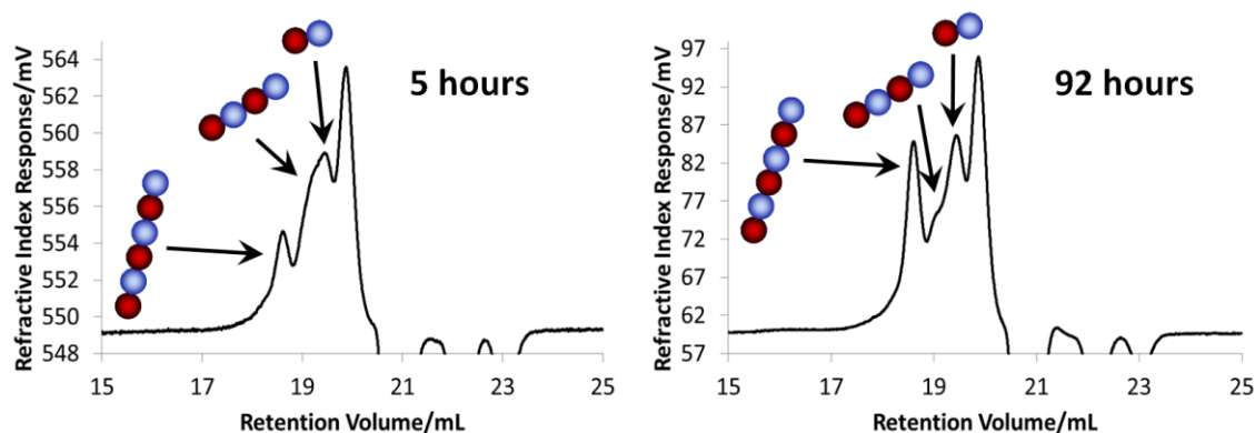
Figure 4.142: Size exclusion chromatography (RI) data for the copolymerization of styrene (blue balls) and DPE-CN (red balls) after 5 hours and 92 hours (initiated with sec -butyllithium).
