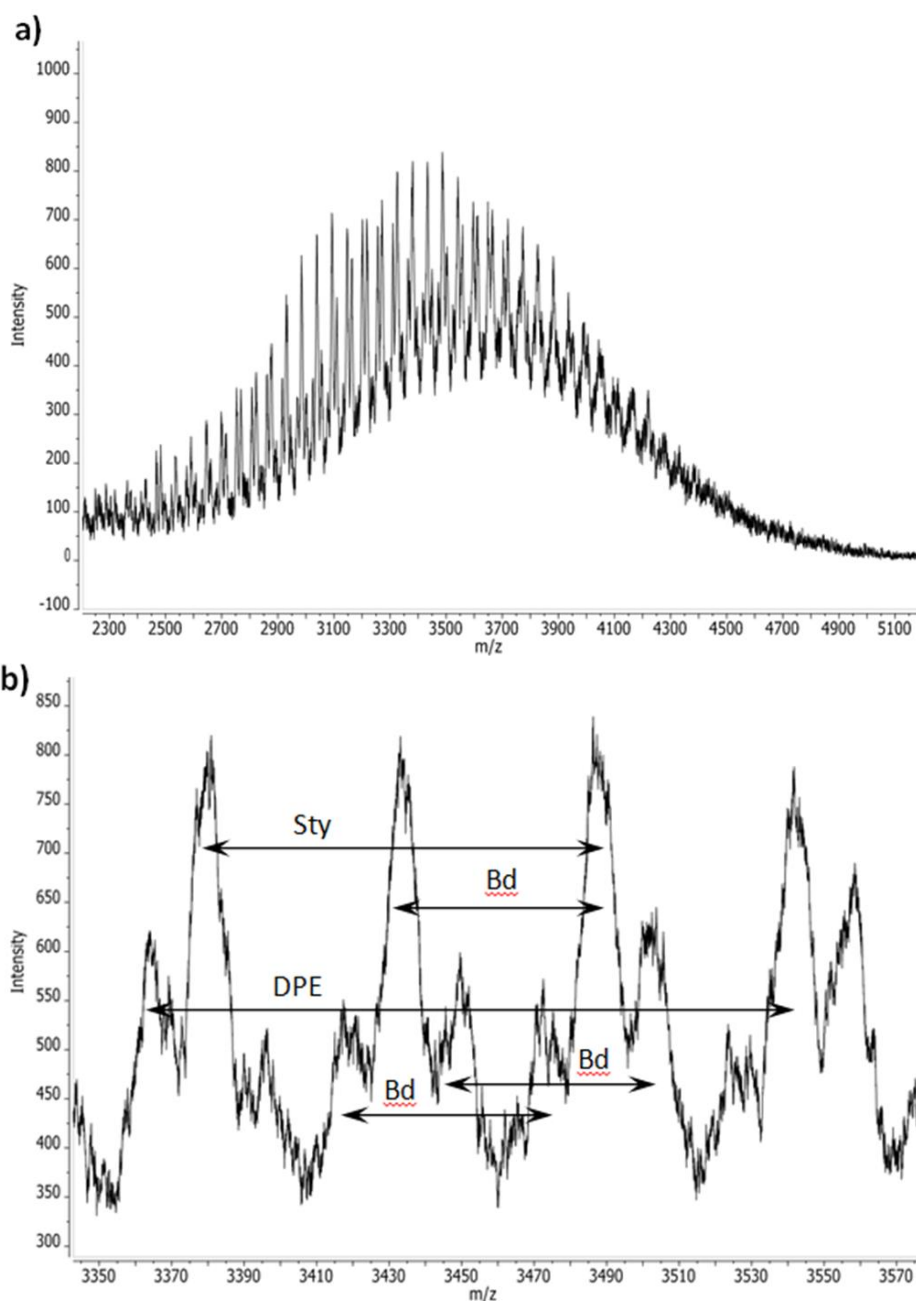
Figure 2.42: (a) MALDI-ToF mass spectrum and (b) expansion over the range m/z = 3350 - 3570 for the copolymer P(SD)-PBd-4 prepared by sequential addition of butadiene to a copolymerization (in benzene) of styrene and DPE using living anionic polymerization (monomer molar feed ratio of styrene : DPE : butadiene = 1.00 : 1.03 : 5.33).
