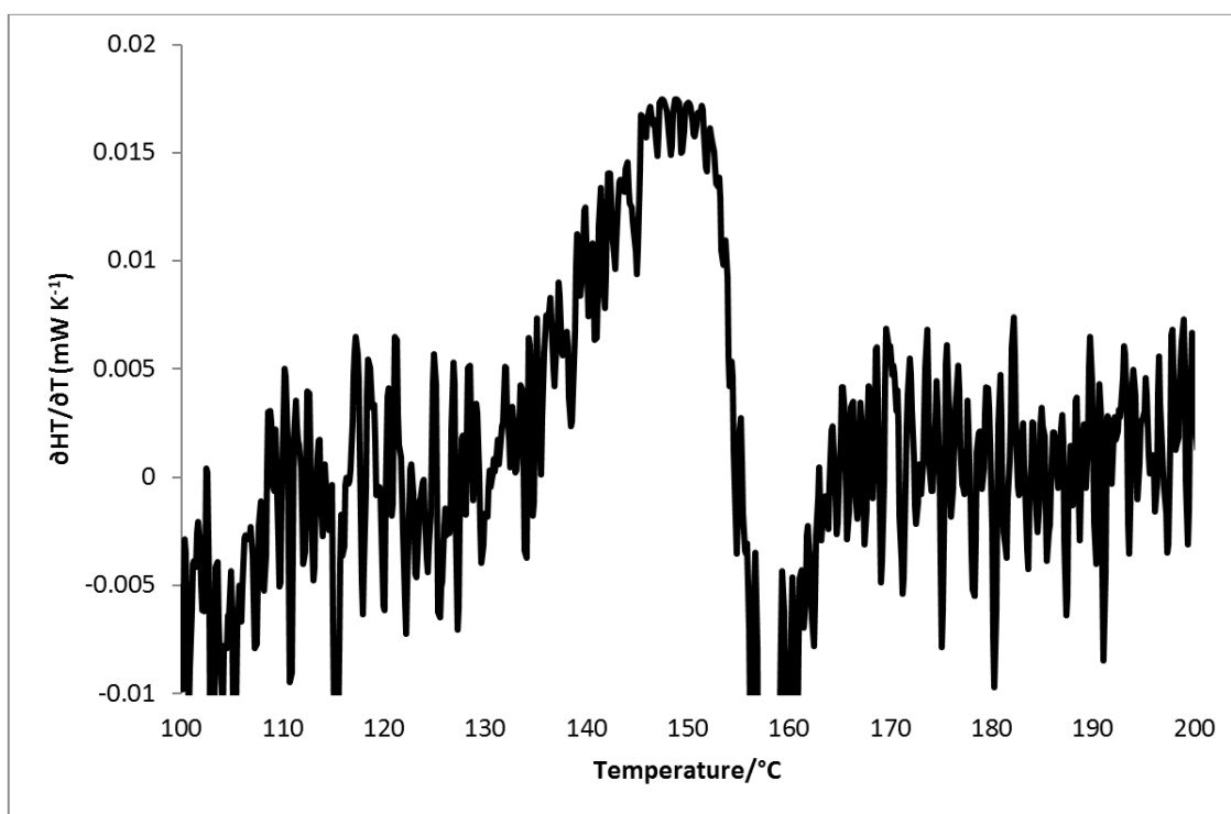
Figure 3.136: Derivative of Heat Flow (HF) vs Temperature (T) for the poly(butadiene- co -styrene- co -DPE) copolymer, PBdSD-10d.
