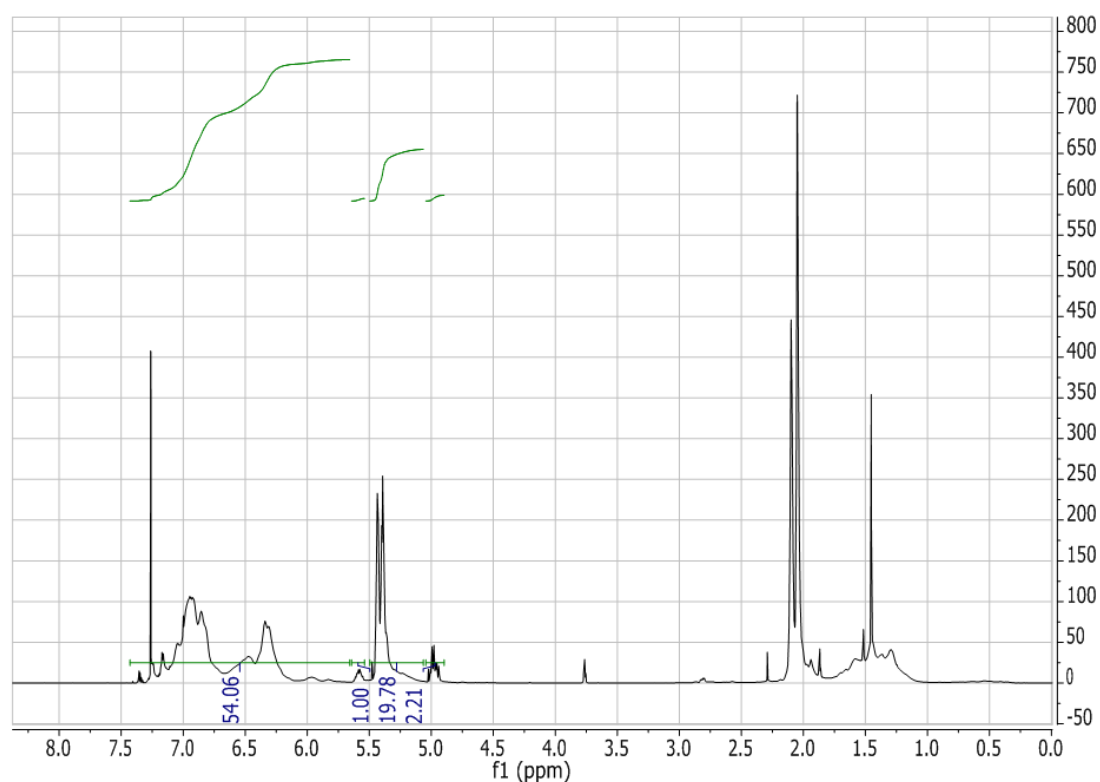
Figure 2.39: ^1H NMR spectrum (in CDCl_3 ) of Poly(styrene-co-DPE)- block -polybutadiene, P(SD)-PBd-3, sequentially synthesized in benzene with a molar feed ratio of 1.00 : 1.55 : 2.36 styrene : DPE : butadiene.
