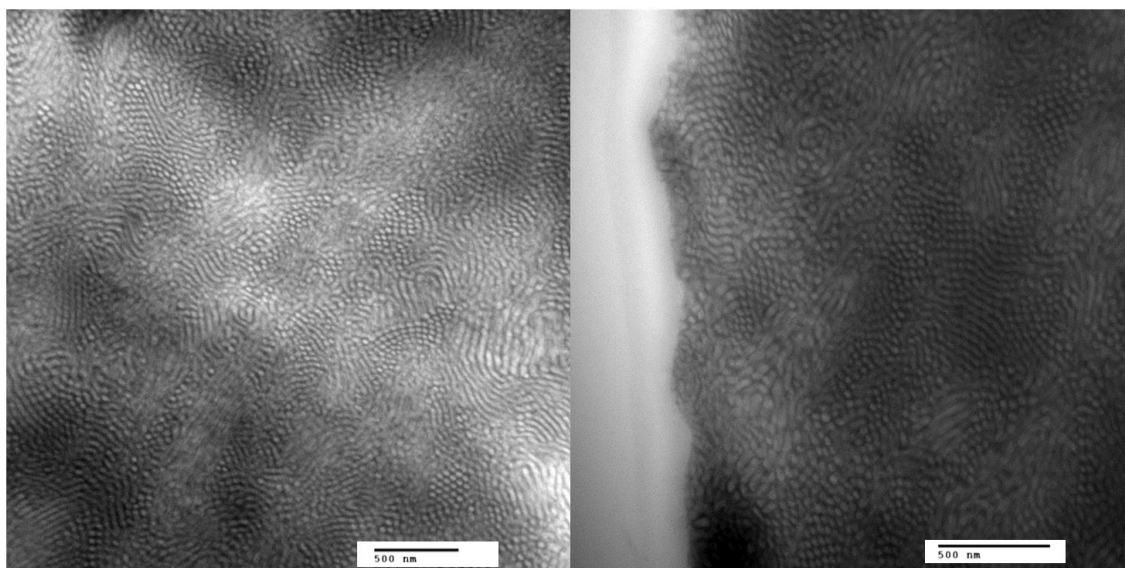
Figure 3.118: TEM images of the copolymer poly(styrene- co -DPE)- block -polybutadiene, PSD-PBd-8, with the butadiene blocks stained black with OsO 4 .
