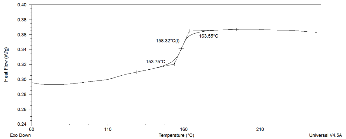
Figure 3.100: DSC thermogram obtained for the poly(styrene- co -DPE) copolymer, PSD-2, heated at a rate of 10 °C/min.
