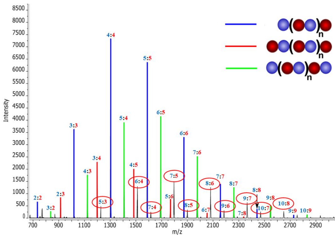
Figure 2.17: MALDI-ToF mass spectrum for the copolymer PSD-6 prepared by the anionic copolymerization (in benzene) of styrene and DPE (monomer molar feed ratio of styrene : DPE = 0.65 : 1.00). The mole ratio of styrene : DPE for any given chain is labelled with styrene in blue and DPE in red.
