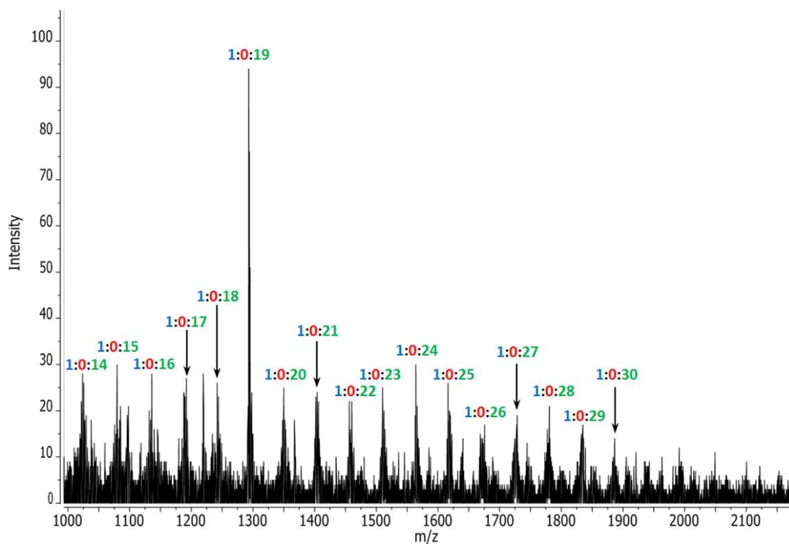
Figure 2.54: MALDI-ToF mass spectrum for the copolymer PBdSD-3d prepared by the anionic copolymerization (in benzene) of styrene, DPE and butadiene (monomer molar feed ratio of styrene : DPE : butadiene = 1.00 : 1.55 : 1.99) after 11.5 hours. The mole ratio of styrene : DPE : butadiene for any given chain is labelled with styrene in blue, DPE in red and butadiene in green.
