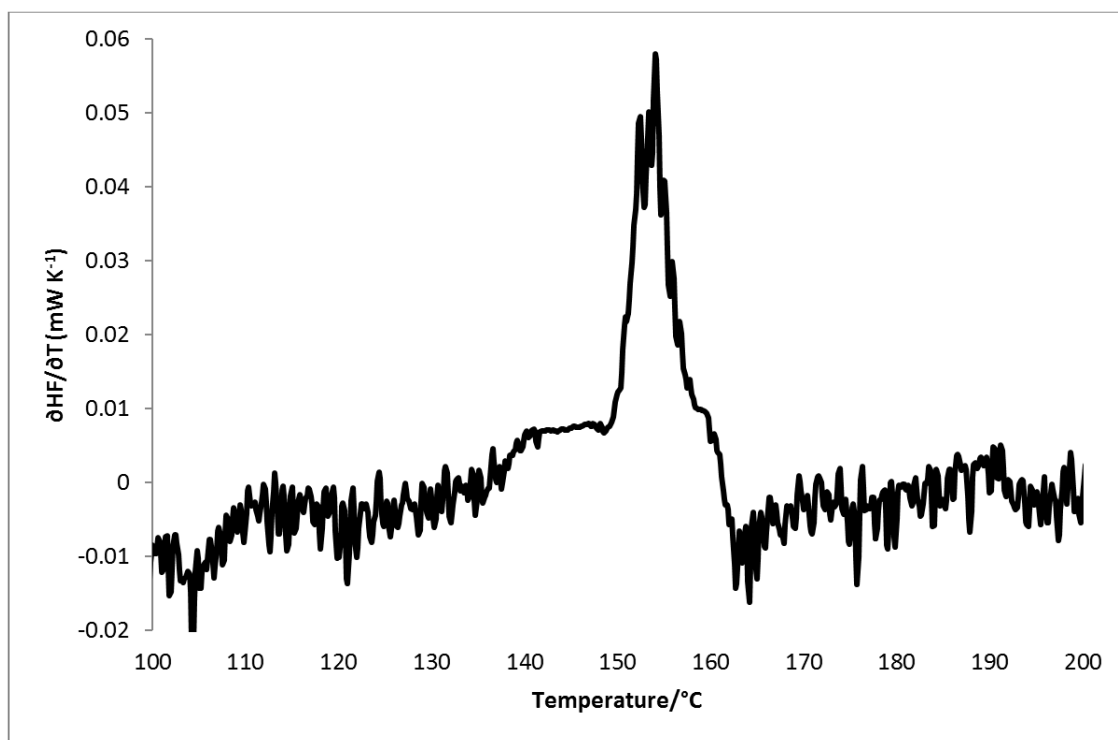
Figure 3.135: Derivative of Heat Flow (HF) vs Temperature (T) for the poly(butadiene- co -styrene- co -DPE) copolymer, PBdSD-10c.
