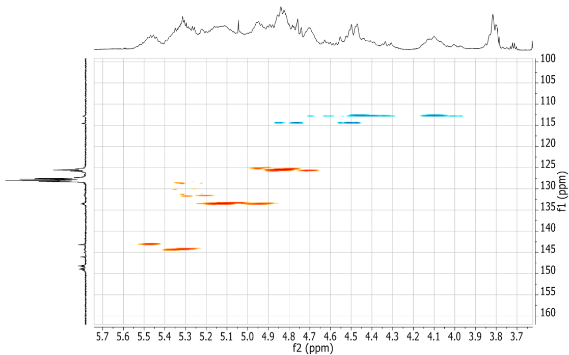
Figure 2.26: HSQCAD NMR spectrum (in \text{CDCl}_3 ) of alkene region of poly(butadiene- co -DPE), PBdD-2.
