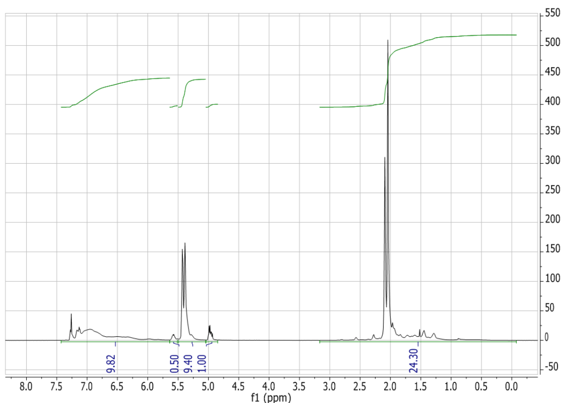
Figure 2.47: ^1H NMR spectrum (in CDCl_3 ) of Poly(butadiene- co -styrene- co -DPE), PBdSD-1d, synthesized in benzene with a molar feed ratio of 1.00 : 0.67 : 5.37 styrene : DPE : butadiene.
