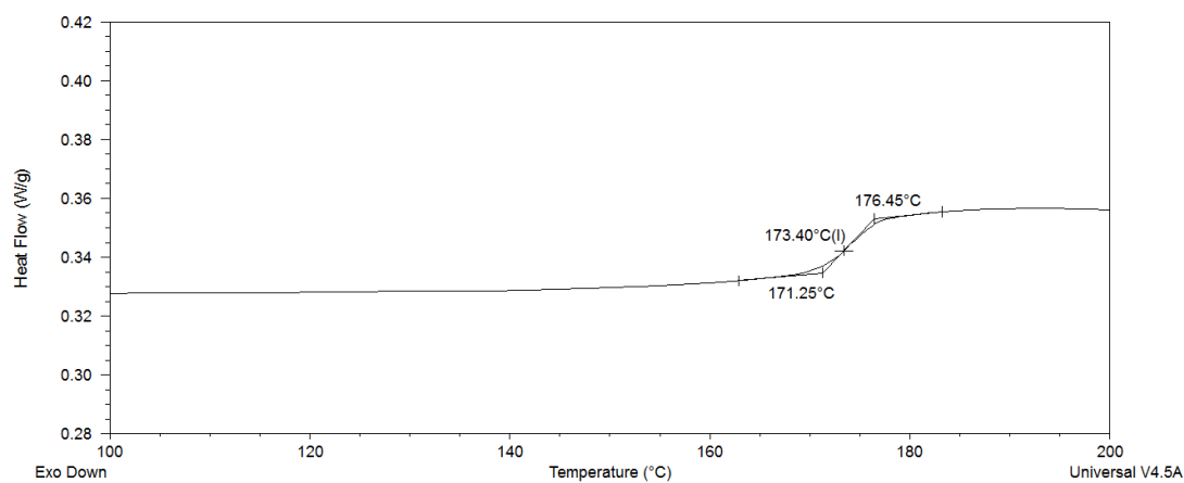
Figure 3.108: DSC thermogram obtained for the poly(styrene- co -DPE)- block -polybutadiene copolymer, PSD-PBd-3, showing the T_g observed upon heating at 40 °C/min.
