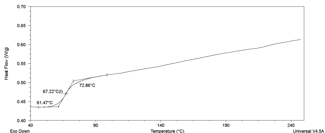
Figure 3.105: DSC thermogram obtained for the poly(butadiene-co-DPE) copolymer, PBdD-2, heated at a rate of 10 °C/min.
