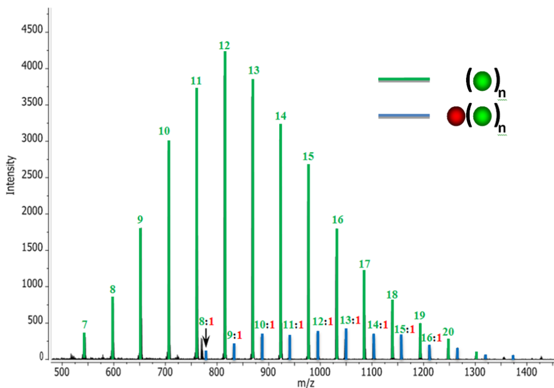
Figure 2.34: MALDI-ToF mass spectrum for the copolymer PBdD-3a prepared by the anionic copolymerization (in benzene) of butadiene and DPE (monomer molar feed ratio of butadiene : DPE = 3.26 : 1.00) after 1.9 hours. The mole ratio of butadiene : DPE for any given chain is labelled with butadiene in green and DPE in red.
