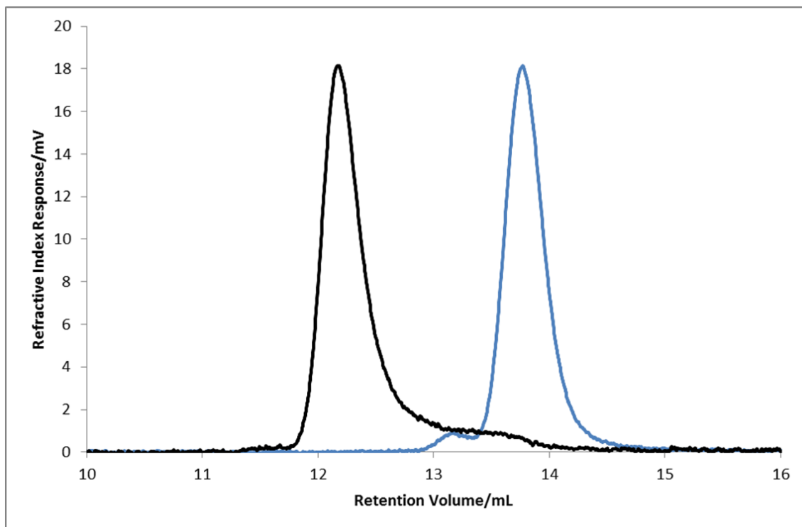
Figure 2.89: Overlay of the SEC chromatograms (refractive index) for the poly(butadiene-co-DPE) copolymers, PBdD-6a (blue) and PBdD-6b (black).
