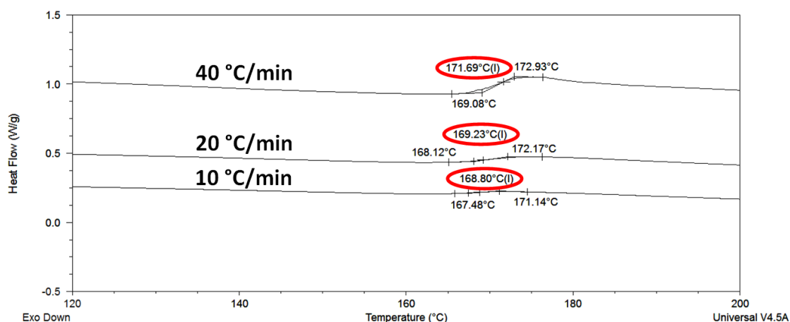
Figure 3.102: DSC thermogram obtained for the poly(styrene-co-DPE) copolymer, PSD-4, using a heating rate of 40 °C/min; 20 °C/min and 10 °C/min with the T_g highlighted by red circles.
