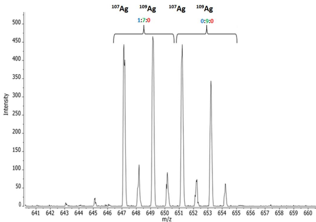
Figure 2.52: Expansion of MALDI-ToF mass spectrum (over the range m/z = 641 - 660 ) for the copolymer PBdSD-3b prepared by the anionic copolymerization (in benzene) of styrene, DPE and butadiene (monomer molar feed ratio of styrene : DPE : butadiene = 1.00 : 1.55 : 1.99) after 1.3 hours. The mole ratio of styrene : DPE : butadiene for any given chain is labelled with styrene in blue, DPE in red and butadiene in green.
