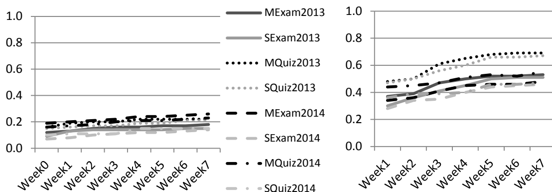
Figure 1: Predictive power of BB track data, and MML and MSL system data for six performance measures
