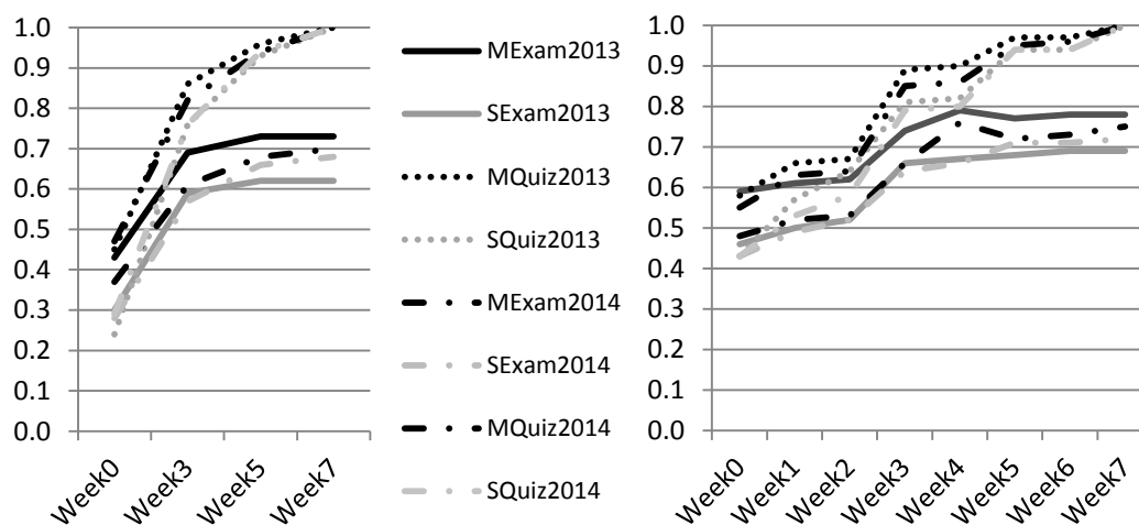
Figure 2: Predictive power of EntryTest and Quiz data, and all data combined for six performance measures
