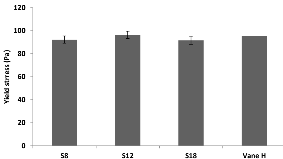
Figure 4 Yield stress of the Carbopol gel using creeping sphere with different sizes compared to the measured data of the same sample using vane H (error bars are due to out of roundness of the lead spheres)
