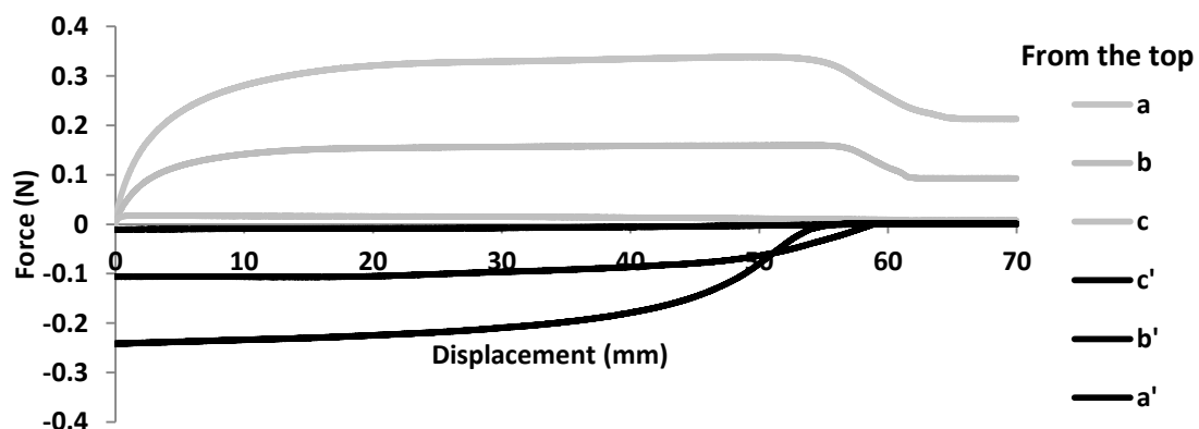
Figure 3 Force vs. displacement for S18 (a, a'), S12 (b, b'), and the thin rod (c, c') within the Carbopol gel at the velocity of 9.58 mm/min (upward and downward movements are shown by grey and black lines, respectively)
