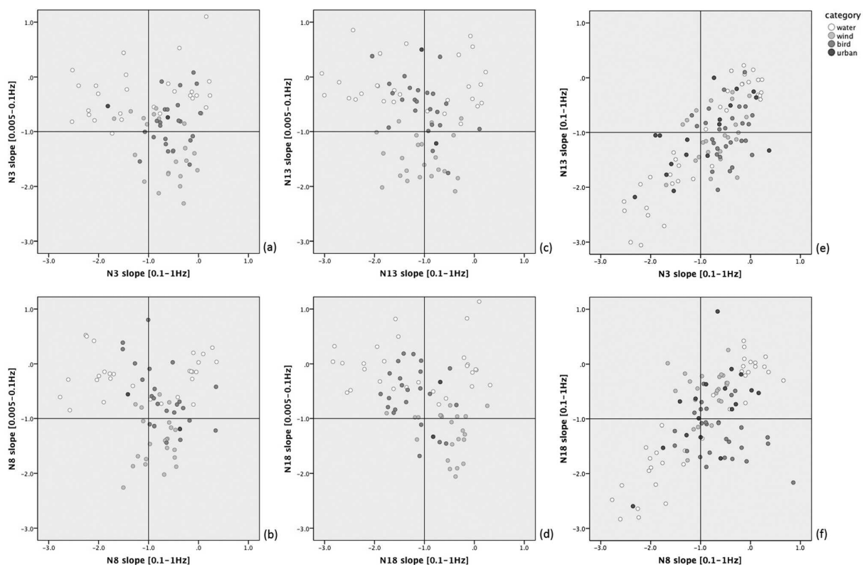
FIG. 5. Characteristics of the four types of sound in terms of the 1/f structure slope indices of specific loudness in the ranges of [0.1–1 Hz] and [0.005–0.1 Hz].
