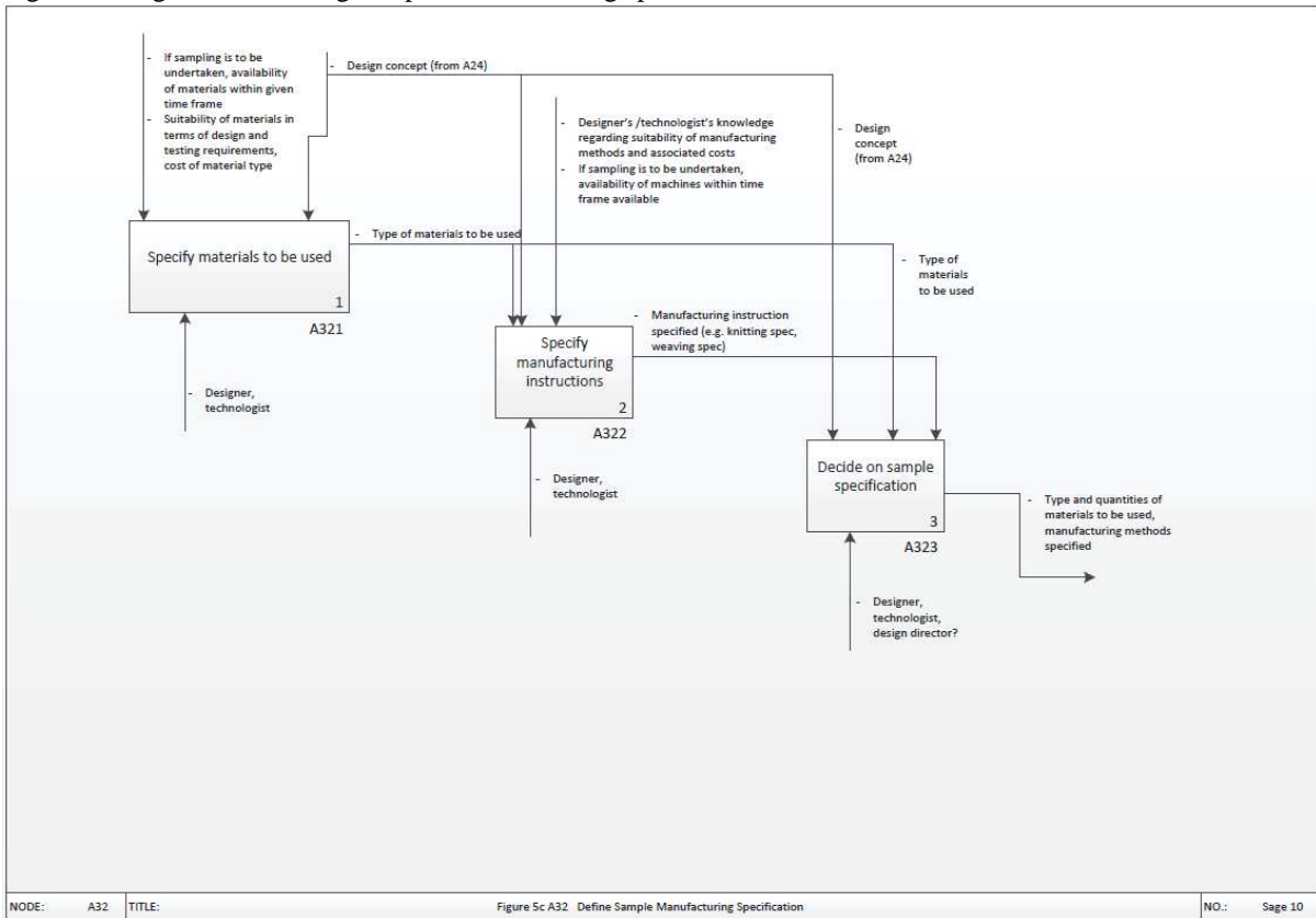
Figure 5c stage A32: defining sample manufacturing specification
