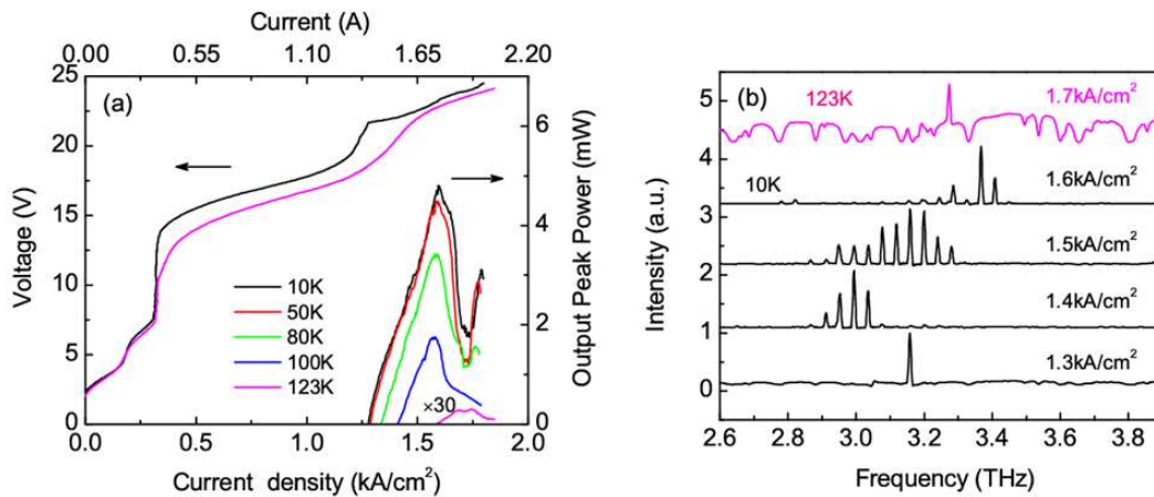
Fig. 2: (a) L–I–V characteristics at various temperatures. (b) Spectra at 10 K and 123 K. The device was 1000 \mu\text{m} long and 110 \mu\text{m} wide, processed into a gold–gold waveguide configuration.
