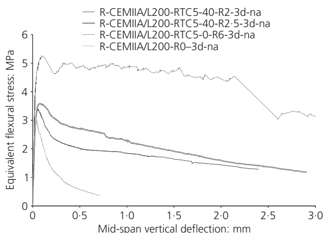
Figure 11. Bending test results for SFR-RCC mixes at various RTSF5-40 dosages in low cement content matrix ( 200 \text{ kg/m}^3 of CEMII/A-L) at age 3 d
