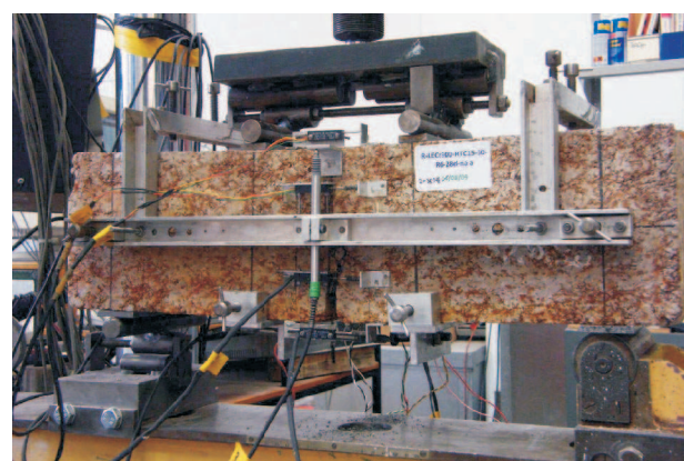
Figure 5. Bending test set-up
