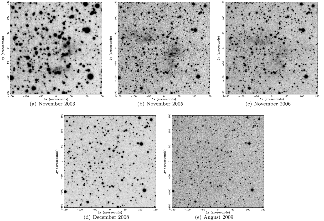
Figure 6. H\alpha images of V2275 Cyg from IPHAS. A faint nebula is apparent in images (a)–(c) but is not present in images (d) and (e). In all images, north is up, east is left.
