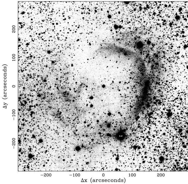
Figure 5. H\alpha image of the nebula surrounding V1315 Aql. The image is 10 arcmin \times 10 arcmin, with north up and east to the left. V1315 Aql is the bright star located at the centre of the image.
