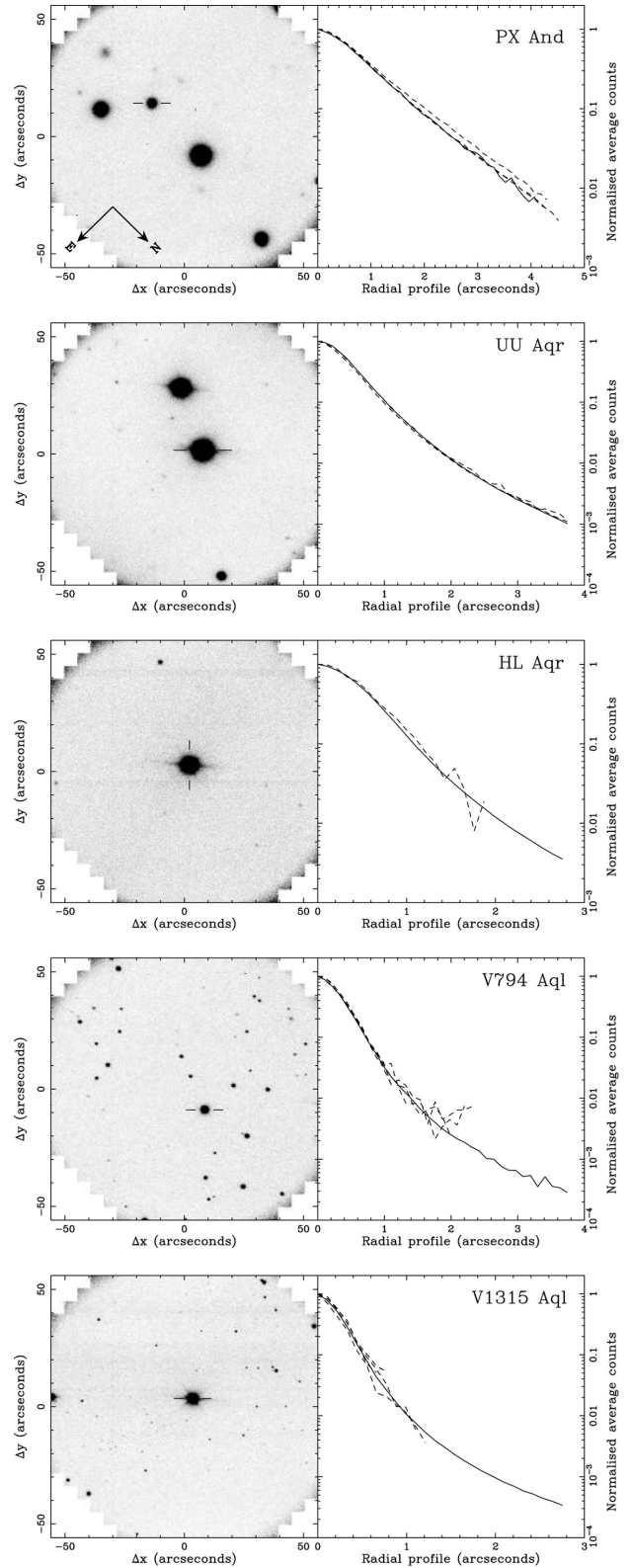
Figure A1. WHT images of our target CVs (left) and the associated radial profiles (right); the solid line is the radial profile of the CV and the dashed lines are field stars. The radial profiles are normalized to unity and plotted until they reach 1\sigma above the background level. The CVs are marked by bars and are located towards the centres of the images. The orientation of all images is the same, and is shown in the image of PX And.
