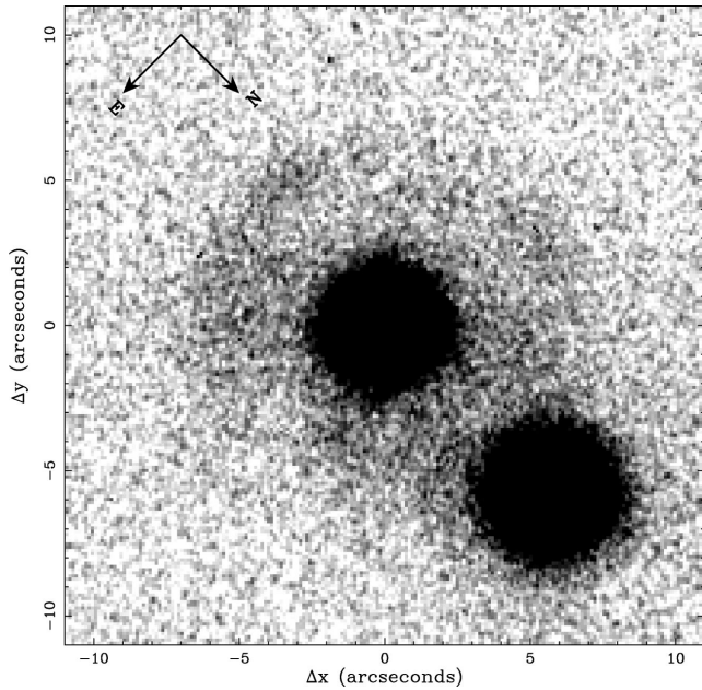
Figure 3. Enlarged image of the BT Mon nova shell. Note that the second star to the lower right is an unassociated foreground/background star.
